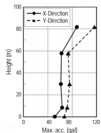
Figure 16. Peak acceleration
