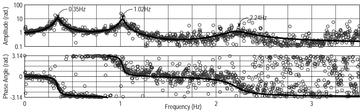
(a) Case 1: derived from records at 20th floor and 1st floor (below isolator)
