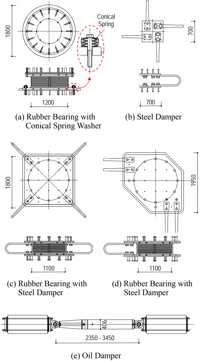
Figure 4. Rubber Bearing and Damper (unit: mm)
