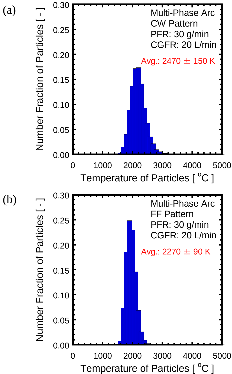
Fig. 4.6 Particle temperature distribution estimated by high-speed camera with different electrode configurations: (a) CW pattern and (b) FF pattern
