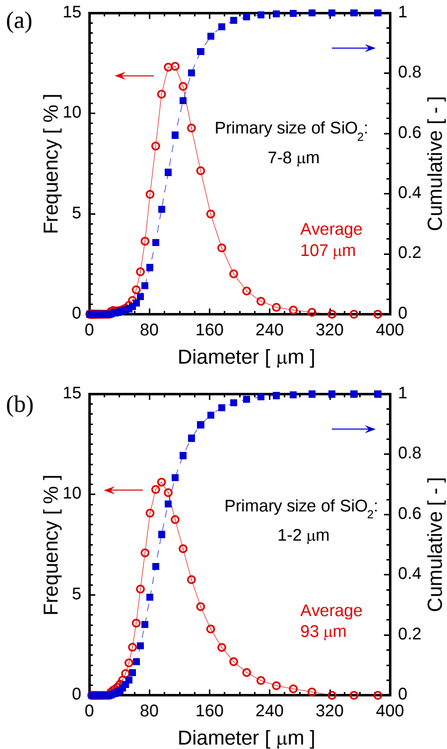
Fig. 6.26 Particle size distributions of melted alkali-free glass particles by hybrid plasma at feed rate of 150 g/min with different raw materials: (a) primary \text{SiO}_2 size of 7~8 \mu\text{m} and (b) primary \text{SiO}_2 size of 1~2 \mu\text{m}
