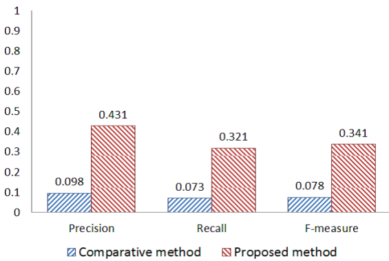
Fig. 6 Comparison of Precision, Recall, and F-measure for all Test Cases
