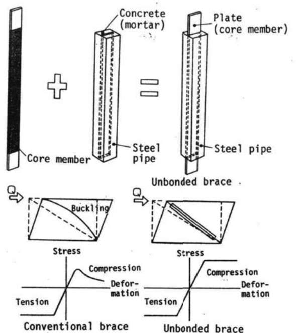
Fig. 3 Unbonded braces
