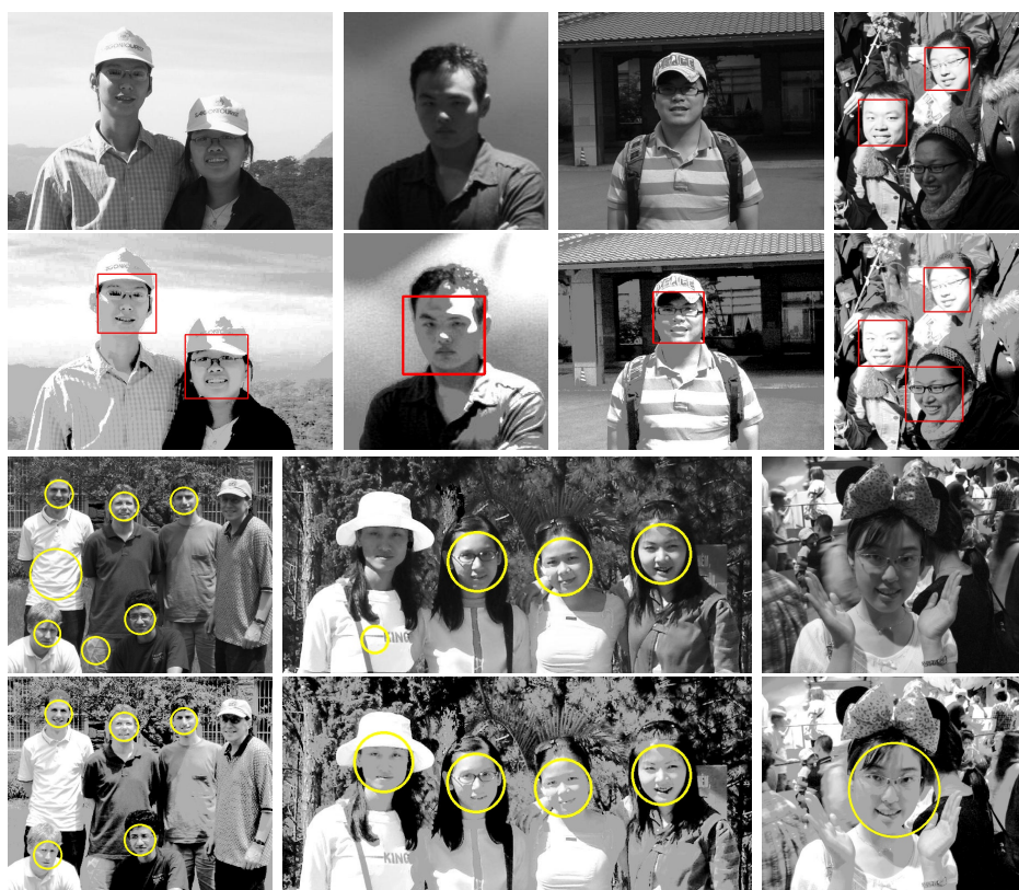
Figure 3.13: Sample results by using the original Haar-like face detector, Haar-like face detector with our normalization method, the original LBP face detector, and LBP face detector with our method (from top row to bottom row).
