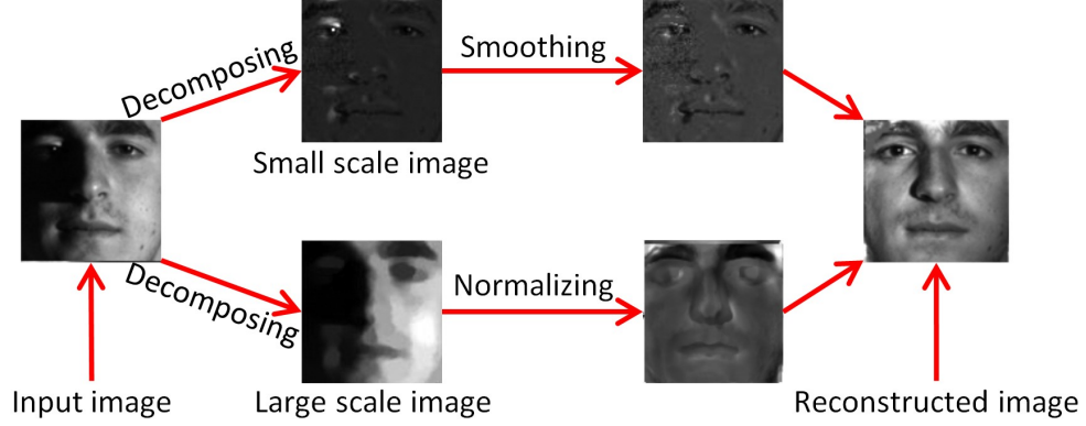
Figure 6.3: Illustration of illumination processing based on large and small scale features.
