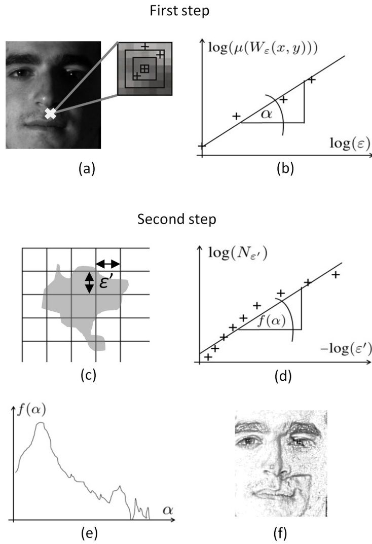
Figure 5.3: Computation of f(\alpha) features. (a) Input image and outcomes ("×") of multifractal measure of a pixel ("×"). (b) Estimation of h_\mu(\alpha) . (c) Process of non-zero-box counting. (d) Estimation of f(\alpha) . (e) Formation of multifractal spectrum. (f) Output face representation ( f(\alpha) -image).
