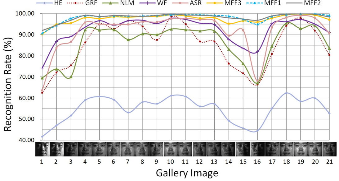
Figure 5.7: Recognition rates versus galleries under different illumination conditions visually shown along the horizontal axis.
