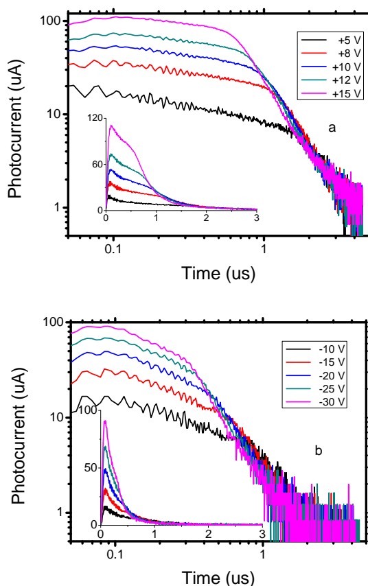
Figure 5-21 Typical transient photocurrent of Tru6 by time of flight at 165°C
