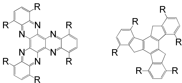
Figure 1-23 Molecular structures of typical triangular discotic liquid crystals, Hexaazatriphenylenes (HATNA) and truxene with bay-located substituents
