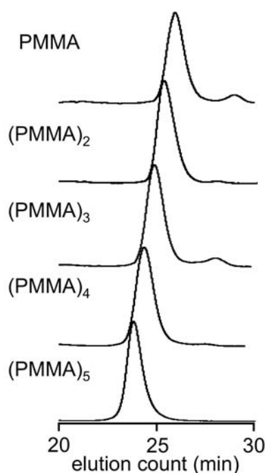
Figure 5-3-18. SEC charts of PMMA, (PMMA) 2 , (PMMA) 3 , (PMMA) 4 , and (PMMA) 5 .
