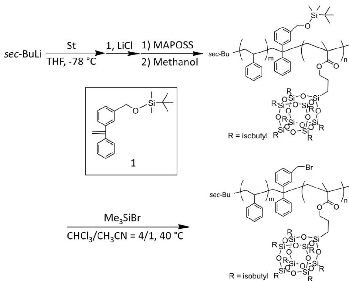
Figure 5-3-19. Synthetic scheme of star-branched PS- b -PI- b -PMAPOSS polymer.
