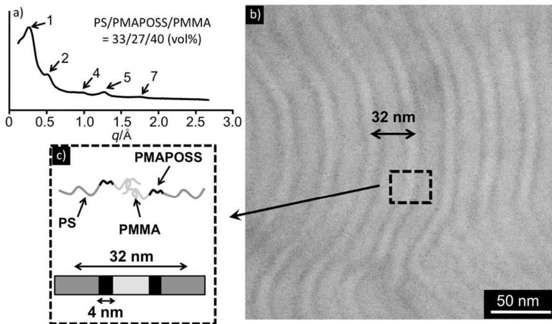
Figure 4-3-10. SAXS profile, TEM image and schematic illustration; a) SAXS profile of PS- b -PMAPOSS- b -PMMA5, b) TEM image of PS- b -PMAPOSS- b -PMMA5, and c) schematic illustration of three-domain layered lamellae.
