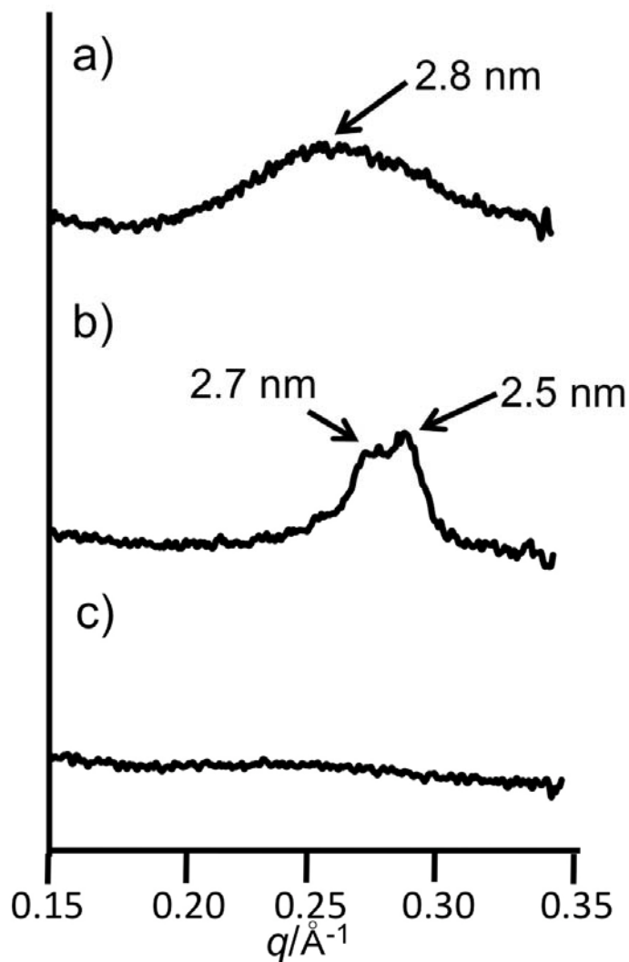
Figure 3-3-11. WAXS profiles of a) PMAPOSS- b -PMAHFC 1 , b) PMAPOSS- b -PMAHFC 2 and c) PMAPOSS- b -PMAHFC 3 .
