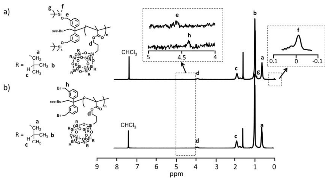
Figure 5-3-27. ^1\text{H} NMR spectra of a) PMAPOSS-OTBS 2 , b) PMAPOSS-BnBr 2 in CDCl 3 .
