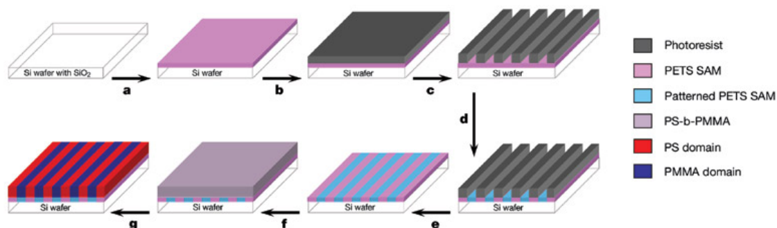
Figure 1-1-5. Schematic representation of the strategy used to create chemically nanopatterned surfaces and investigate the epitaxial assembly of block-copolymer domains. A, A SAM of PETS was deposited on a silicon wafer, b, Photoresist was spin-coated on the SAM-covered substrate, and c, patterned by EUV-IL with alternating lines and spaces of period L_s . D, The topographic pattern in the photoresist was converted to a chemical pattern on the surface of the SAM by irradiating the sample with soft X-rays in the presence of oxygen. E, The photoresist was then removed with repeated solvent washes. F, Asymmetric, lamella-forming PS-b-PMMA copolymer of L_o was spin-coated onto the patterned SAM surface and g, annealed, resulting in surface-directed block-copolymer morphologies. Chemically modified regions of the surface presented polar groups containing oxygen and were preferentially settled by the PMMA block, and unmodified regions exhibited neutral wetting behavior by the block copolymer.
