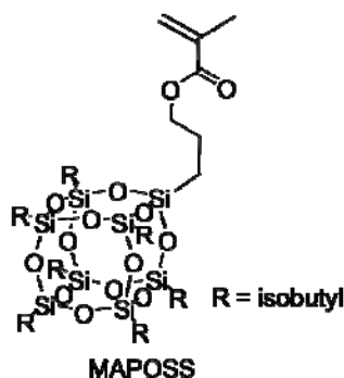
Figure 1-1-11. Chemical structure of POSS-containing methacrylate monomer (MAPOSS).
