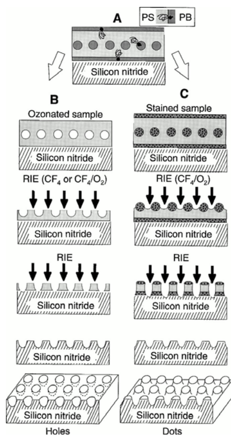
Figure 1-1-8. (A) Schematic cross-sectional view of a nanolithography template consisting of a uniform monolayer of PB spherical microdomains on silicon nitride. PB wets the air and substrate interfaces. (B) Schematic of the processing flow when an ozonated copolymer film is used, which is used to form holes in silicon nitride. (C) Schematic of the processing flow when an osmium-stained copolymer film is used, which is used to form dots in silicon nitride.
