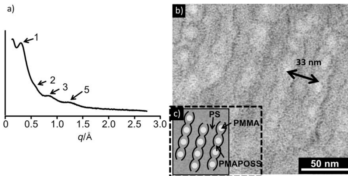
Figure 4-3-9. SAXS and TEM results of PS- b -PMAPOSS- b -PMMA 1, a) SAXS profile, b) TEM image, and c) schematic illustration of microphase separated structure.
