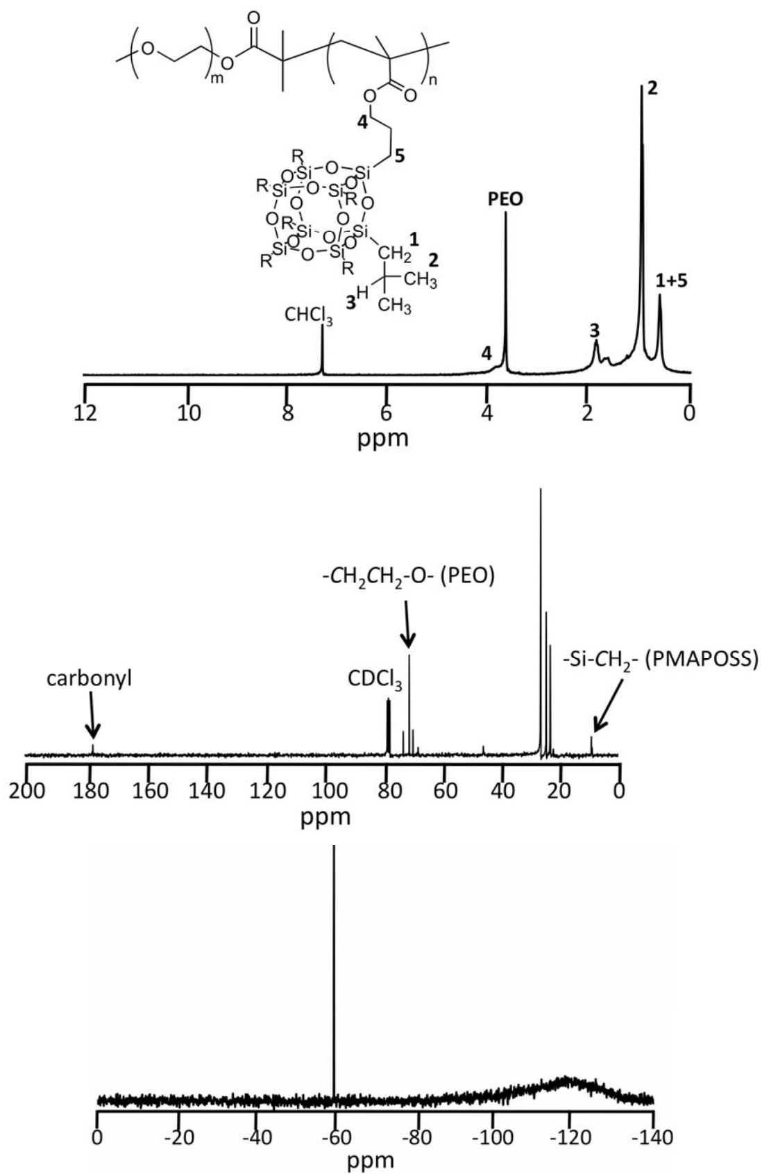
Figure 2-3-2. ^1\text{H} , ^{13}\text{C} and ^{29}\text{Si} NMR spectra of PEO- b -PMAPOSS in \text{CDCl}_3 .
