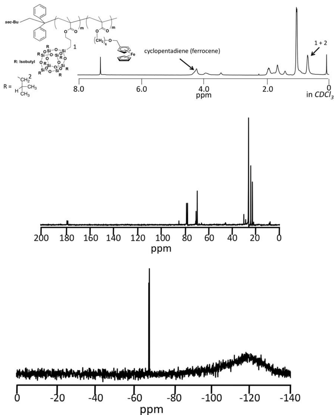
Figure 3-3-7. 1 H, 13 C, and 29 Si NMR spectra of PMAPOSS- b -PMAHFC in CDCl 3 .
