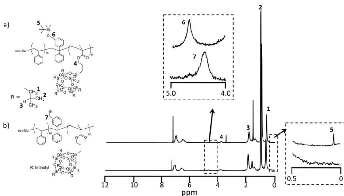
Figure 5-3-20. ^1\text{H} NMR spectra of a) in-chain TBDMSOM-functionalized PS- b -PMAPOSS, and b) in-chain BnBr-functionalized PS- b -PMAPOSS in \text{CDCl}_3 .
