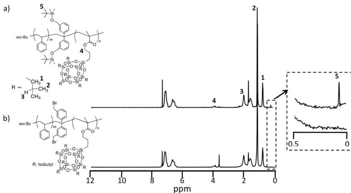
Figure 5-3-31. ^1\text{H} NMR spectra of in-chain difunctionalized a) TBDMMSO 2 PS- b -PMAPOSS, b) BnBr 2 PS- b -PMAPOSS in CDCl 3 .
