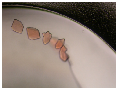
Figure 3-1. Co-crystals of FECH•SA complex. Crystallization was performed using the sitting drop vapour diffusion method, and crystals were grown at 20°C for 3 days.
