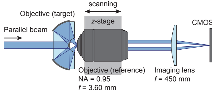
Figure 3.4 Setup to evaluate the ARO by the objective pair method.
