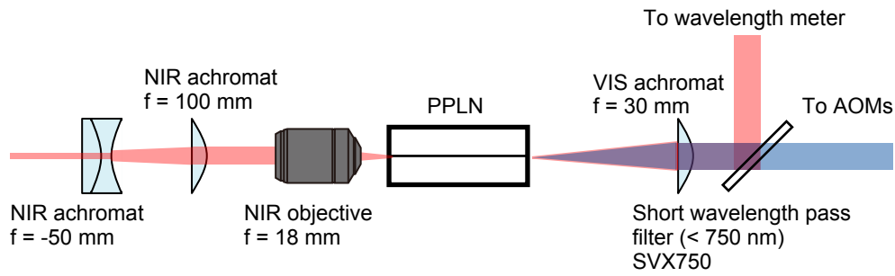
Figure 3.17 Optical arrangement of the PPLN wavelength converter.
