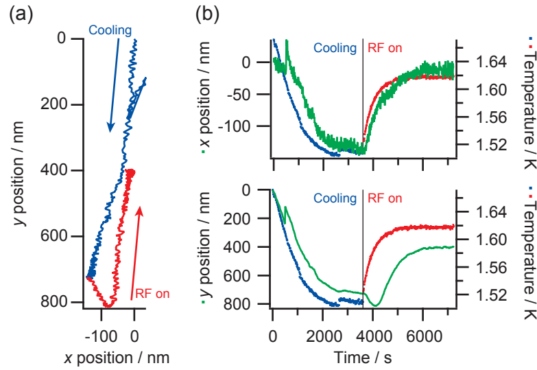
Figure 3.14 Thermal strain of the insert unit monitored for 2 hours in a vacuum cooling process of superfluid helium. (a) Trace of focal position r = (x, y) measured by the reflection imaging system. RF irradiation was applied after 1 hour elapsed from acquisition started. (b) Plots of x and y positions with the temperature.
