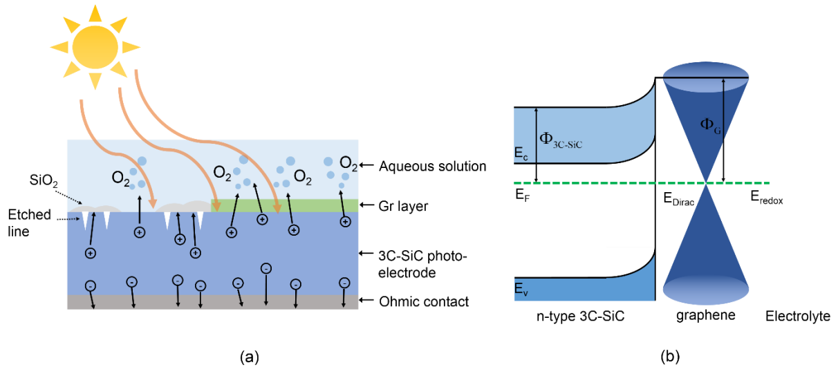
Figure 5.1. (a) Cross-sectional schematic of 3C-SiC photo-electrode in comparison between Gr passivated-surface and exposed-surface to solution. (b) Model of the interface for graphene covered-3C-SiC photo-electrode in solution ( \Phi : work function).
