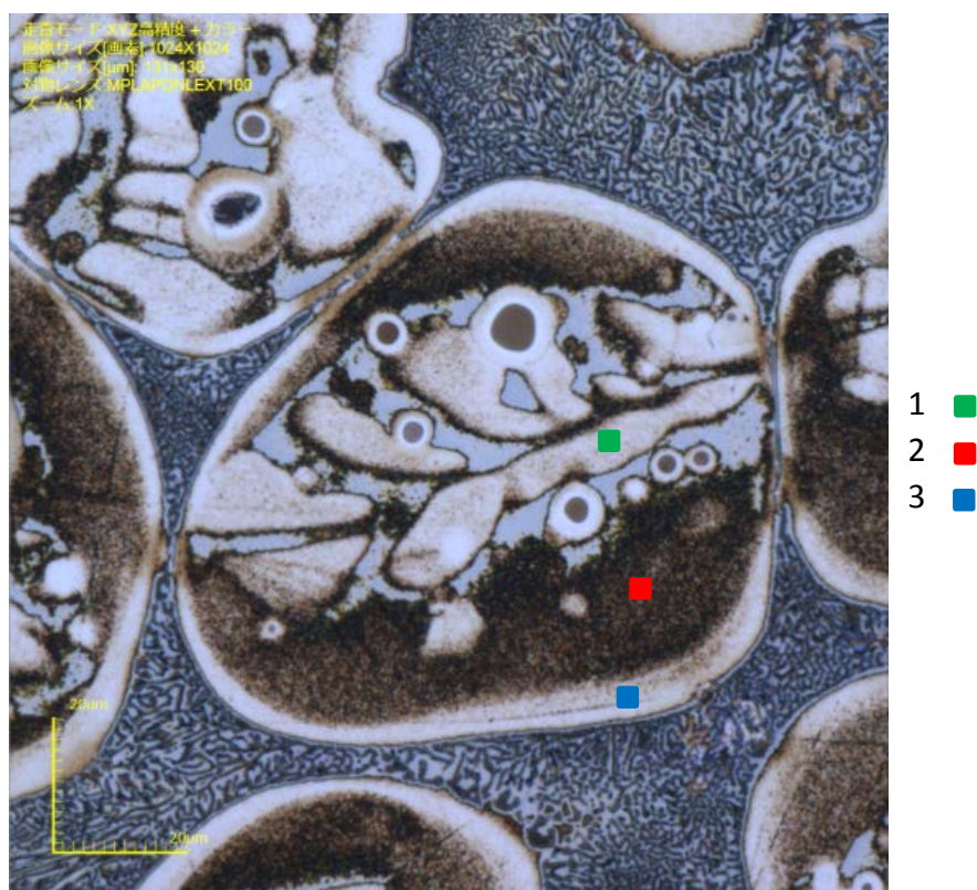
Fig. 5-15. Optical micrograph of the spheroidal grain which was characterized by AFM. The three analysis locations are indicated by three points.
