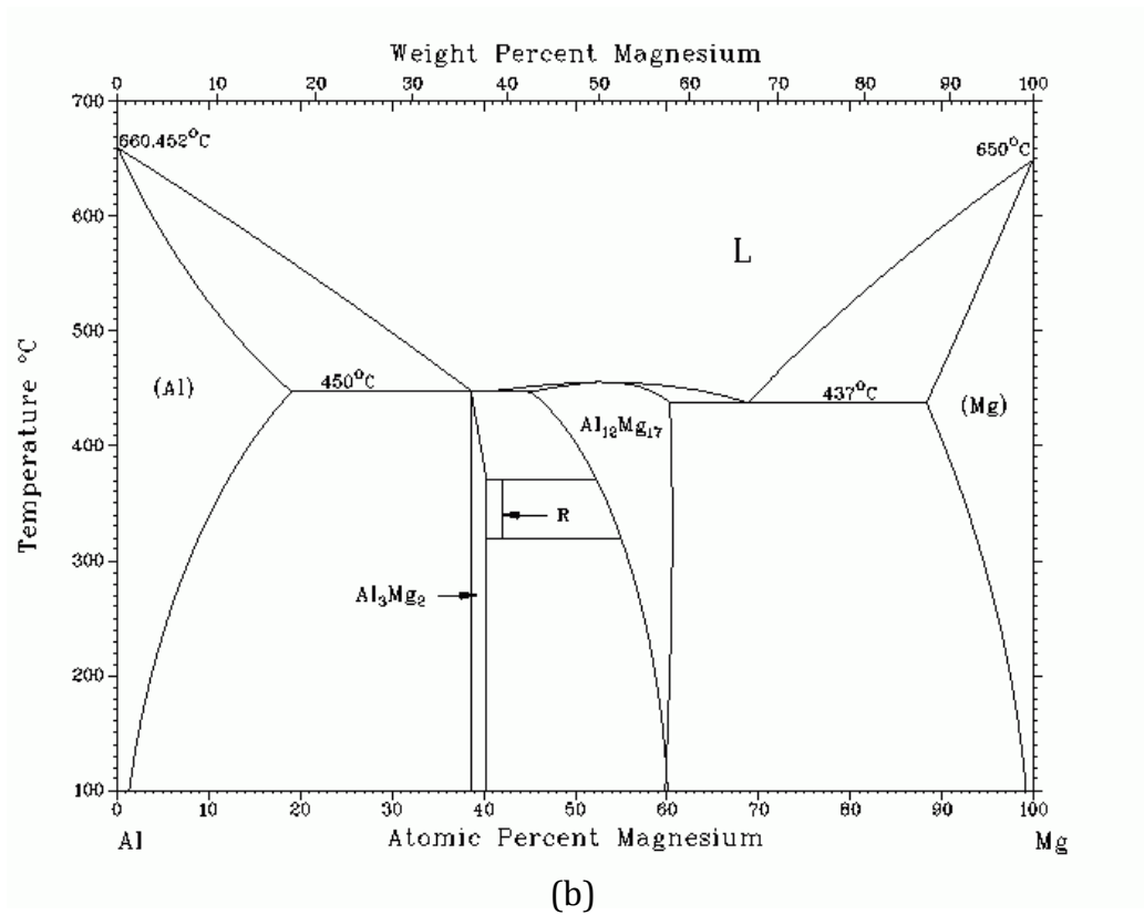
Fig. 2-8. Al-Si (a) and Al-Mg (b) phase diagrams
