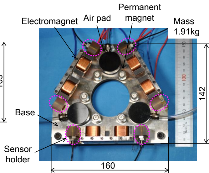
Fig. 3.10 Prototype stator
