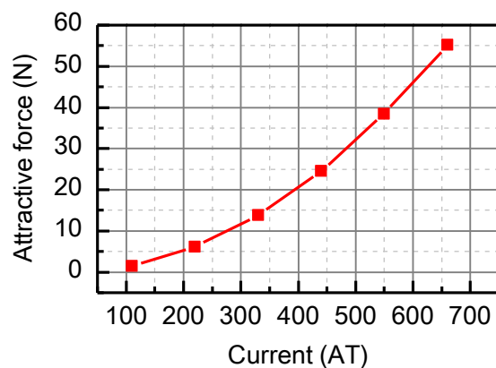
Fig. 2.14 Simulated attractive force
