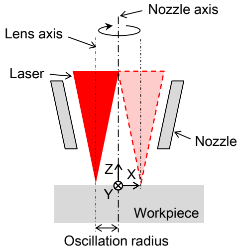
Fig. 5.7 Orbital oscillation
