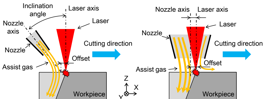
Fig. 2.2 Laser cutting with separated nozzle
