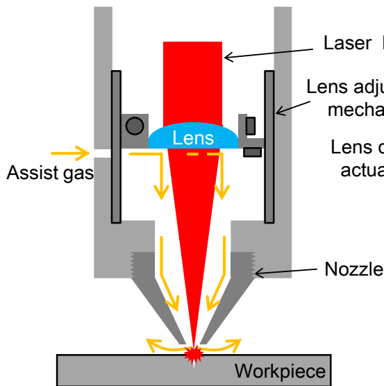
Fig. 2.6 Conventional laser head
