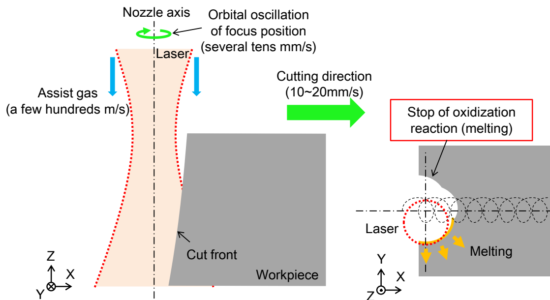
(b) Stop of a part of oxidization combustion
