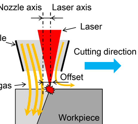
Fig. 2.3 Off-axis laser cutting
