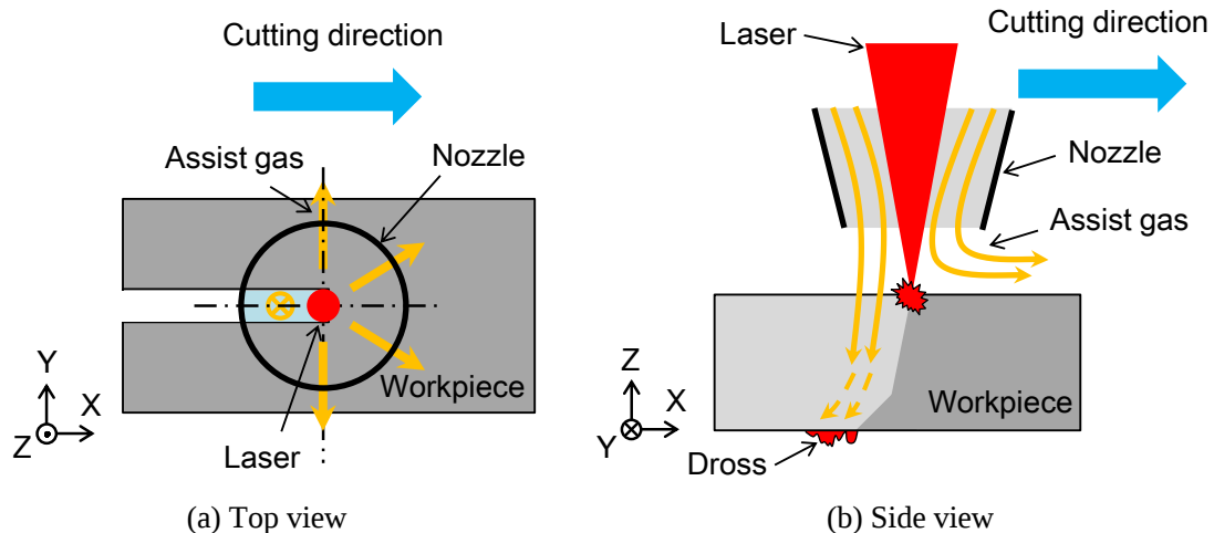
Fig. 2.1 Assist gas flow with co-axial setting of laser beam and nozzle axes
