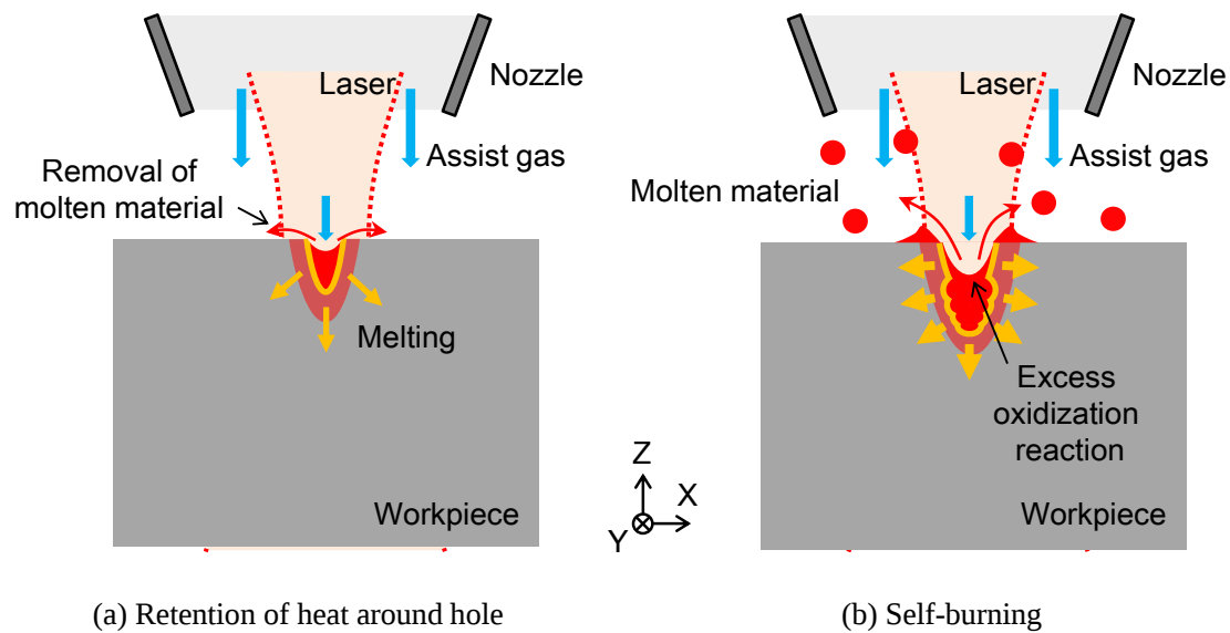
Fig. 1.8 Self-burning mechanism
