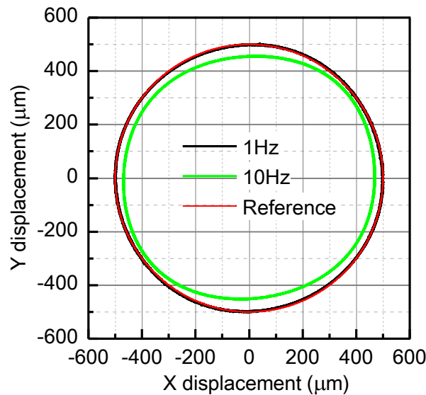
Fig. 2.24 Circle trajectory tracking control (500 \mu\text{m} radius)
