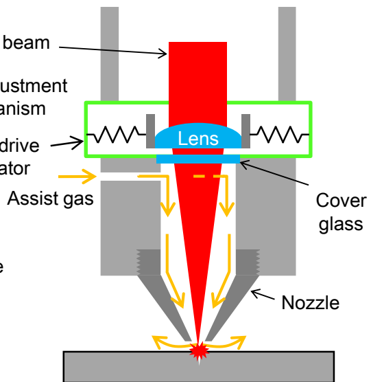
Fig. 2.7 Laser head with lens drive actuator
