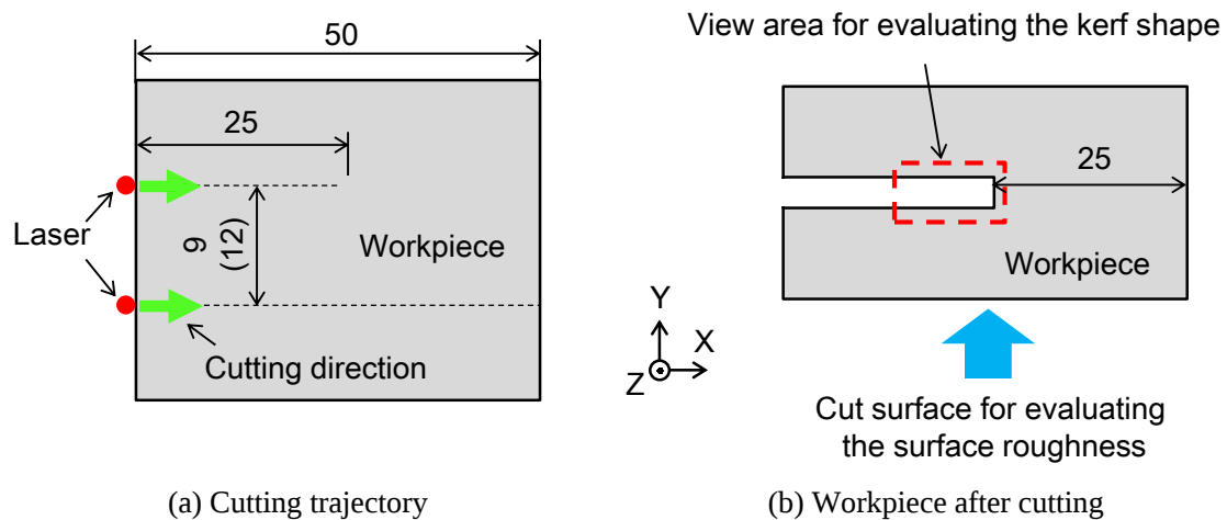
Fig. 4.7 Method for cutting workpiece
