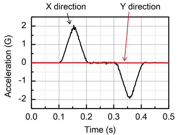
Fig. 2.26 Acceleration of the laser head (accelerated in the X direction)
