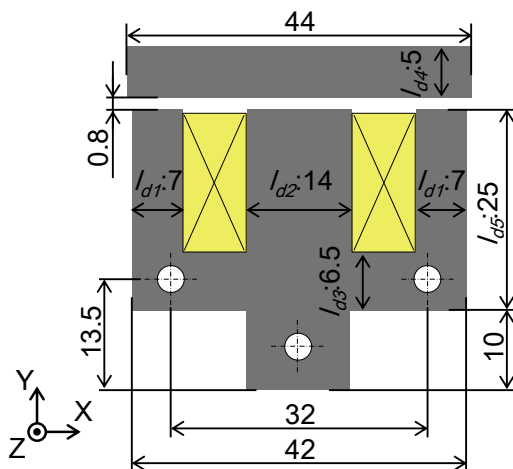
Fig. 2.13 Simulation model of electromagnetic field analysis (t=18mm)
