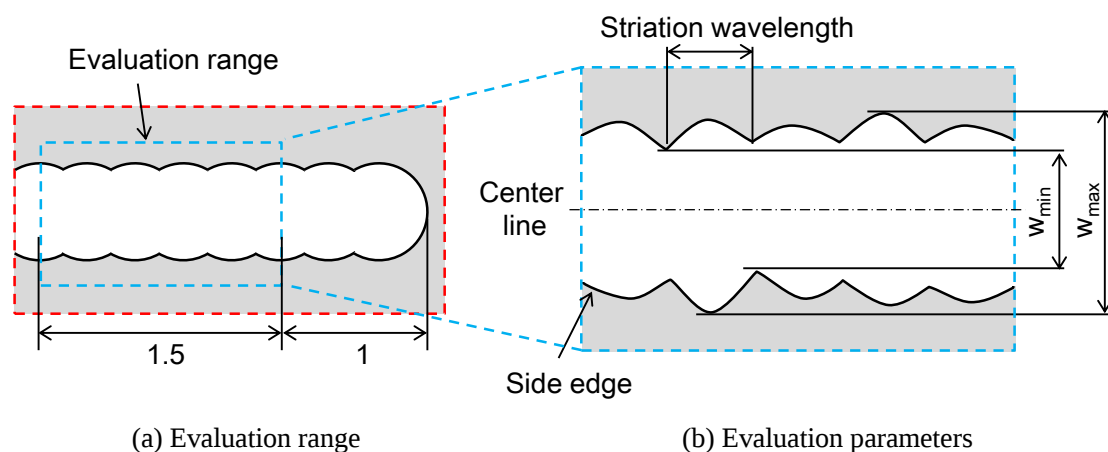
Fig. 4.8 Evaluation of the kerf shape
