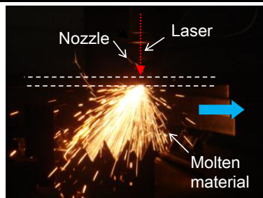
(a) Without off-axis ( 1,300\text{mm/min} )
