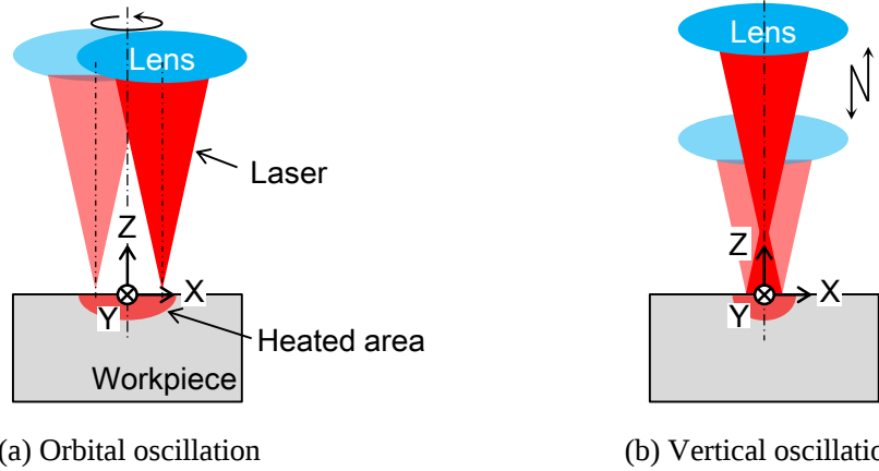
Fig. 5.2 Concepts of laser piercing with oscillation of laser focus position
