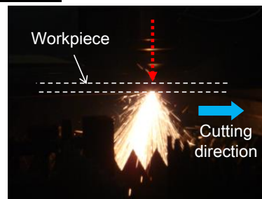
(b) With off-axis of 150\mu\text{m} ( 1,500\text{mm/min} )
