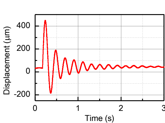
Fig. 3.13 Impulse response (X direction)
