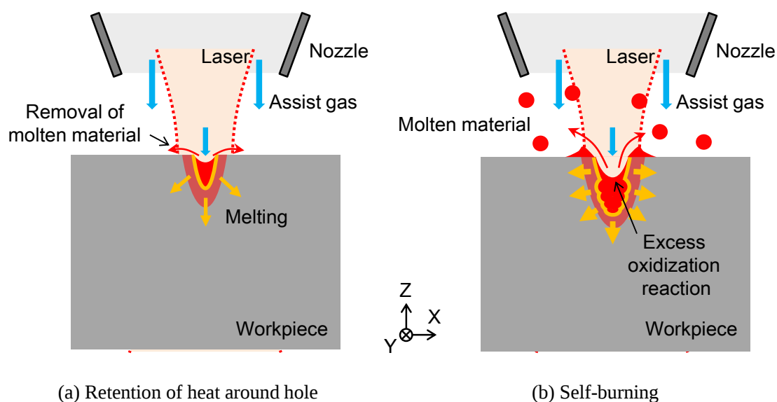
Fig. 1.8 Self-burning mechanism
