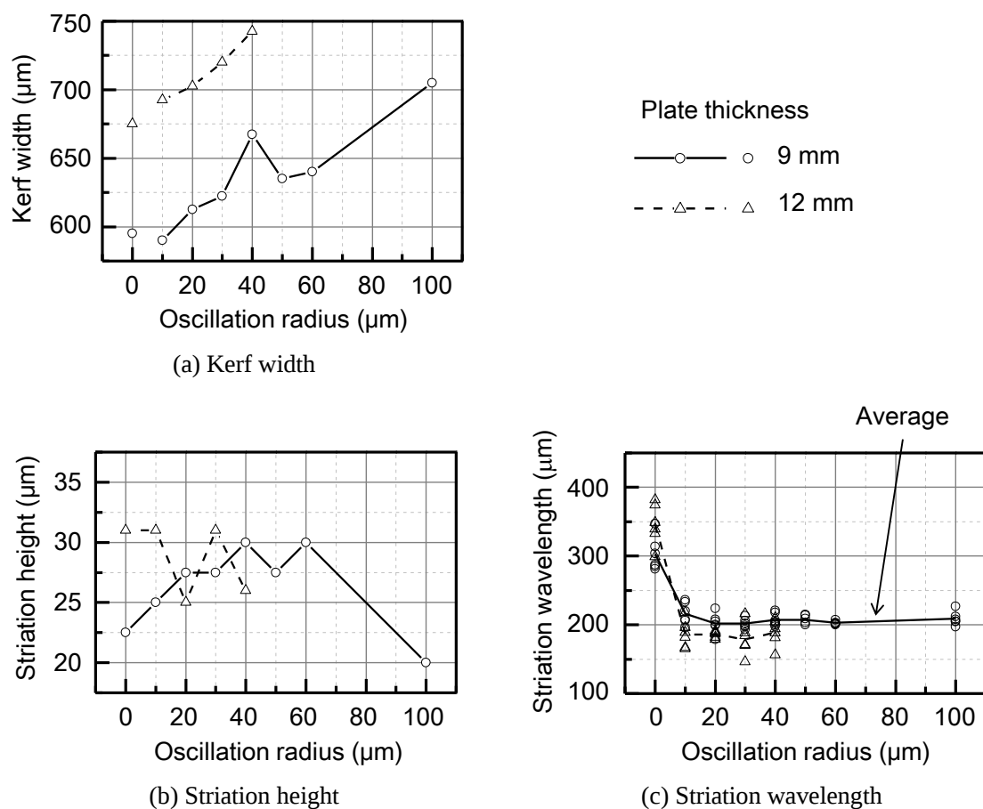
Fig. 4.10 Relationship between the orbital oscillation radius and striation structure (orbital oscillation frequency: 80\text{Hz} )
