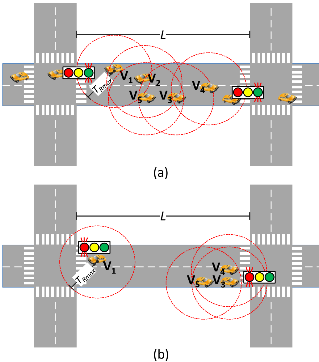
Figure 2.1. Vehicle distribution examples for (a) fully connected network and (b) fragmented network.
