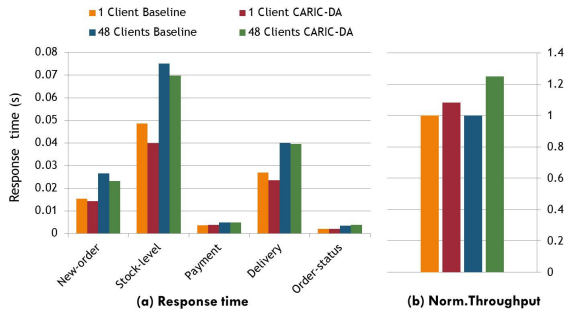
Fig. 13 Performance for the TPC-C benchmark.
