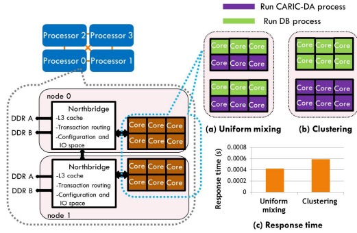
Fig. 3 Core affinity in the system.
