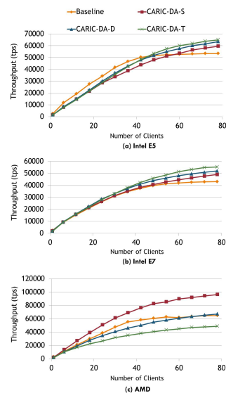
Fig. 9 Scalability of different CARIC-DA systems.
