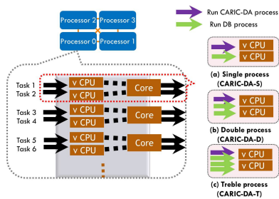
Fig. 5 Different CARIC-DA systems.
