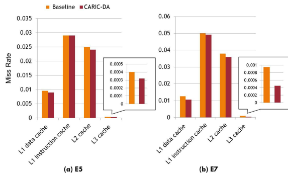
Fig. 7 Cache miss rate on different platforms.
