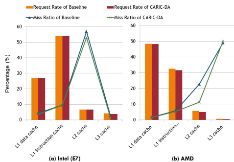
Fig. 8 Cache miss ratio and request rate of different platforms.
