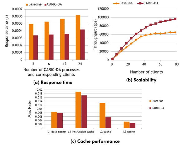
Fig. 4 Advantage of CARIC-DA system.
