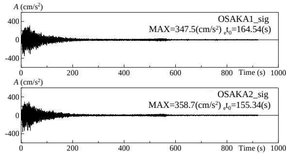
Figure 11. Time history of input earthquakes
