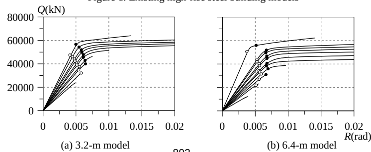
Figure 2. Static analysis results
