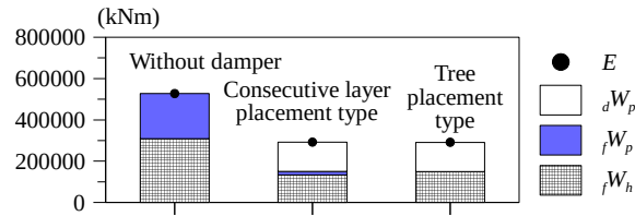
Figure 8. Energy distribution of 3.2-m model
