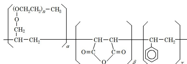
Fig. 1 Molecular structure of P- n .
