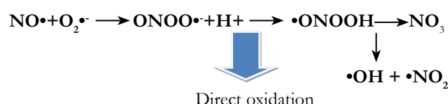
Figure 18. Production of peroxynitrite anion radical ( \text{ONOO}^{\bullet-} ) from NO radical combines with superoxide anion radical ( \text{O}_2^{\bullet-} )
