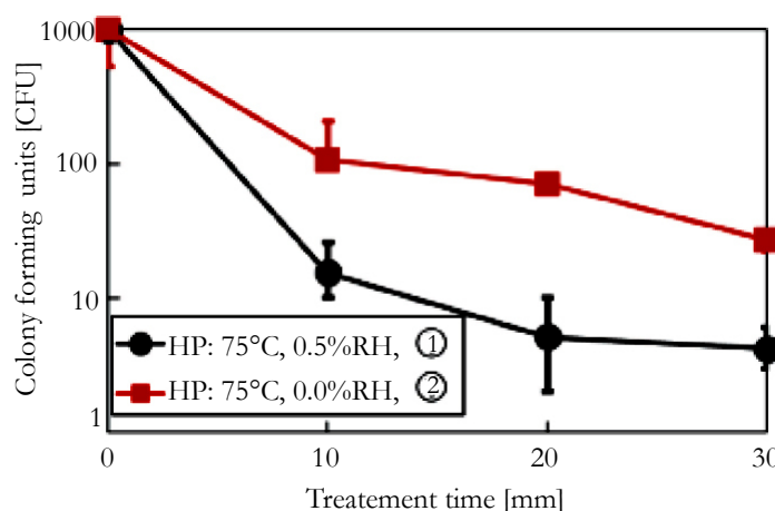
Figure 11. Relationship between treatment time and colony forming units at water vapor supply portion of ①, RH of 0.5% and 0% and temperature at 75°C 0.5% RH was found to be the most appropriate.
