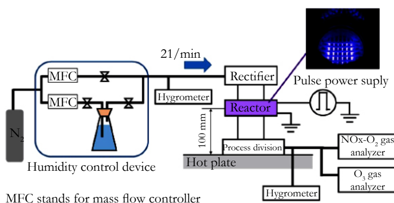
Figure 2. Plasma generation part.
