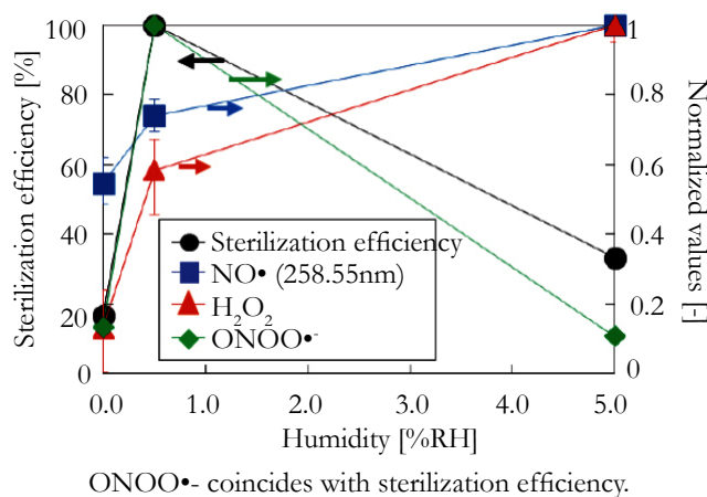
Figure 22. Relationship between sterilization efficiency and relative humidity (RH) for NO radical, H 2 O 2 or ONOO•-.
