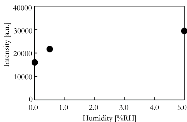
Figure 16. Relationship between H 2 O 2 concentration and relative humidity (RH).
