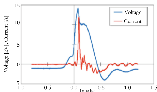
Figure 3. Waveform of voltage and that of current when plasma generated under the experimental conditions presented in Table 1.
