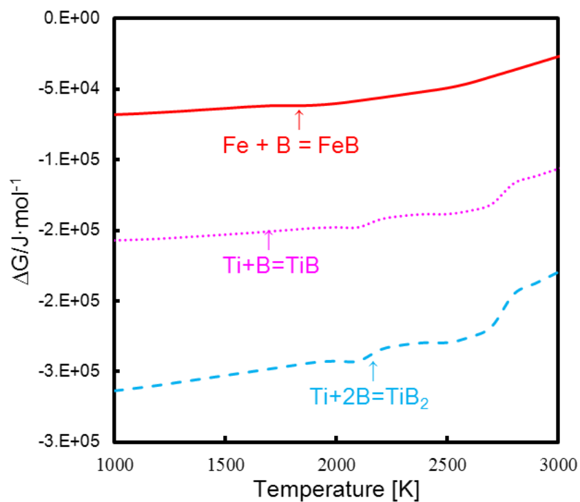
Fig.9 Gibbs free energy of generating FeB, TiB and TiB 2 .
