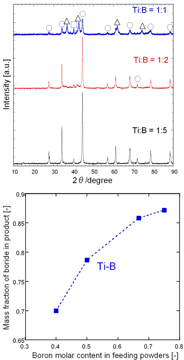
Fig. 15 XRD patterns and mass fraction of prepared nanoparticles at different boron content in feed powders; Feed rate: 120 mg/min, Carrier gas: 1 L/min. (○: \text{TiB}_2 △: \text{TiB} □: \text{Ti} )
