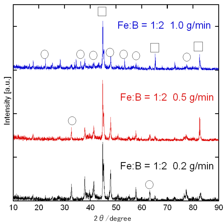
Fig. 7 XRD patterns of product with different powder feed rate at fixed initial composition of Fe:B = 1:2. ( \circ : FeB \square : Fe)
