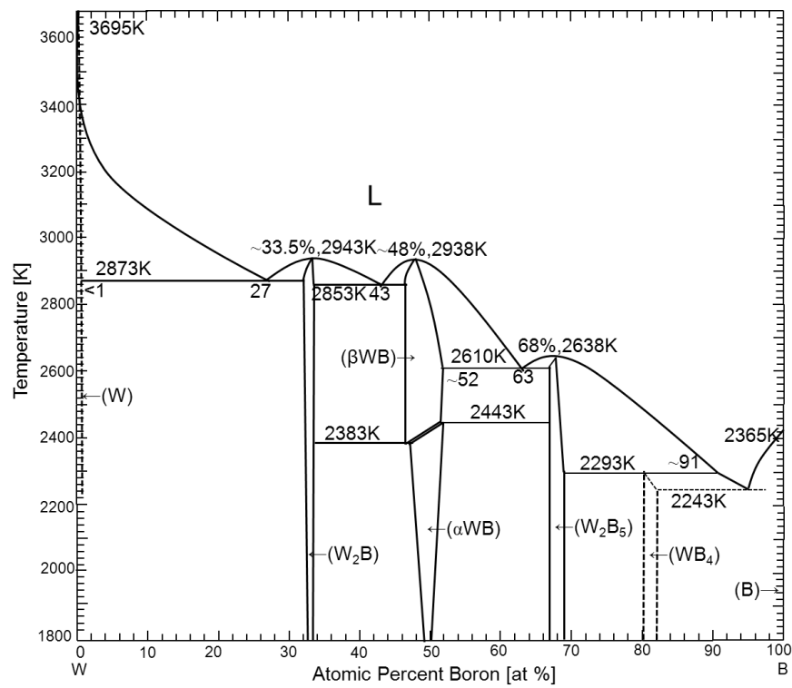
Fig. 4 Binary W-B phase diagram.
