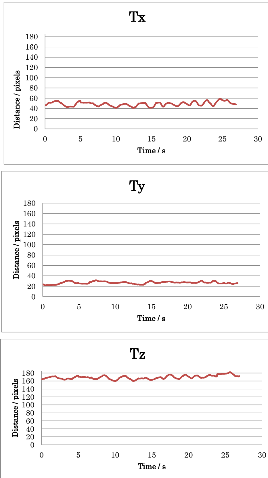
Figure 24 Estimated translation values in x, y and z directions (top to bottom)
