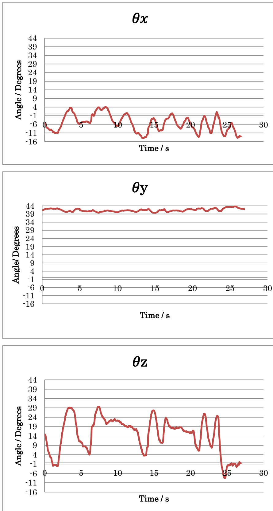
Figure 23 Estimated pose angles for \theta_x , \theta_y and \theta_z (top to bottom)
