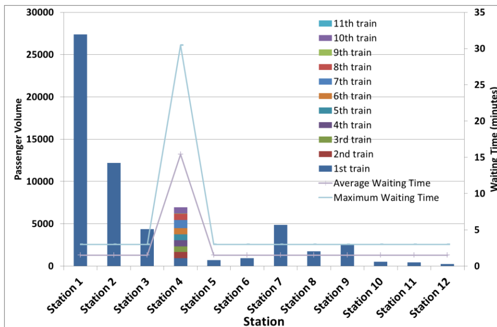
Figure 6.24. Waiting time for constant operations
