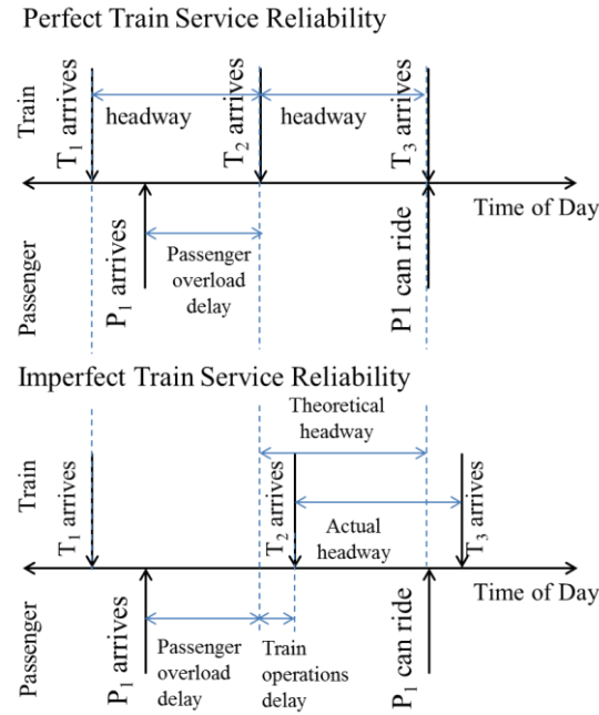
Figure 6.23. Definition of passenger overload delay
