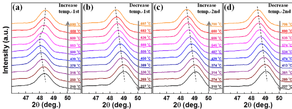
Fig. 6-8 In-situ XRD profiles of TiN(30 nm)/CoPt(10 nm) with N 2 flow rate ratio of 20% during the deposition of CoPt: (a) Increasing temperature in the first cycle, (b) decreasing
