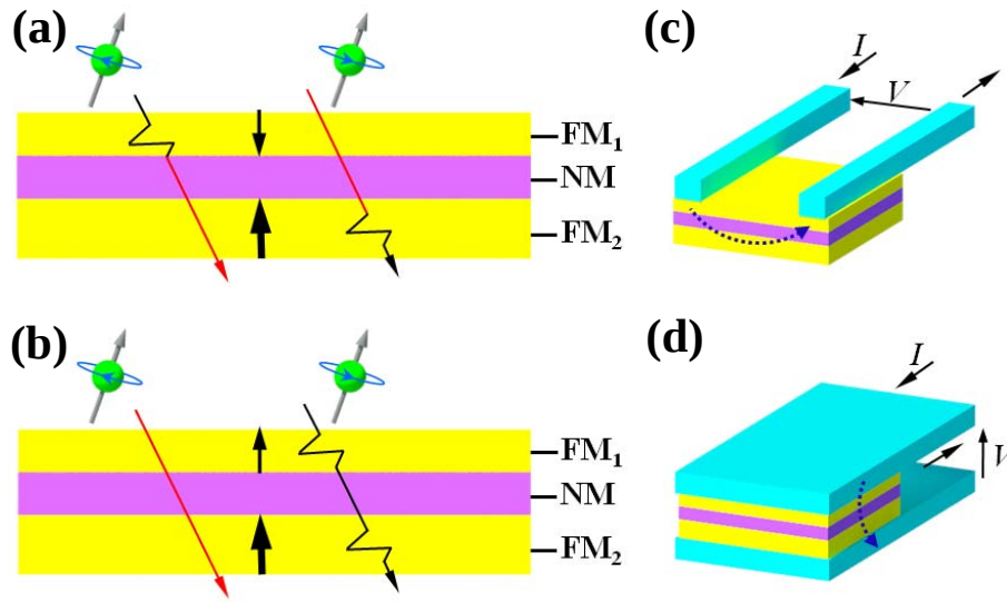
Figure 1-9 Schematic illustrations of (a) electron scattering with parallel magnetization direction, (b) electron scattering with antiparallel magnetization direction, (c) current in plane (CIP) set up of spin valve, (d) current perpendicular to plane (CPP) set up of spin valve.
