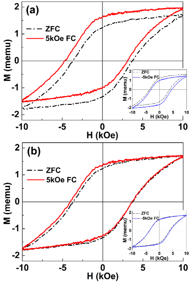
Figure 5-1 Perpendicular M-H curves of \text{TiN}(5 \text{ nm})[\text{CoPt}(4 \text{ nm})/\text{TiN}(2 \text{ nm})]_{15} multilayer film after 5 kOe field cooling from 350 °C to room temperature (sample was annealed at 800 °C before applying FC). (a) before correcting the vertical shift (inset: -5 kOe FC was applied). (b) after correcting the vertical shift (inset: -5 kOe FC was applied).
