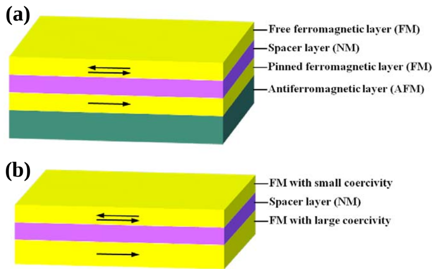
Figure 1-8 Schematic illustrations of (a) spin valve (b) pseudo spin valve.
