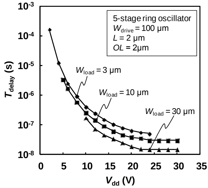
Fig. 4.4 Measured characteristics of 5-stage ring oscillator consist of diode connected type inverters: dependence of T_{\text{delay}} on W_{\text{load}} .
