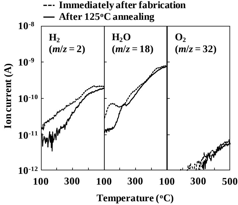
Fig. 2.6 Thermal desorption spectra of \text{H}_2 , \text{H}_2\text{O} and \text{O}_2 from a-InGaZnO films immediately after deposition and after 3 hours of 125^\circ\text{C} annealing.
