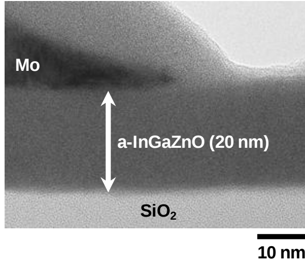
Fig. 3.5 Cross-sectional transmission electron micrograph of a-InGaZnO TFT.
