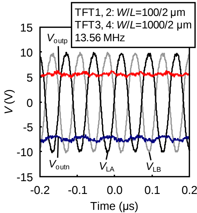
Fig. 3.9 Measured full-wave rectifying characteristics of four-TFT a-InGaZnO rectifier for 13.56-MHz wired input.
