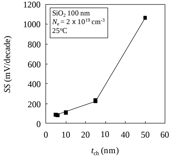
Fig. 2.9 Dependence of subthreshold slope (SS) on channel layer thickness ( t_{\text{ch}} ) measured at 25°C.
