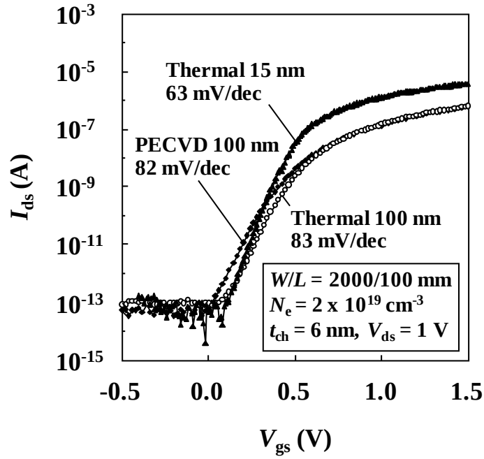
Fig. 2.10 I_{ds} - V_{gs} curves of a-InGaZnO TFTs with various \text{SiO}_2 gate insulators measured at 25^\circ\text{C} .
