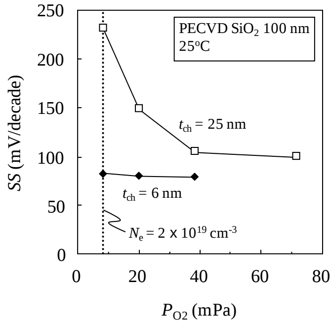
Fig. 2.7 Dependence of subthreshold slope (SS) on oxygen partial pressure ( P_{\text{O}_2} ) measured at 25°C.
