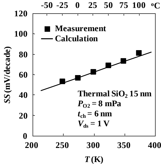
Fig. 2.12 Dependence of SS on T . The linear curve is calculated data using equation (2.8) by substituting C_{\text{itf}} + C_{\text{itb}} + 2C_{\text{sg}} + 2C_{\text{fr}} = 1.17 \times 10^{-4} \text{ F/m}^2 .
