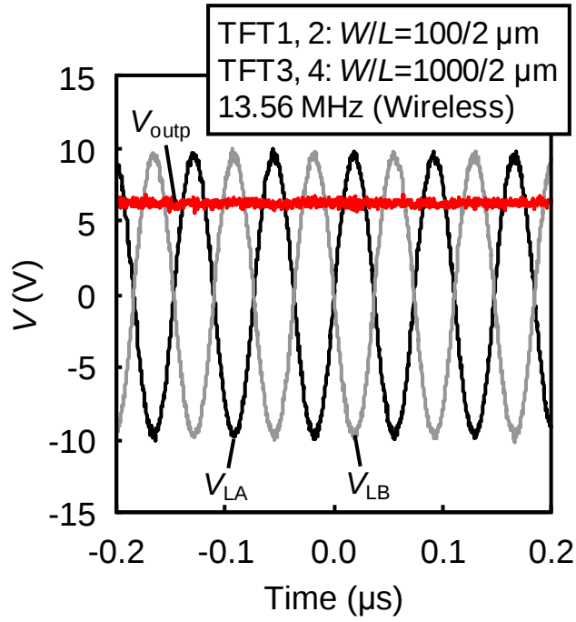
Fig. 3.13 Measured full-wave rectifying characteristics of four-TFT a-InGaZnO rectifier for 13.56-MHz wireless input.
