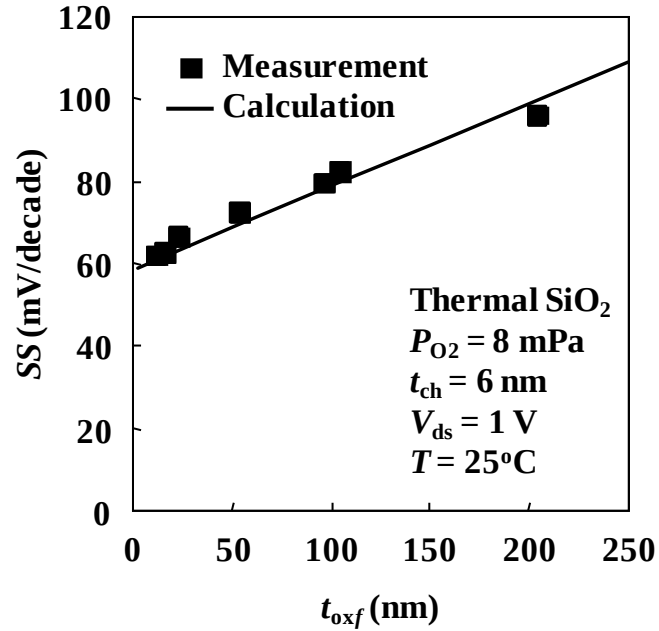
Fig. 2.11 Dependence of SS on t_{oxf} at 25^\circ\text{C} . The linear curve is calculated data using equation (2.8) by substituting C_{itf} + C_{itb} + 2C_{sg} + 2C_{fr} = 1.17 \times 10^{-4} \text{ F/m}^2 .
