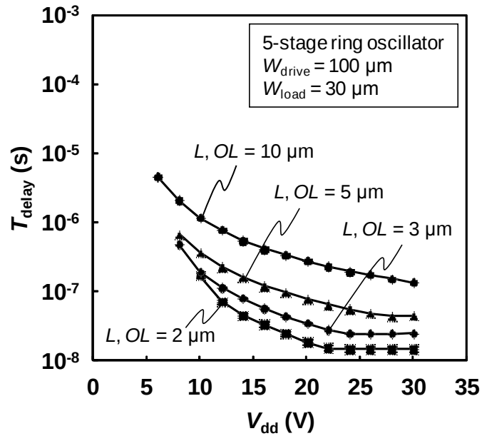
Fig. 4.5 Measured characteristics of 5-stage ring oscillator consist of diode-connected type inverters: dependence of T_{\text{delay}} on L and OL .
