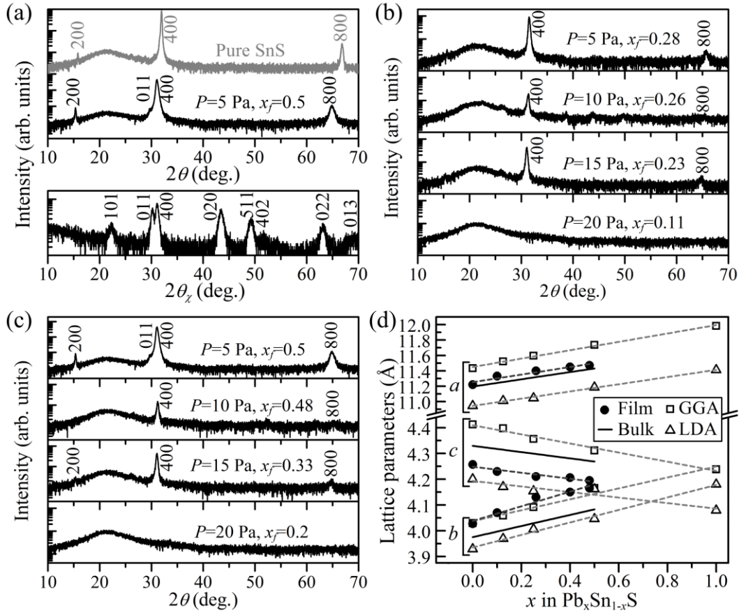
Figure 5.1. Structural properties of (\text{Sn}_{1-x_f}\text{Pb}_{x_f})\text{S} films. (a) Typical out-of-plane (top panel) and in-plane (bottom panel) XRD patterns of (\text{Sn}_{1-x_f}\text{Pb}_{x_f})\text{S} film with x_f=0.5 grown at 300 °C and 5 Pa. (b and c) XRD patterns of the (\text{Sn}_{1-x_f}\text{Pb}_{x_f})\text{S} films grown at 300 °C with various conditions. (d) Lattice parameters ( a, b, c ) of (\text{Sn}_{1-x}\text{Pb}_x)\text{S} as a function of x . The closed circles indicate those obtained with the thin films, the solid lines are those of bulk (\text{Sn}_{1-x}\text{Pb}_x)\text{S} taken from Ref. 3, and the open symbols are the calculation results obtained by DFT in this work. The dashed straight lines are guides for eyes.
