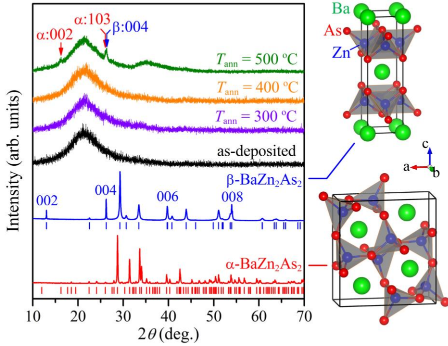
Figure 2.1. XRD patterns of \text{BaZn}_2\text{As}_2 films deposited at room temperature and annealed at various temperature ( T_{\text{ann}} ) along with those of polycrystalline \alpha - and \beta - \text{BaZn}_2\text{As}_2 bulks for comparison. The crystal structures of \alpha - \text{BaZn}_2\text{As}_2 ( \alpha - \text{BaCu}_2\text{S}_2 -type, space group Pnma ) and \beta - \text{BaZn}_2\text{As}_2 ( \text{ThCr}_2\text{Si}_2 -type, space group I4/mmm ) are also shown on the right.
