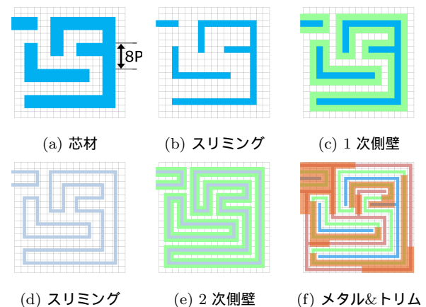
図1 Self-aligned quadruple-patterning (SAQP) Process (half pitch = 1P , grid pitch = 2P )
