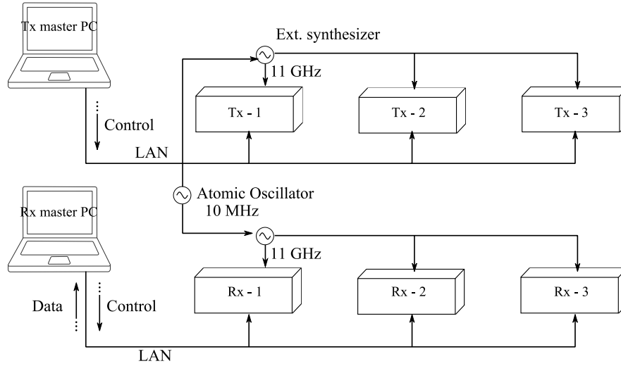
Figure 5.3 High-level diagram of the single-link measurement (external high-precision LO were used both at Tx and Rx).
