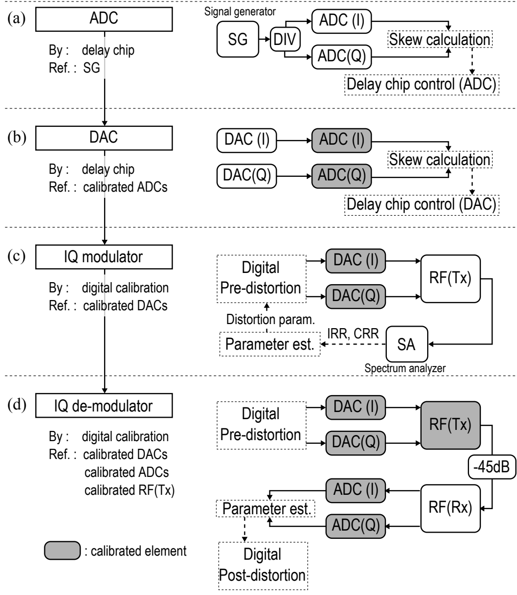
Figure 3.10 Calibration procedure and corresponding block diagrams.
