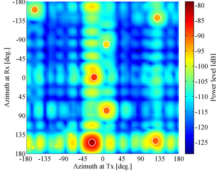
Figure 5.11 Comparison of double-directional angular power spectrum: ray-tracing outputs and reconstructed channel response. (The ray-tracing outputs paths are indicated by the colored dots.)
