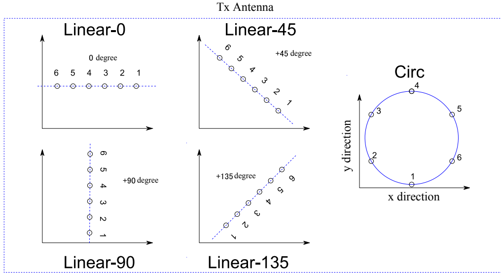
Figure 5.5 Antenna orientation at Tx for multi-link measurement.
