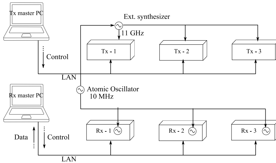
Figure 5.4 High-level diagram of the multi-link measurement. (external high-precision Lo was used at Tx, but at Rx side, internal normal-precision LOs were used to enable spatial separation of Rxs.)
