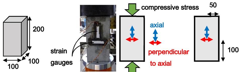
Figure 1: Specimen size, appearance of experiment and attached positions of specimen surface [mm]
