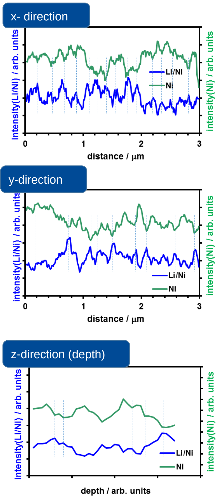
Figure 28 Line analysis of Ni, and Li/Ni in x, y, and z direction indicated in Figure 27.
