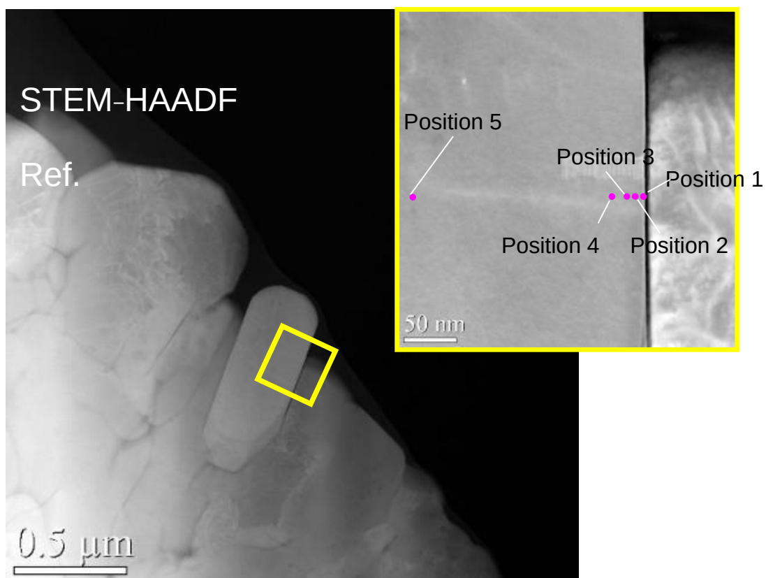
Figure 23 HAADF image for ref. NCM particle.
