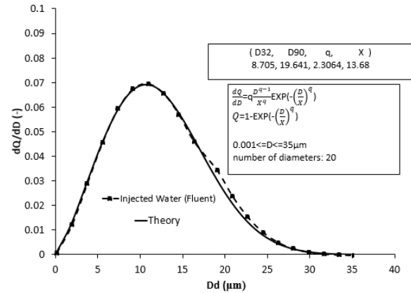
Fig. 5 Comparison of volume fraction distribution with theory.
