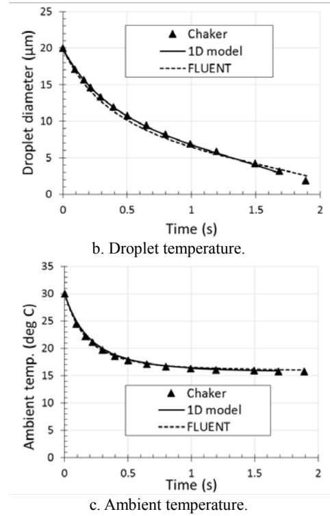
Fig. 4 Chaker [3] versus predicted numerical and 1D model method values of relative humidity (a), droplet diameter (b) and ambient temperature (c).
