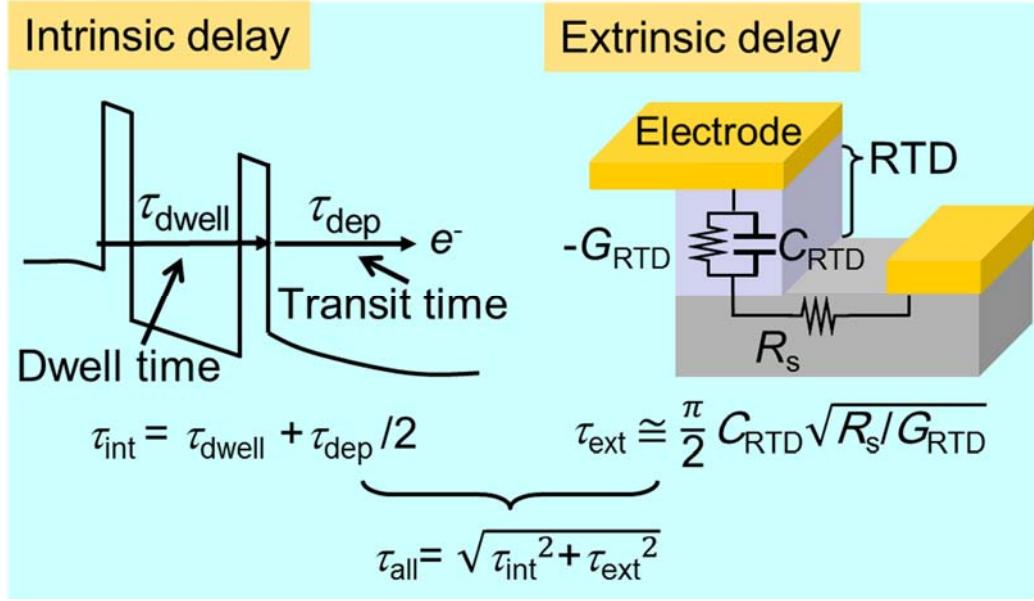
Fig. 2.12 Components of total, intrinsic, and extrinsic delay time.
