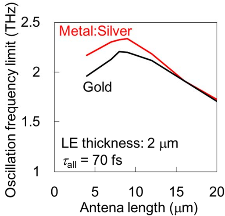
Fig. 5.20 Oscillation frequency limit versus antenna length with 2- \mu\text{m} lower electrode and silver as metal.
