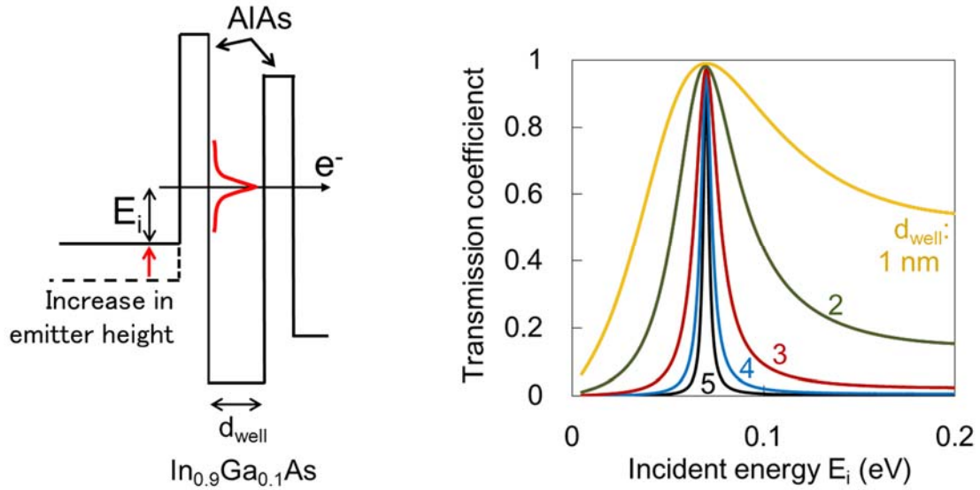
Fig. 3.7 Estimation of tunneling coefficient with reduction in well thickness and increase in emitter height.
