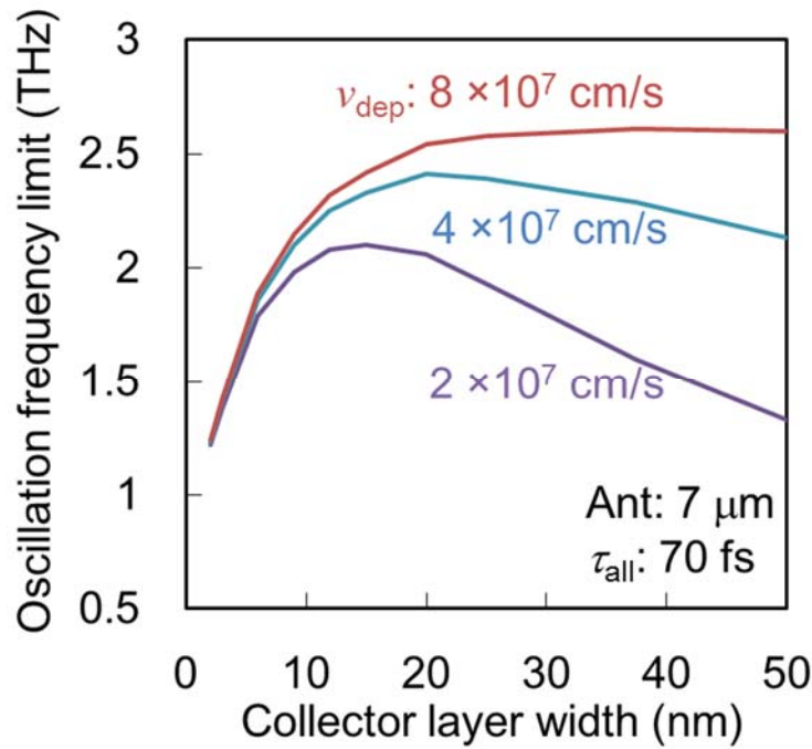
Fig. 4.2 Theoretical calculation of oscillation frequency vs. collector layer width for several electron velocities in collector depletion region.
