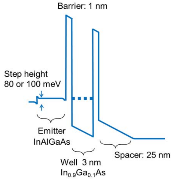
Fig. 3.16 Schematic band diagram of step emitter structure.
