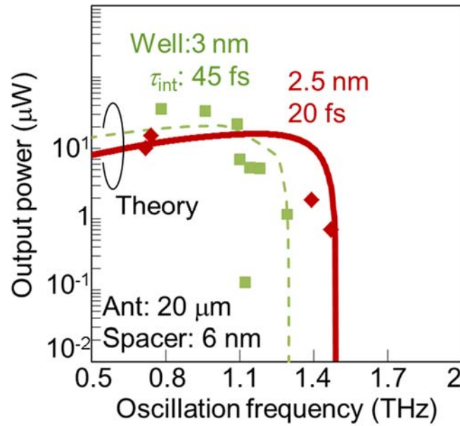
Fig. 3.24 Measured output power as a function of oscillation frequency of RTDs with different well thickness. The antenna length is 20 \mu\text{m} . Theoretical curves and extracted intrinsic delay time are also shown.
