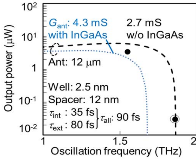
Fig 5.22 Theoretical curves with and without InGaAs under air bridge. Black dots show the experimental results with the air-bridge structure.
