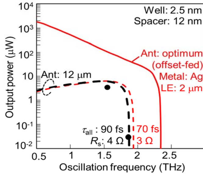
Fig. 5.21 Theoretical output power as function of oscillation frequency for RTDs with resistances of 4 and 3 \Omega at f_{\text{int}} , and 12- \mu\text{m} antenna without InGaAs under air bridge shown by dotted black and red curves. The red solid curve shows the estimation for the optimum antenna offset-fed for each oscillation frequency, with silver and a lower electrode thickness of 2 \mu\text{m} .
