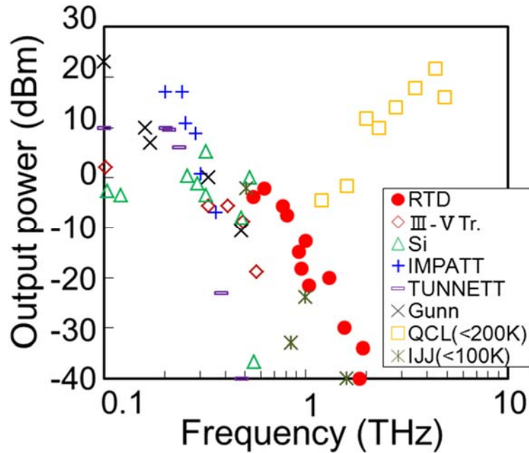
Fig 1.11 Output power as a function of frequency of solid-state terahertz sources in 2015
