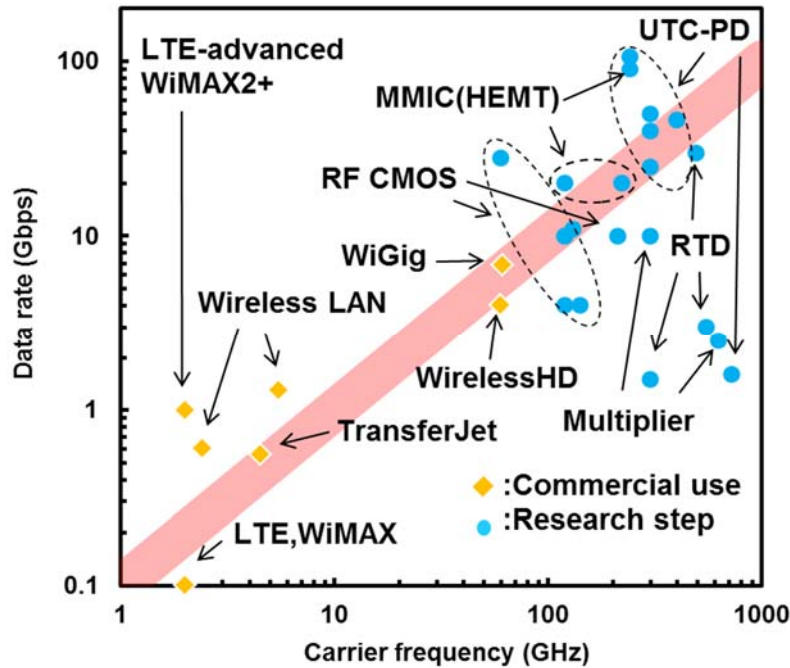
Fig 1.3 Recent progress of wireless communication data rate as a function of carrier frequency in THz range.
