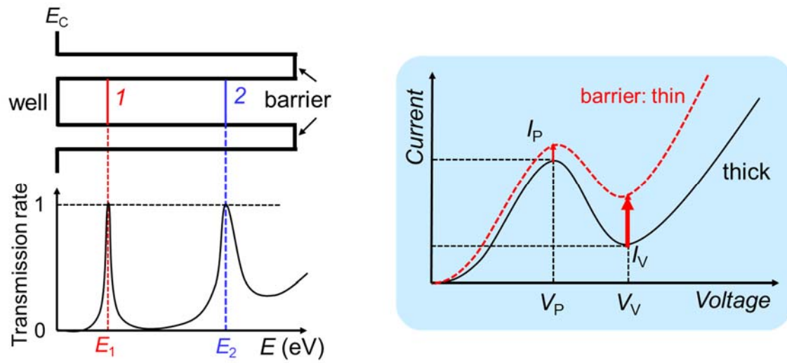
Fig. 3.9 Schematic diagram of increase in valley current because of increase in transmission rate of 2 nd level resonance from Ref. 3.6.
