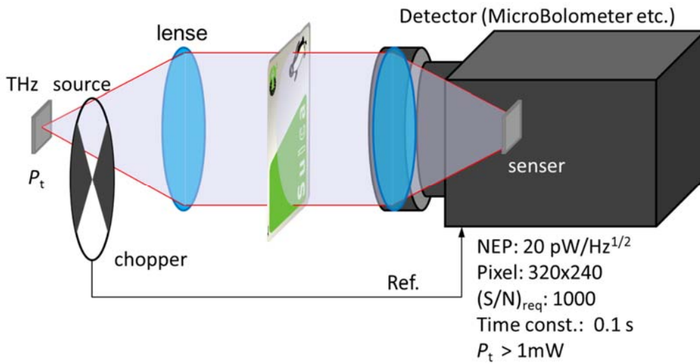
Fig. 1.6 Schematic of imaging system transmission.
