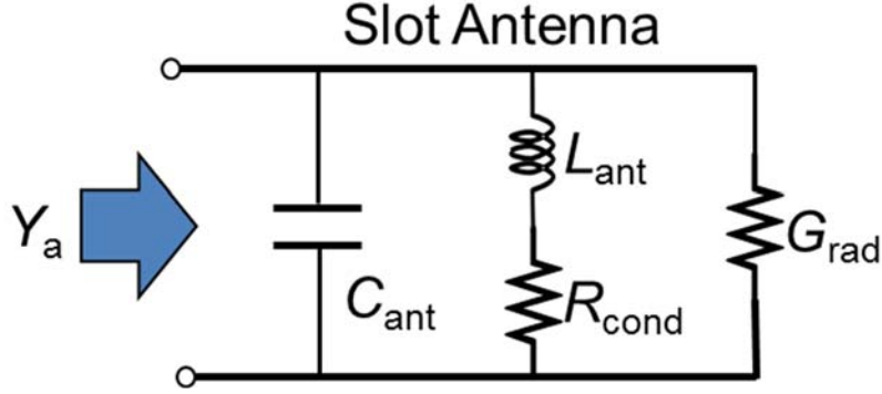
Fig. 2.11 Equivalent circuit of slot antenna.
