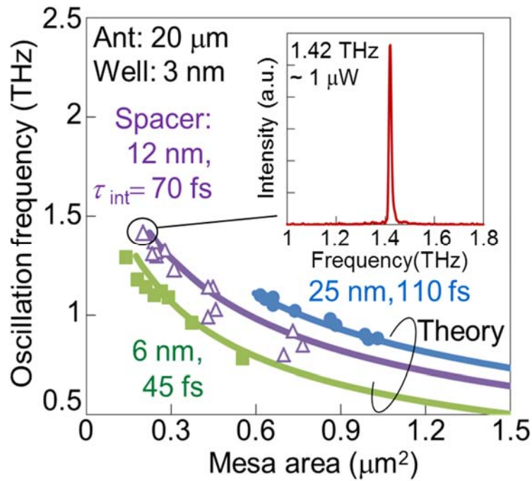
Fig. 4.5 Dependence of oscillation frequency on RTD mesa area for different spacer thicknesses. The inset is the measured spectrum of fundamental oscillation at 1.42 THz of the RTD with 12-nm thick spacer.
