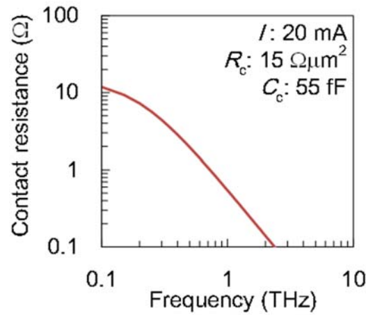
Fig. 2.15 Decrease in contact resistance caused by contact capacitance of RTD.
