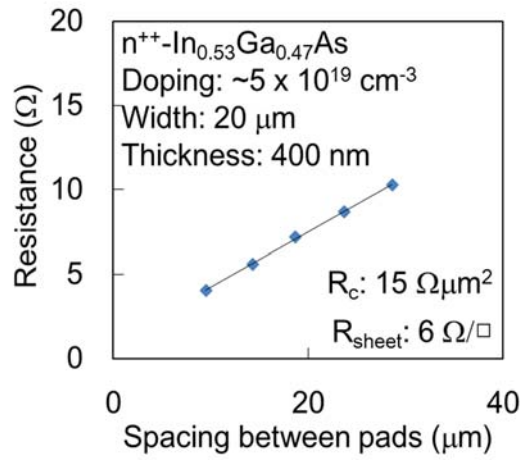
Fig. 2.14 Typical experimental result of contact resistance measured with transmission line method.
