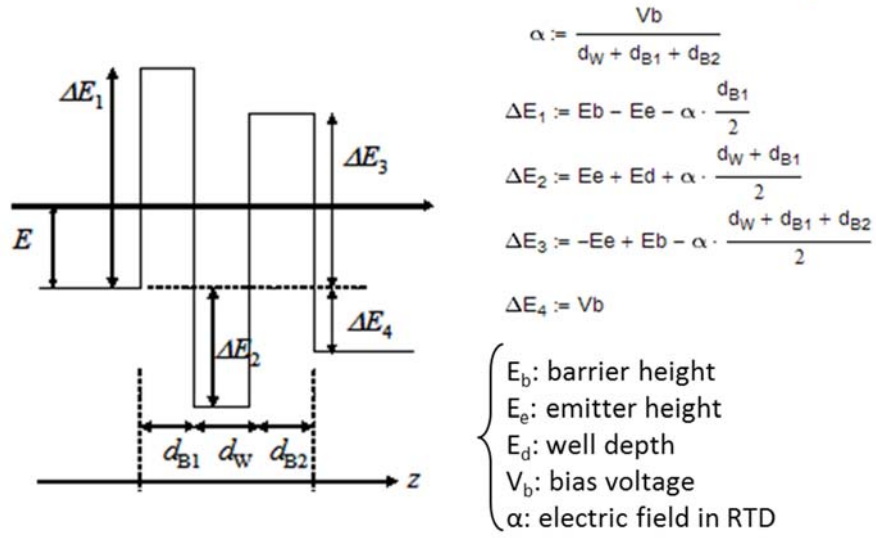
Fig. 3.2 Calculation model of band diagram for tunneling transmission coefficient and the parameters of the rectangular potential of RTD.
