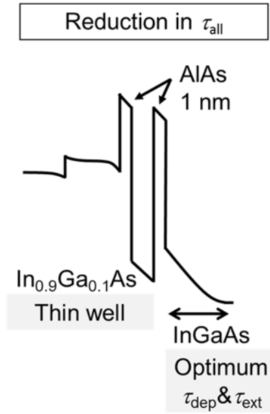
Fig. 5.1 Reduction in total delay with thin well and optimum spacer.
