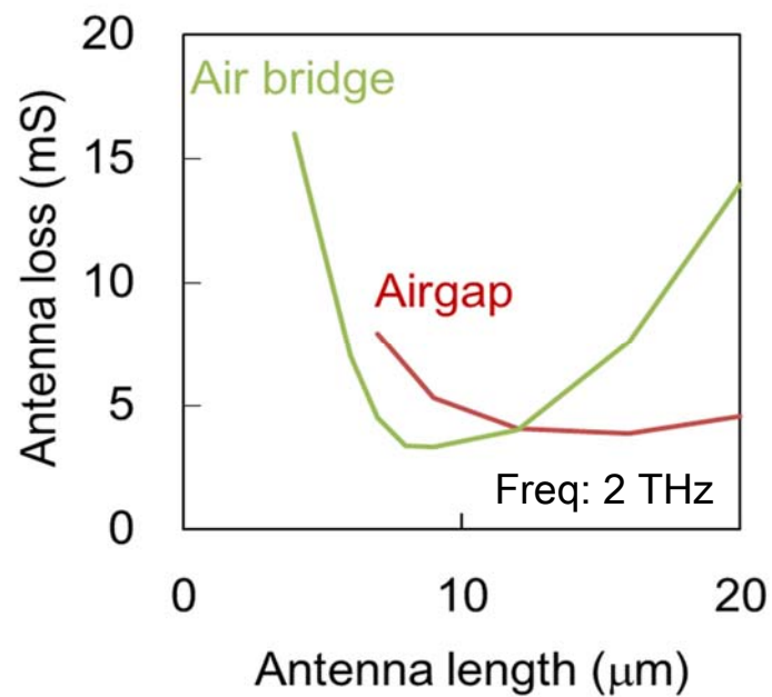
Fig. 5.15 Antenna loss versus antenna length for air-gap and air-bridge structures.
