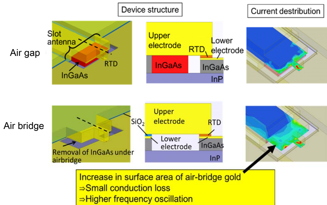
Fig. 5.14 Reduction in antenna loss with reduction in InGaAs under air bridge.
