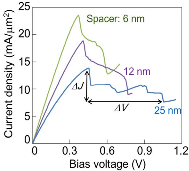
Fig. 4.4 Measured current-voltage characteristics of RTDs with different spacer thicknesses.
