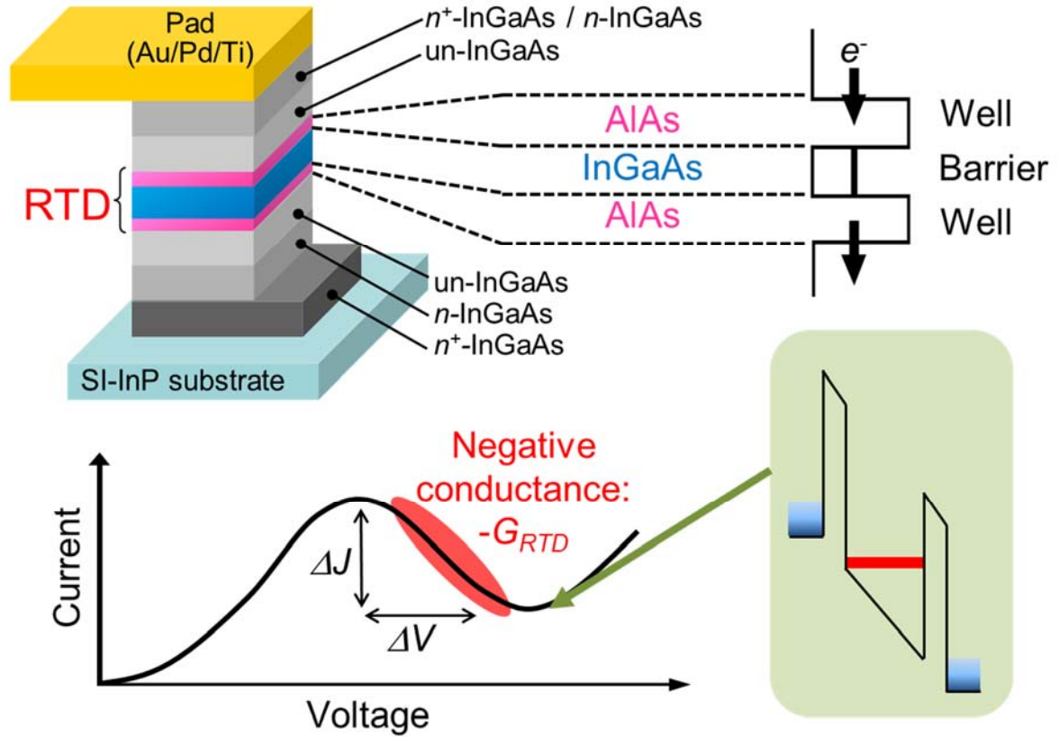
Fig. 2.7 Schematic diagram of I - V curve, energy band, and negative differential conductance region.
