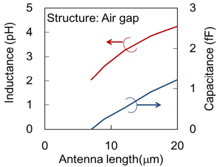
Fig. 5.9 Antenna inductance and capacitance vs. antenna length.
