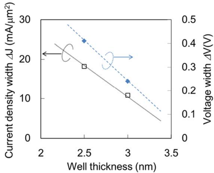
Fig. 3.22 Measured current density and voltage widths as a function of well thicknesses of RTD.
