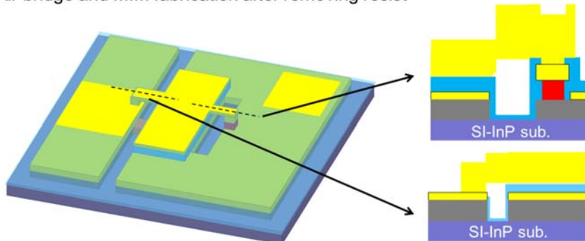
Fig. 2.5 Fabrication process 4.
