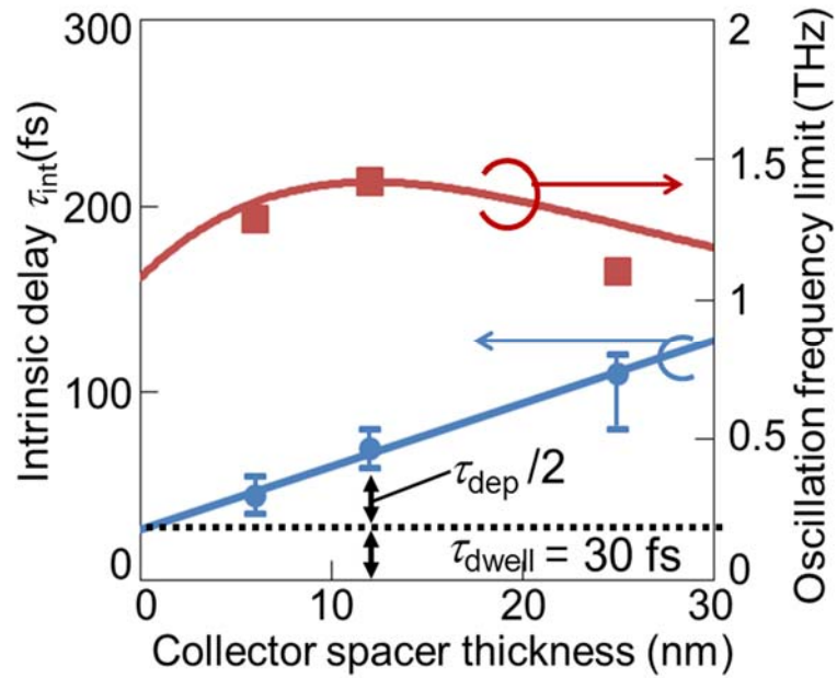
Fig. 4.6 Intrinsic delay time and the highest limit to oscillation frequency extracted by fitting between measurement and theory in Fig. 4.4 as a function of collector spacer thickness.
