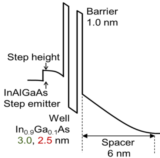
Fig. 3.19 Schematic band diagram of RTDs with different quantum-well thickness.
