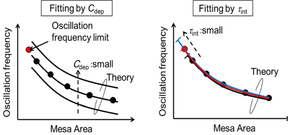
Fig. 2.13 Schematic diagram of procedure for fitting of C_{\text{dep}} and \tau_{\text{int}} .
