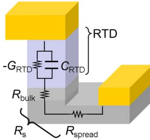
Fig. 5.3 Schematic structure of series resistance.
