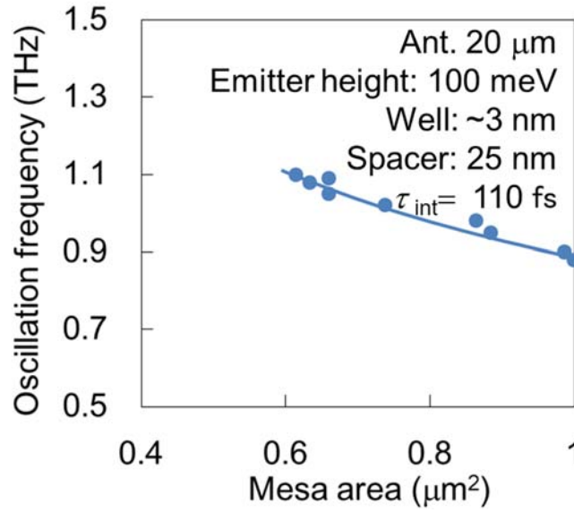
Fig. 3.18 Oscillation frequency versus mesa area for the RTD with 100-meV step emitter.
