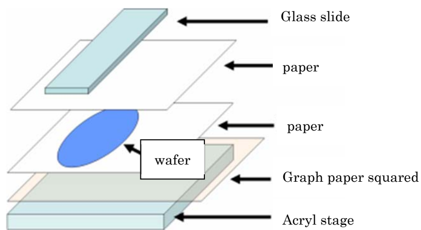
Fig. A.1 Cutting wafer
