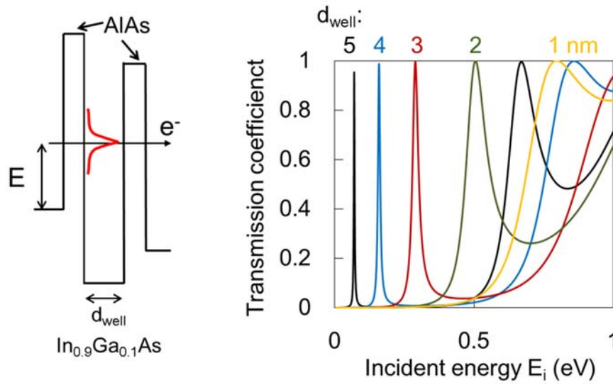
Fig. 3.4 Estimation of tunneling coefficient with rectangular potential of RTD.
