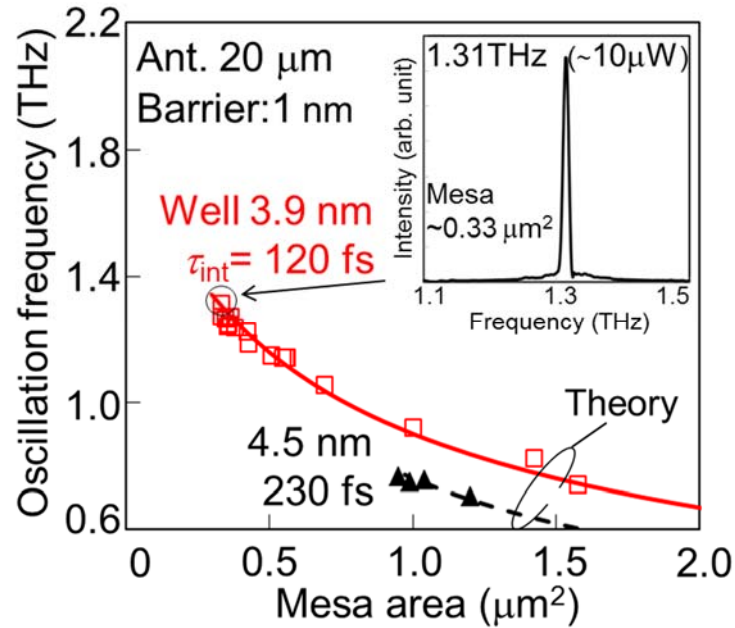
Fig. 3.12 Dependence of oscillation frequency on RTD mesa area of 4.5- and 3.9-nm-thick wells and measured spectrum of fundamental oscillation of 1.31 THz. The intrinsic delay of the RTD with 4.5nm-thick well is recalculated with resent discussion of increase in series resistance with frequency mentioned in chapter 2.
