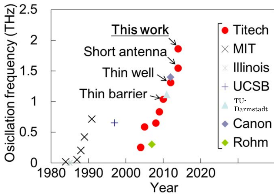
Fig 1.12 The history of increase in oscillation frequency for RTD oscillators
