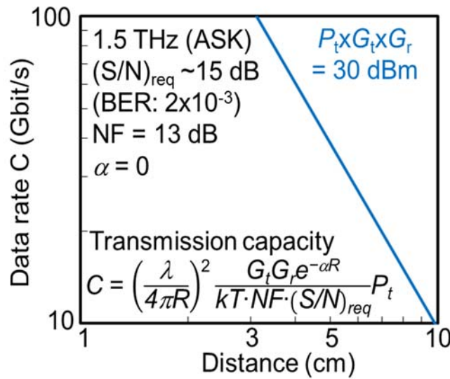
Fig. 1.4 Examples of transmission capacity as a function of distance.
