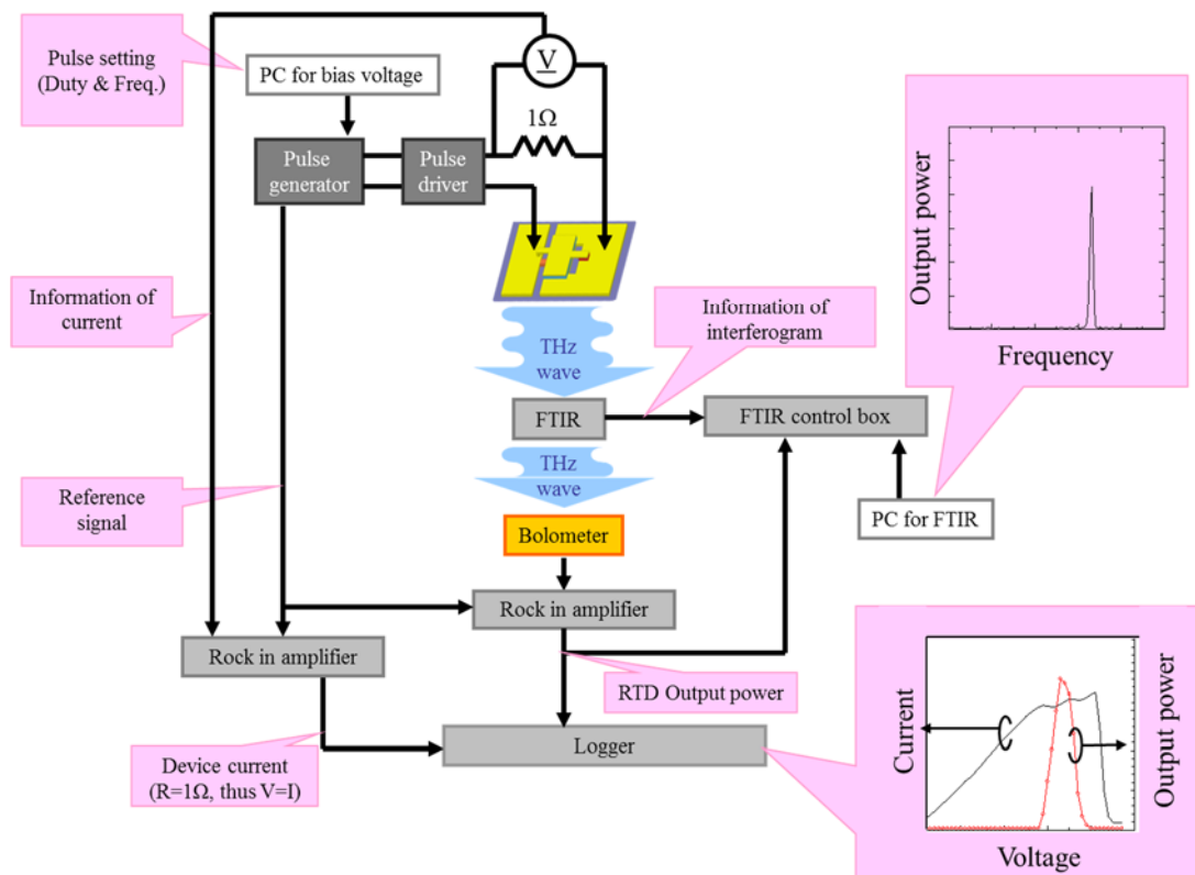
Fig A.4 Precise measurement system of oscillation frequency.
