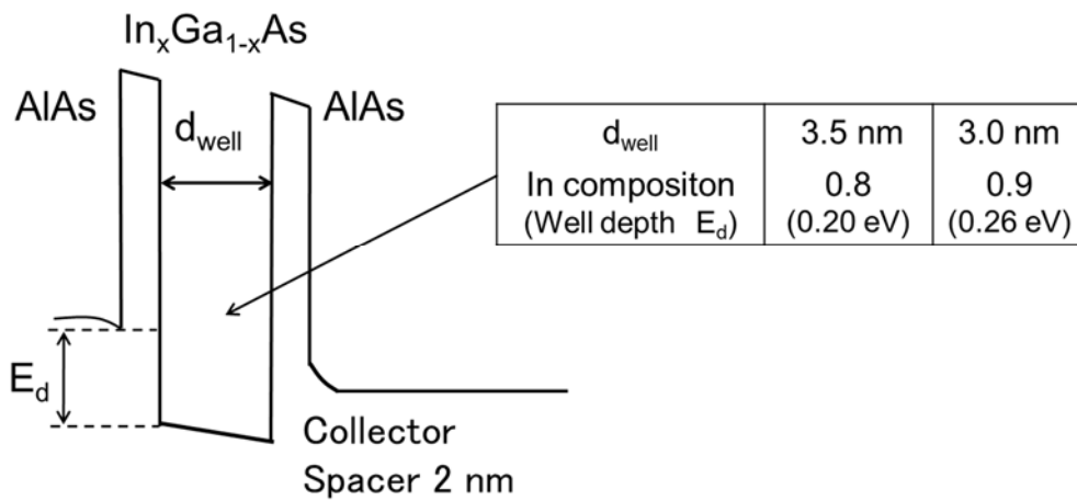
Fig. 3.13 Schematic band diagram of with and without thin and deep well.
