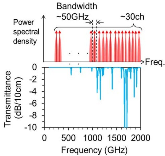
Fig. 1.5 Examples of frequency division duplex under 2 THz.
