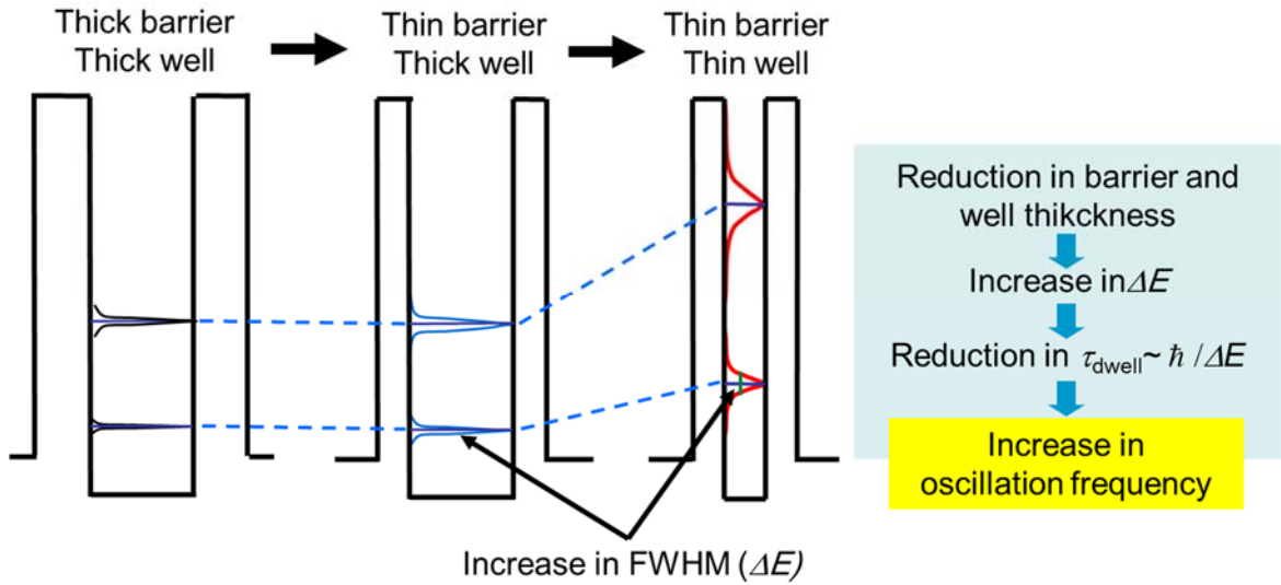
Fig. 3.1 Reduction in dwell time with increase in FWHM associated by thin barrier and well.
