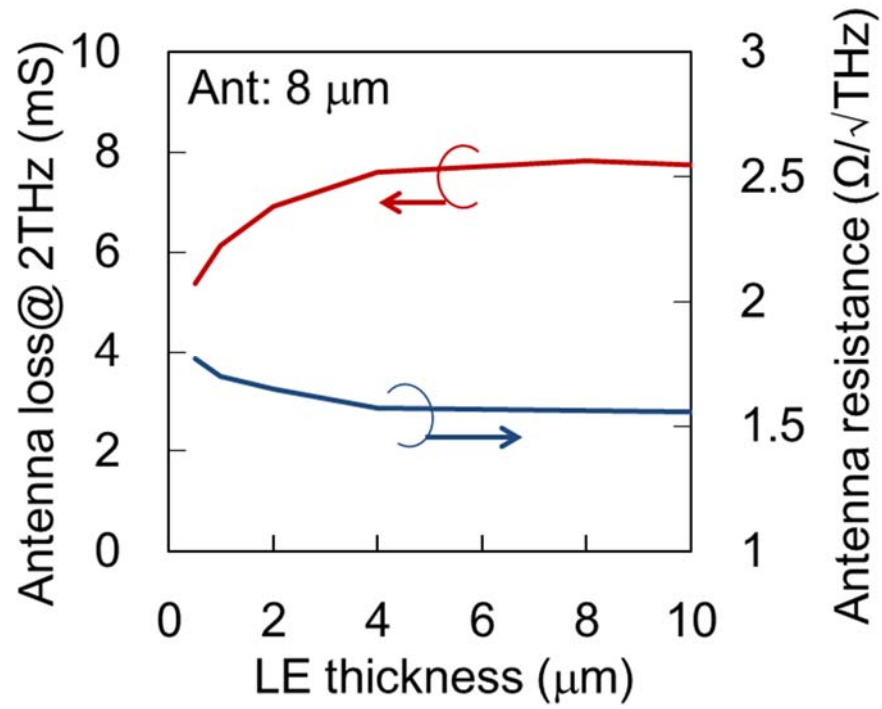
Fig. 5.18 Antenna loss and resistance versus lower electrode thickness.
