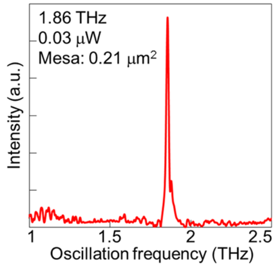
Fig 5.23 Measured spectrum of fundamental oscillation at 1.86 THz.
