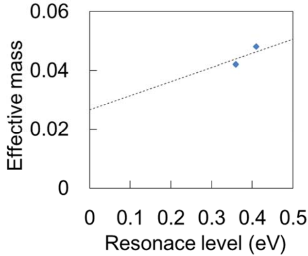
Fig. 3.3 Increase in effective mass with resonance level from bottom of the well.
