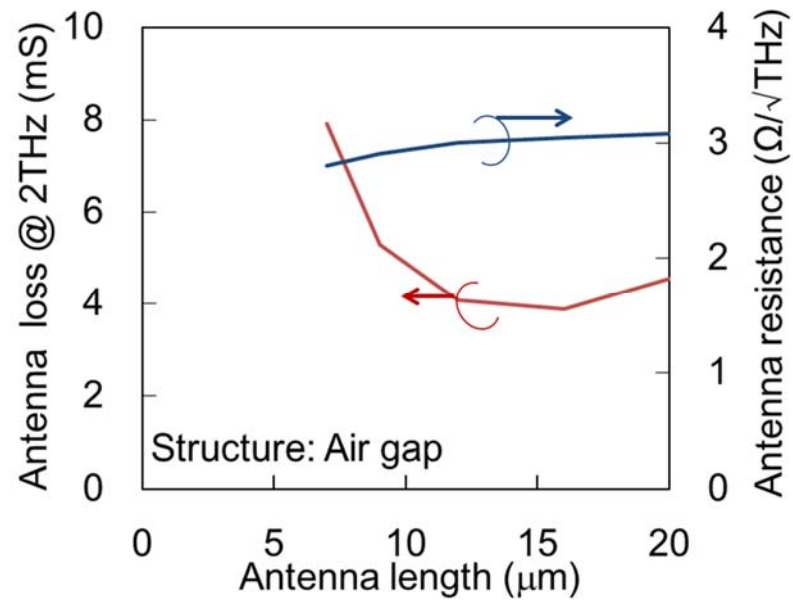
Fig. 5.10 Antenna admittance at frequency of 2 THz vs. antenna length.
