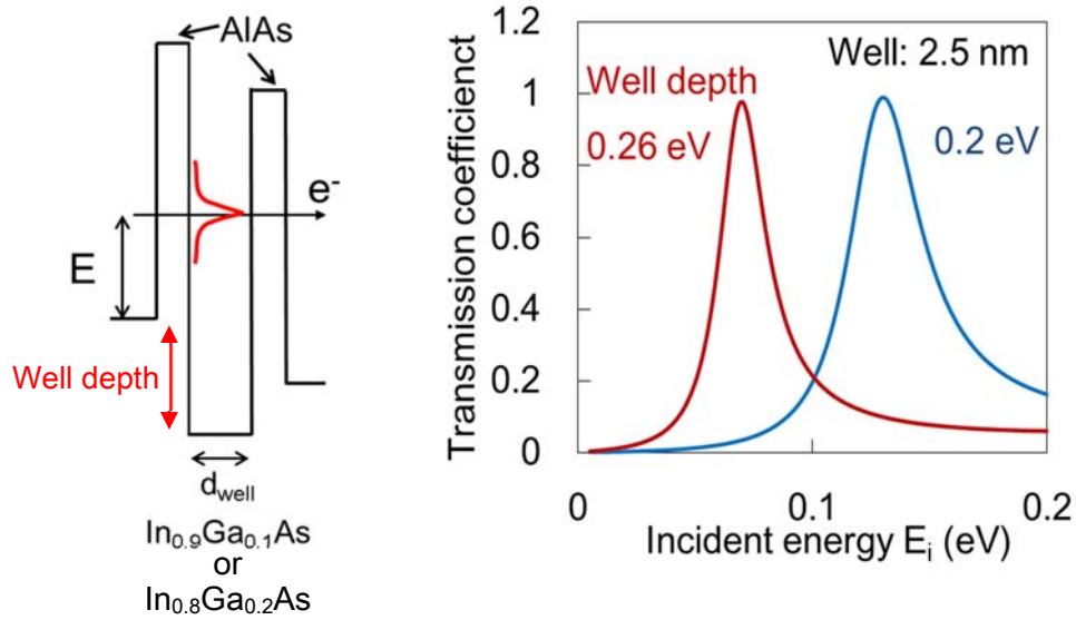
Fig. 3.5 Tunneling coefficient rates with two different well depth.
