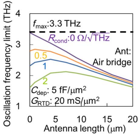
Fig. 5.13 Oscillation frequency limit versus antenna length with reduction in antenna resistance calculated with usual air bridge structure.
