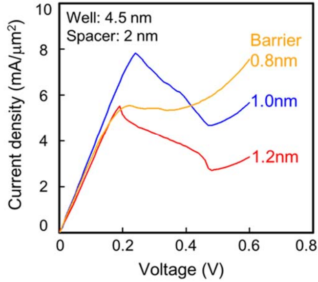
Fig. 3.8 I - V characteristics for the RTDs with different barrier thickness from Ref. 3.6.
