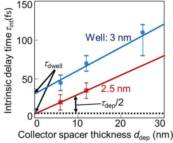
Fig. 5.2 Intrinsic delay time as function of collector spacer thickness for different well and spacer thicknesses in this research.
