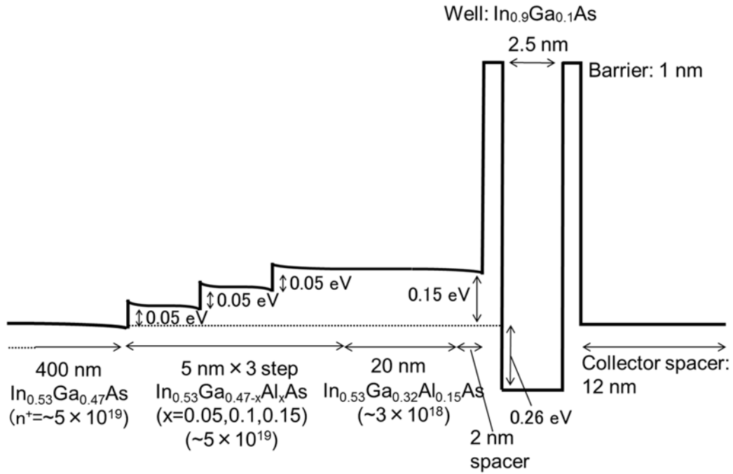
Fig. 3.20 Band diagram of RTD with the well thickness of 2.5-nm well and 3-step emitter structure.
