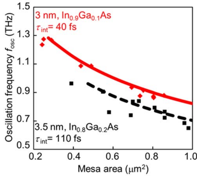
Fig. 3.15 Dependence of oscillation frequency on RTD mesa area of 3-nm-thick \text{In}_{0.9}\text{Ga}_{0.1}\text{As} and 3.5-nm-thick \text{In}_{0.8}\text{Ga}_{0.2}\text{As} .
