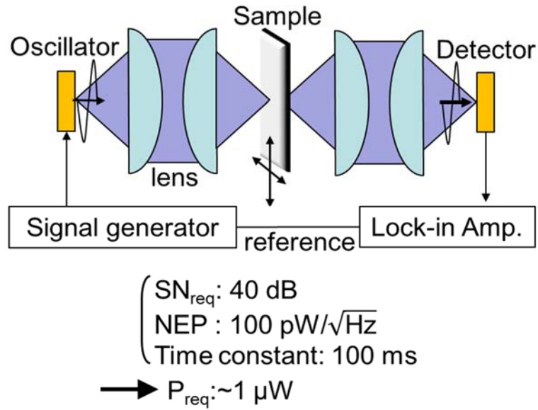
Fig 1. 8 Schematic measurement system of transmission spectroscopy.
