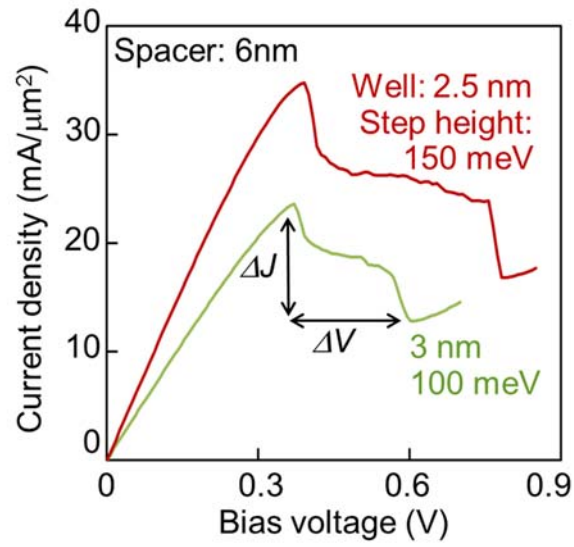
Fig. 3.21 Measured current density-voltage characteristics of RTDs with different quantum-well thicknesses.
