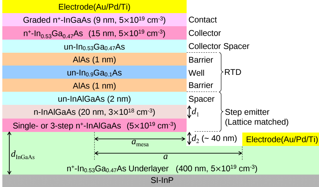
Fig. 2.6 Typical layer structure of RTD in this thesis. An InAlGaAs step emitter, details of which are described in Chapter 3, and an indium-rich deep quantum well were employed to reduce the bias voltage for NDC.
