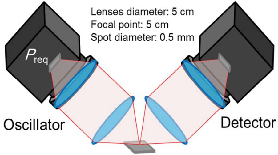
Fig 1.9 Schematic diagram of reflection sensing.
