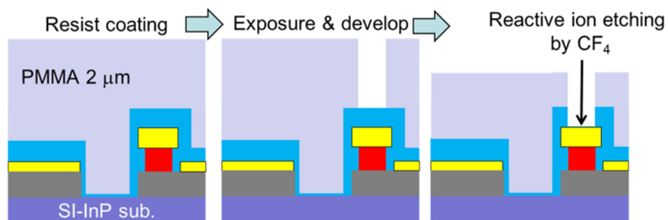
Fig. 2.4 Fabrication process 3.
