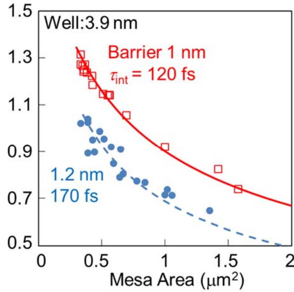
Fig. 3.10 Oscillation frequency vs mesa area with two different barrier thicknesses.
