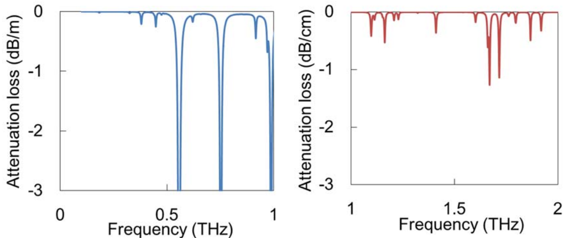
Fig 1.2 Atmospheric attenuation of terahertz region. The data was calculated by Amaterasu offered by NICT
