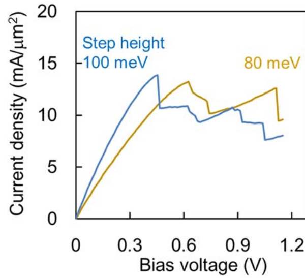
Fig. 3.17 Experimental results of I - V characteristics for two step emitter height.
