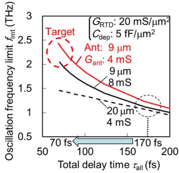
Fig. 2.16 Reduction in total delay time and reduction in antenna length and loss for higher oscillation frequency limit.
