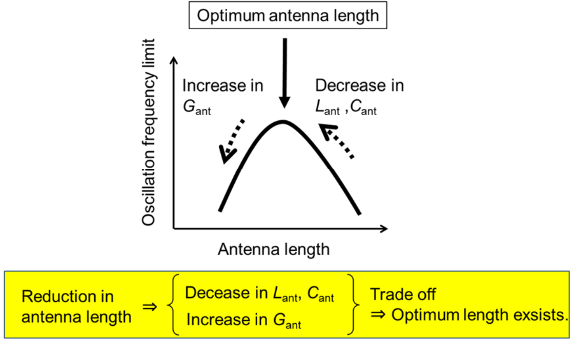
Fig. 5.8 Antenna length optimization.
