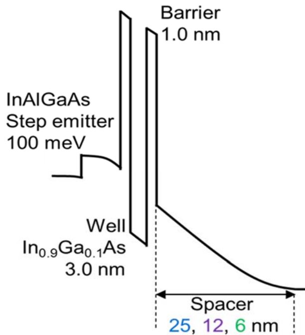
Fig. 4.3 Band diagram of the fabricated RTDs with spacer thickness of 25, 12, 6 n.m
