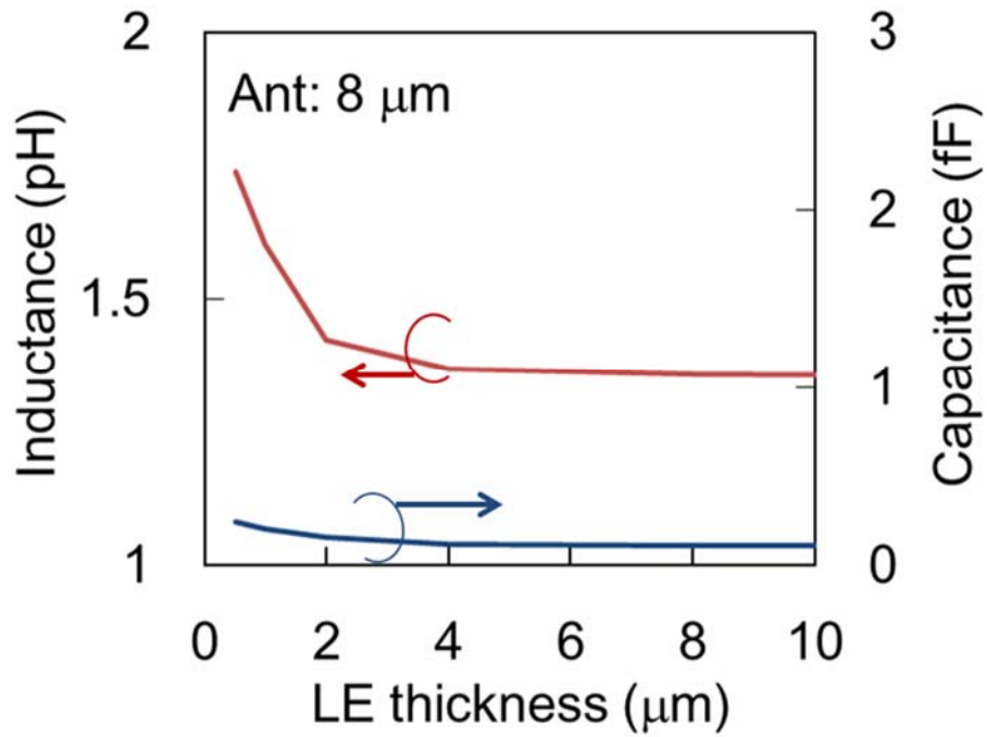
Fig. 5.19 Antenna inductance and capacitance versus lower electrode thickness.
