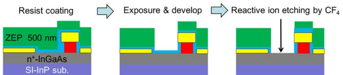
Fig. 2.3 Fabrication process 2.
