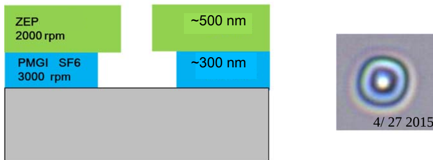
Fig. A.2 Schematic structure and picture near RTD mesa of resist after bottom resist development
