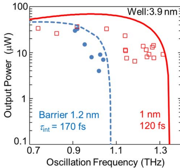
Fig. 3.11 Output power vs oscillation frequency of two RTDs with 1.2- and 1-nm barrier with 20- \mu\text{m} antenna.
