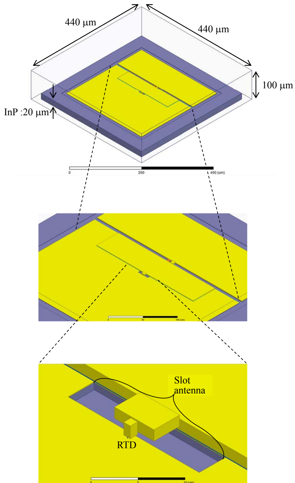
Fig. 2.10 Calculated antenna model of HFSS.
