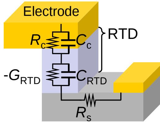
Fig. 2.8 Schematic structure of RTD mesa with equivalent circuit.
