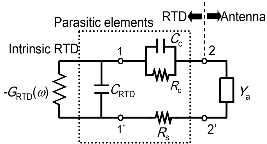
Fig. 2.9 Equivalent circuit of RTD oscillator with parasitic elements.
