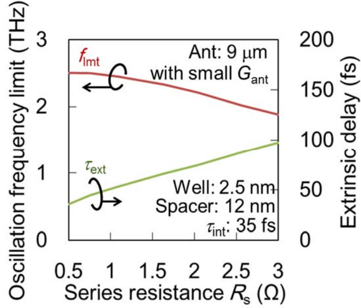
Fig. 5.4 Increase in oscillation frequency with reduction in extrinsic delay \tau_{ext} and series resistance R_s at oscillation frequency limit.
