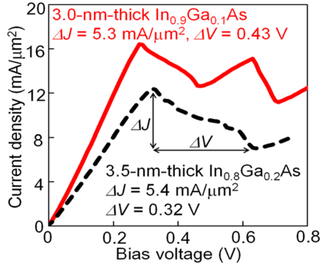
Fig. 3.14 I - V characteristics for the RTDs with and without deep quantum well.
