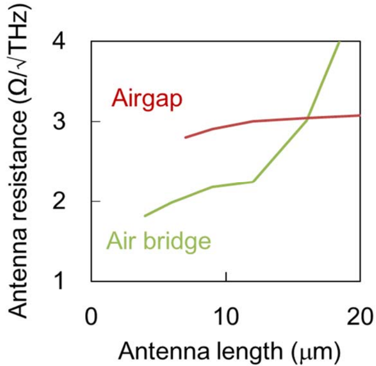
Fig. 5.16 Antenna resistance versus antenna length for air-gap and air-bridge structures.
