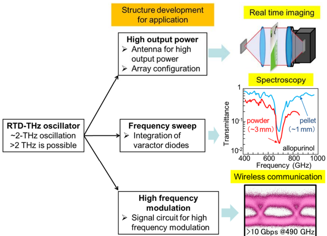
Fig. 6.1 Future prospects of RTD-THz oscillators.
