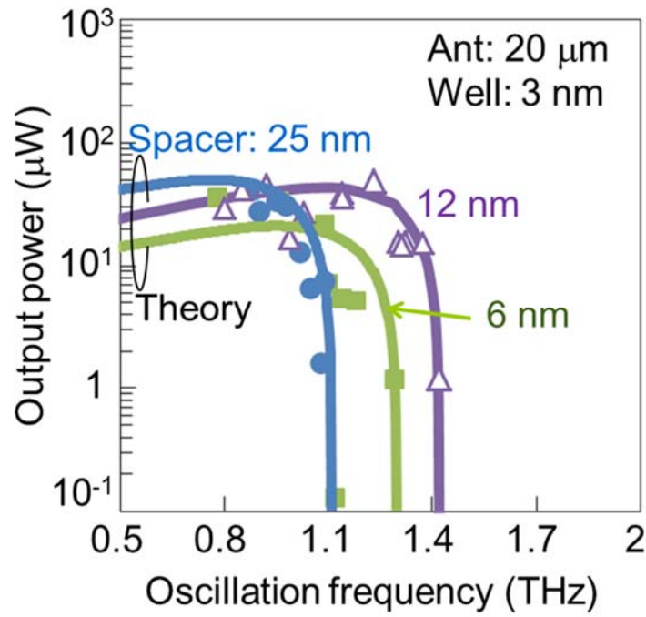
Fig. 4.7 Experimental and theoretical output power as a function of oscillation frequency for different spacer thicknesses.
