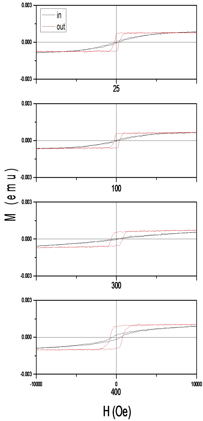
Fig 2-19 Hysteresis loops of as-deposited, 100°C-annealed, 300°C-annealed and 400°C-annealed \text{CoO}_{20\text{nm}}/[\text{CoPt}_{5\text{nm}}/\text{CoO}_{5\text{nm}}]_5 films (measured at RT).
