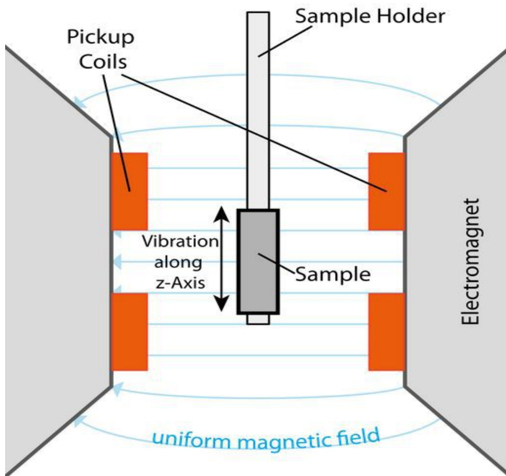
Fig 2-18 The schematic diagram of VSM.
