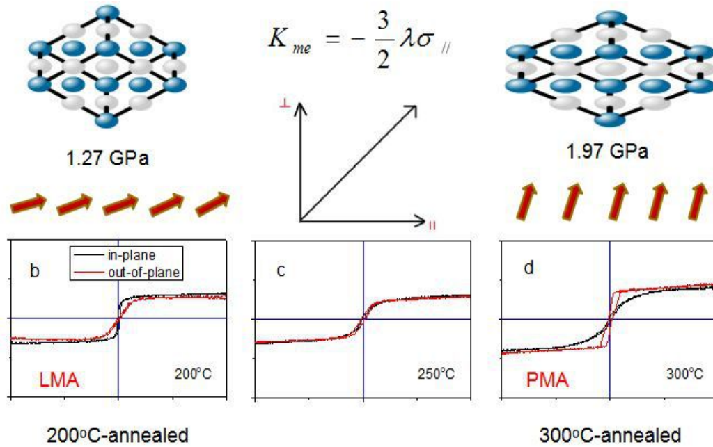
Fig 4-11 Magnetoelastically induced magnetic anisotropy transition in [\text{CoO}5\text{nm}/\text{CoPt}7\text{nm}]_5 .
