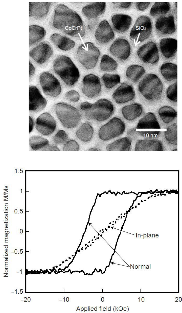
Fig 1-3 In-plane TEM image and hysteresis loop of CoCrPt-SiO 2 medium [9] .
