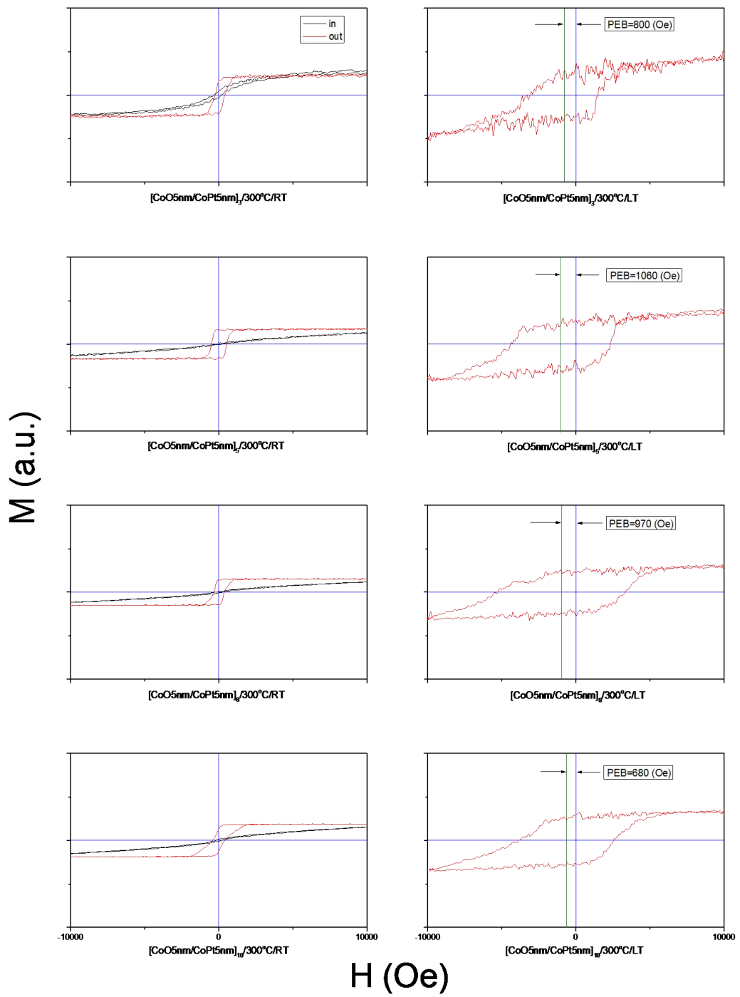
Fig 5-5 PMA (left: measured at RT) and corresponding PEB (right: measured at LT 80K) of 300^\circ\text{C} -annealed [\text{CoO5nm}/\text{CoPt5nm}]_3 , 300^\circ\text{C} -annealed [\text{CoO5nm}/\text{CoPt5nm}]_5 , 300^\circ\text{C} -annealed [\text{CoO5nm}/\text{CoPt5nm}]_8 and 300^\circ\text{C} -annealed [\text{CoO5nm}/\text{CoPt5nm}]_{10} samples.
