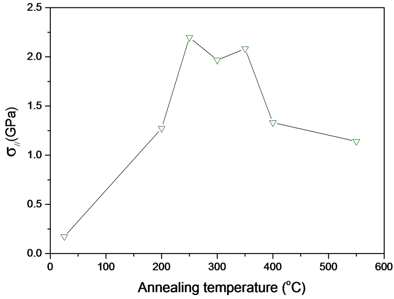
Fig 4-8 CoPt in-plane tensile stress \sigma_{//} of [CoO5nm/CoPt7nm] 5 samples.
