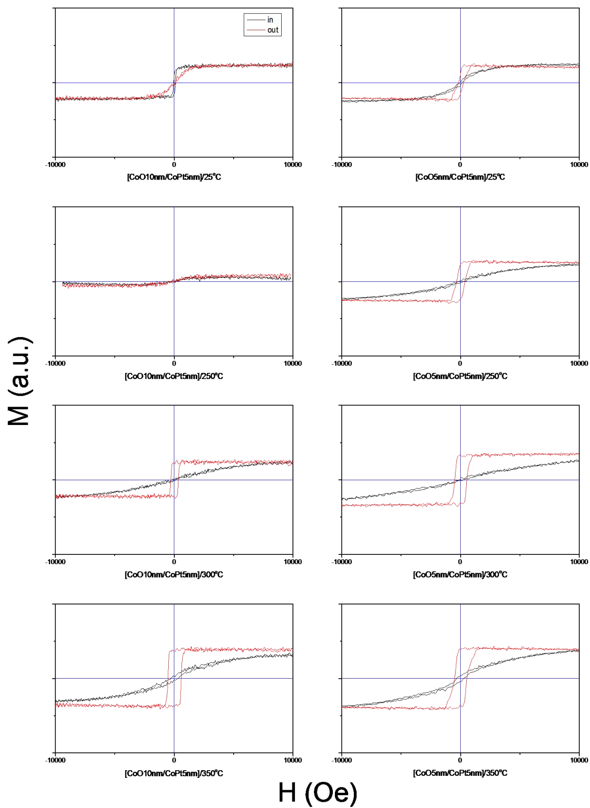
Fig 3-7 Left: hysteresis loops of [\text{CoO}_{10\text{nm}}/\text{CuPt}_{5\text{nm}}]_3 samples (measured at RT).
