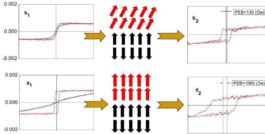
Fig 6-11 Schematic diagrams of Co magnetic moments arrangement at CoO/CoPt interface in [\text{CoO}5\text{nm}/\text{CoPt}5\text{nm}]_5 ( b : is 100°C-annealed sample, d : is 300°C-annealed sample).
