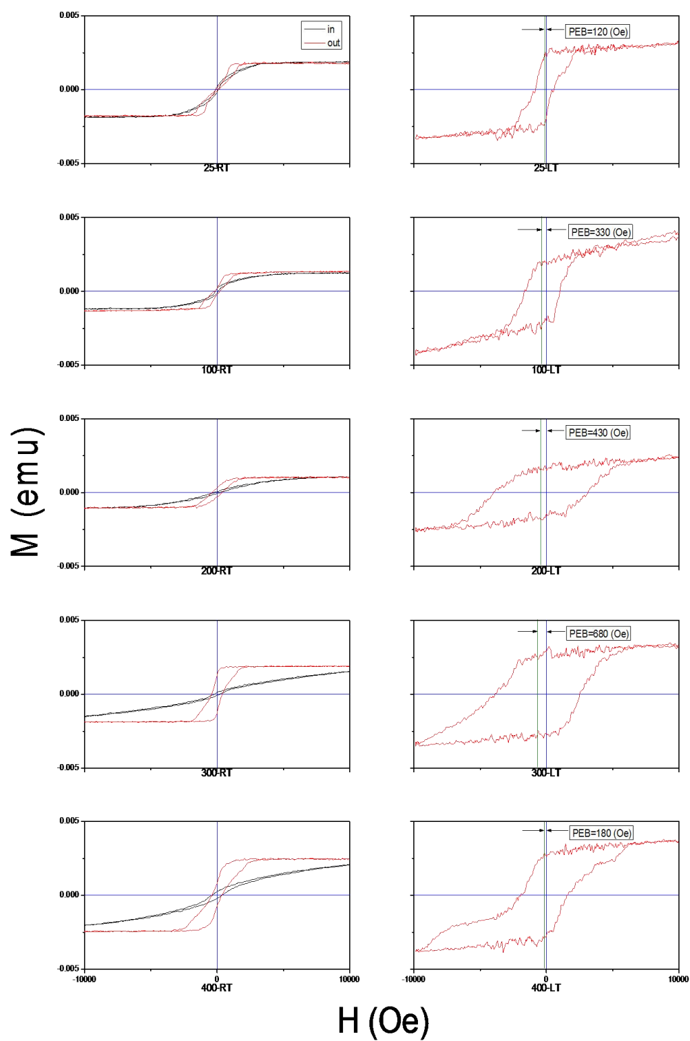
Fig 5-2 PMA (left: measured at RT) and corresponding PEB (right: measured at LT 80K) of as-deposited, 100°C-annealed, 200°C-annealed, 300°C-annealed and 400°C-annealed [CoO5nm/CoPt5nm] 10 samples.
