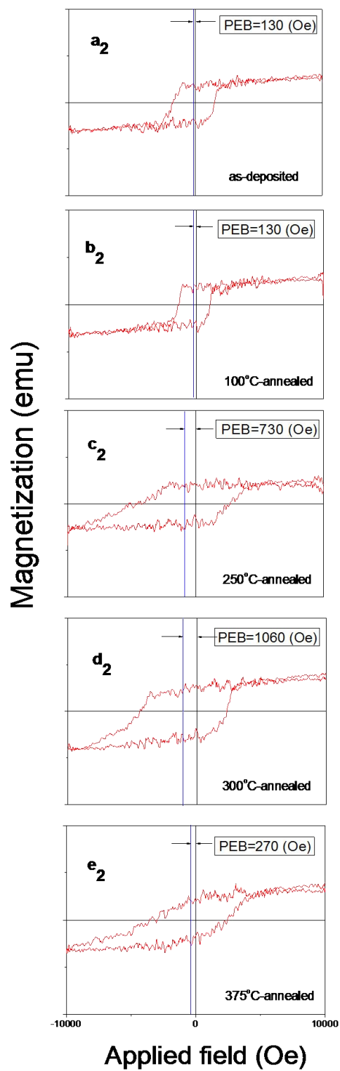
Fig 6-3 PEB out-of-plane M-H hysteresis loops of [\text{CoO5nm}/\text{CoPt5nm}]_5 samples (measured at 80K after perpendicular field cooling).
