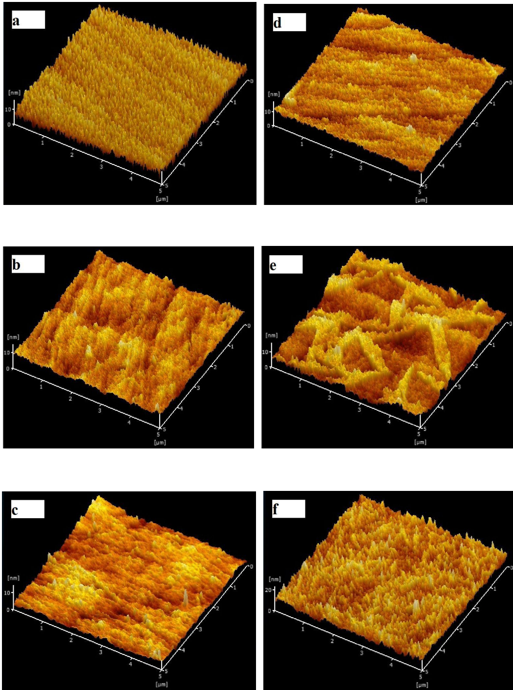
Fig 2-13 Three-dimensional AFM images of [\text{CoO}5\text{nm}/\text{CoPt}2.5\text{nm}]_5 film (a: as-deposited, b: 250°C-annealed, c: 300°C-annealed, d: 350°C-annealed, e: 400°C-annealed, f: 500°C-annealed).
