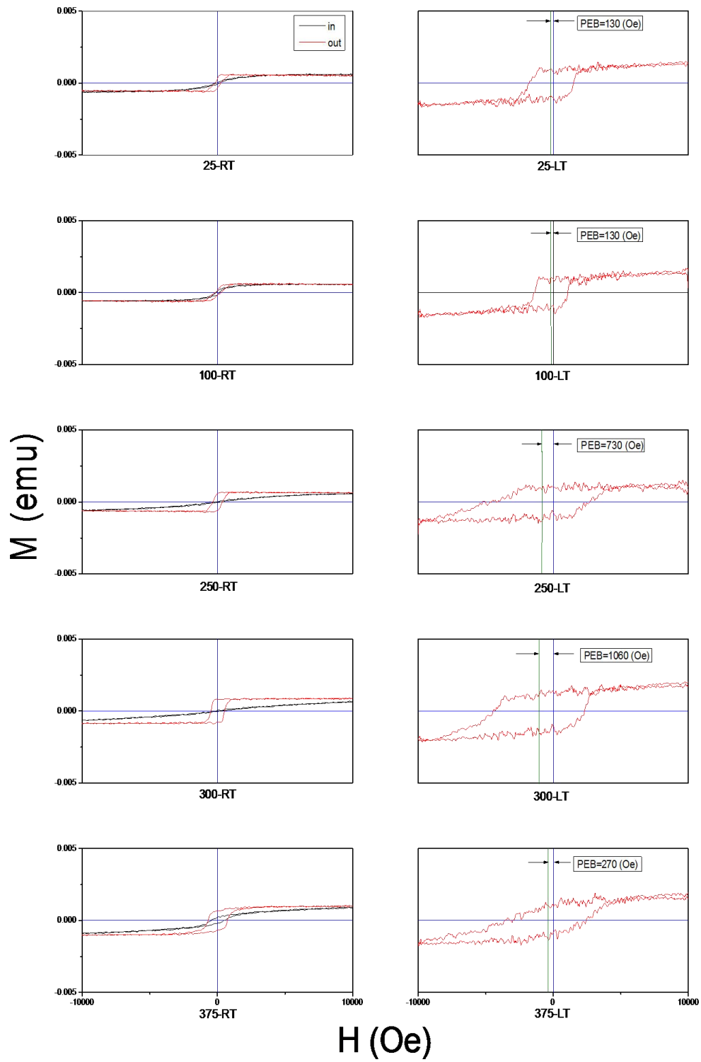
Fig 5-1 PMA (left: measured at RT) and corresponding PEB (right: measured at LT 80K) of as-deposited, 100°C-annealed, 250°C-annealed, 300°C-annealed and 375°C-annealed [\text{CoO5nm}/\text{CoPt5nm}]_5 samples.
