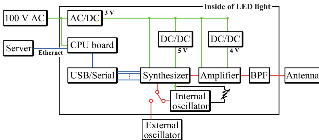
Figure II.1 Detailed structure of wireless energy transmitter.
