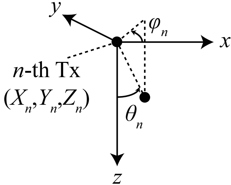
Figure 5.2 Relationship between Cartesian and Spherical coordinate systems.
