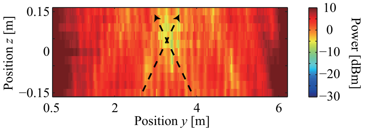
Figure 3.25 Experimental result of power distribution of multi-point wireless energy transmission with carrier shift diversity in vertical plane.
