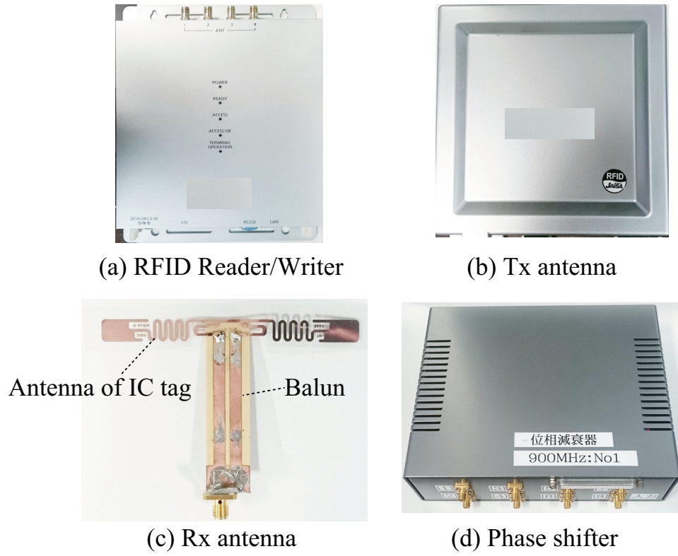
Figure 3.10 Experimental equipments.
