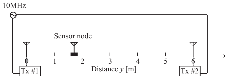
Figure 4.14 Experimental environment.
