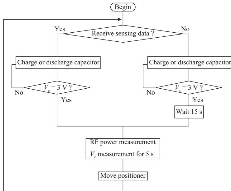
Figure 5.12 Experimental flow.
