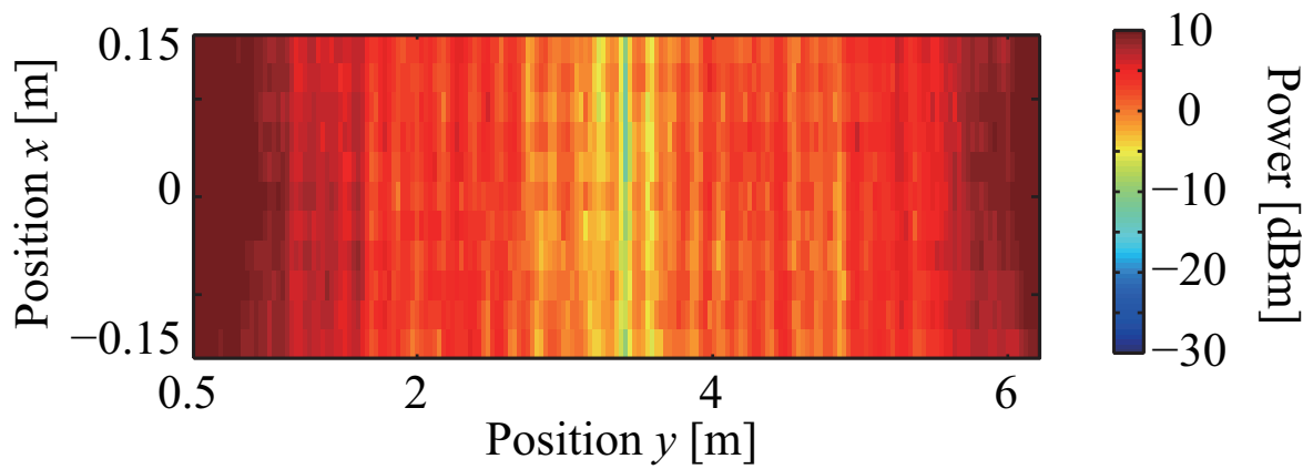
Figure 3.21 Experimental result of power distribution of multi-point wireless energy transmission with carrier shift diversity in horizontal plane.
