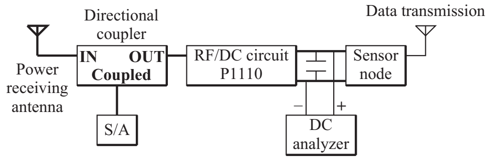
Figure 4.19 Receiver network.
