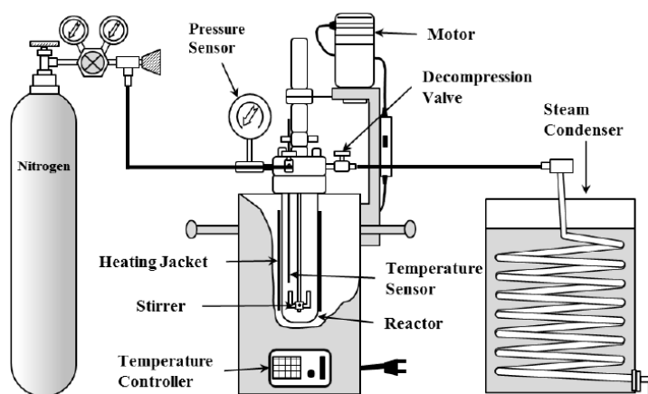
Figure 3-1. Lab scale hydrothermal apparatus (adapted from [7])
