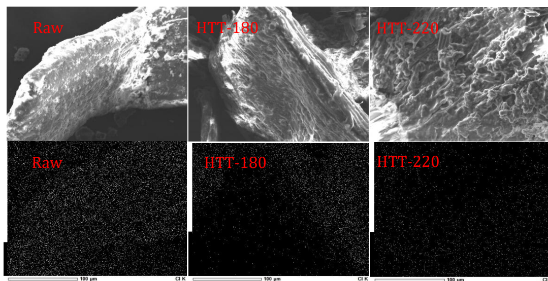
Figure 2-3. Mapping of the chlorine content on the hydrochar surface by SEM-EDX
