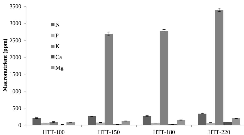
Figure 2-12. Macronutrient in liquid product
