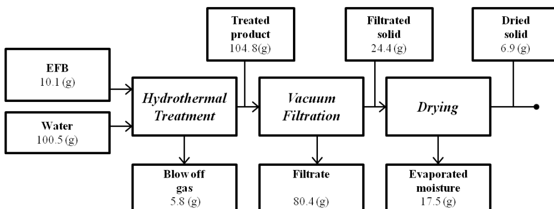
Figure 2-4. Mass balance for HTT of EFB at the temperature of 180°C
