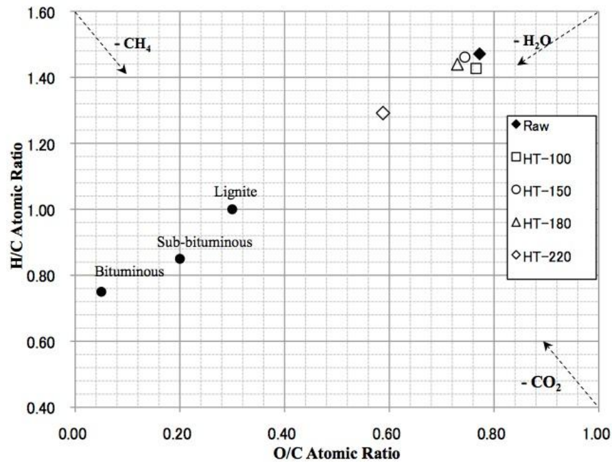
Figure 2-6. Van Kravlen diagram of raw EFB and its resulting hydrochar at various HTT temperatures
