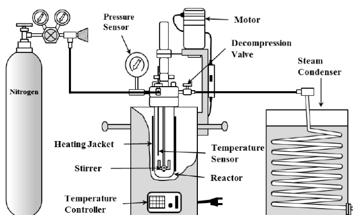
Figure 2-1. Lab scale hydrothermal apparatus (adapted from [6])
