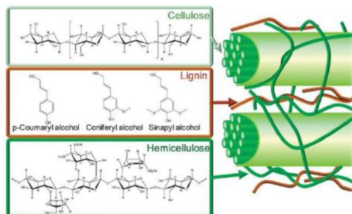
Figure 1-1. Lignocellulosic biomass
