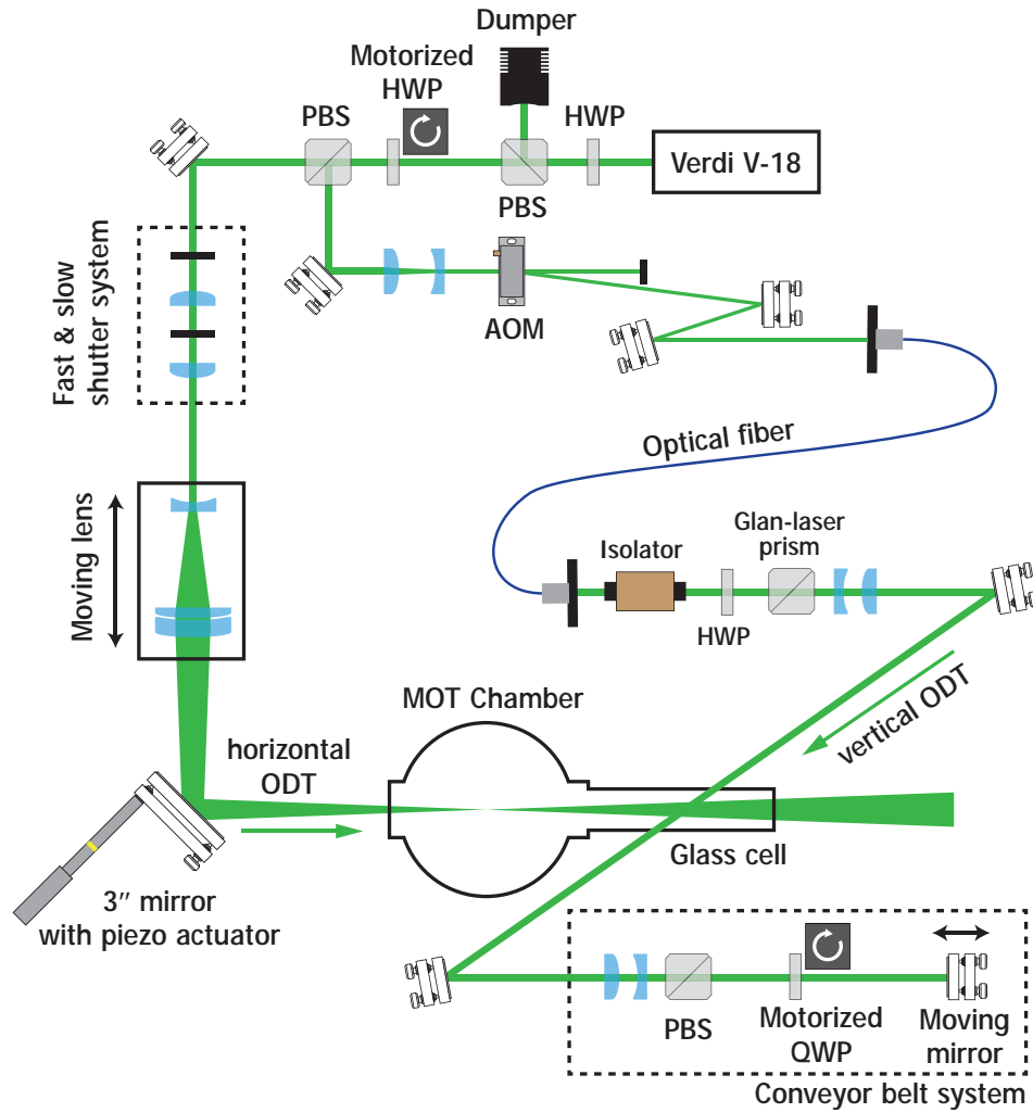
Figure 4.13: Optical system for the horizontal and vertical ODT derived from a 18W, frequency-doubled DPSS laser.
