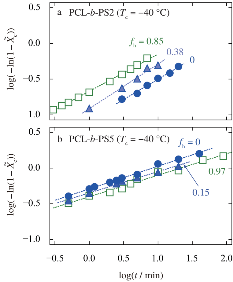
Figure 4.7. Avrami plots for the isothermal crystallization of PCL- b -PS2 blends (a) and PCL- b -PS5 blends (b) at -40 °C. Only the data for representative values of f_h are shown. Dashed lines indicate the results of linear fitting.
