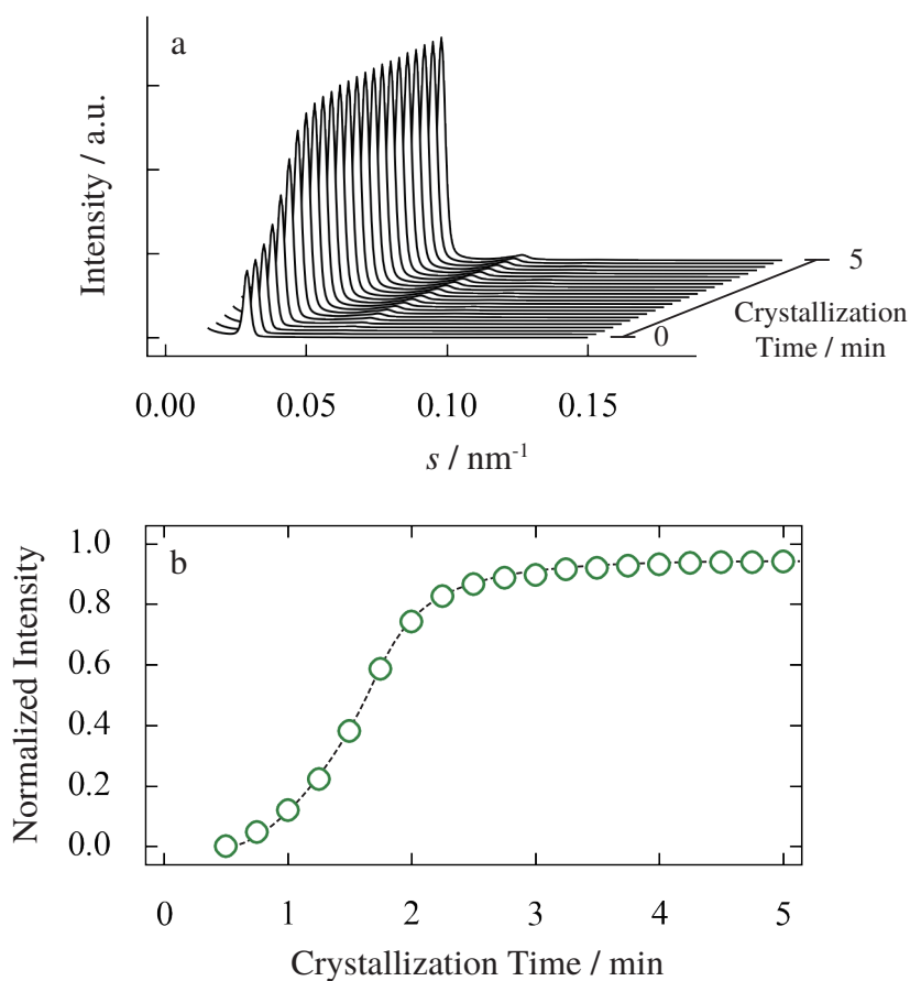
Figure 5.9. Time development of SAXS curves (a) and normalized primary peak intensity (b) for PCL/PS7 during isothermal crystallization at T_c = 40\text{ }^{\circ}\text{C} . A dashed curve is just a guide for the eye.
