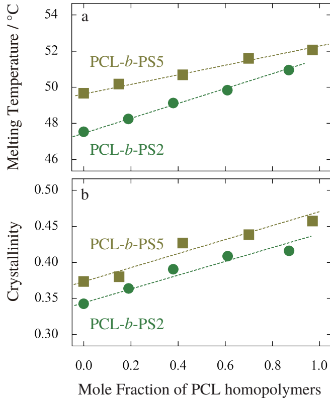
Figure 4.5. Final melting temperature T_m (a) and crystallinity X_c (b) of PCL crystals after isothermal crystallization at -40^\circ\text{C} plotted against the mole fraction of PCL homopolymers f_h for PCL- b -PS2 (circles) and PCL- b -PS5 (squares). Dashed lines are just a guide for the eye.
