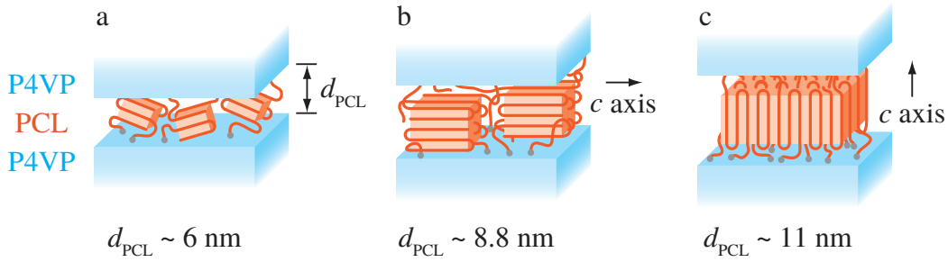
Figure 1.11. Schematic illustration of the crystal orientation of PCL blocks confined in nanolamellae formed in PCL- b -P4VP.
