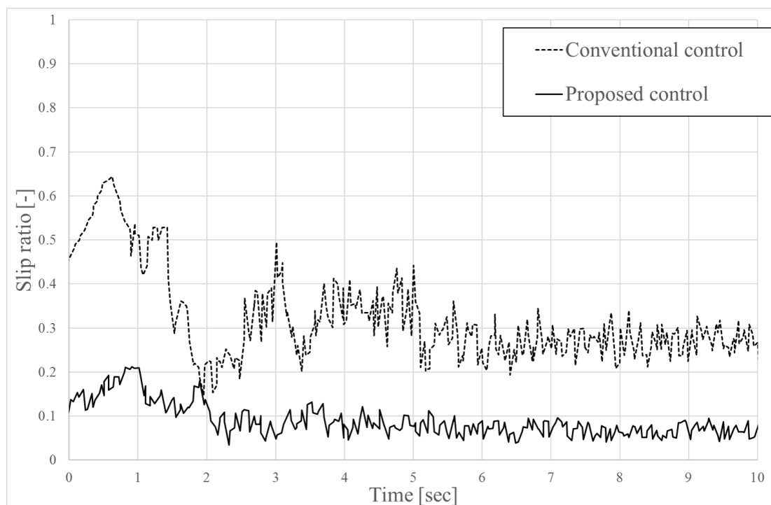
Figure 6-12 Control result
