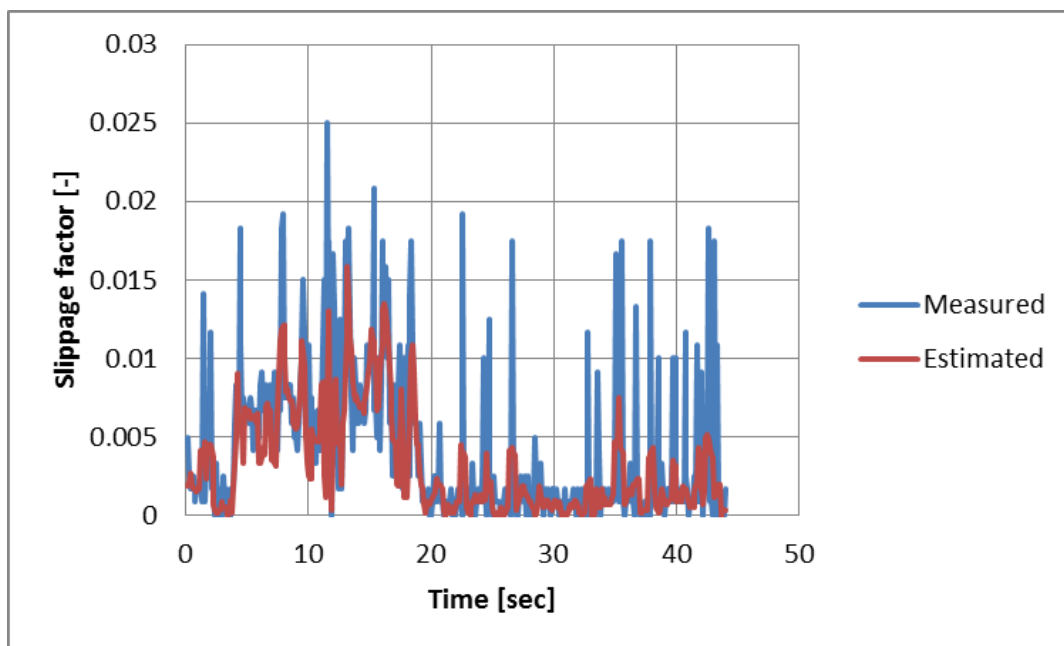
Figure 5-28 Amount of slip on the rotation direction
