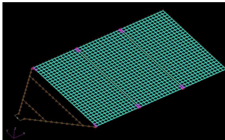
Figure 3-13 Initial thermal-structural model for solar array (Global image)
