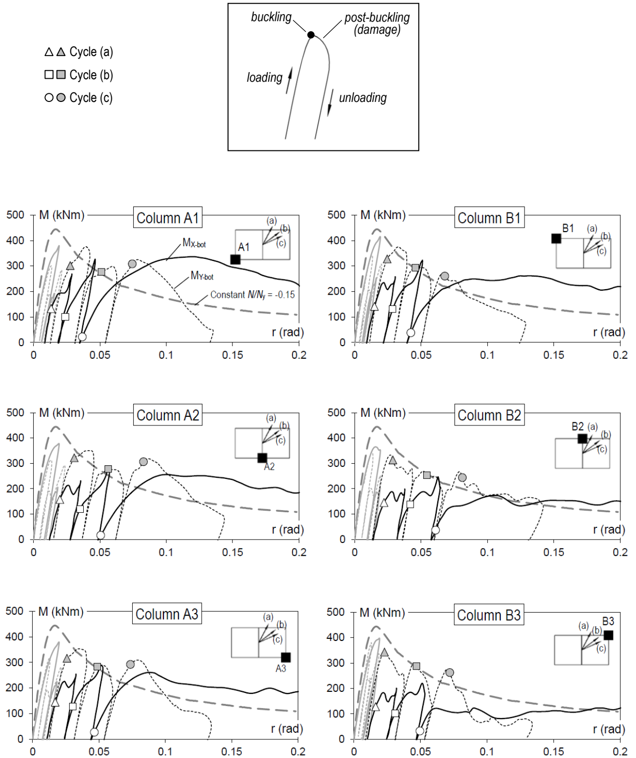
Figure 3.6 Accumulated deteriorations of first-story column bottom moments characterized by skeleton curves for the negative M_{Y-bot} and positive M_{X-bot} , with symbols commonly showing both values at the times of 3.35s, 4.43s and 5.73s of three cycles (a), (b) and (c), respectively.
