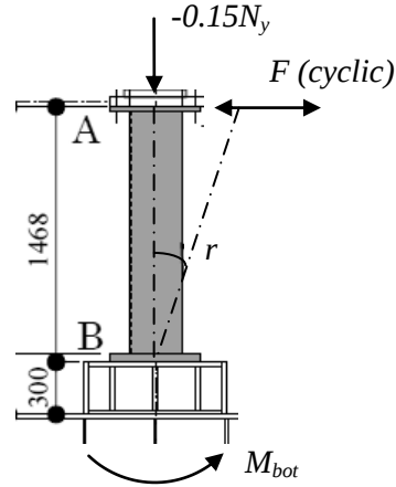
Component test setup
