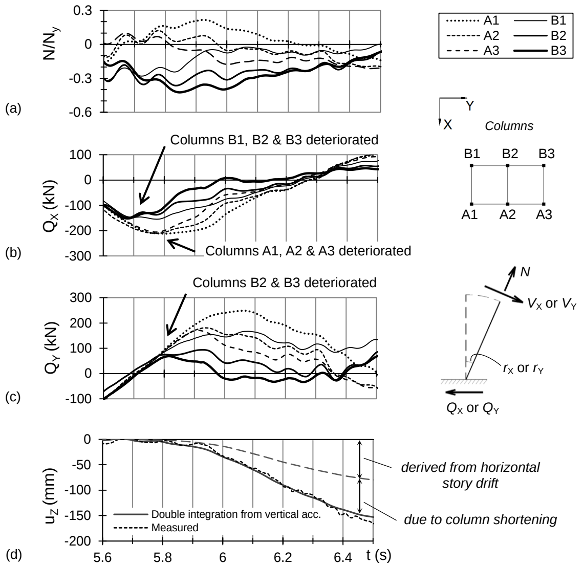
Figure 3.7 Time histories of 1 st -story column (a) axial forces, (b) horizontal shear forces Q_x , (c) Q_y , and (d) 2 nd -floor downward displacement (100% Takatori level).
