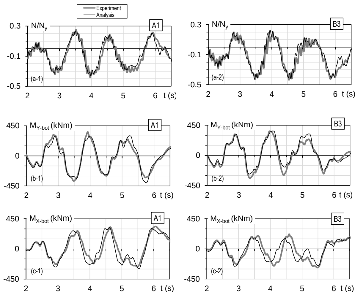
Figure 5.4 Comparison of the nonlinear local responses between analytical results (thin line) and experimental records (thick line) at 100% Takatori level: (a) axial load, (b) M_{Y-bot} and (c) M_{X-bot} of the first-story columns A1 and B3.
