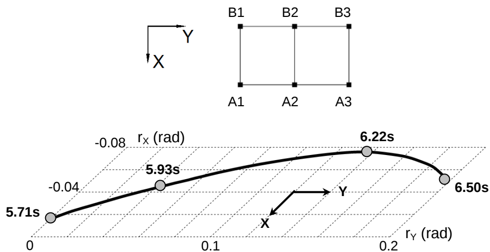
Figure 3.12 First-story drift ratio orbit (5.71-6.50s, 100% Takatori)
