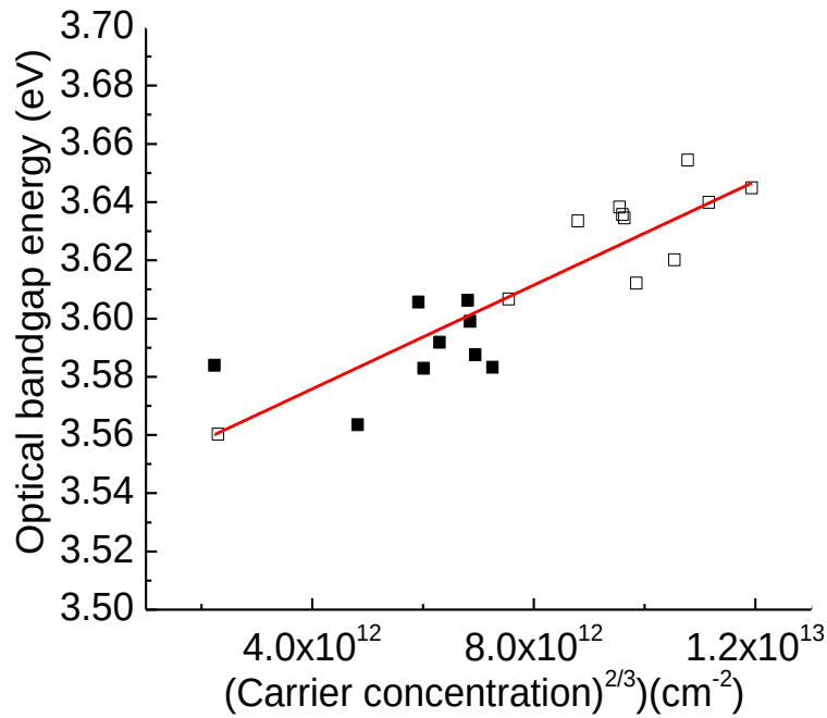
Fig. 3.26 Dependence of E_{opt} of Al doped \text{Zn}_{0.87}\text{Mg}_{0.13}\text{O} thin film on carrier concentration. The red line is linear fitting to the data. The void points refer to the sample that firstly annealed in nitrogen at 650 °C and secondly annealed in forming gas at 500 °C, while the filled points refer to the sample that firstly annealed in air at 500 °C and secondly annealed in forming gas at 450 °C.
