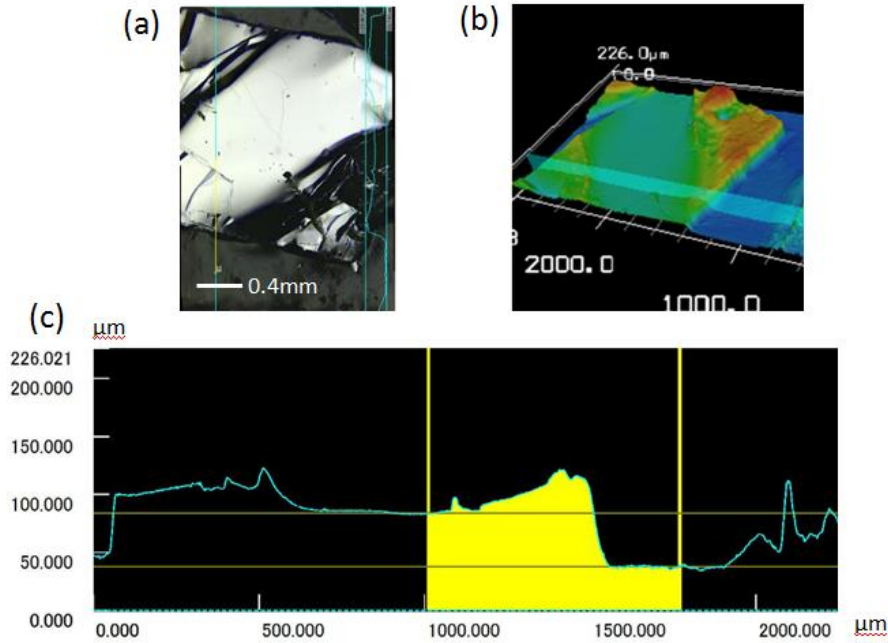
Fig. 2-3 The laser microscope images of Bi 2 Se 3 single crystal, (a) metal-like and (b) flat surface, and (c) the bulk sample thickness of 46 μm.
