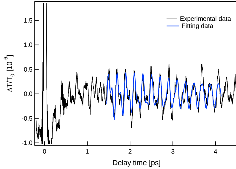
Fig. 3-14 Transient transmission of Sb 2 Te 3 ultra thin-film.
