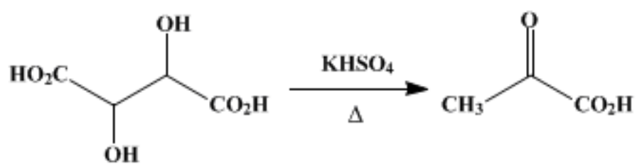
Figure 3-3. Chemical synthesis route of pyruvic acid from heating tartaric acid and KHSO 4 .
