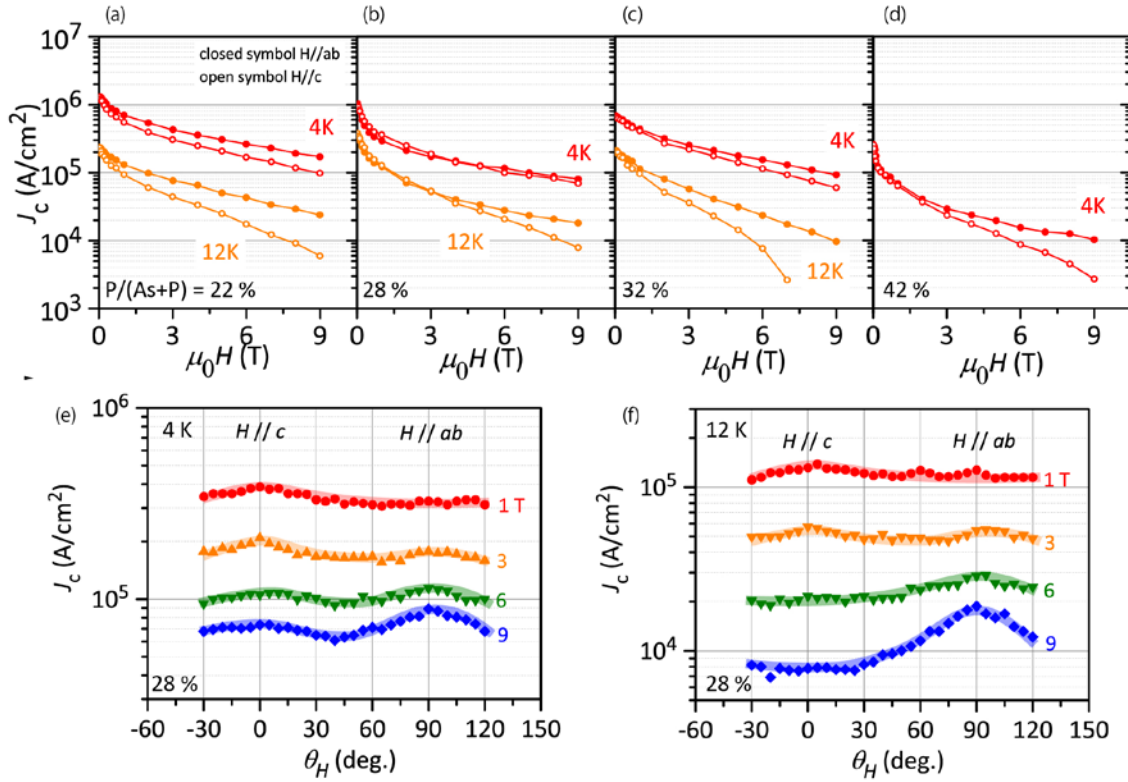
Figure 8 - 7. Doping concentration dependence of transport J_c . J_c of \text{P}/(\text{P}+\text{As}) = 0.22 (a), 0.28 (b), 0.32 (c) and 0.42 (d) as a function of magnetic field. (e, f) angular dependence of J_c of optimally-doped \text{BaFe}_2(\text{As}_{1-x}\text{P}_x)_2 film on IBAD-substrate at 4 K (e) and 12 K (f)
