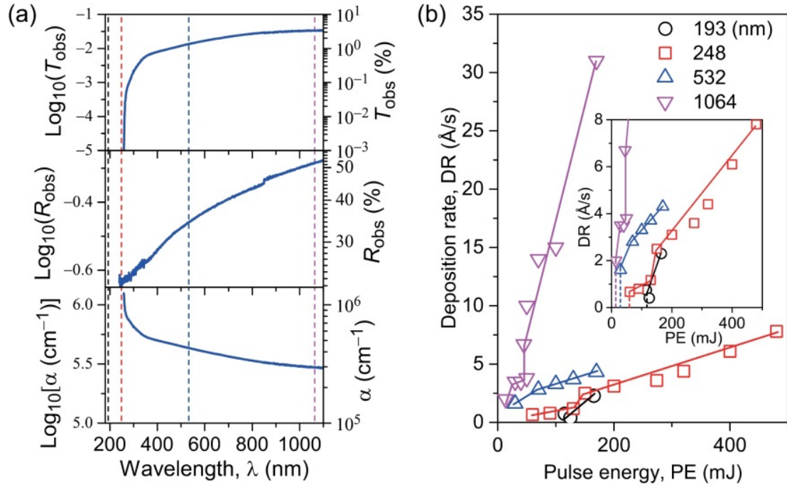
Figure 2 - 1. (a) Optical spectra ( T_{\text{obs}} , R_{\text{obs}} , and \alpha ) of a 90-nm-thick BaFe 2 As 2 :Co epitaxial film at room temperature. The vertical dashed lines indicate the laser wavelengths used in this study. (b) Dependence of deposition rate of BaFe 2 As 2 :Co films on pulse energy. The PLD laser wavelengths are shown in the upper right. The inset shows an enlarged image from the region of deposition rates less than 8 \text{\AA/s} , more clearly showing the kinks.
