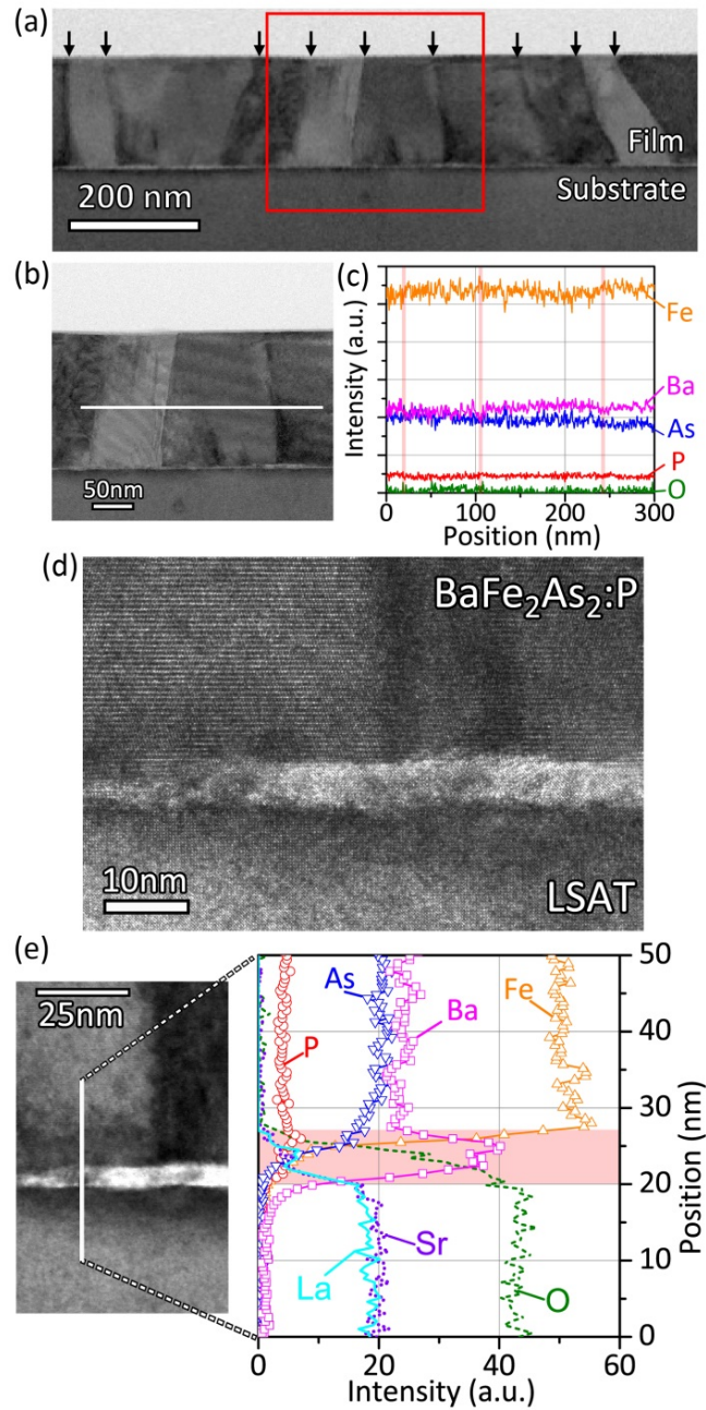
Figure 6 - 3 Microstructure and chemical composition of a BaFe 2 As 2 :P epitaxial film on a LSAT (001) substrate. The incident direction of the electron beam is BaFe 2 As 2 :P [100]. (a) Cross-sectional bright-field STEM image. Vertical arrows show the vertical defects. (b) Magnified image of the square region in Fig (a). (c) STEM-EDX line scan along the horizontal line shown in Fig. (b). The vertical lines correspond to the positions of the vertical defects. (d) HR-TEM image at the interface between the BaFe 2 As 2 :P film and LSAT substrate. (e) Left panel shows STEM image at the interface. Right panel shows the results of STEM-EDX line scan along the vertical line shown in the left panel. The shaded region corresponds to the interfacial layer.
