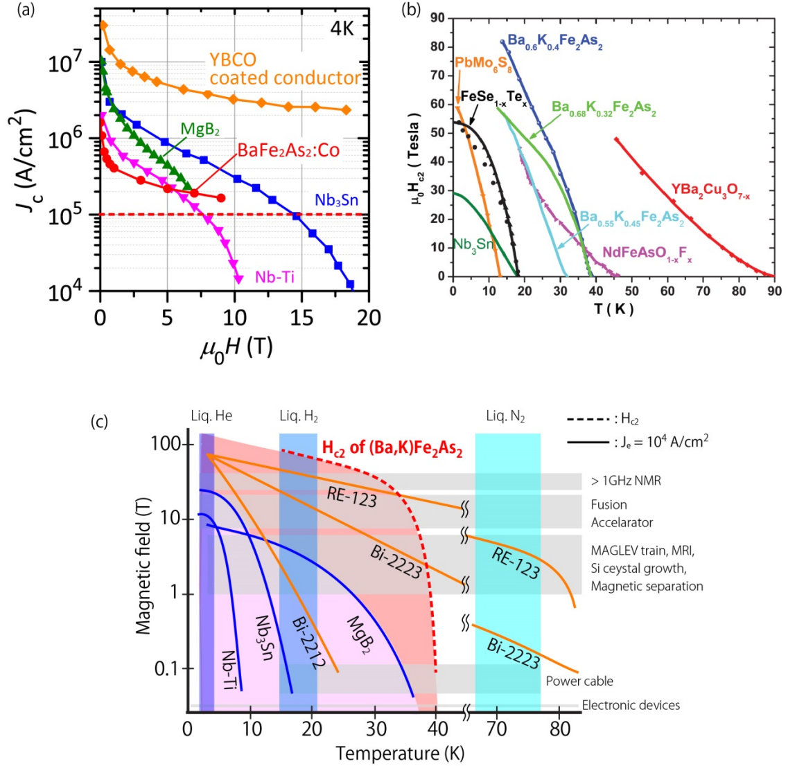
Figure 1 - 9. Comparison of superconducting properties with other superconductors. (a) magnetic field dependence of J_c . Also shown for comparison are the data for YBCO 137 , MgB_2 138 , Nb_3Sn 65 and Nb-Ti . Dashed lines indicate the J_c limits if it was operate in practical applications. (b) Temperature dependence of H_{c2} 139 . (c) Applicable conditions for engineering J_c J_e > 10^4 A cm 2 for various superconducting tapes and wires. The low temperature and low temperature region area (magenta shaded area) can be covered by using conventional superconductors. Compared with conventional superconductors 140 , iron-based conductors have great potential not only in high magnetic field but also high temperature (red shaded area).
