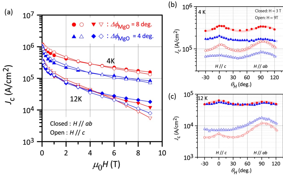
Figure 8 - 9. Misorientation angle dependence of transport J_c of \text{BaFe}_2(\text{As}_{0.72}\text{P}_{0.28})_2 on IBAD-substrates with \Delta\phi_{\text{MgO}} = 4^\circ and 8^\circ (a) Transport J_c as a function of magnetic field. (b, c) Angular dependence of J_c at 4 K (b) and 12 K (c)
