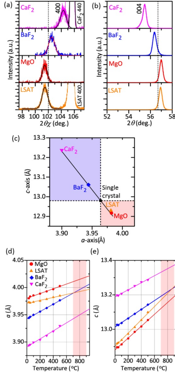
Fig. 2. XRD patterns and structural parameters of BaFe 2 As 2 :Co thin films on oxide and fluoride single-crystal substrates. (a) In-plane \phi -coupled 2\theta\chi patterns around 400 diffractions at room temperature. Solid lines are results of deconvolution. (b) Out-of-plan \omega -coupled 2\theta patterns around 004 diffractions at room temperature. (c) Summary of lattice parameters calculated from (a) and (b). Vertical dotted lines in (a) – (b) indicates the peak position of a single crystal taken from ref ** [A. S. Sefat et al., PRL (2008)]. Upper left shaded area indicates a -axis is compressed and c -axis is expanded. Lower right shaded area indicates a -axis expanded and c -axis is compressed. (d, e) Temperature dependence of lattice parameters of the films. The shaded temperature regions correspond to the epitaxial growth windows. Solid lines are fitted lines from RT to 500 °C as the guide to the eye.
