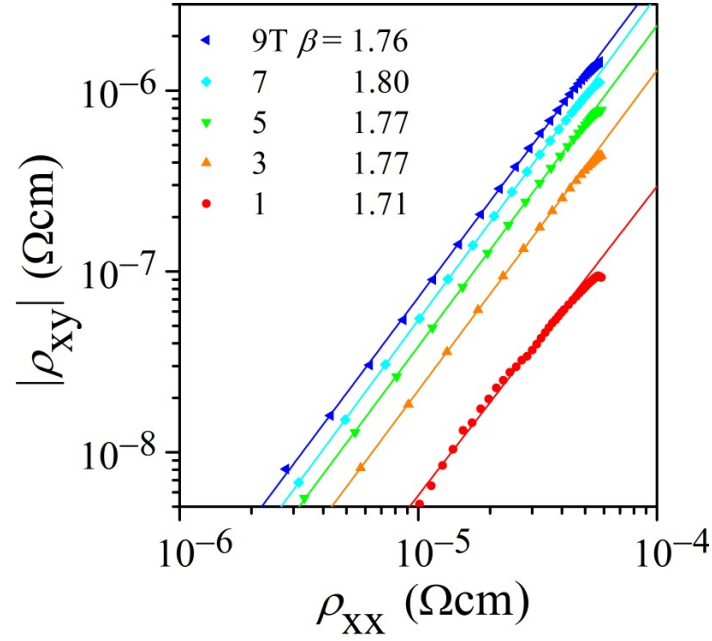
Figure 3 - 2. T sweep scaling behavior between \rho_{xy} and \rho_{xx} under fixed magnetic fields varied from 1 to 9 T. Solid lines show fitted results using the relation \rho_{xy} = A\rho_{xx}^\beta . Magnetic fields and the \beta values are shown on top left.
