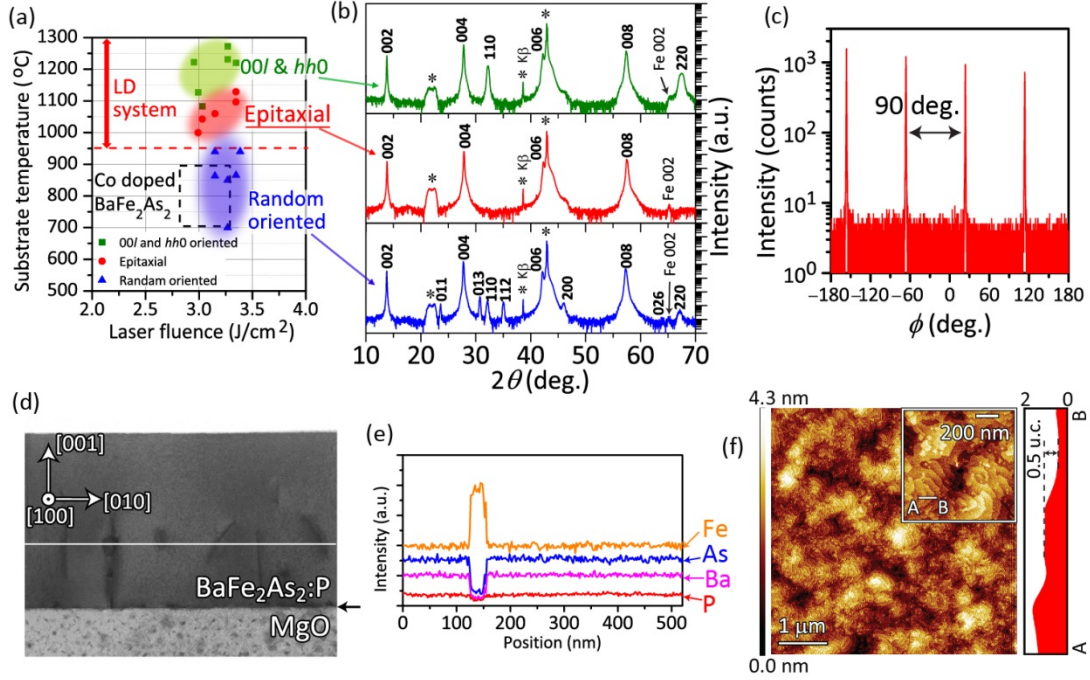
Figure 6 - 1. Growth of BaFe 2 As 2 :P films and structural and electrical properties of the epitaxial film. (a) Relationship between growth condition (substrate temperature T_s and laser fluence) and crystallographic orientation of BaFe 2 As 2 :P films. Three regions with different orientation structures obtained with different T_s values are shown. The dashed square region shows the optimum condition for epitaxial growth of BaFe 2 As 2 :Co. [17] (b) Typical XRD patterns, measured in Bragg-Brentano configuration, of BaFe 2 As 2 :P thin films for the three T_s regions in panel (a). (c) In-plane \phi scan of the 200 diffractions of the BaFe 2 As 2 :P thin film grown at the optimum T_s . (d) Cross-sectional bright-field STEM images of BaFe 2 As 2 :P epitaxial films. Horizontal arrows indicate the heterointerfaces between the films and MgO substrates. (e) the results of EDXS line-scans along the white horizontal lines in panels (d) (f) AFM scan showing surface morphology of BaFe 2 As 2 :P film grown at the optimum T_s . Upper-right inset shows a magnified image. A cross-sectional profile along the horizontal line A-B in the inset is shown to the right ("0.5 u.c." denotes the half size of the c-axis unit-cell length).
