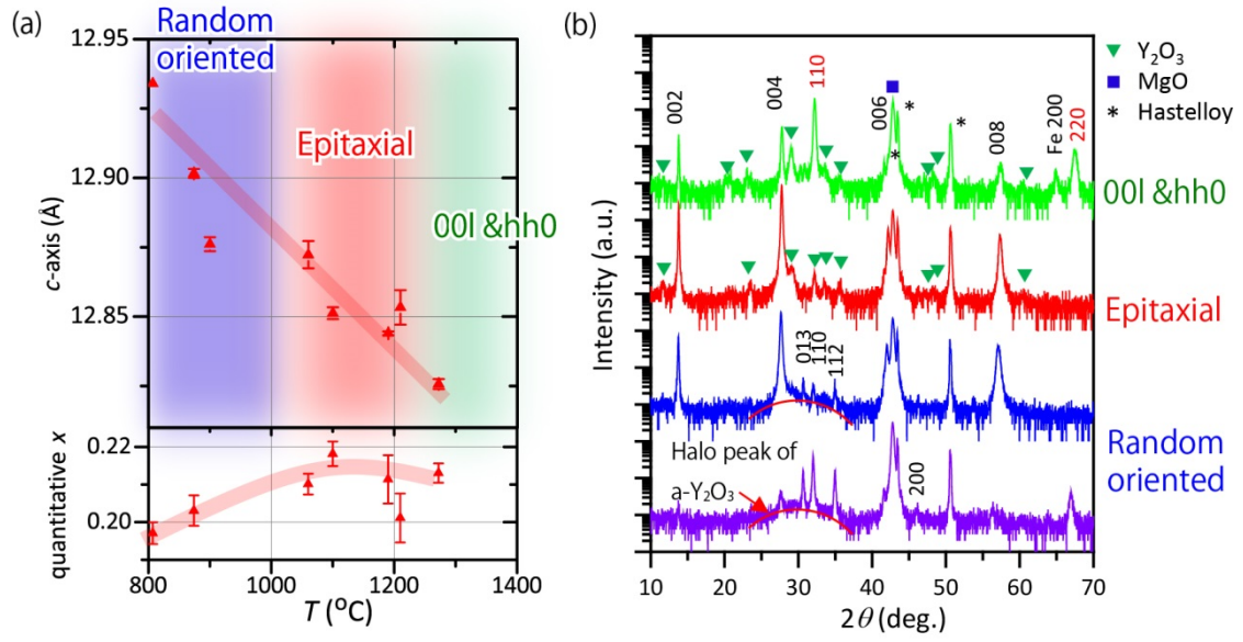
Figure 8 - 3 Growth condition of \text{BaFe}_2(\text{As}_{0.78}\text{P}_{0.22})_2 epitaxial films on IBAD-substrates. (a) Relationship between growth condition (substrate temperature T_s , c -axis length and doping concentration). Crystallographic orientation of \text{BaFe}_2\text{As}_2\text{:P} films are also shown. Three regions with different orientation structures obtained with different T_s values are shown. (b) Typical XRD patterns, measured in Bragg–Brentano configuration, of \text{BaFe}_2\text{As}_2\text{:P} thin films for the three T_s regions in panel (a). In T_s > 1000 °C, a- \text{Y}_2\text{O}_3 start to crystalize.
