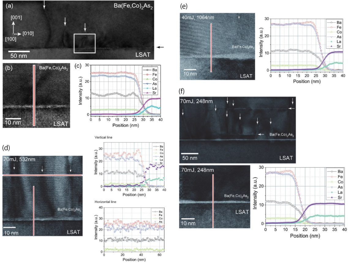
Figure 2 - 3. Examination of a BaFe 2 As 2 :Co epitaxial film grown by several excitation sources. (a) Cross-sectional TEM image of a BaFe 2 As 2 :Co epitaxial film grown by the KrF excimer laser at the optimum pulse energy. The vertical white arrows indicate defects along the c -axis. The horizontal black arrow on the right shows the position of the film/LSAT interface. (b) Magnified view of the white square shown in (a). (c) EDX line-scan spectra along the red vertical line shown in (b). Cross-sectional TEM images of BaFe 2 As 2 :Co films grown by ablations at (d) optimum pulse energy (70 mJ) of 532 nm, (e) optimum pulse energy (40 mJ) of 1064 nm, and (f) low pulse energy (70 mJ) of 248 nm. The vertical and horizontal white arrows indicate the vertical defects along the c -axis and stacking faults, respectively. (right) EDX line-scans along the red lines in the TEM images.
