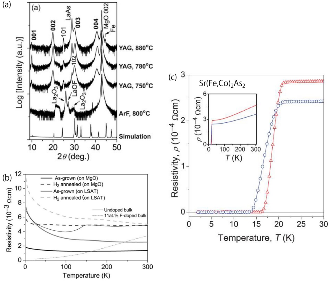
Figure 1 - 5. (a) XRD patterns of LaFeAsO 1-x F x epitaxial films. (b) \rho - T curve of LaFeAsO epitaxial films which treated by annealing technique. (c) \rho - T curve of Sr(Fe 1-x Co x ) 2 As 2 film in temperature range 0–30 K 47 .
