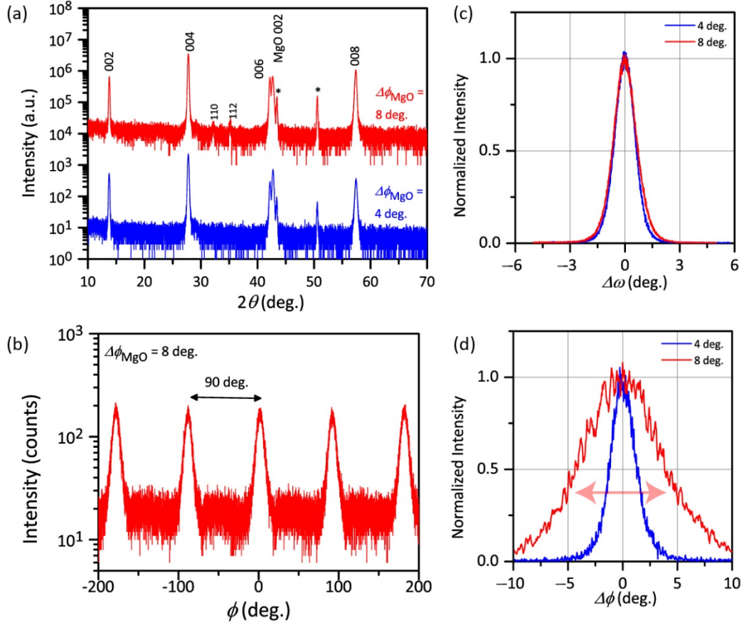
Figure 8 - 8. XRD patterns and structural parameters of \text{BaFe}_2(\text{As}_{0.72}\text{P}_{0.28})_2 epitaxial films on IBAD-substrates with \Delta\phi_{\text{MgO}} = 8^\circ . (a) Out-of-plan \omega -coupled 2\theta patterns. (b) \phi scan of 103 diffraction of \text{BaFe}_2(\text{As}_{0.72}\text{P}_{0.28})_2 . (c, d) Normalized rocking curves of the out-of-plane 004 (b) and the in-plane 200 reflections (c). For comparison, the rocking curves of \text{BaFe}_2(\text{As}_{0.72}\text{P}_{0.28})_2 epitaxial film on IBAD-substrate with \Delta\phi_{\text{MgO}} = 4^\circ is plotted.
