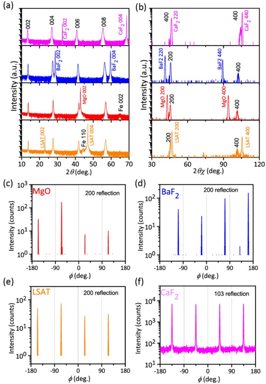
Supplemental Figure 2. HR-XRD data of BaFe 2 As 2 :Co thin films. Wide range scan data of BaFe 2 As 2 :Co thin films show the clear 00l diffractions in out-of-plane (a) and h00 diffractions in in-plane (b) with small peak of non-oriented Fe and/or Fe-Co alloy particles. According to the tetragonal lattice of BaFe 2 As 2 :Co, clear four-fold symmetric peaks are observed in \phi scan (c – f). BaFe 2 As 2 :Co on CaF 2 has very close a -axis value; therefore 103 reflection is used to confirm the four-fold symmetry of tetragonal lattice.
