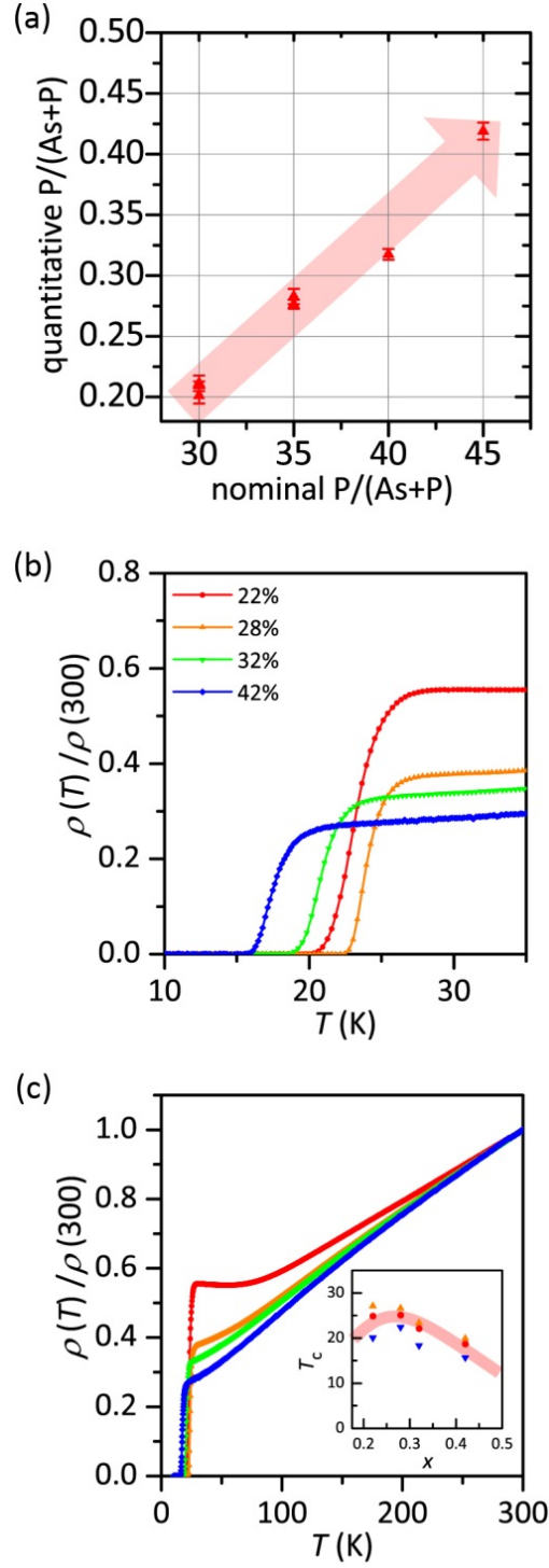
Figure 8 - 6. Doping concentration dependence of structural parameters and T_c . (a) Chemical composition analysis using EPMA. (b,c) Temperature dependence of resistivity \rho of \text{BaFe}_2(\text{As}_{1-x}\text{P}_x)_2 film on IBAD-substrate as a function of the doping concentration x . (b) magnified image around T_c . (c) Wide range : 10 – 300 K. Inset figure of (c) is phase diagram of \text{BaFe}_2(\text{As}_{1-x}\text{P}_x)_2 . Circles, triangles and reversed triangles indicate T_c , T_c onset and T_c zero.
