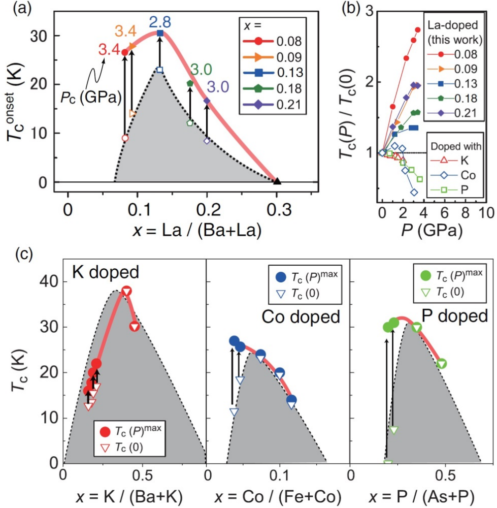
Figure 5 - 6 (a) High-pressure electronic phase diagram of (\text{Ba}_{1-x}\text{La}_x)\text{Fe}_2\text{As}_2 epitaxial films in comparison with that under an ambient pressure. Solid and open symbols show the maximum T_c^{\text{onset}} ( T_c^{\text{max}} ) obtained under high pressures and those under an ambient pressure, respectively. The critical pressures ( P_c ), where T_c^{\text{max}} was obtained, are indicated in the figure. (b) Enhancement factors defined by T_c(P)/T_c(0) as a function of P for (\text{Ba}_{1-x}\text{La}_x)\text{Fe}_2\text{As}_2 epitaxial films. Those of the optimally, K(indirect hole)-, P(indirect isovalent)-, and Co(direct electron)-doped \text{BaFe}_2\text{As}_2 single crystals are shown for comparison (Refs. 7,8, and 11). (c) Pressure phase diagrams of (\text{Ba}_{1-x}\text{K}_x)\text{Fe}_2\text{As}_2 (indirect hole-doped), \text{BaFe}_2(\text{As}_{1-x}\text{P}_x)_2 (indirect isovalent-doped), and \text{Ba}(\text{Fe}_{1-x}\text{Co}_x)_2\text{As}_2 (direct electron-doped) single crystals (Refs. 7–11). Typical electronic phase diagrams under an ambient pressure are shown by the dark areas. Solid and open symbols indicate T_c^{\text{max}} under external pressures [ T_c(P)^{\text{max}} ] and T_c at 0 GPa, respectively.
