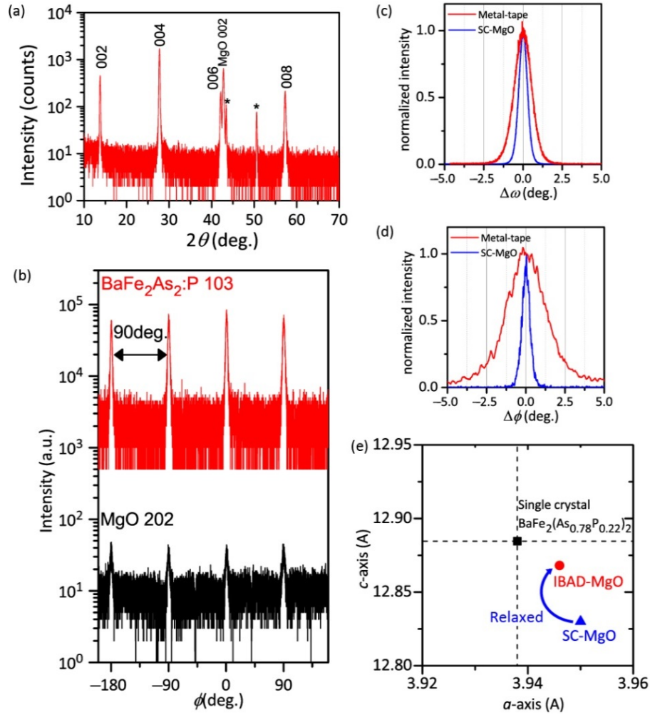
Figure 8 - 4. XRD patterns and structural parameters of \text{BaFe}_2(\text{As}_{0.78}\text{P}_{0.22})_2 epitaxial films on IBAD-substrates. (a) Out-of-plan \omega -coupled 2\theta patterns. (b) \phi scan of 103 diffraction of \text{BaFe}_2(\text{As}_{0.78}\text{P}_{0.22})_2 and 202 diffraction of MgO. (c, d) Normalized rocking curves of the out-of-plane 004 (c) and the in-plane 200 reflections (d). For comparison, the rocking curves of \text{BaFe}_2(\text{As}_{0.78}\text{P}_{0.22})_2 epitaxial film on single-crystal MgO (SC-MgO) is referred from chapter 6. (e) Comparison of lattice parameters with those of \text{BaFe}_2(\text{As}_{0.78}\text{P}_{0.22})_2 epitaxial film on SC-MgO. Dotted lines indicates the lattice parameters of a single crystal \text{BaFe}_2(\text{As}_{0.78}\text{P}_{0.22})_2 taken from ref 11 .
