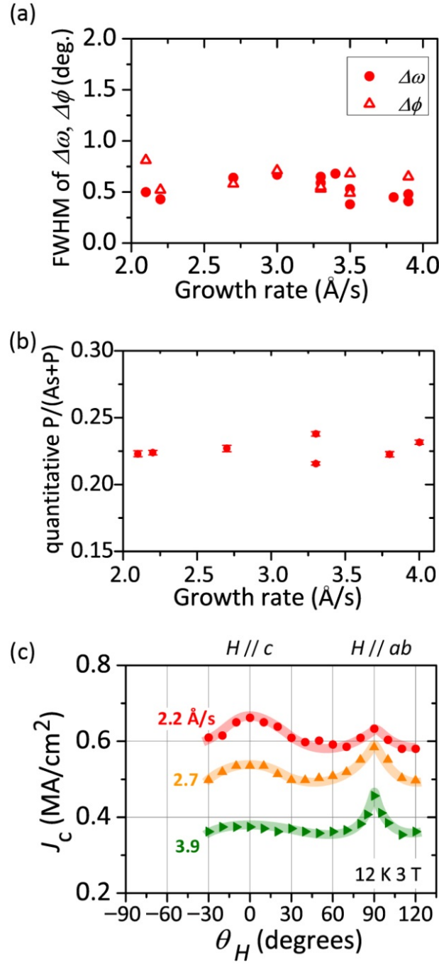
Figure 7 - 3 Growth rate dependence of crystallinity, chemical composition and vortex pinning property. (a) Dependence of FWHM of \Delta\omega and \Delta\phi on growth rate of BaFe 2 As 2 :P films grown at the optimum T_s . (b) Quantitative P concentration of thin films grown at the various growth rate. (c) Critical current density J_c as a function of angle of applied magnetic field \theta_H for BaFe 2 As 2 :P epitaxial films grown at three growth rates, with \mu_0 H = 3 T and T = 12 K.
