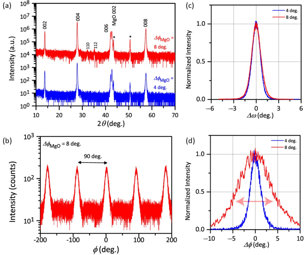
Figure 8 - 8. XRD patterns and structural parameters of \text{BaFe}_2(\text{As}_{0.72}\text{P}_{0.28})_2 epitaxial films on IBAD-substrates with \Delta\phi_{\text{MgO}} = 8^\circ . (a) Out-of-plan \omega -coupled 2\theta patterns. (b) \phi scan of 103 diffraction of \text{BaFe}_2(\text{As}_{0.72}\text{P}_{0.28})_2 . (c, d) Normalized rocking curves of the out-of-plane 004 (b) and the in-plane 200 reflections (c). For comparison, the rocking curves of \text{BaFe}_2(\text{As}_{0.72}\text{P}_{0.28})_2 epitaxial film on IBAD-substrate with \Delta\phi_{\text{MgO}} = 4^\circ is plotted.
