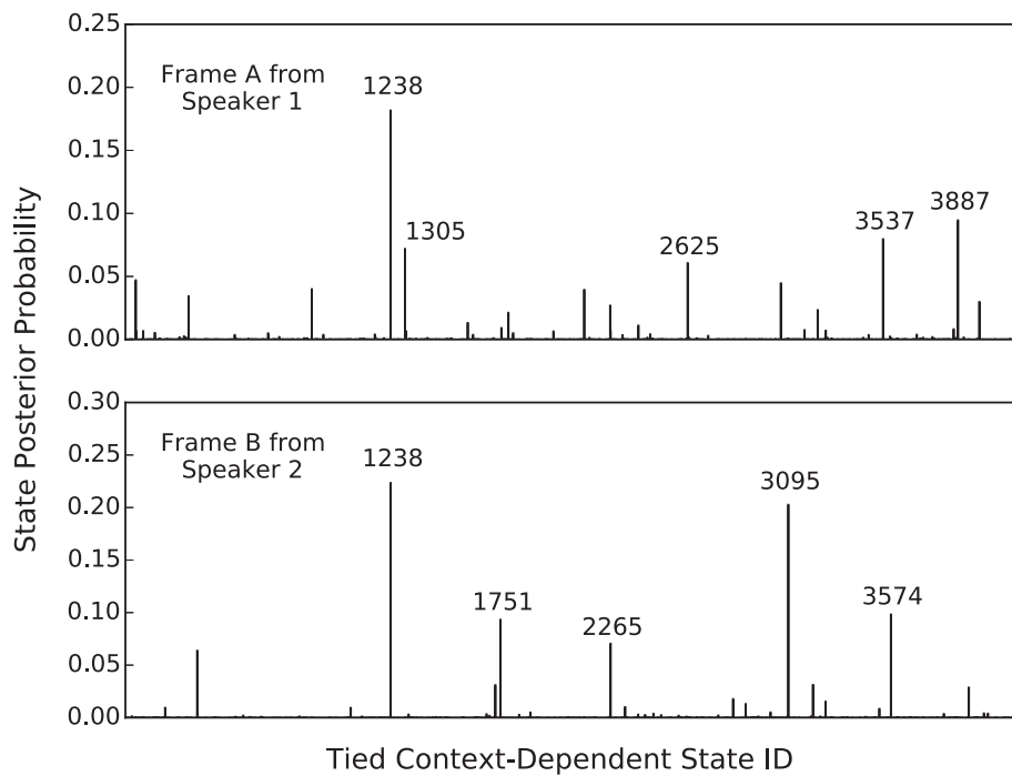
Fig. 2 Teacher DNN outputs for inputs from the same class. Posterior probability outputs by a teacher DNN for two inputs belonging to the same tied CD state are shown with state IDs for the five states having the highest posterior probability shown next to their corresponding bars. Even though the center frame belongs to the state, the output distributions are markedly different for the two inputs from different speakers, revealing different notions of similarity to other states learned by the teacher. This information can be conveyed to the student through soft targets but not hard targets
