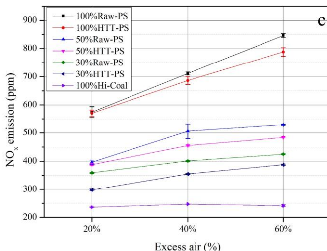
Figure 5-3 Average \text{NO}_x emission (ppm): (a) combustion; (b) co-combustion with low reactivity coal; (c) co-combustion with high reactivity coal. (Raw-PS: raw paper sludge; HTT-PS: hydrothermally treated paper sludge; Lo-Coal: low reactivity coal; Hi-Coal: high reactivity coal)
