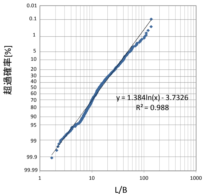
図2-20 L/BのHazen-plot
