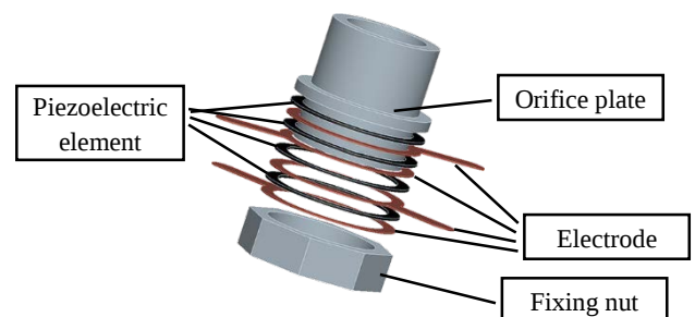
Fig. 2 Structure of the valve.
