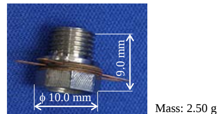
Fig. 1 Photograph of the assembled valve.
