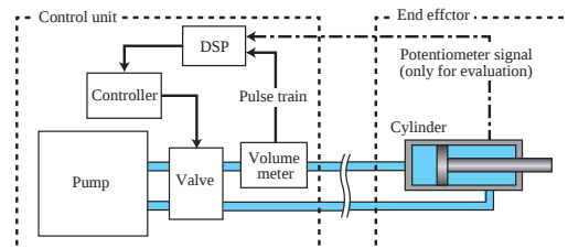
Fig.1 Schematic figure of the proposed feedback system.
