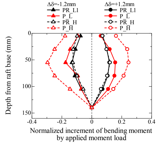
(h) Pull-out pile ( \delta_{LDT} = \pm 2\text{mm} , h/S=1.8 )
