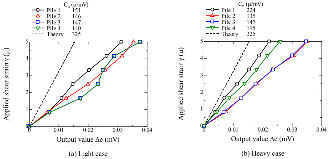
Figure 3.6.9 Relationship between output value and applied shear strain.
