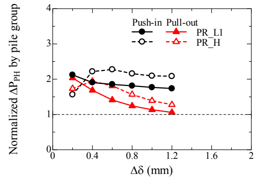
(f) Push-in & pull-out piles ( \delta_{LDT} = \pm 2\text{mm} , h/S=1 )
