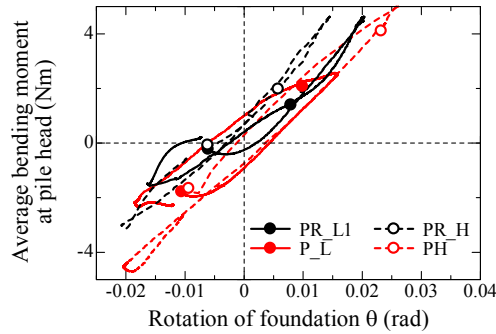
Figure 5.5.2.7 Relationship between rotation of foundation \theta and average bending moment at pile head for \delta_{LDT} = \pm 2\text{mm} and h/S = 1.8 .
