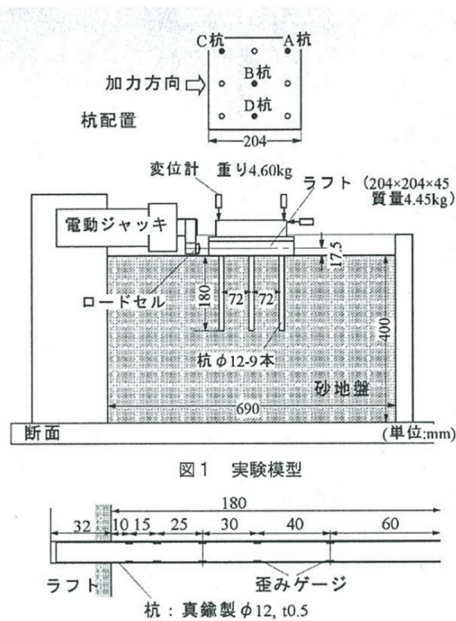
Figure 2.3.32 Model setup. (Mano et al. (2002, 2003))
