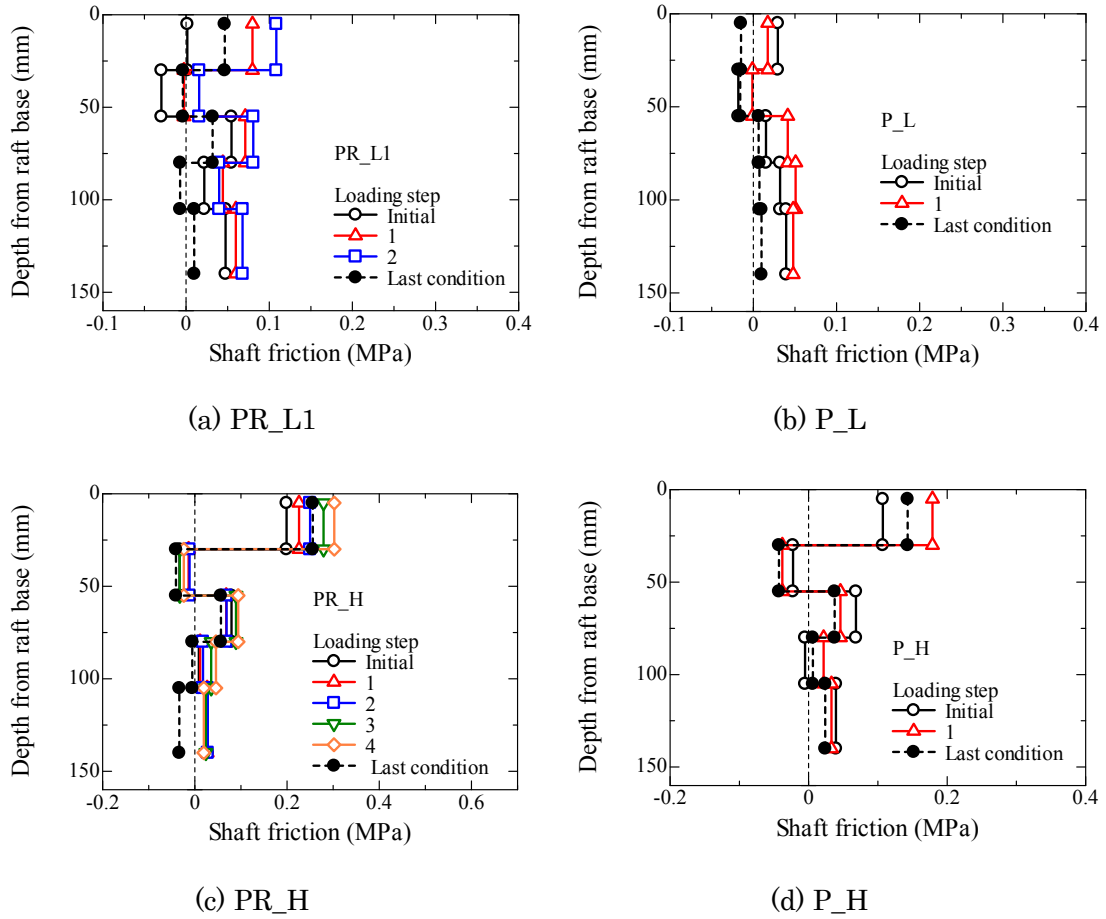
Figure 4.4.2.9 Profiles of shaft friction during pre-vertical loading process. (A. 4.4.2.14-4.4.2.17)
