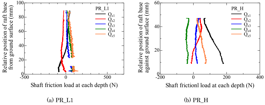
Figure 4.2.1.12 Variation of shaft friction at each depth with relative position of raft base from ground surface for PR_L1 and PR_H during penetration process.
