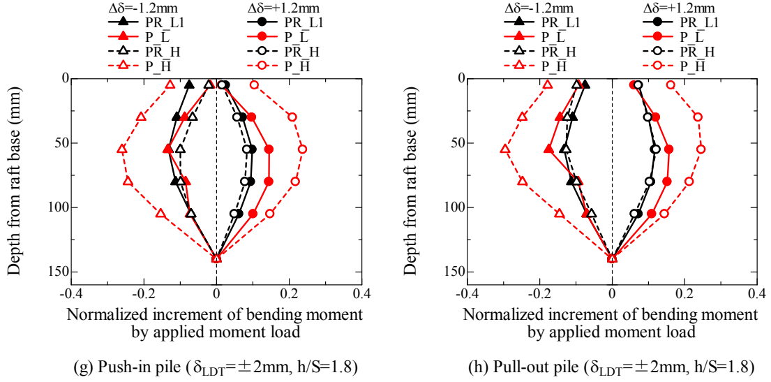
Figure 5.5.2.6 Profile of normalized bending moment by applied moment load at \Delta\delta = \pm 1.2\text{mm} . (A. 5.5.2.2)
