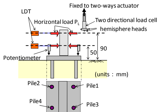
Figure 3.5.10 Schematic illustration of horizontal loading tests.
