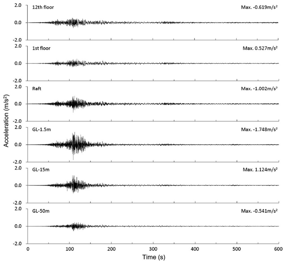
Figure 2.3.26 Time histories of acceleration at ground and superstructure. (Yamashita et al. (2012))
