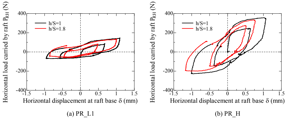
Figure 5.4.2.3 Relationship between \delta and horizontal load carried by raft part in piled raft P_{RH} .
