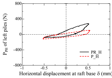
(c) Left piles ( \delta_{LDI} = \pm 1\text{mm} , h/S=1.8 )
