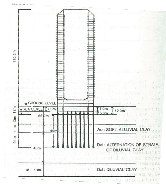
Figure 2.3.5 Soil profiles and section of the building. (Kishida (1991))
