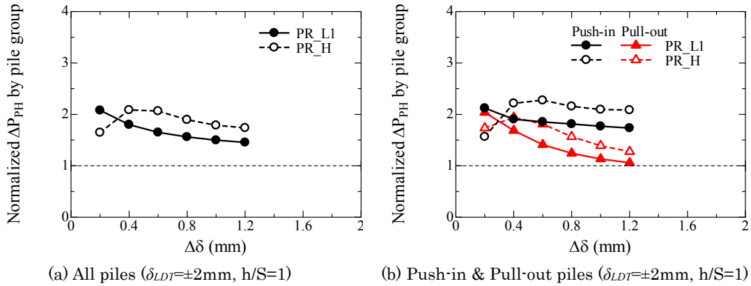
Figure 5.4.3.14 Relationship between \Delta\delta and normalized \Delta P_{PH} by that of pile group. (A. 5.4.3.11)
