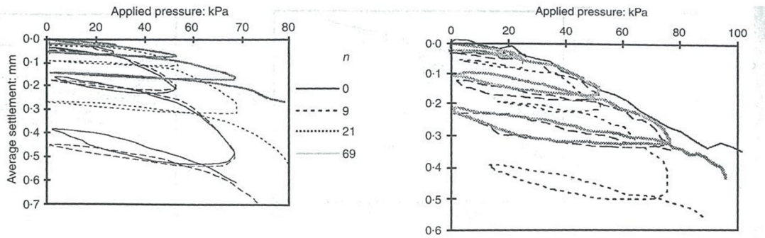
Figure 2.3.12 Average settlement of raft during loading tests. (Horikoshi and Randolph (1996))
