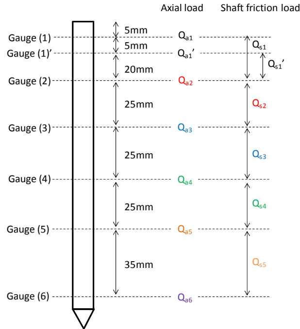
Figure 4.2.1.7 Definition of axial load and shaft friction load acting on pile.
