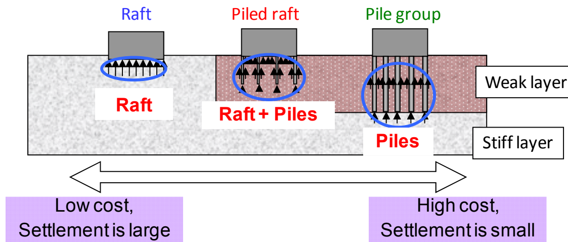
Figure 1.1.1 Foundation type and bearing capacity mechanism
