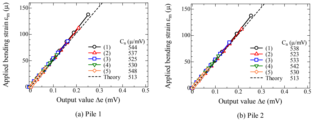
Figure 3.6.3 Relationship between output value and applied bending strain for light case pile.
