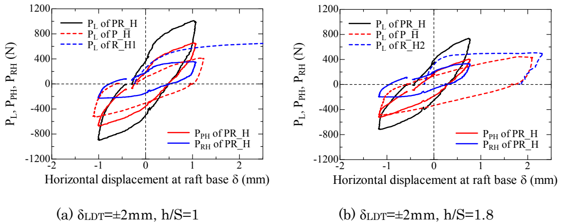
Figure 5.4.3.2 Variation of horizontal load P_L and horizontal load carried by raft P_{RH} and piles P_{PH} with horizontal displacement at raft base \delta for heavy case. (A. 5.4.2.2)
