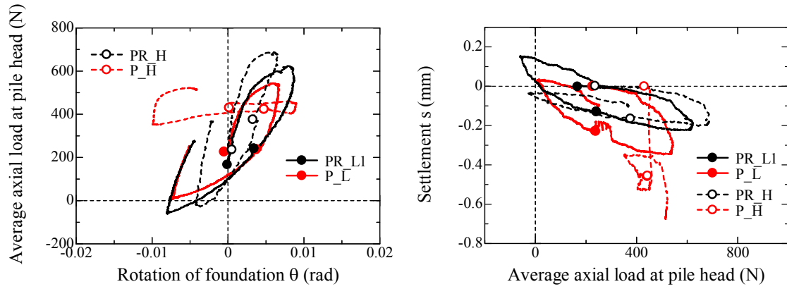
(a) Axial load at pile head (Left pile)
