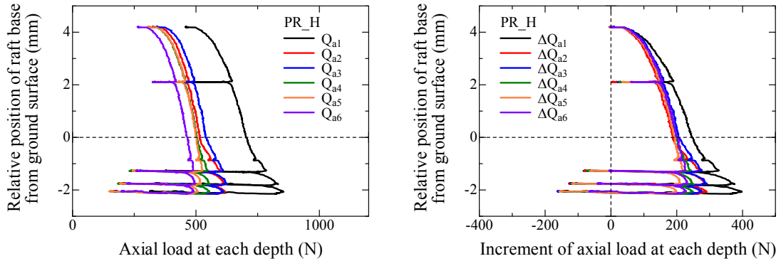
Figure 4.3.3.12 Variation of axial load and axial load increment at each depth with relative position of raft base from ground surface for PR_H during penetration process.
