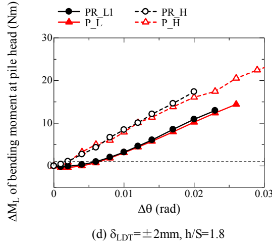
Figure 5.5.3.8 Relationship between \Delta\theta and \Delta M of bending moment at pile head for \delta_{LDT} = \pm 2\text{mm} and h/S = 1.8 . (A. 5.5.3.7)
