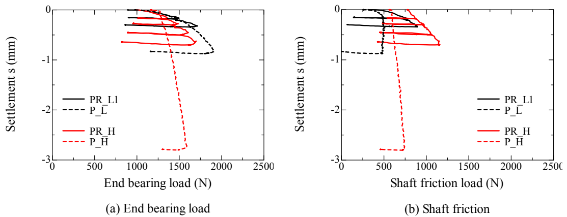
Figure 4.4.2.3 Relationship between pile load and settlement (a) end bearing load, (b) shaft friction load.
