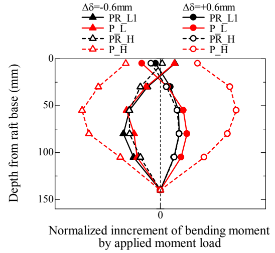
(b) Pull-out pile ( \delta_{LDT} = \pm 1\text{mm} , h/S=1 )
