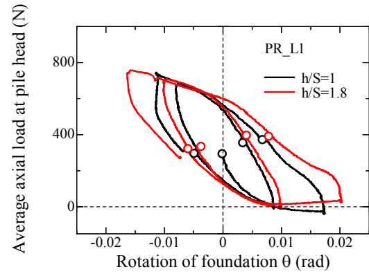
(b) Axial load at pile head (Right pile)
