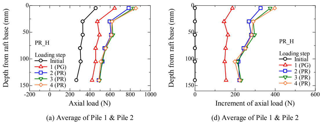
Figure 4.3.3.15 Profiles of axial load and axial load increment for PR_H during vertical loading process.
