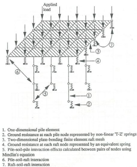
Figure 2.3.2 Numerical representation of piled raft. (Clancy and Randolph (1993))
