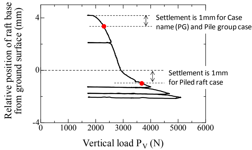
Figure 4.3.3.16 Positions in which axial loads are compared in Fig. 4.3.3.18.
