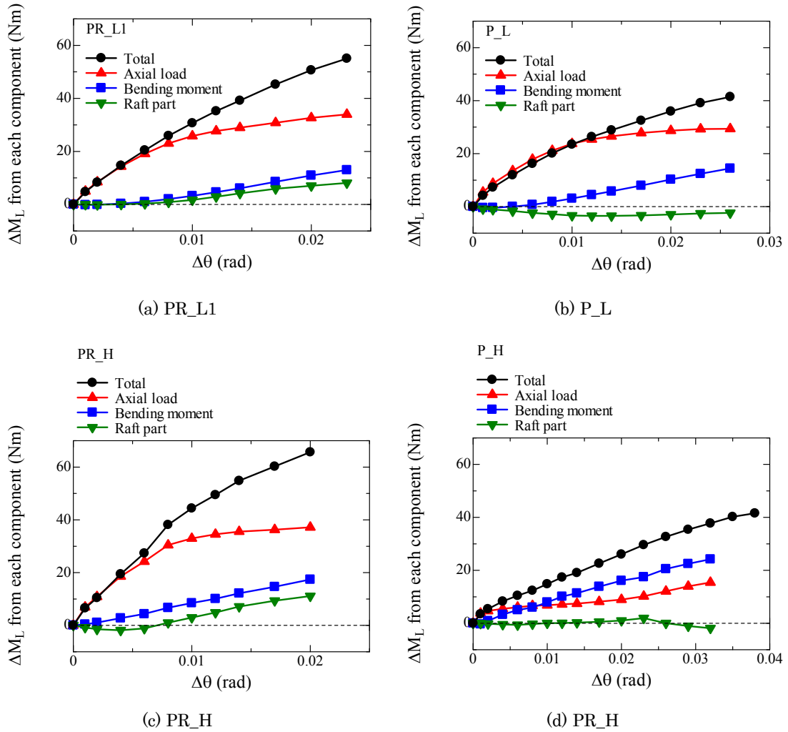
Figure 5.5.3.2 Relationship between \Delta\theta and \Delta M_L from axial load at pile head, bending moment at pile head and raft part. for \delta_{LDT} = \pm 2 mm, h/S = 1.8 . (A. 5.5.3.1-5.5.3.4)
