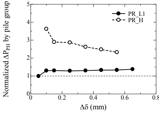
(a) All piles ( \delta_{LDT} = \pm 1\text{mm} , h/S = 1 )
