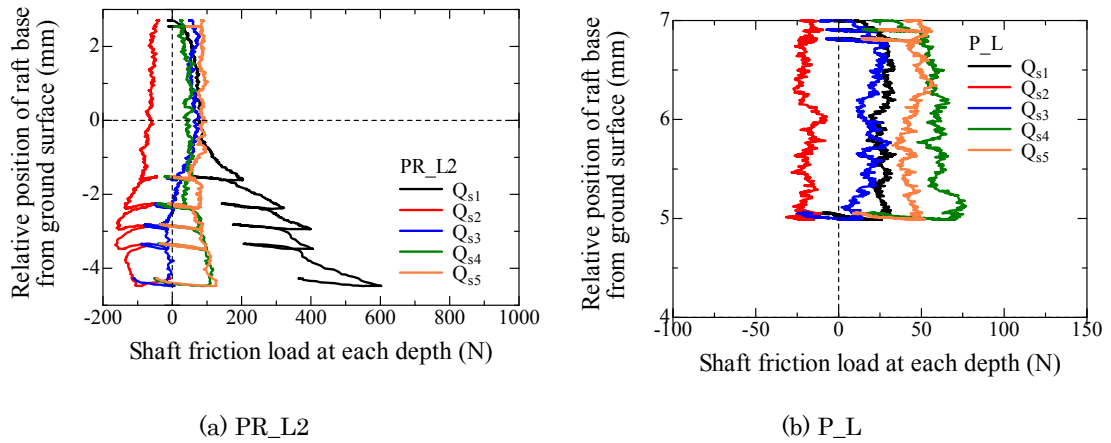
Figure 4.3.3.21 Variation of shaft friction load and shaft friction load increment at each depth with relative position of raft base from ground surface for PR_L2 and P_L during penetration process.
