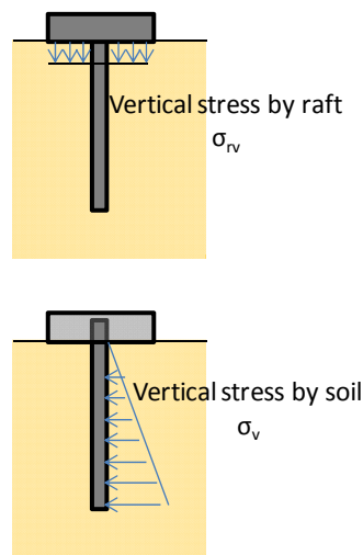
Figure 4.3.3.6 Vertical stress caused by the soil weight and base contact pressure.
