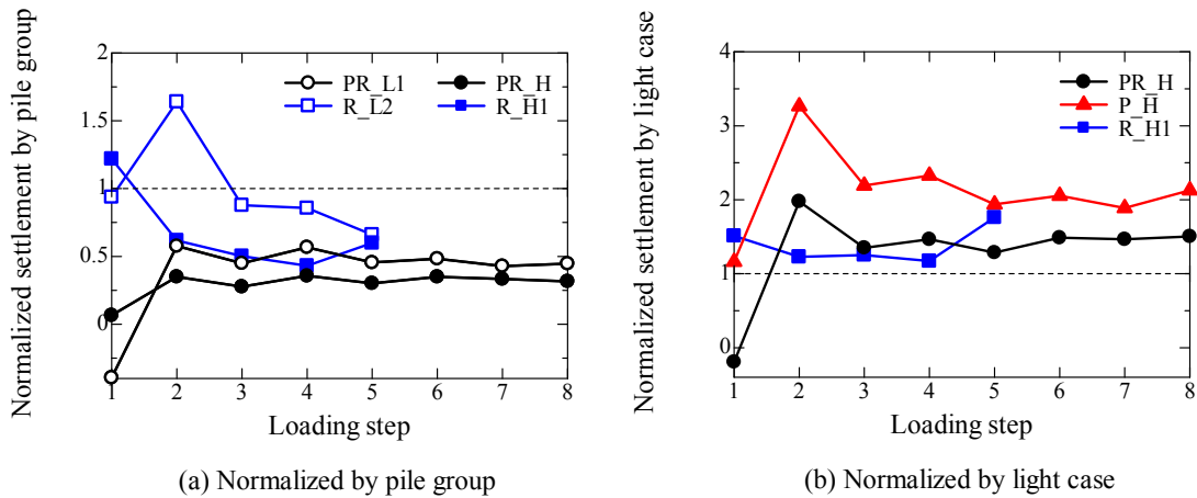
Figure 5.3.1.5 Normalized settlement in each loading step.
