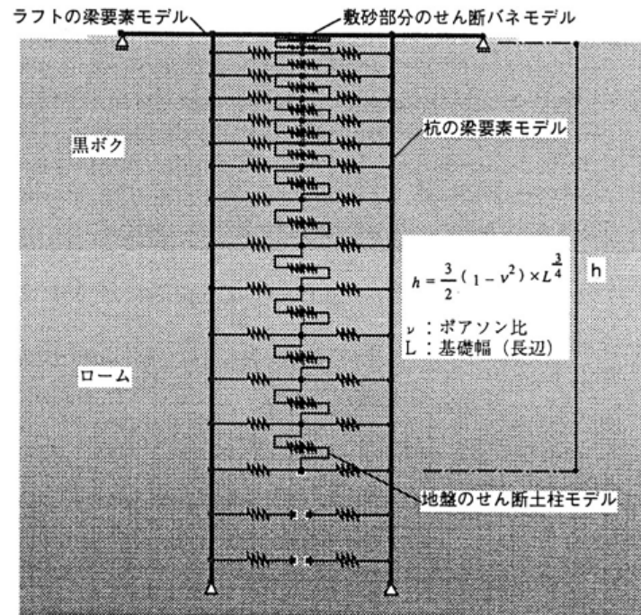
Figure 2.3.18 Concept of the simple model proposed by Nagano et al. (2004)
