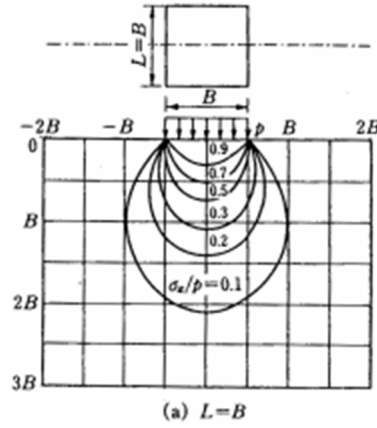
Figure 4.3.3.7 Stress bulb beneath 3D footing.
