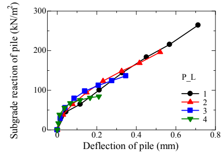
(b) Pull-out pile ( \delta_{LDI} = \pm 1 \text{ mm} , h/S=1 )
