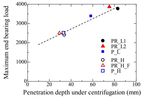
Figure 4.2.1.5 Relationship between penetration depth in the flight and maximum end bearing load.
