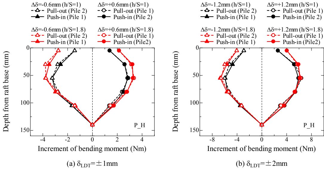
Figure 5.5.2.4 Profile of bending moment for P_H.
