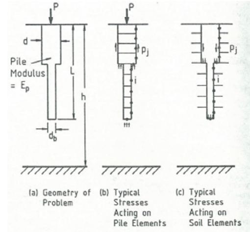
Figure 2.3.1 Boundary element analysis of single pile. (Poulos and Davis (1968))
