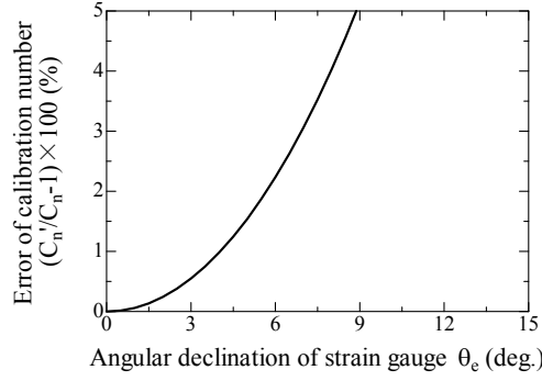
Figure 3.6.6 Error of calibration number caused by angular declination \theta_e .
