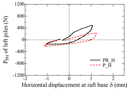
(e) Left piles ( \delta_{LDI} = \pm 2\text{mm} , h/S=1 )
