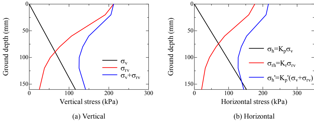
Figure 4.3.3.8 Stress profile in the model ground.
