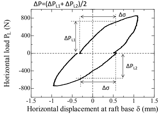
Figure 5.4.1.4 Definition of horizontal load increment \Delta P and horizontal displacement increment \Delta \delta .
