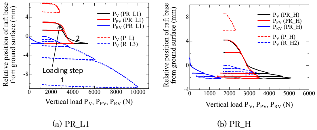
Figure 4.3.1.1 Variation of P_V , P_{PV} and P_{RV} for PR_L1 and PR_H with settlement observed in the vertical loading process. (A. 4.3.2.1 and 4.3.2.2)
