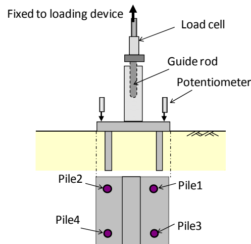
Figure 3.5.7 Schematic illustration of vertical loading tests.
