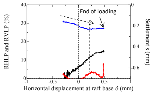
(c) Loading step 3 ( \delta_{LDT} = +1\text{mm} , h/S = 1.8 )
