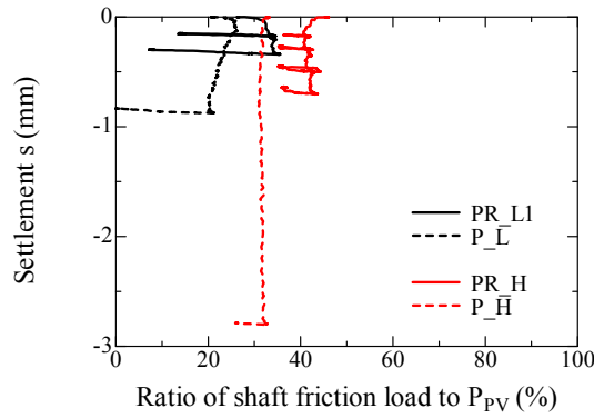
Figure 4.4.2.4 Relationship between ratio of shaft friction load to P_{pv} and settlement s .
