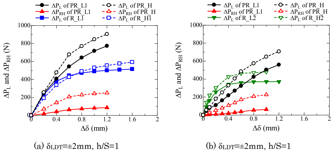
Figure 5.4.2.7 Variation of \Delta P_L and \Delta P_{RH} with \Delta \delta for each loading step. (A. 5.4.2.5)
