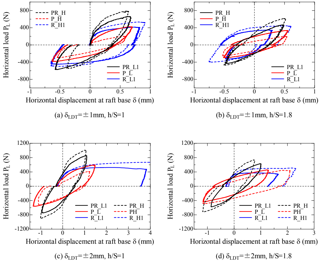
Figure 5.4.1.3 Relationship between horizontal displacement at raft base \delta and horizontal load P_L .
