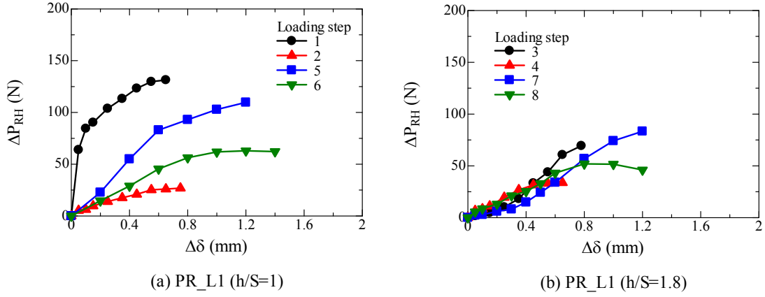
Figure 5.4.2.11 Relationship between \Delta \delta and \Delta P_{RH} for light case observed in each loading step.
