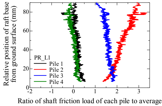
(c) Shaft friction load
