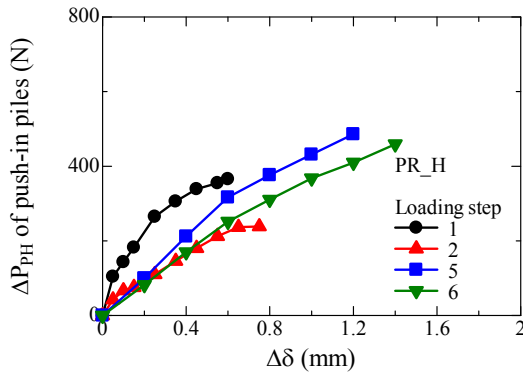
(c) Push-in piles (h/S=1)
