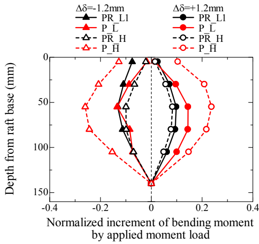
(g) Push-in pile ( \delta_{LDT} = \pm 2\text{mm} , h/S=1.8 )
