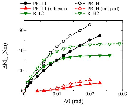
Figure 5.5.3.3 Relationship between \Delta\theta and \Delta M_L of piled raft, raft part in piled raft and raft foundation for \delta_{LDT}=\pm 2\text{mm} , h/S=1.8 . (A. 5.5.3.5)
