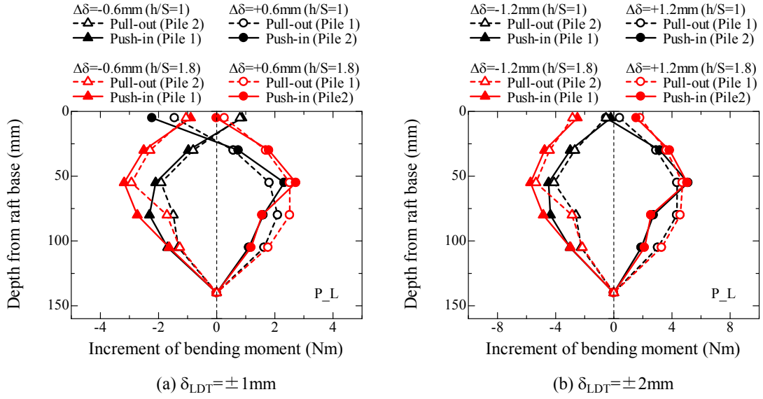
Figure 5.5.2.2 Profile of bending moment for P_L.
