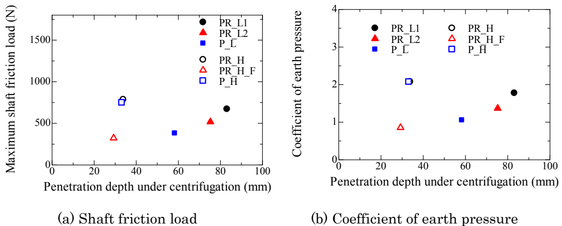
Figure 4.2.1.6 Relationship between penetration depth in the flight and (a) shaft friction load and (b) coefficient of earth pressure during penetration process.
