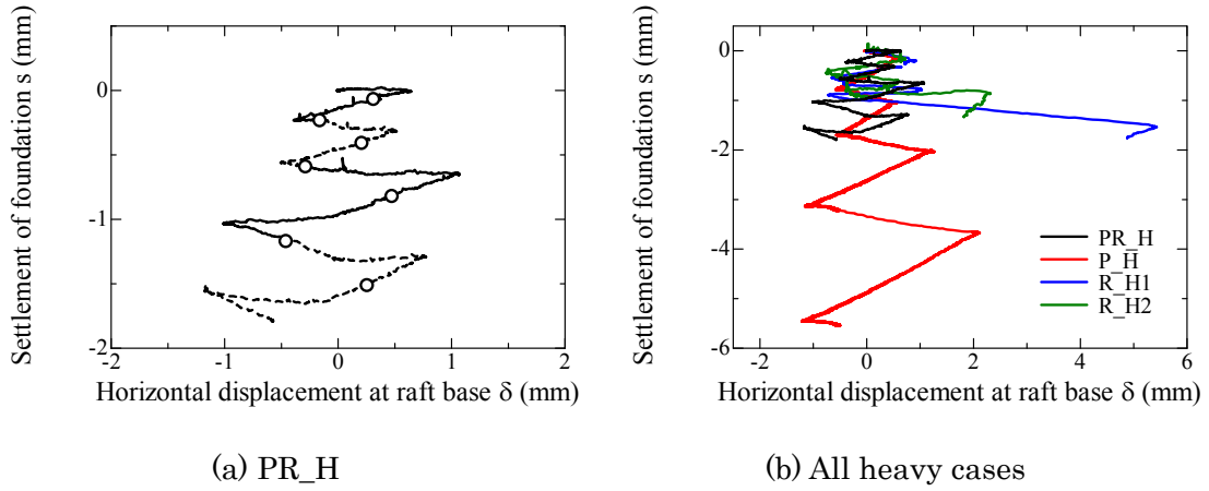
Figure 5.3.1.2 Relationship between horizontal displacement at raft base \delta and settlement s for heavy case. (A.5.3.1.2)
