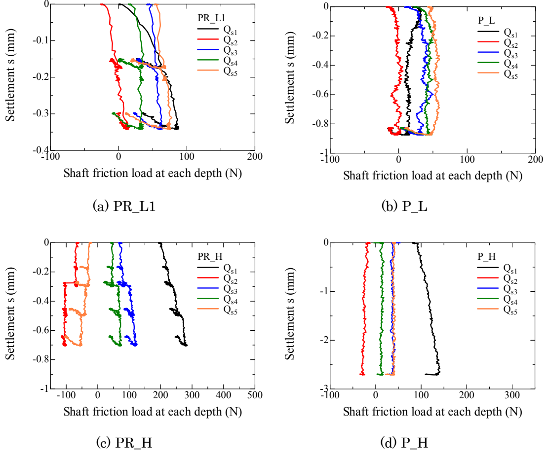
Figure 4.4.2.8 Variation of shaft friction load at each depth with settlement s during pre-vertical loading process. (A. 4.4.2.10-4.4.2.13)
