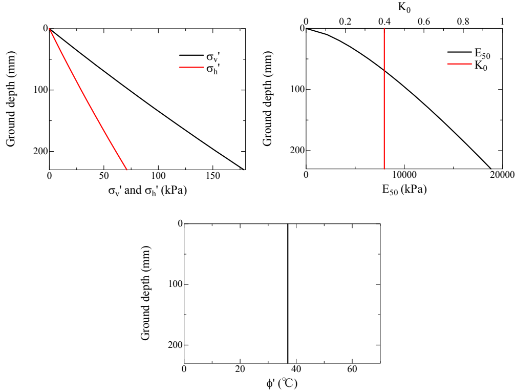
Figure 3.4.17 Variation of (a) stress level, (b) deformation characteristics and (c) strength characteristic with ground depth for present model.
