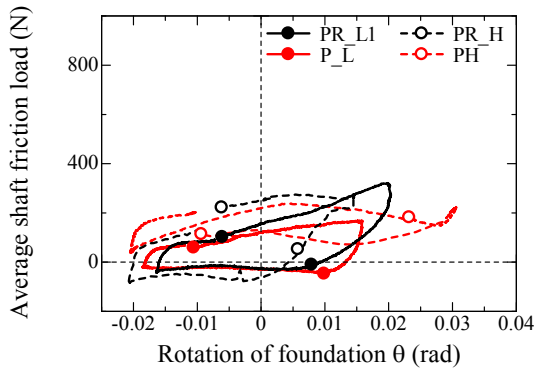
Figure 5.5.2.16 Variation of pile load with rotation of foundation \theta observed in loading step 7 and 8 ( \delta_{LDT}=\pm 2\text{mm} , h/S=1.8 ). (A. 5.5.2.16-5.5.2.19)
