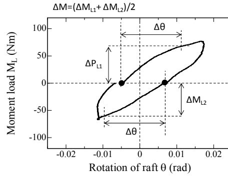
Figure 5.5.1.4 Definition of rotation increment \Delta\theta and moment load increment \Delta M .
