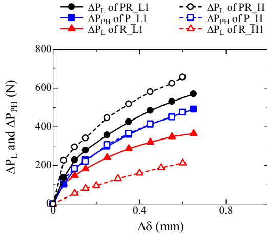
(a) \delta_{LDI} = \pm 1\text{mm} , h/S=1
