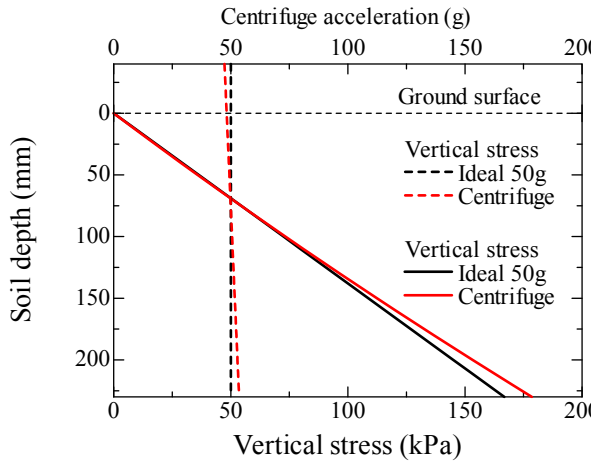
Figure 3.4.2 Distribution of vertical stress in model ground for ideal stress field and centrifuge stress field.
