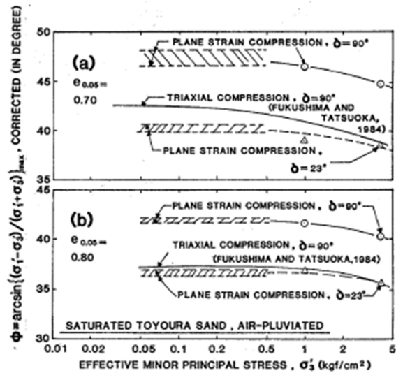
Figure 3.4.16 Relationship between internal friction angle \phi' and \sigma_3' for (a) e=0.7 , (b) e=0.8 . (Tatsuoka et al. (1986))
