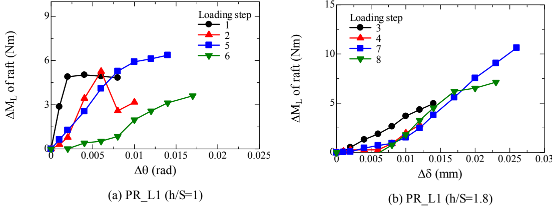
Figure 5.5.3.6 Relationship between \Delta \theta and \Delta M of raft part for light case observed in each loading step.
