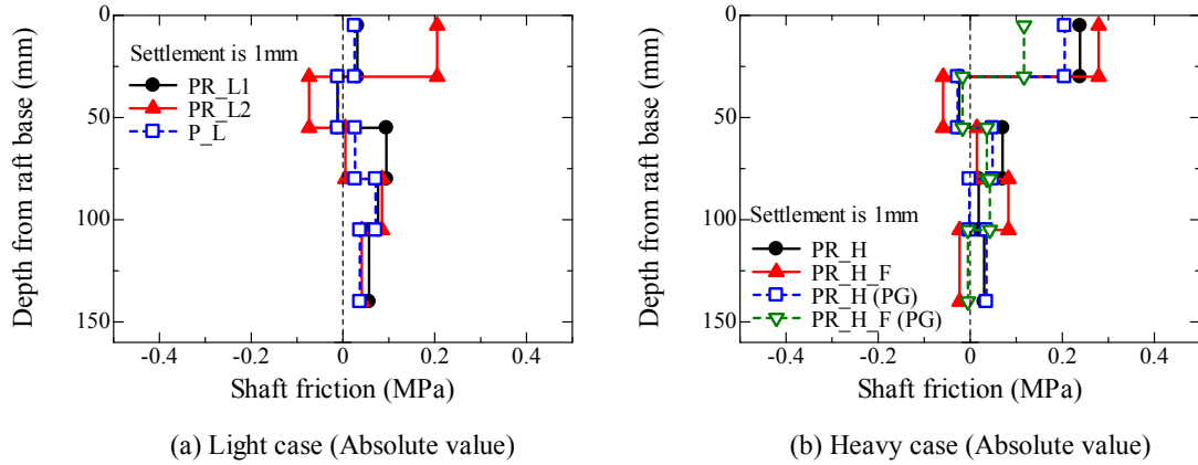
Figure 4.3.3.23 Profile of shaft friction at settlement of 1mm for (a) light case, (b) heavy case. (A. 4.3.3.22)
