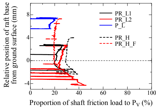
Figure 4.3.3.2 Relationship between proportion of shaft friction load to total vertical load P_V and relative position of raft base from ground surface during vertical loading process.
