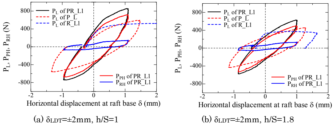
Figure 5.4.2.1 Variation of horizontal load P_L and horizontal load carried by raft P_{RH} and piles P_{PH} with horizontal displacement at raft base \delta for light case. (A. 5.4.2.1)
