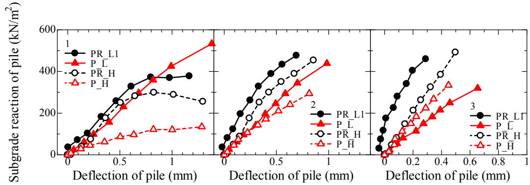
(a) Push-in ( \delta_{LDI}=\pm 2\text{mm} , h/S=1 )
