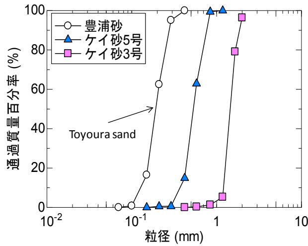
Figure 3.4.12 Cumulative frequency curve for Toyoura sand.
