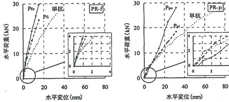
Figure 2.3.42 Relationship between horizontal displacement and horizontal resistance of pile. (Nagai and Tsuchiya (2004))
