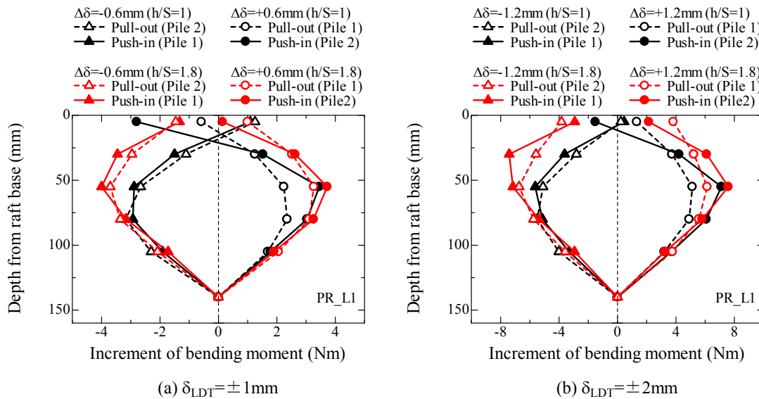
Figure 5.5.2.1 Profile of bending moment for PR_L1.
