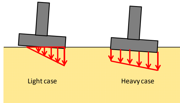
Figure 5.4.3.15 Predicted base contact pressure distribution for piled raft.
