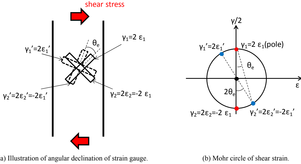
Figure 3.6.11 Measurement error of shear strain gauge caused by angular declination.
