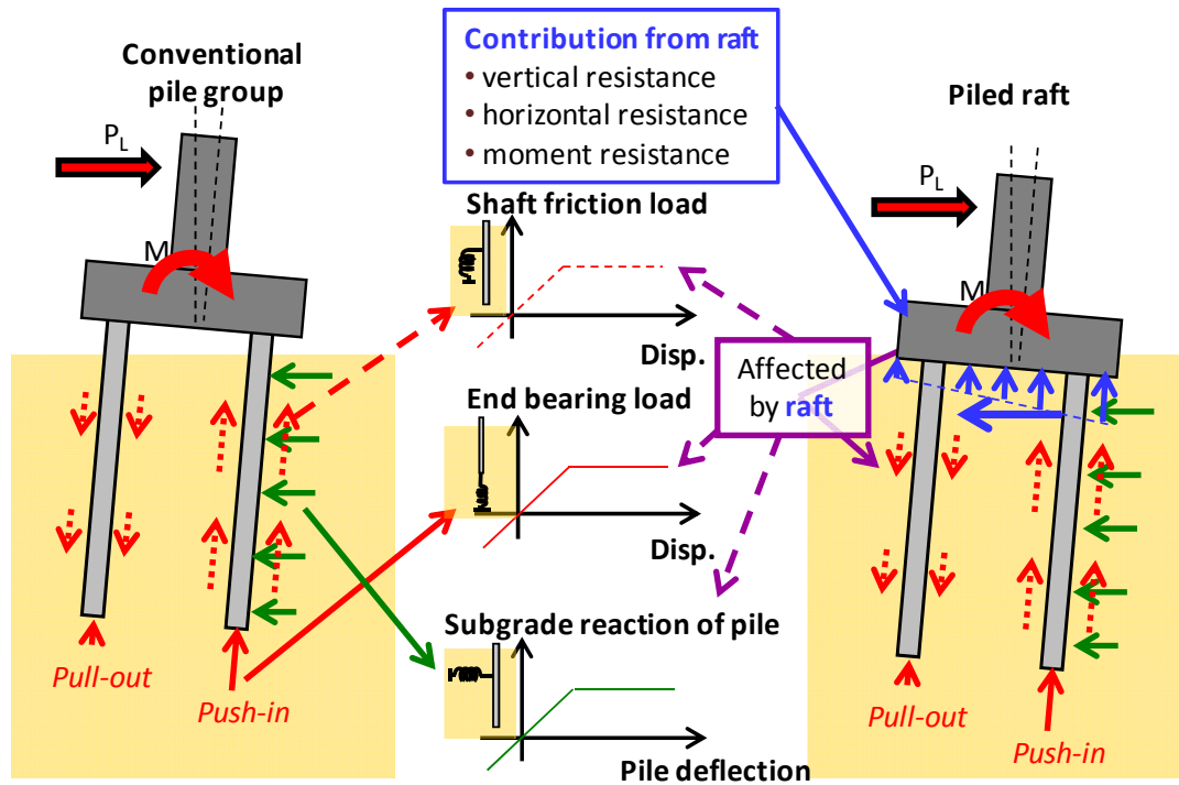
Figure 1.1.2 Complicated behavior of the piled raft subjected to horizontal and moment loads
