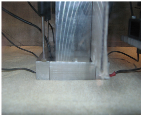
Figure 3.5.8 Model foundation before horizontal loading tests.
