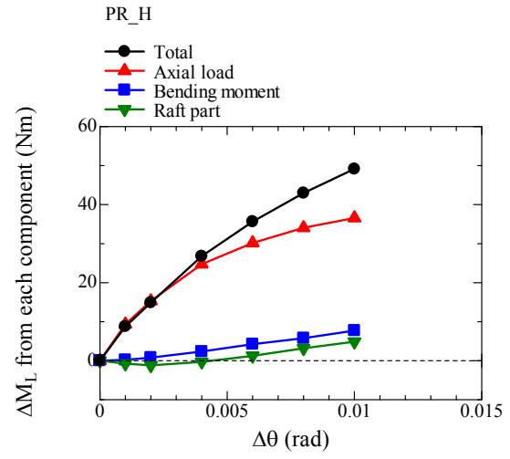
(b) \delta_{LDT} = \pm 1\text{mm} , h/S=1.8
