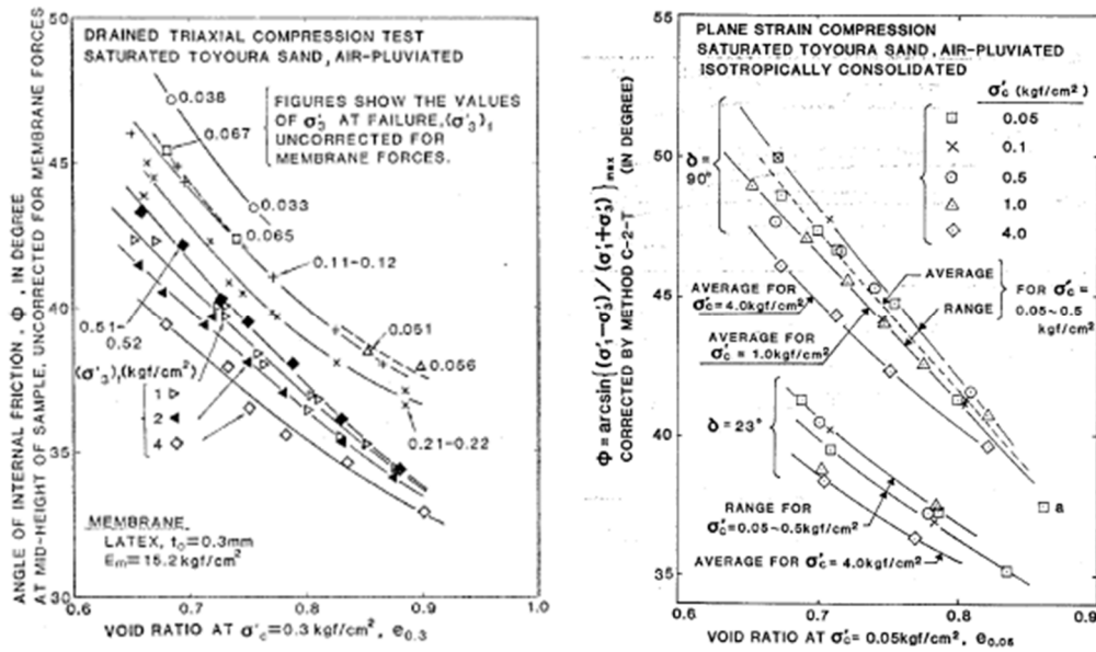
Figure 3.4.15 Relationship between internal friction angle \phi' and void ratio for (a) triaxial compression tests at \sigma_3' of 30kPa (Fukushima and Tatsuoka (1984)), (b) plane strain compression tests at \sigma_3' of 5kPa (Tatsuoka et al. (1986)).
