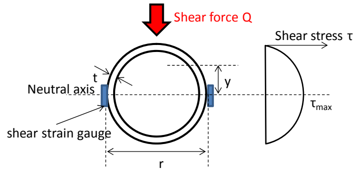
Figure 3.6.10 Distribution of shear stress on pile.
