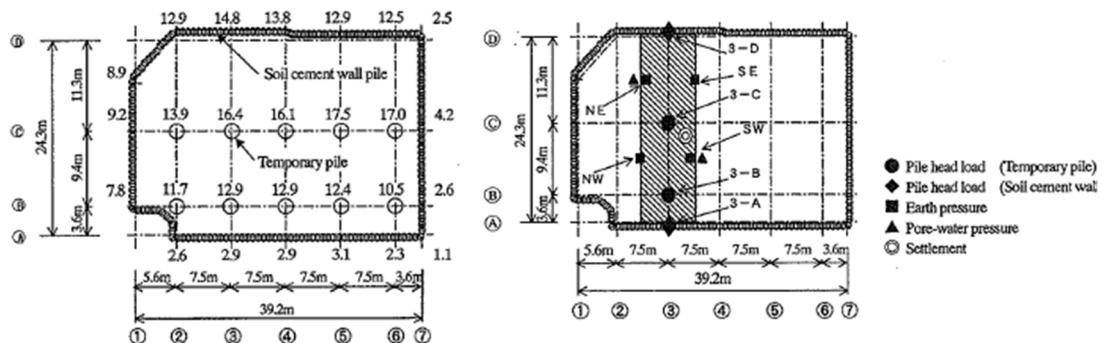
Figure 2.3.23 Foundation plan and monitoring position. (Yamada et al. (2001))
