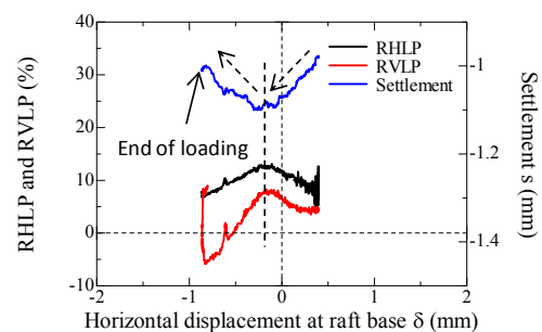
(h) Loading step 8 ( \delta_{LDT} = -2\text{mm} , h/S = 1.8 )
