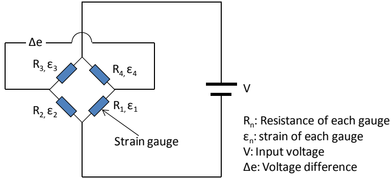
Figure 3.6.1 Bridge circuit for strain gauge.
