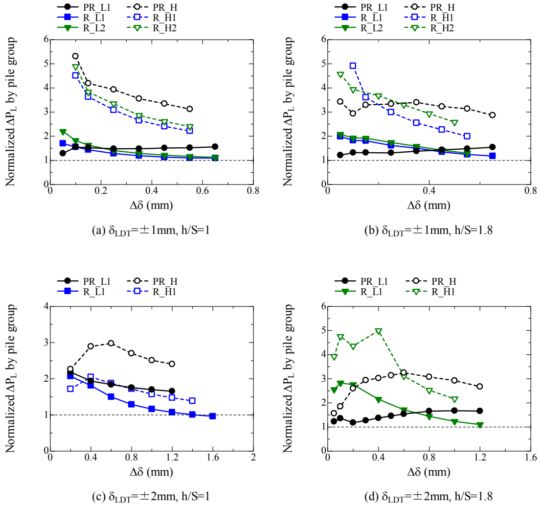
A. 5.4.1.2 Relationship between \Delta\delta and normalized \Delta P_L by that of pile group for each loading step.
