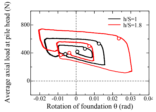
(b) Axial load at pile head (Right pile)
