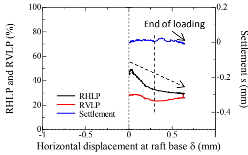
(a) Loading step 1 ( \delta_{LDT}=+1\text{mm} , h/S=1 )
