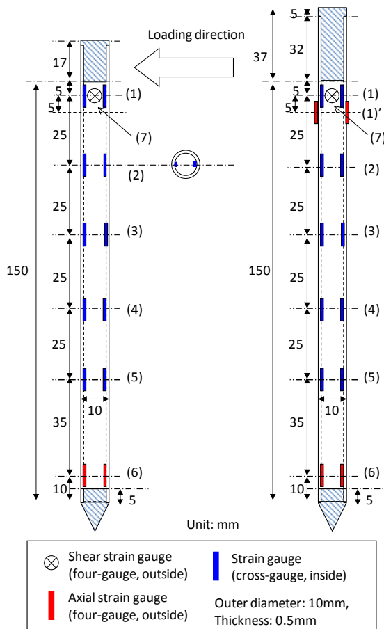
Figure 3.4.8 Model piles for light and heavy cases.
