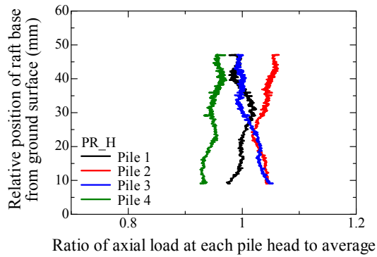
(a) Axial load at pile head
