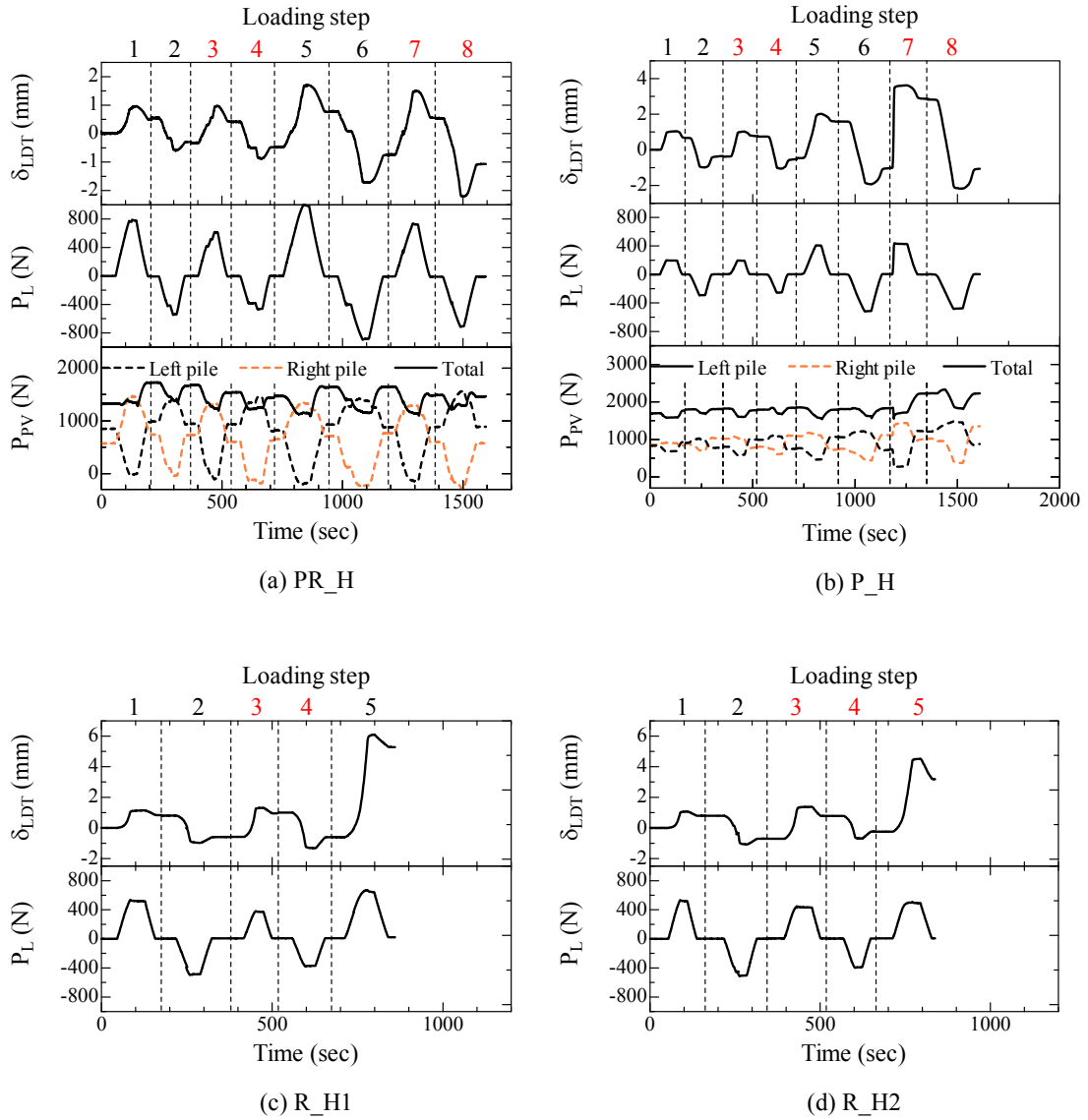
Figure 5.2.2 Applied horizontal displacement at lower LDT \delta_{LDT} , applied horizontal load P_L and measured axial load at pile head P_{PV} for heavy case.
