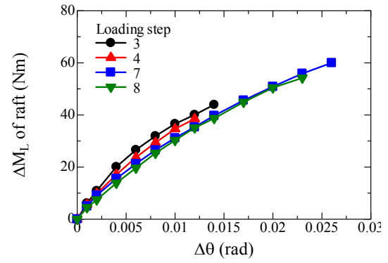
(a2) PR_L1 (h/S=1.8)
