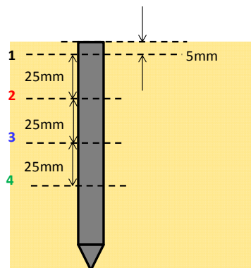
Figure 5.4.3.5 Depth at which horizontal subgrade reaction of pile was estimated.
