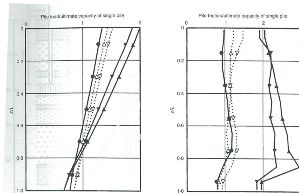
Figure 2.3.14 Distribution of pile load and skin friction. (Poulos (2001))
