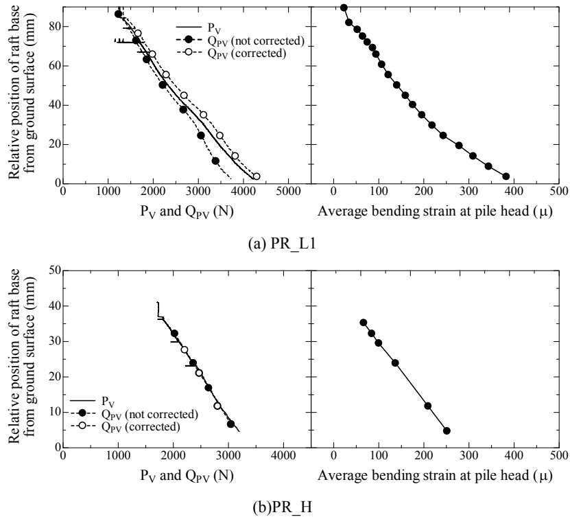
Figure 3.6.15 Variation of PV, QPV and bending strain at pile head with settlement for PR_L1 and P_H during penetration process.
