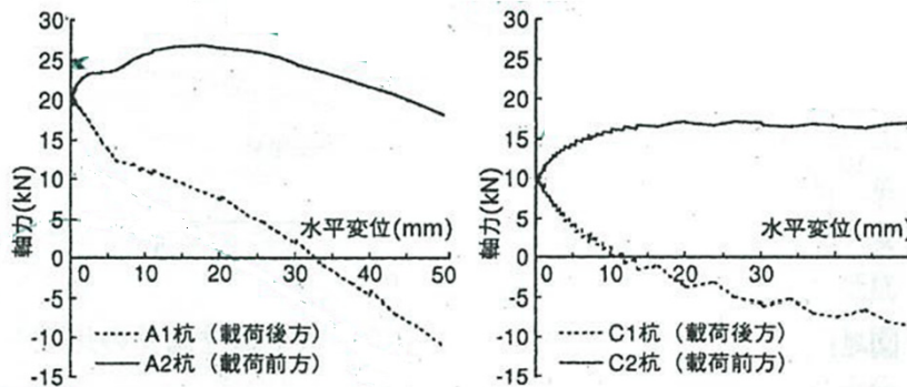
Figure 2.3.31 Relationship between horizontal displacement and axial load at pile head. (Nagano et al. (2002))
