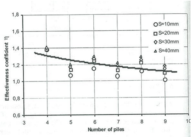
Figure 2.3.16 Effective coefficient \eta of piled raft foundation. (Tejchman et al.(2005))
