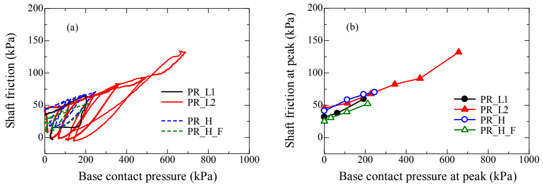
Figure 4.3.3.5 Relationship between base contact pressure and shaft friction during vertical loading process.
