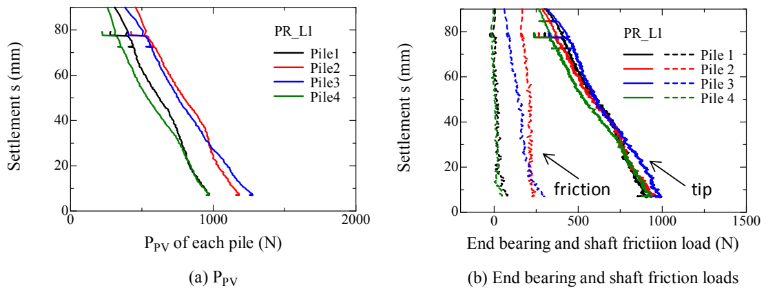
Figure 4.2.2.1 Relationship between pile load acting on each pile and settlement for PR_L1 observed in penetration process.
