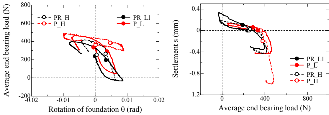
(e) End bearing load (Right pile)
