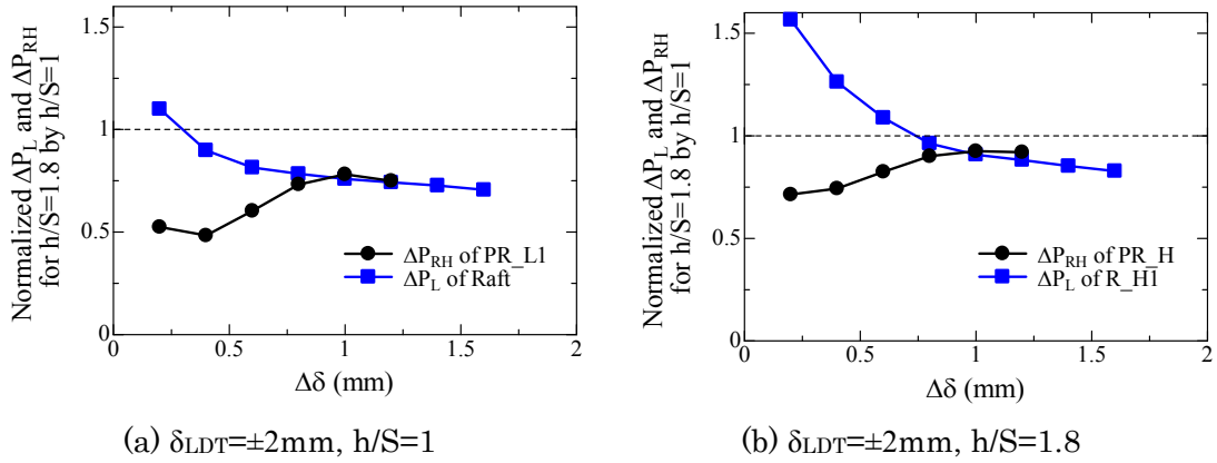
Figure 5.4.2.10 Variation of normalized \Delta P_L and \Delta P_{RH} of heavy case by those of light case with \Delta\delta . (A. 5.4.2.7)
