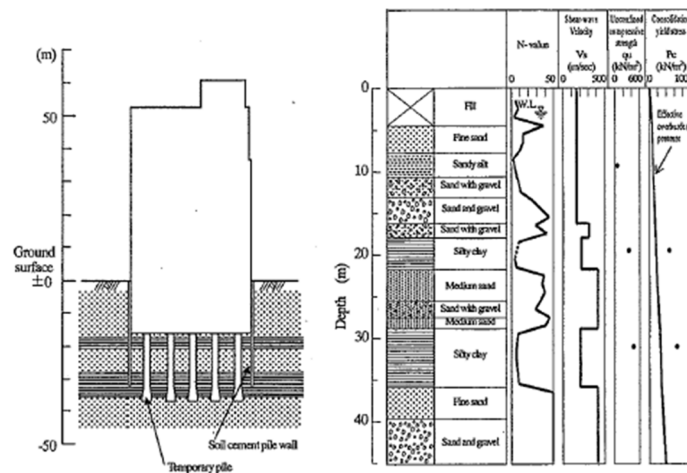
Figure 2.3.22 Schematic illustration of building and soil profile. (Yamashita et al. (2001))
