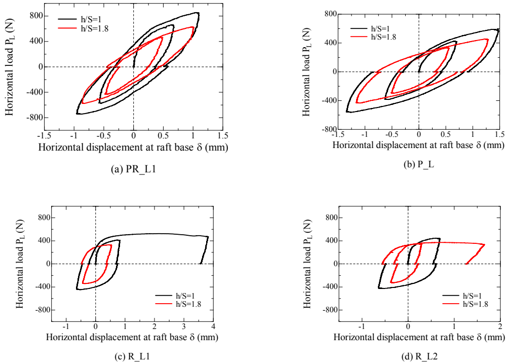
Figure 5.5.1.1 Relationship between horizontal displacement at raft base \delta and horizontal load P_L for light case.
