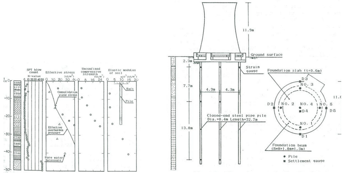
Figure 2.3.3 Schematic illustration of foundation and soil profile. (Kakurai et al. (1987))
