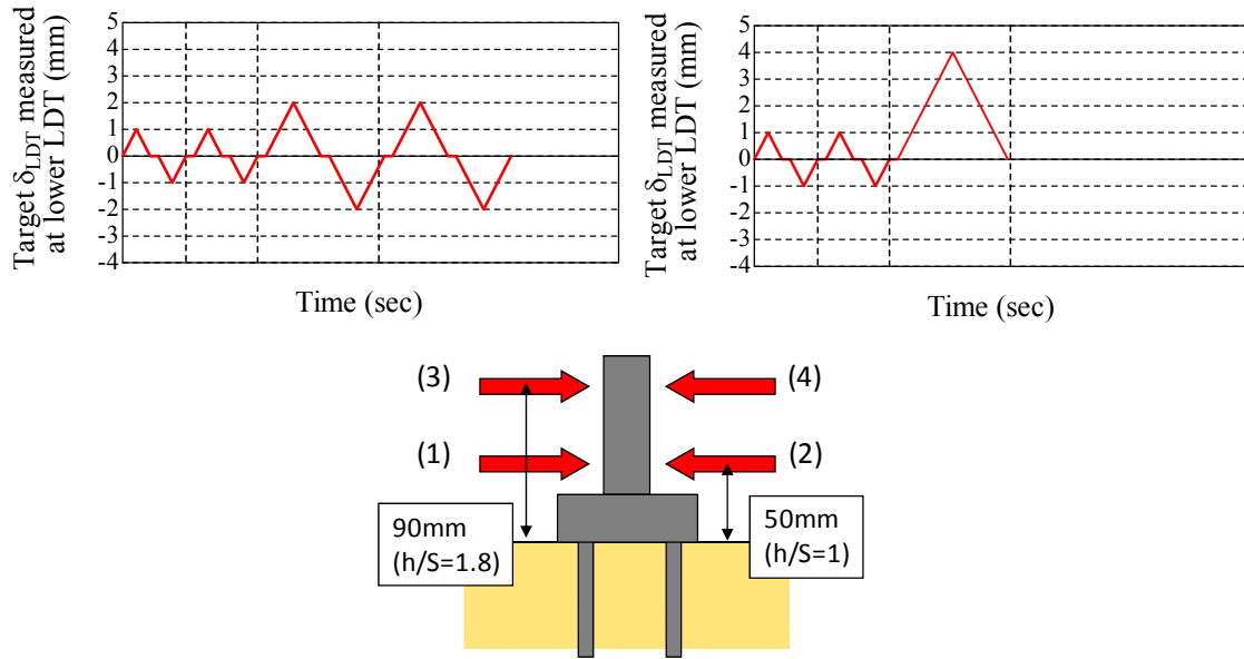
Figure 3.5.11 Applied horizontal displacement at lower LDT, \delta_{LDT} , during horizontal loading tests.
