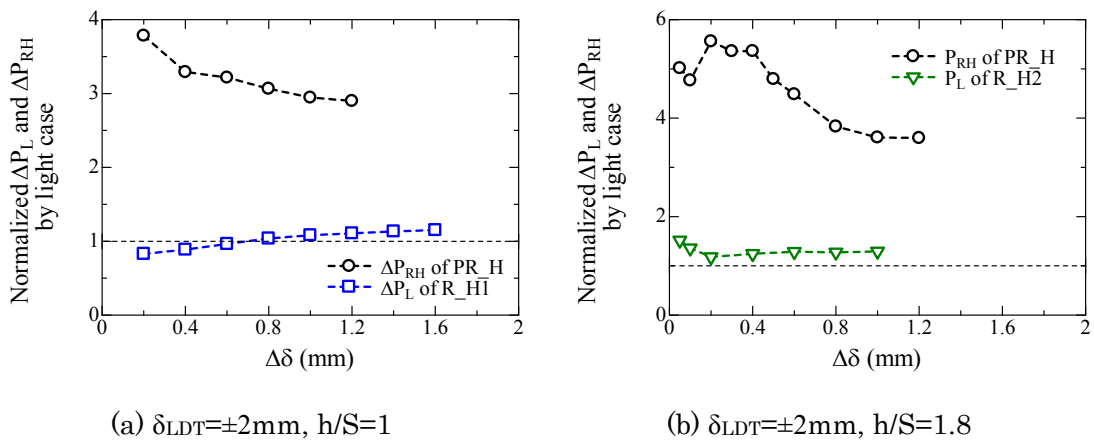
Figure 5.4.2.9 Variation of normalized \Delta P_L and \Delta P_{RH} of heavy case by those of light case with \Delta\delta . (A. 5.4.2.6)
