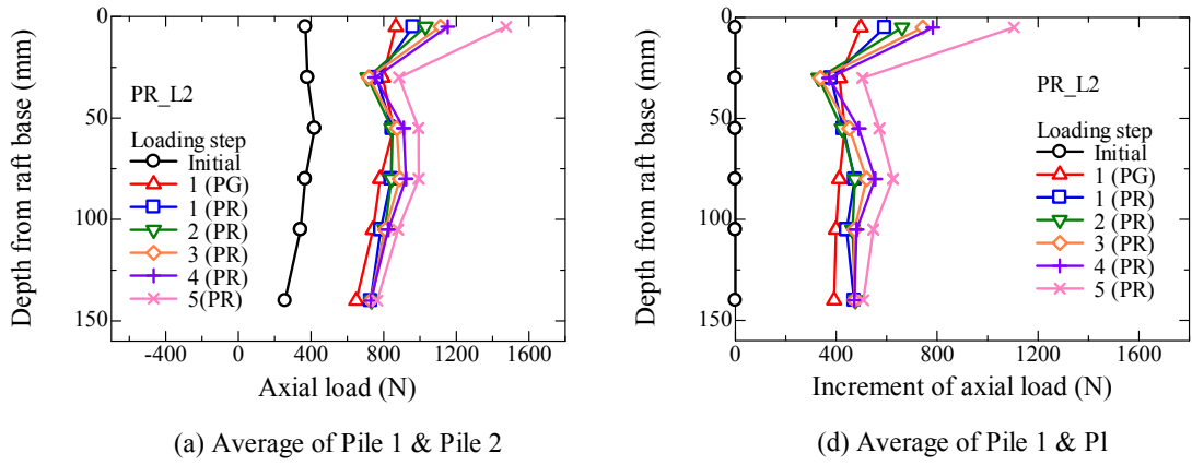
Figure 4.3.3.13 Profiles of axial load and axial load increment for PR_L2 during vertical loading process.
