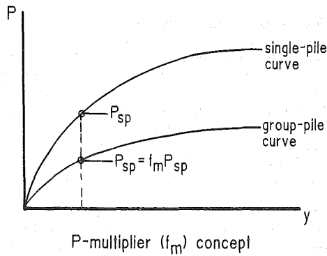
Figure 2.2.2 p-multiplier concept. (Brown et al. (1988))
