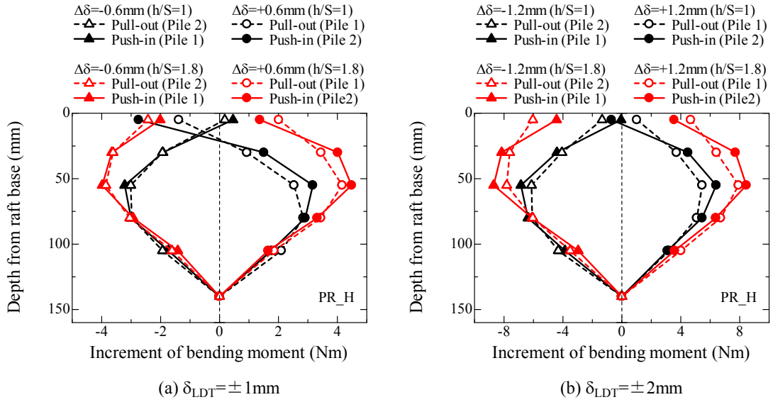
Figure 5.5.2.3 Profile of bending moment for PR_H.
