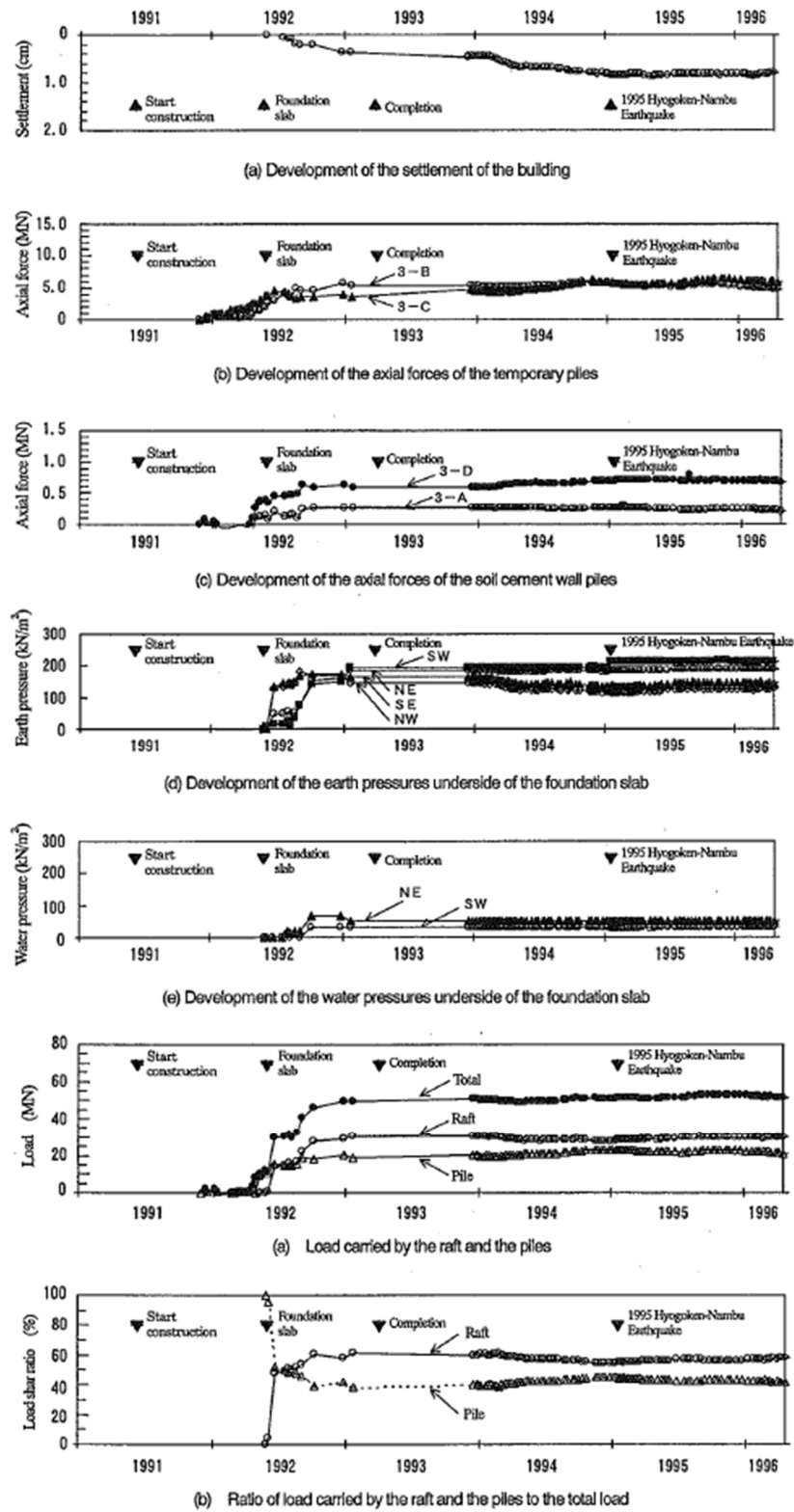
Figure 2.3.24 Measured results. (Yamashita et al. (2001))
