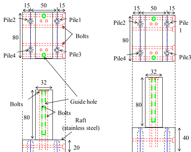
Figure 3.4.4 Model raft and superstructure.
