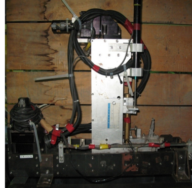
Figure 3.4.19 Two-ways actuator.
