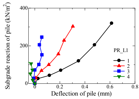
(c) Push-in pile ( \delta_{LDI} = \pm 1 \text{ mm} , h/S=1.8 )
