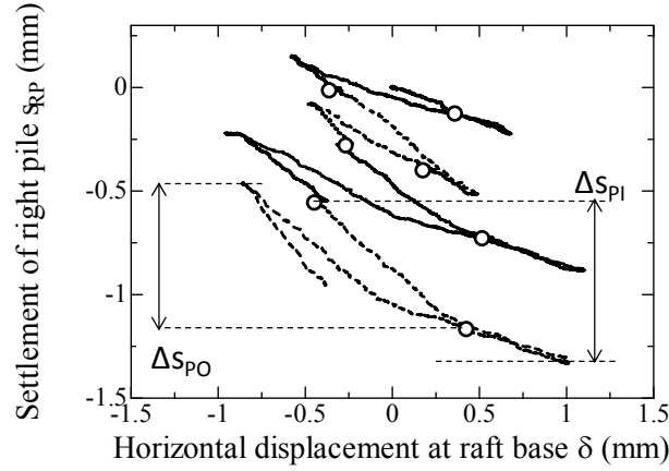
Figure 5.3.2.3 Definition of \Delta s_{PI} and \Delta s_{PO} .
