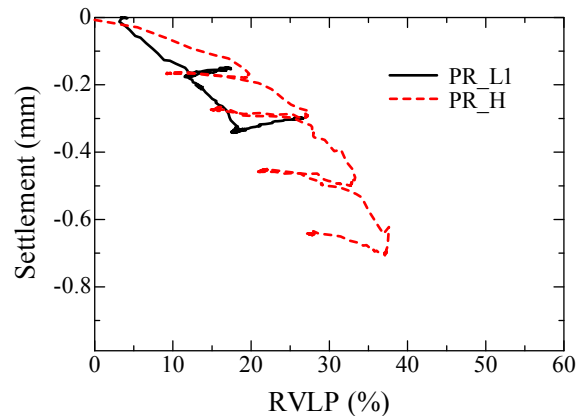
Model 3.5.9 Relationship between RVLP – settlement for PR_L1 and PR_H during pre-vertical loading process.
