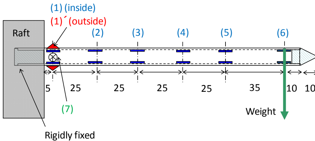
Figure 3.6.2 Calibration method of model pile.
