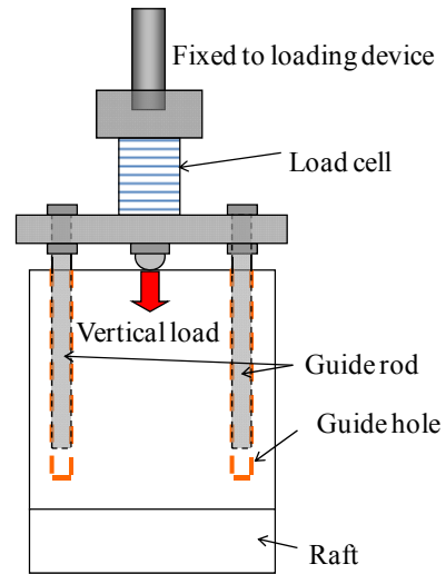
Figure 3.4.7 Guide rod and guide holes.
