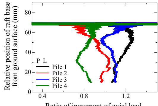
(a) Axial load at pile head
