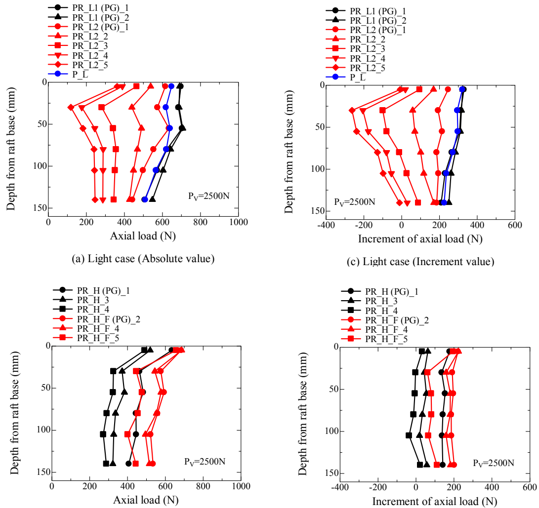
Figure 4.3.3.19 Profile of axial load at P_v of 2500N.
