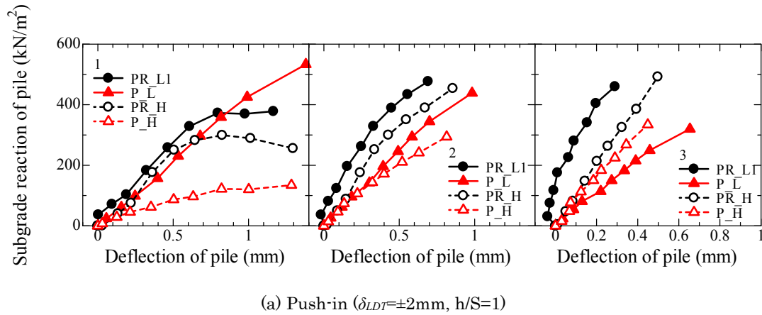
Figure 5.4.3.10 Relationship between pile deflection and horizontal subgrade reaction of push-in pile at depth of 1, 2 and 3. (A. 5.4.3.7)
