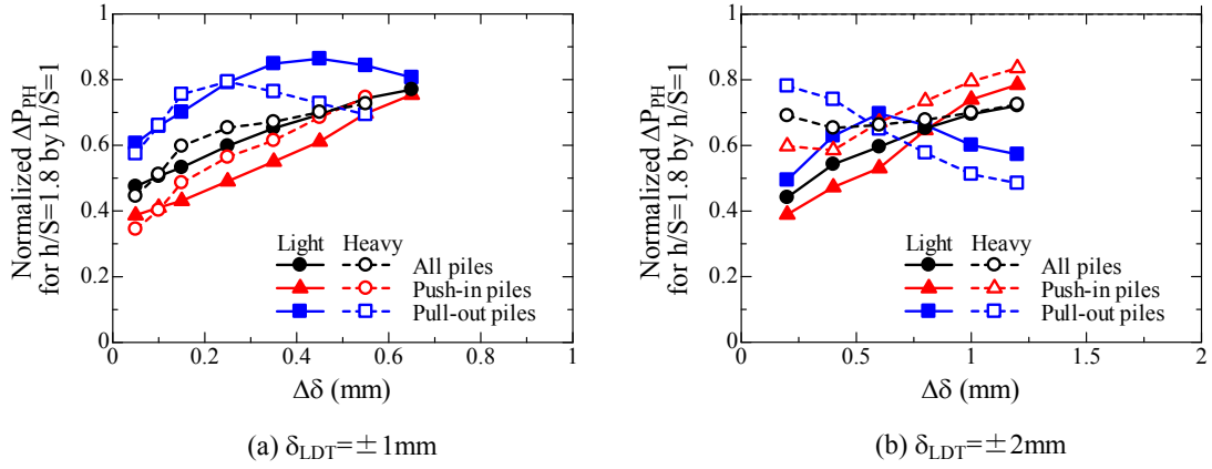
Figure 5.4.3.17 Relationship between \Delta\delta and normalized \Delta P_{PH} for h/S=1.8 by that for h/S=1 .
