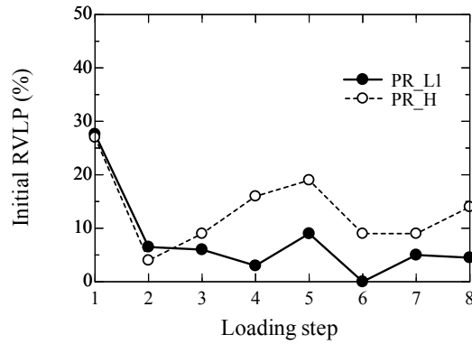
Figure 5.2.3 Initial RVLP for each loading step at each loading step.
