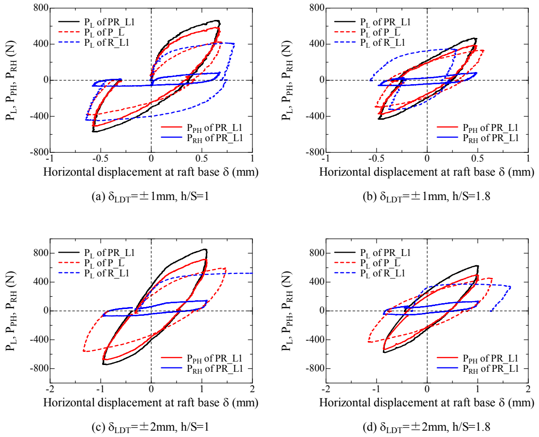
A. 5.4.2.1 Variation of horizontal load P_L and horizontal load carried by raft P_{RH} and piles P_{PH} with horizontal displacement at raft base \delta for light case.
