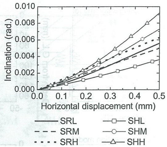
Figure 2.3.40 Horizontal displacement - inclination relationship (Matsumoto et al. (2004a))
