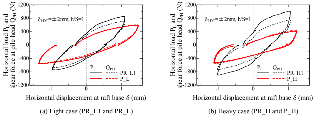
Figure 3.6.17 Variation of P_L and Q_{PH} with \delta for \delta_{LDT}=\pm 2\text{mm} , h/S=1 .
