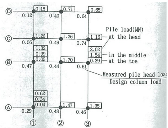
Figure 2.3.9 Measured pile loads at the time of completion. (Yamashita et al. (1994))
