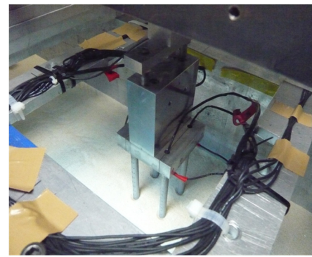
Figure 3.5.2 Model foundation fixed to actuator using guide rods for (a) piled raft and pile group, (b)raft.
