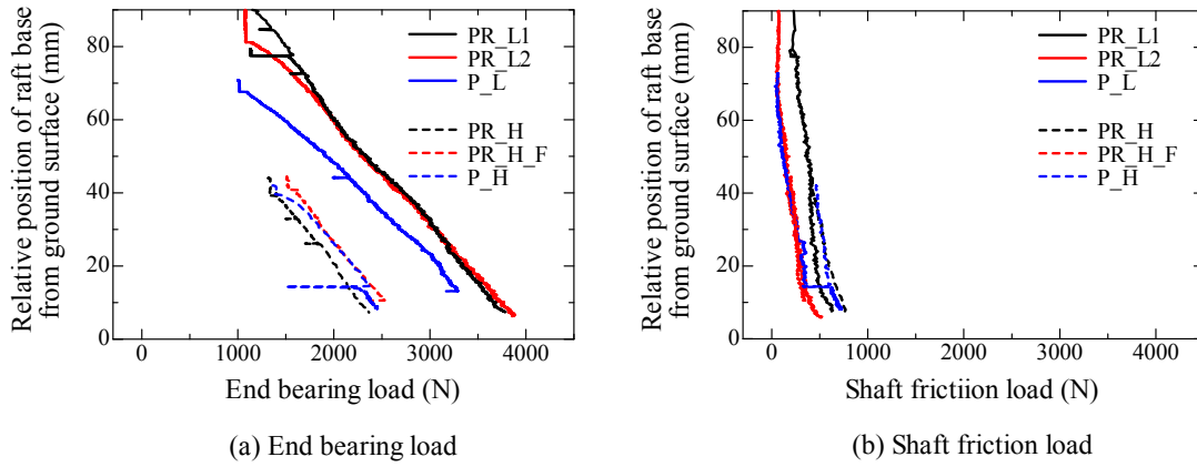
Figure 4.2.1.3 Relationship between pile force and relative position of raft base from ground surface during penetration process for all cases.
