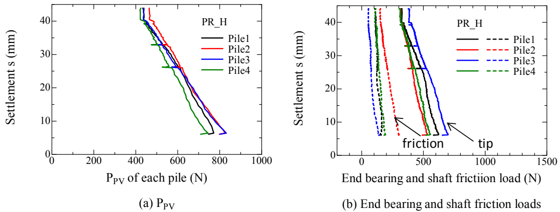
Figure 4.2.2.2 Relationship between pile load acting on each pile and settlement for PR_H observed in penetration process. (A. 4.2.2.1-4.2.2.12)
