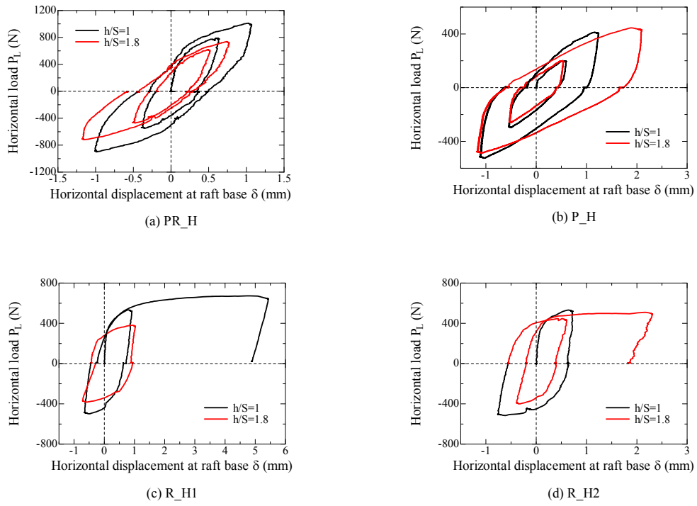
Figure 5.5.1.2 Relationship between horizontal displacement at raft base \delta and horizontal load P_L for heavy case.
