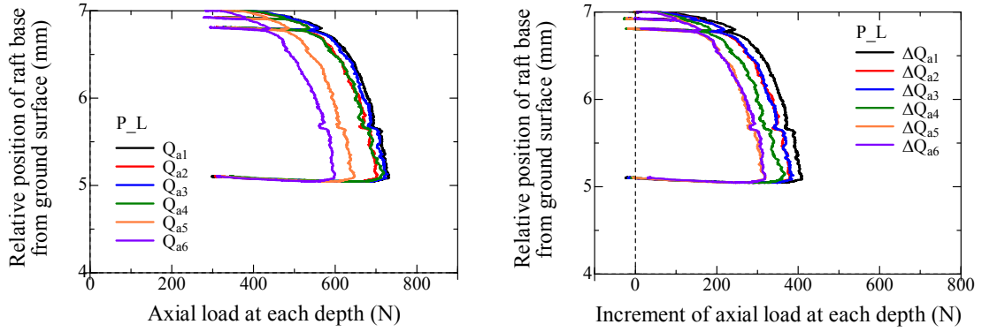
Figure 4.3.3.11 Variation of axial load and axial load increment at each depth with relative position of raft base from ground surface for P_L during penetration process.
