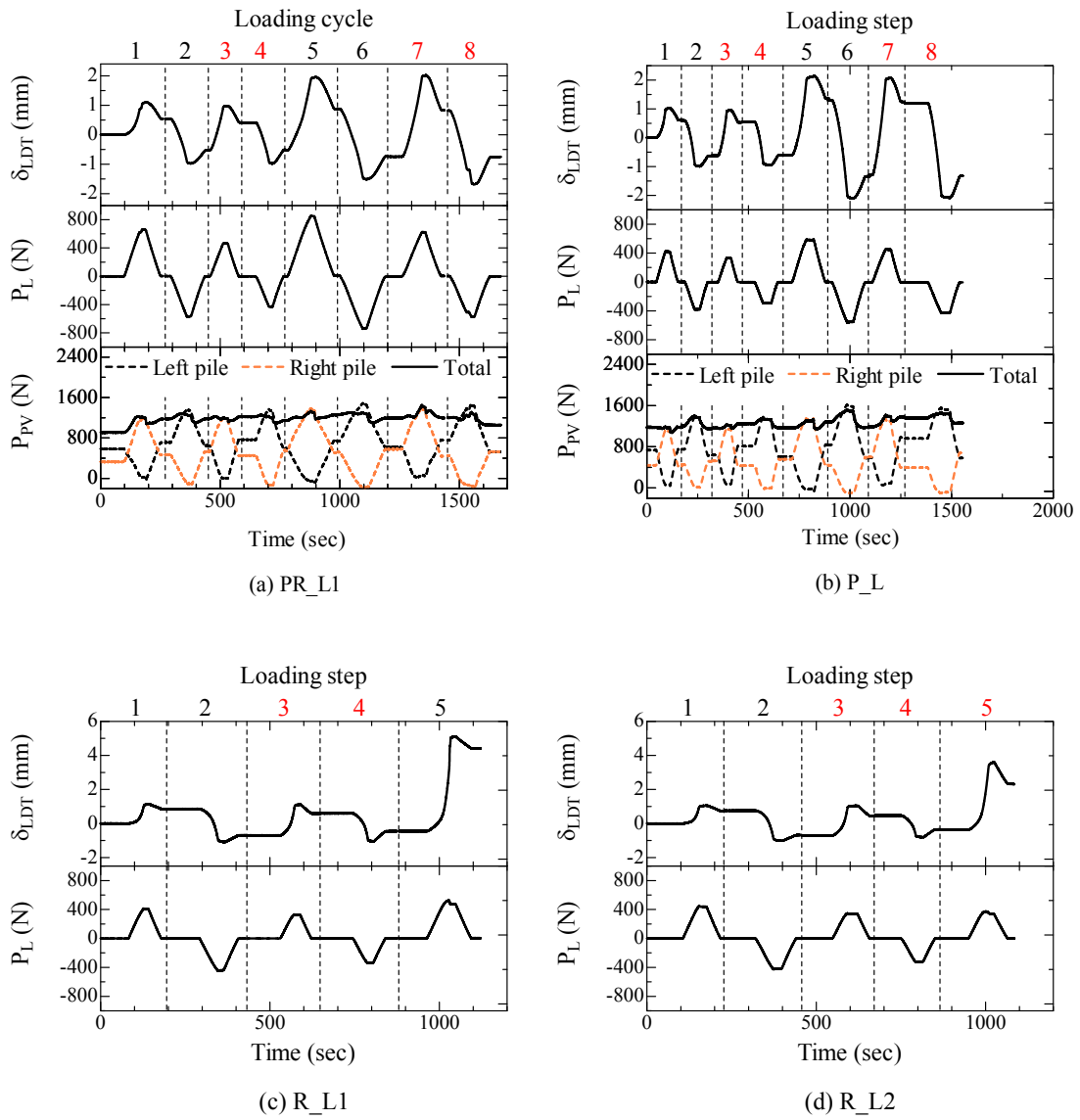
Figure 5.2.1 Applied horizontal displacement at lower LDT \delta_{LDT} , applied horizontal load P_L and measured axial load at pile head P_{PV} for light case.
