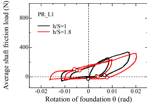
(c) Shaft friction load (left pile)
