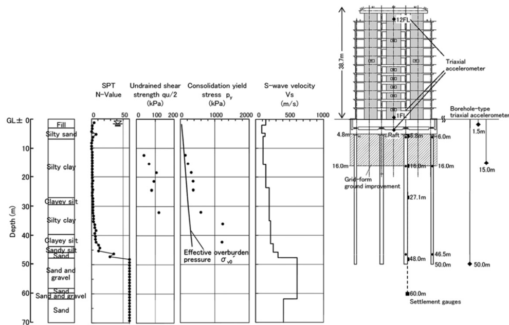
Figure 2.3.25 Schematic view of building and soil profile. (Yamashita et al. (2012))
