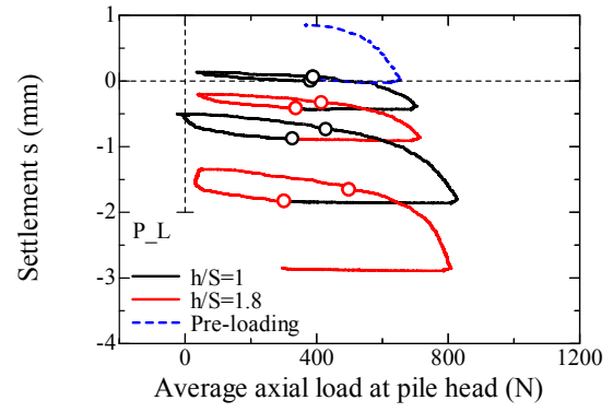
(b) Axial load at pile head (Right pile)
