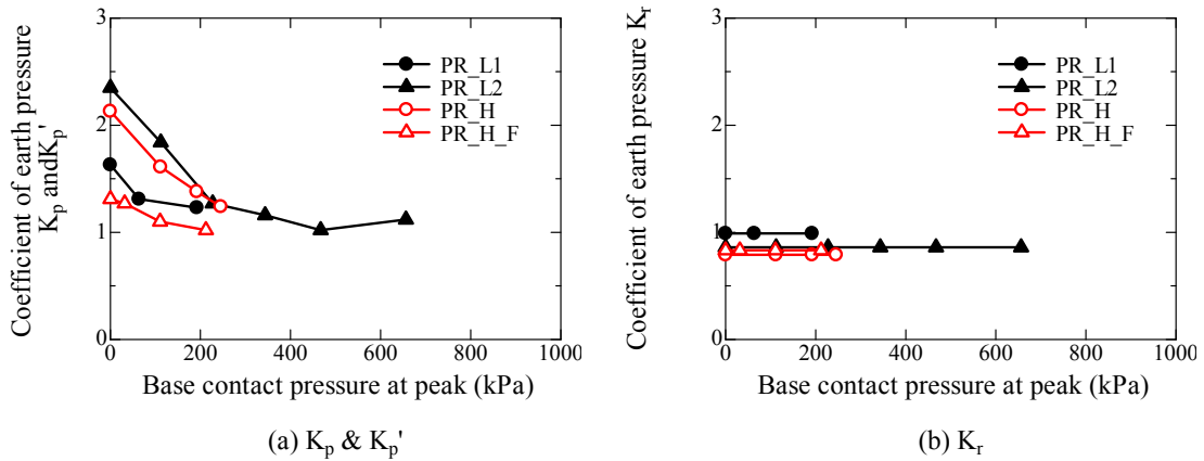
Figure 4.3.3.9 Coefficient of earth pressure back-calculated from the soil weight and raft pressure.
