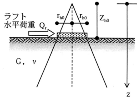
Figure 2.3.17 Concept of the cone model. (Ishii et al. (2003))
