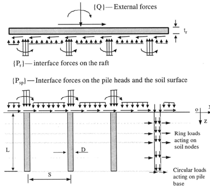
Figure 2.3.21 Finite layer method. (Small and Zhang (2002))
