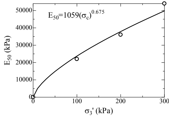
Figure 3.4.13 Relationship between confining stress \sigma_3' and Young's modulus E_{50} for Toyoura sand with relative density of 50% (Kaku (1996))
