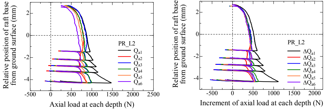
Figure 4.3.3.10 Variation of axial load and axial load increment at each depth with relative position of raft base from ground surface for PR_L2 during penetration process.
