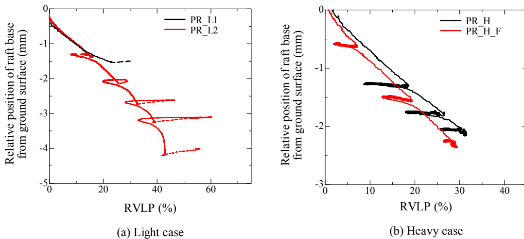
Figure 4.3.2.2 Variation of RVLP with relative position of raft base from ground surface observed in vertical loading process.
