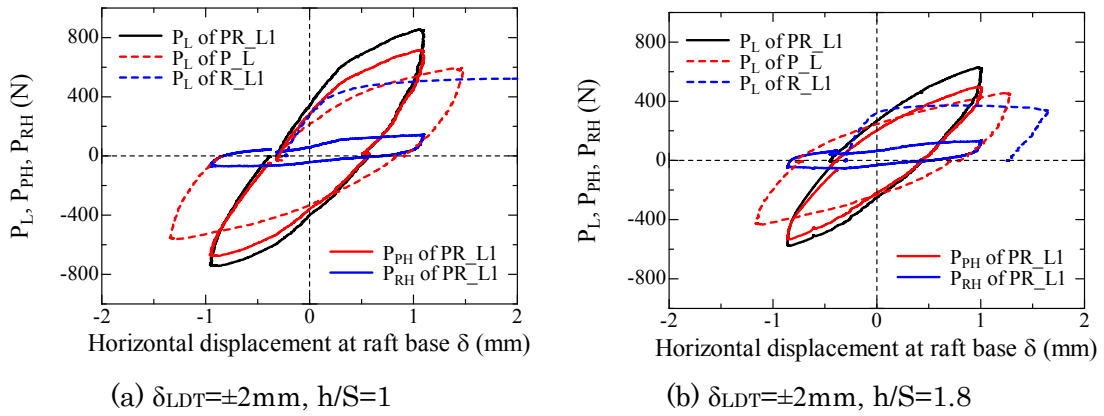
Figure 5.4.3.1 Variation of horizontal load P_L and horizontal load carried by raft P_{RH} and piles P_{PH} with horizontal displacement at raft base \delta for light case. (A. 5.4.2.1)
