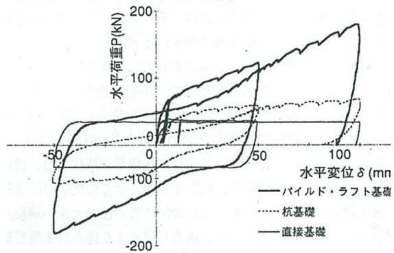
Figure 2.3.30 Relationship between horizontal displacement and horizontal load (Nagano et al. (2002))
