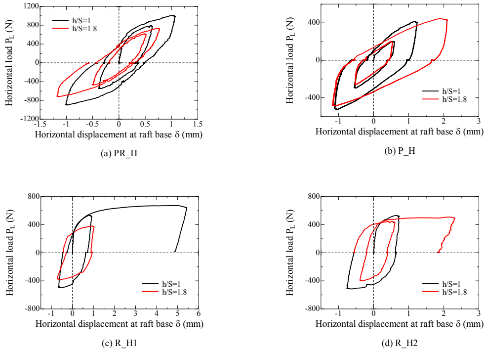
Figure 5.4.1.2 Relationship between horizontal displacement at raft base \delta and horizontal load P_L for heavy case.
