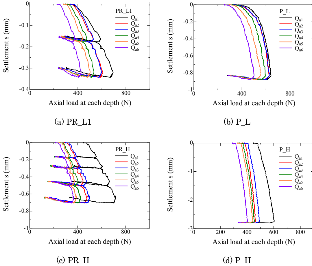
Figure 4.4.2.6 Variation of axial load at each depth Q_{an} with settlement s during pre-vertical loading process. (A. 4.4.2.2-4.4.2.5)
