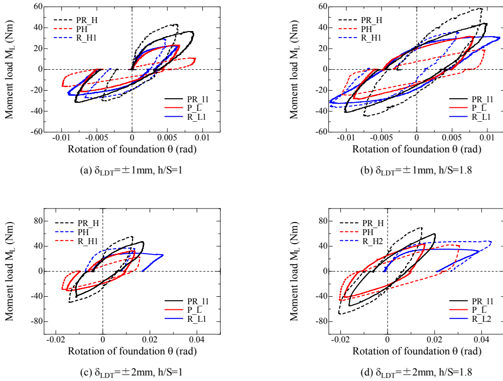
Figure 5.5.1.3 Relationship between rotation of foundation \theta and moment load M_L for each loading step.
