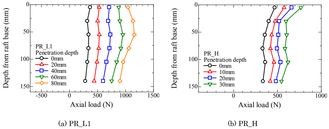
Figure 4.2.1.9 Profiles of axial load for PR_L1 and PR_H during penetration process.
