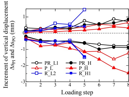
Figure 5.3.2.4 Increment vertical displacements \Delta s_{PI} and \Delta s_{PO} observed in each loading step.
