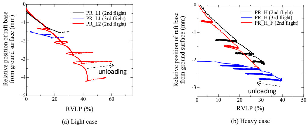
Figure 4.4.2.2 Variation of RVLP with settlement observed in pre-vertical loading process.
