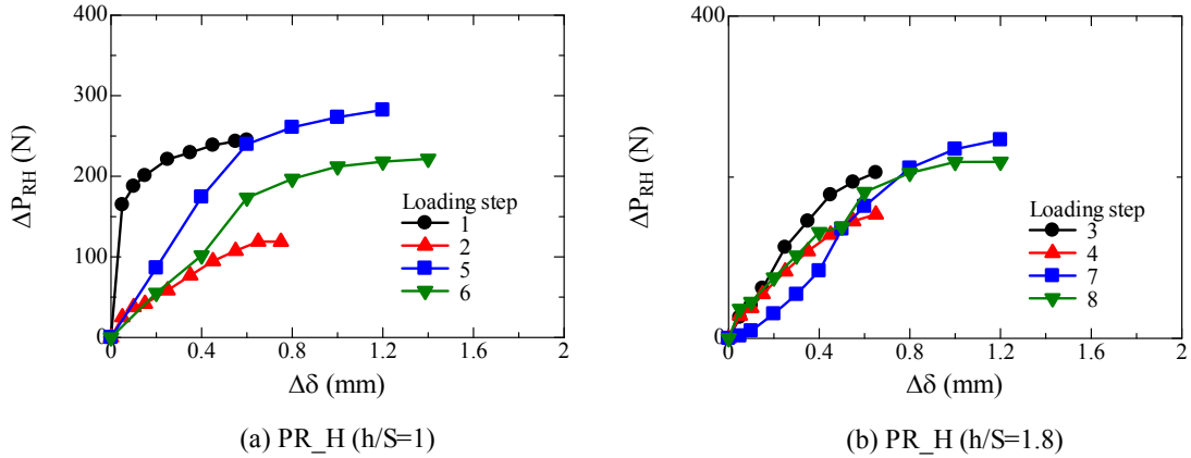
Figure 5.4.2.12 Relationship between \Delta \delta and \Delta P_{RH} for heavy case observed in each loading step.
