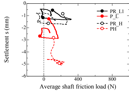
Figure 5.5.2.17 Variation of pile load with settlement observed in loading step 7 and 8 ( \delta_{LDT}=\pm 2\text{mm} , h/S=1.8 ). (A. 5.5.2.16-5.5.2.19)
