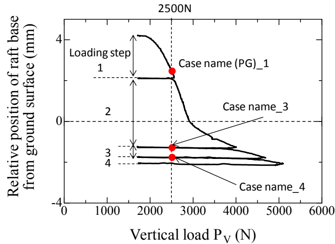
Figure 4.3.3.17 Positions in which axial loads are compared in Fig. 4.3.3.19.
