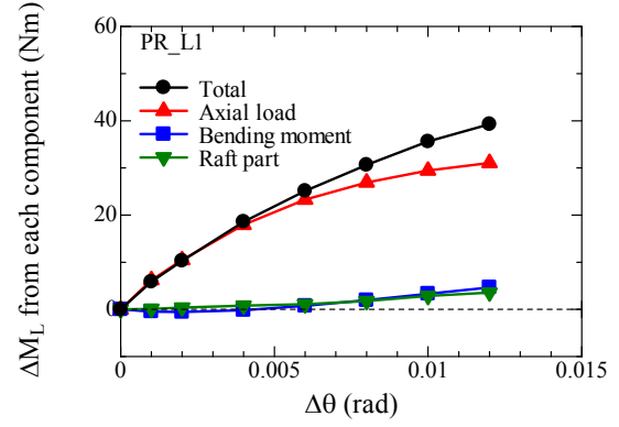
(b) \delta_{LDT} = \pm 1\text{mm} , h/S=1.8
