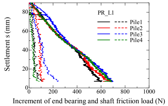
(b) End bearing and shaft friction loads
