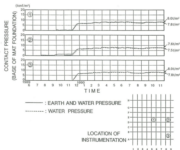
Figure 2.3.7 Measured earth pressure and water pressure. (Kishida (1991))
