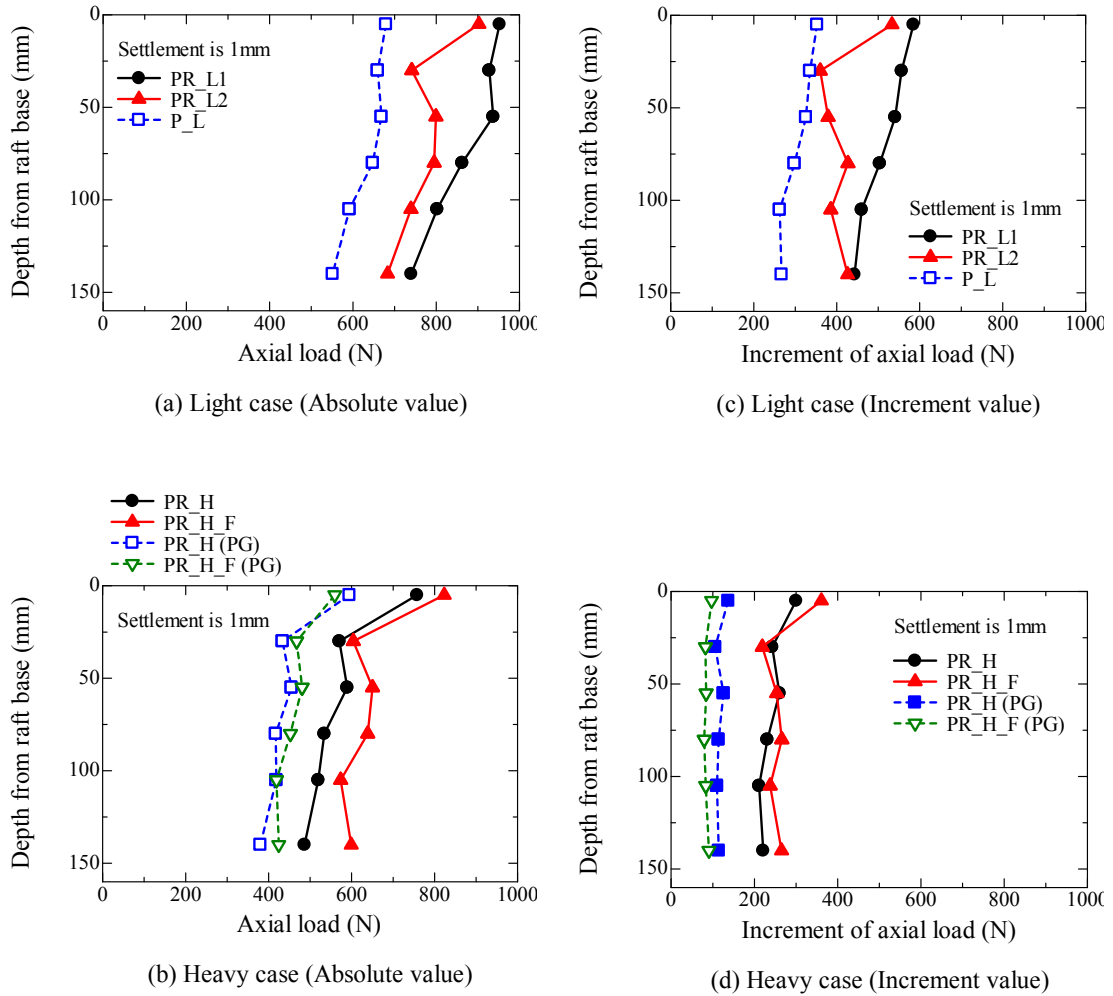
Figure 4.3.3.18 Profile of axial load and axial load increment at settlement of 1mm.
