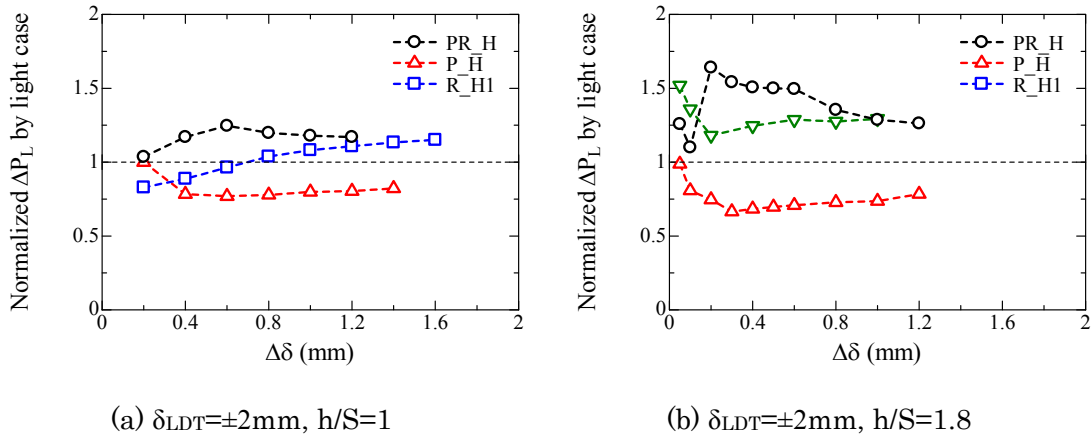
Figure 5.4.1.7 Relationship between \Delta\delta and normalized \Delta P_L of heavy case by that of light case for \delta_{LDT}=\pm 2\text{mm} , h/S=1, 1.8 . (A.5.4.1.3)
