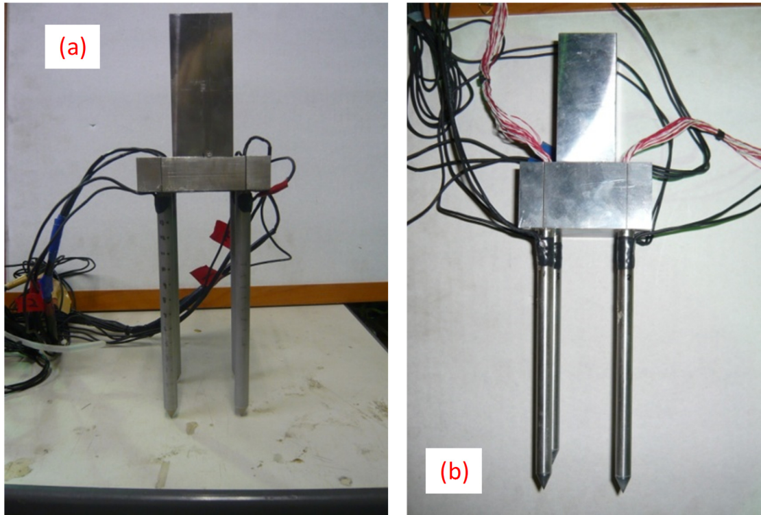
Figure 3.4.11 Model piled raft and pile group (a) for light case, (b) for heavy case.
