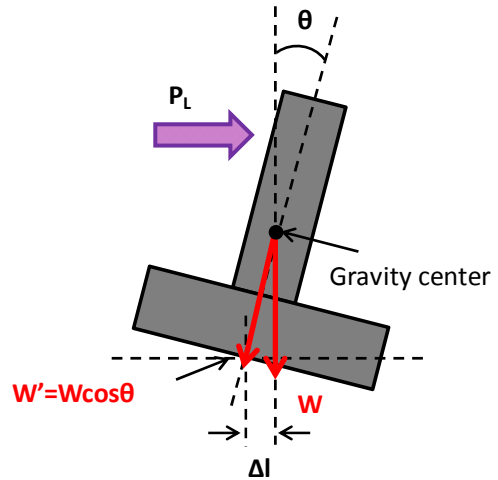
Figure 3.4.3 Influence of foundation rotation on the vertical load of the foundation.
