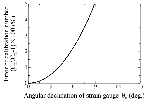
Figure 3.6.12 Error of calibration number caused by angular declination \theta_e .
