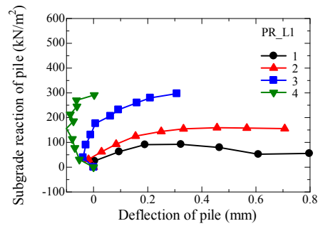
(f) Pull-out pile ( \delta_{LDI} = \pm 2 \text{ mm} , h/S=1 )
