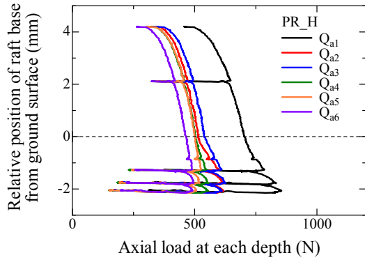
(a) Average of Pile 1 & Pile 2
