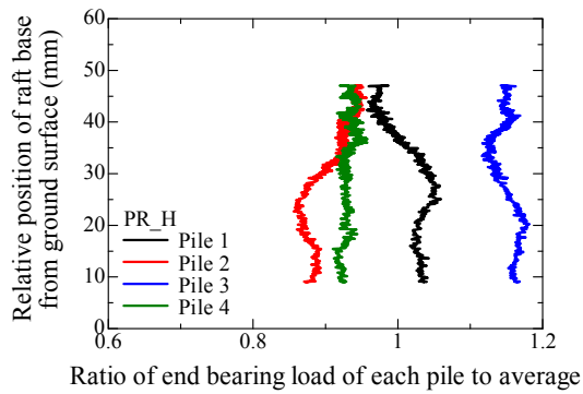
(b) End bearing load
