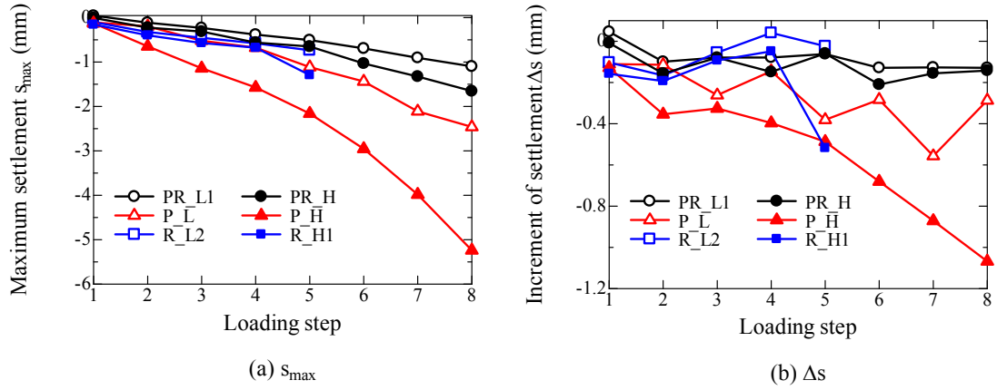
Figure 5.3.1.4 Observed settlement in each loading step.
