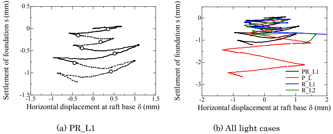
Figure 5.3.1.1 Relationship between horizontal displacement at raft base \delta and settlement s for light case. (A.5.3.1.1)
