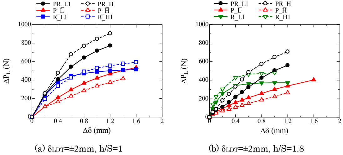
Figure 5.4.1.5 Relationship between \Delta \delta and \Delta P_L observed in \delta_{LDT}=\pm 2\text{mm} , h/S=1, 1.8 . (A. 5.4.1.1)
