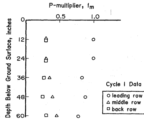
Figure 2.2.3 Experimental p-multipliers vs. depth. (Brown et al. (1988))
