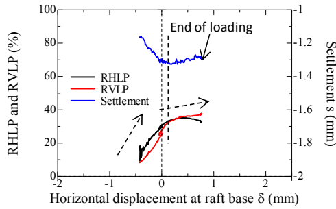
(g) Loading step 7 ( \delta_{LDT}=+2\text{mm} , h/S=1.8 )
