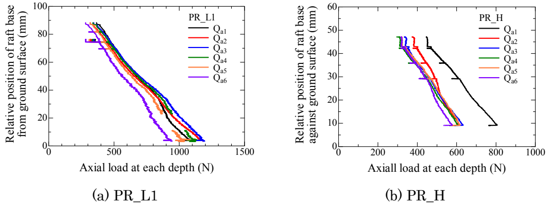
Figure 4.2.1.7 Variation of axial load at each depth with relative position of raft base from ground surface for PR_L1 and PR_H during penetration process.
