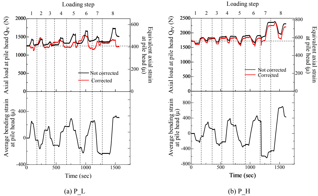
Figure 3.6.16 Variation of axial load and bending strain at pile head with time for P_L and P_H during horizontal loading tests.
