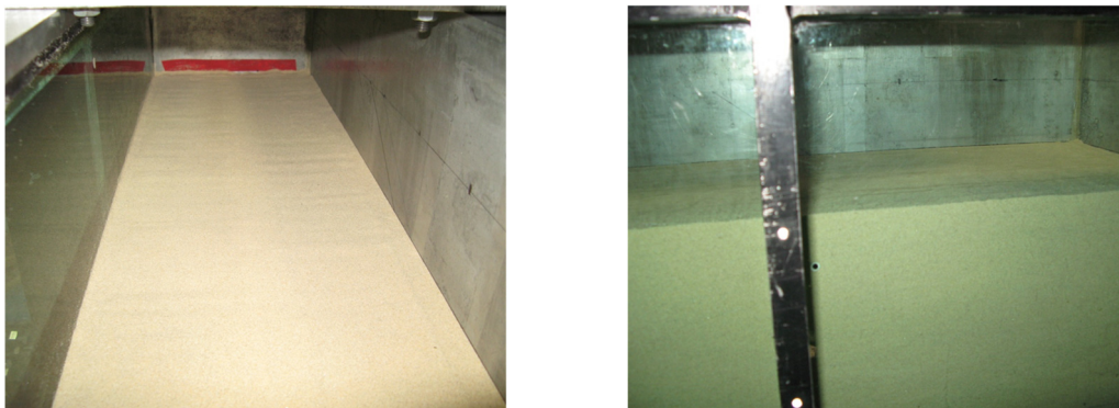
Figure 3.5.1 Model ground prepared by air-pluviation method.
