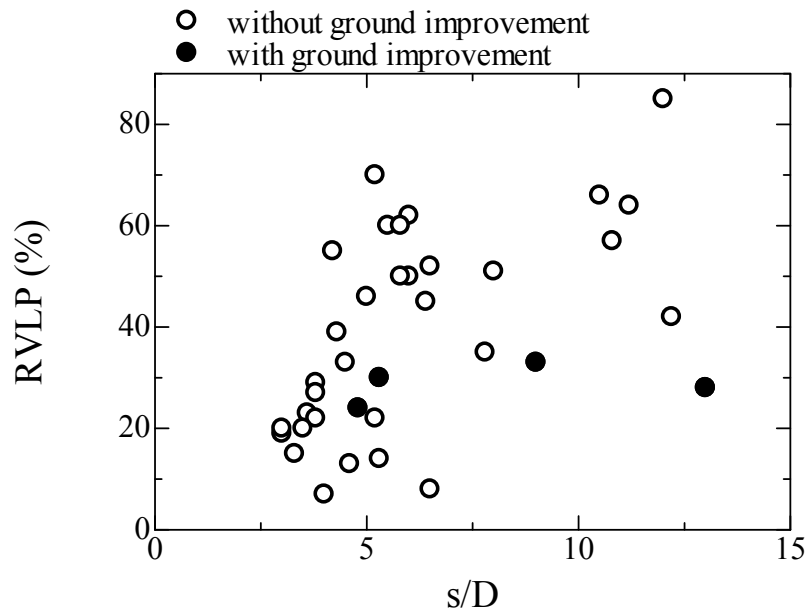
Figure 2.3.10 Relationship between pile spacing ratio ( s/D ) and RVLP.
