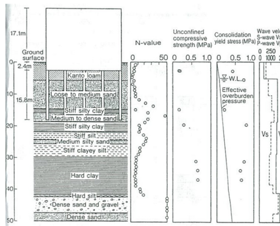
Figure 2.3.8 Schematic illustration of building and soil profiles. (Yamashita et al. (1994))
