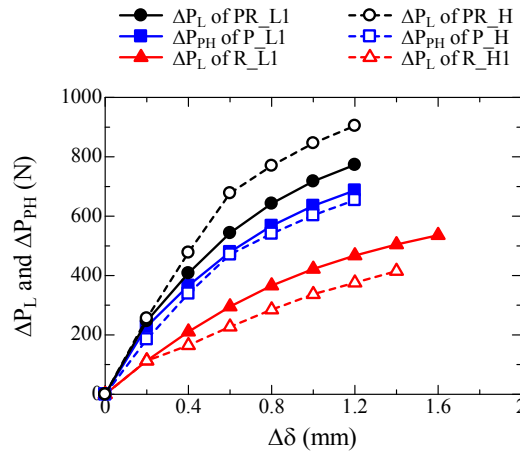
Figure 5.4.3.12 Variation of \Delta P_L and \Delta P_{PH} with \Delta\delta for each loading step for. \delta_{LDT}=\pm 2\text{mm} , h/S=1 . (A. 5.4.3.9)
