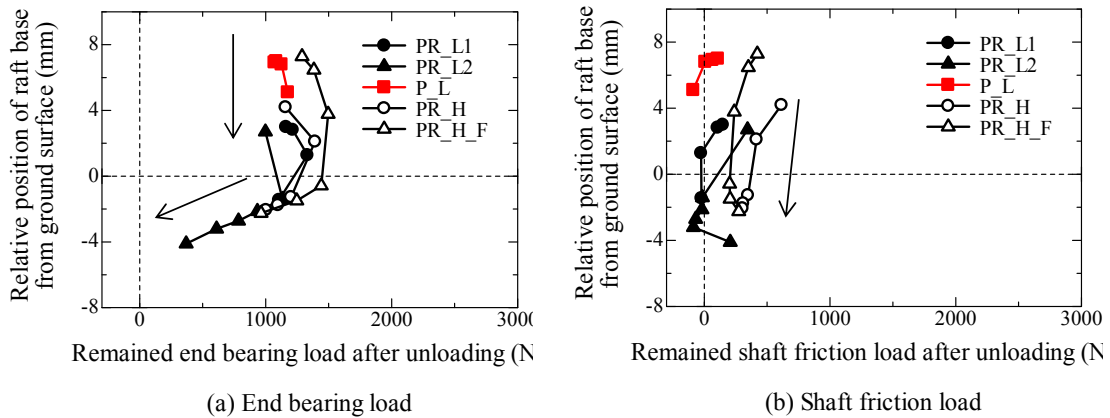
Figure 4.3.3.3 Variation of remained pile loads with relative position of raft base from ground surface observed in vertical loading process.
