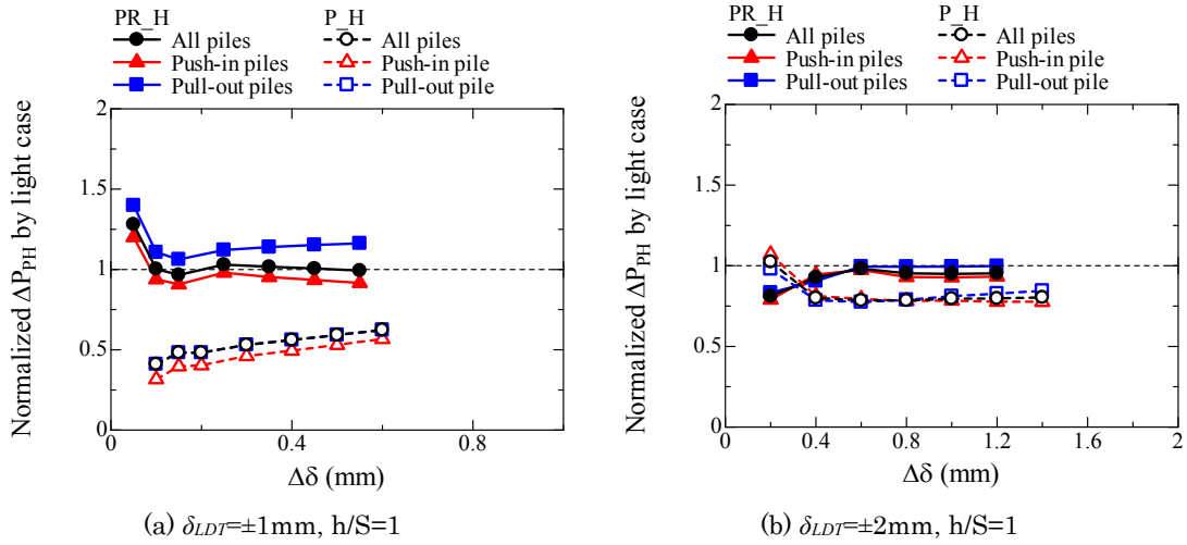
Figure 5.4.3.16 Relationship between \Delta\delta and normalized \Delta P_{PH} of heavy case by that of light case.
