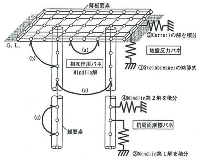
Figure 2.3.19 Concept of Hybrid approach proposed by Tsuchiya et al. (2001)
