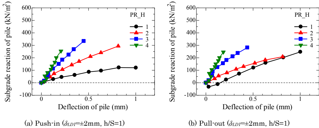
Figure 5.4.3.9 Relationship between pile deflection and subgrade reaction of pile for P_H. (A. 5.4.3.6)
