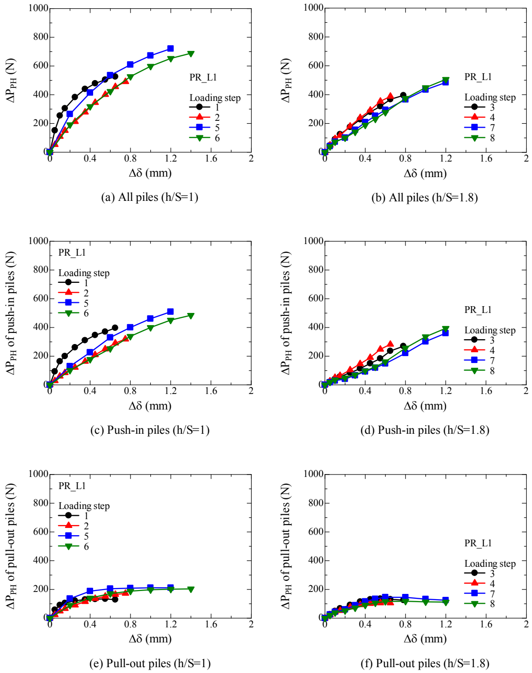
Figure 5.4.3.18 Relationship between \Delta\delta and \Delta P_{PH} for PR_L1 observed in each loading step. (A. 5.4.3.13)
