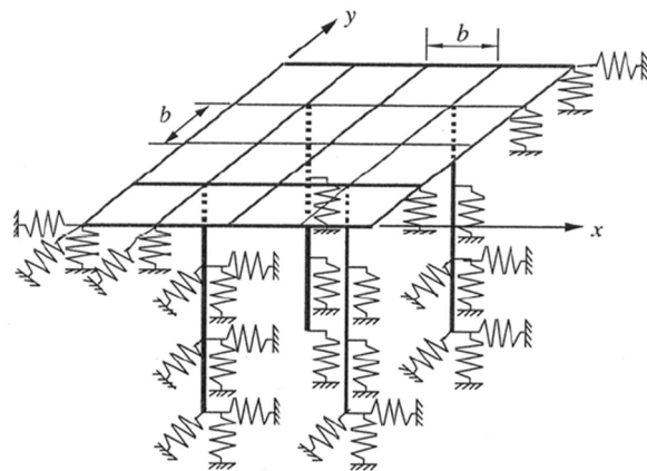
Figure 2.3.20 Hybrid model proposed by Kitiyodom and Matsumoto (2002).
