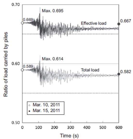
Figure 2.3.28 Ratio of load carried by piles during earthquake. (Yamashita et al. (2012))
