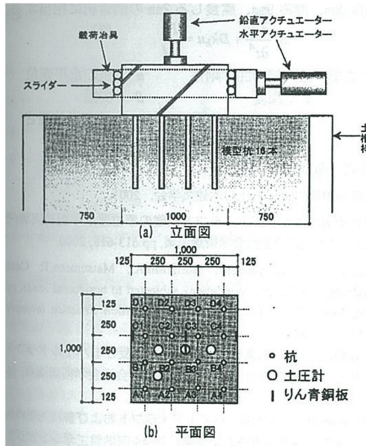
Figure 2.3.34 Schematic view of model setup. (Tsuchiya et al. (2003))
