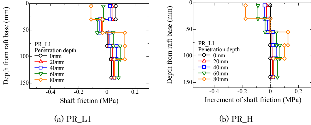
Figure 4.2.1.14 Profiles of shaft friction and shaft friction increment for PR_L1 and PR_H during penetration process.
