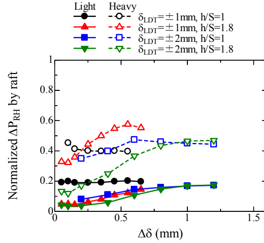
Figure 5.4.2.8 Relationship between \Delta\delta and normalized \Delta P_{RH} by that of raft foundation.
