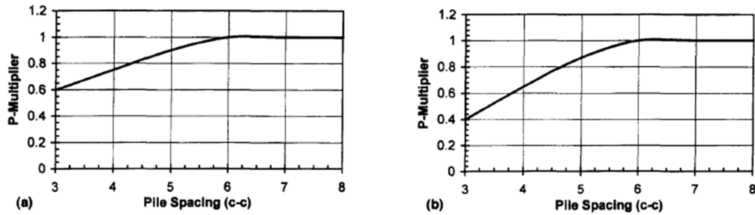
Figure 2.2.4 Interim design curves for p-multipliers as function of pile spacing. (Rollins et al. (1998))
