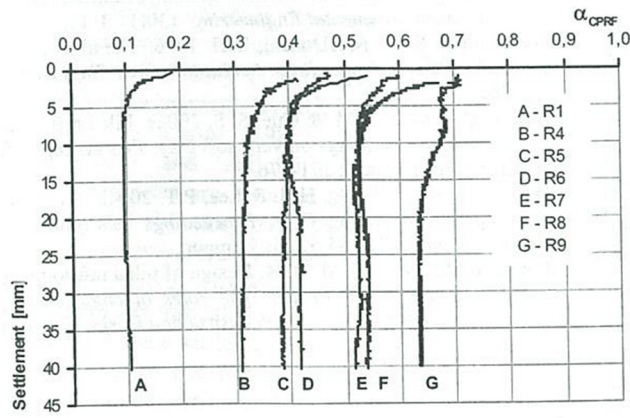
Figure 2.3.15 \alpha_{CPRF} ratio determined by model tests (Tejchman et al. (2005))
