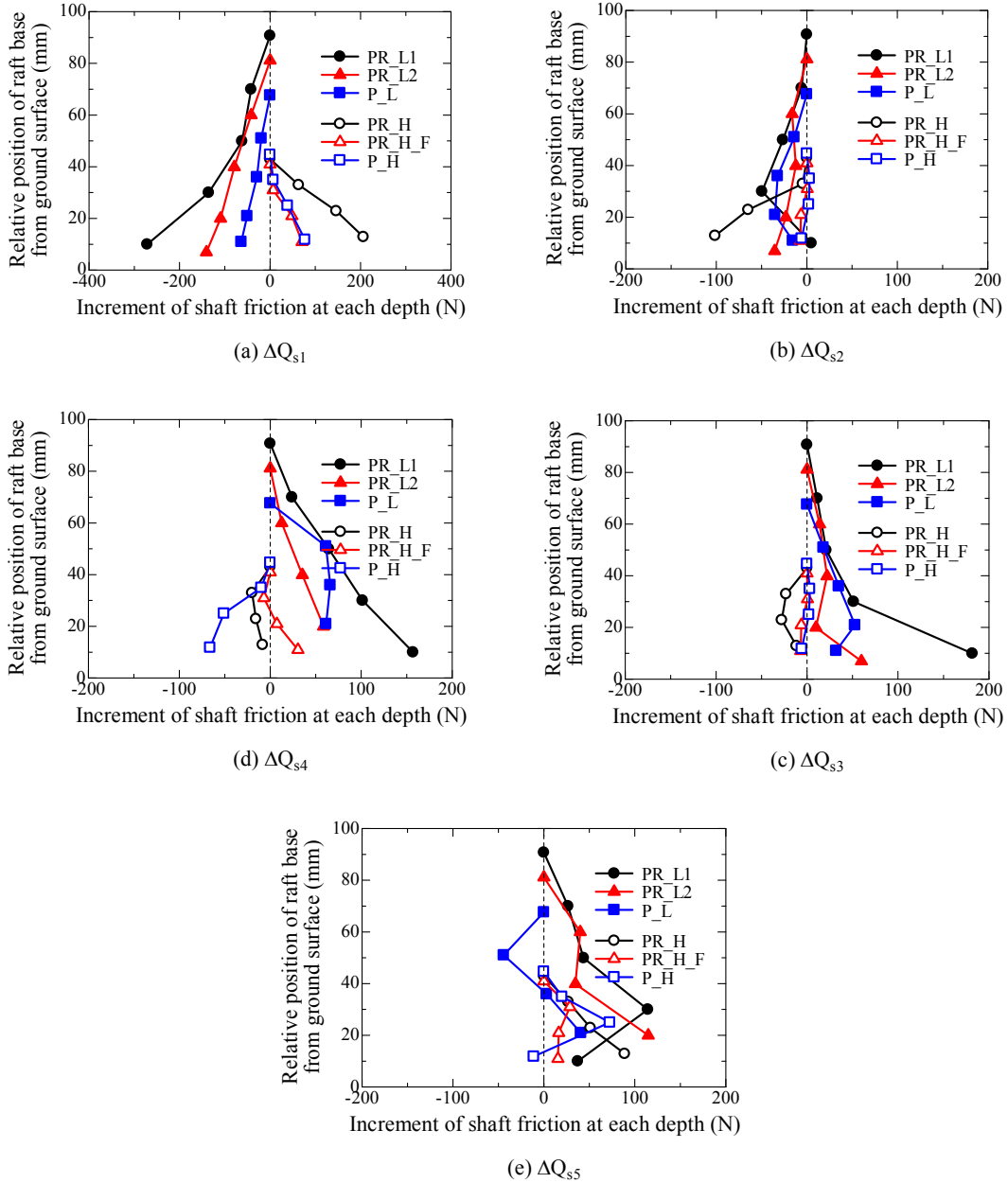
Figure 4.2.1.16 Variation of shaft friction increment at each depth with relative position of raft base from ground surface.
