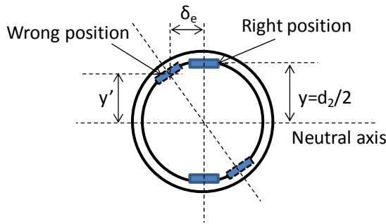
Figure 3.6.7 Measurement error of strain gauge by position gap.
