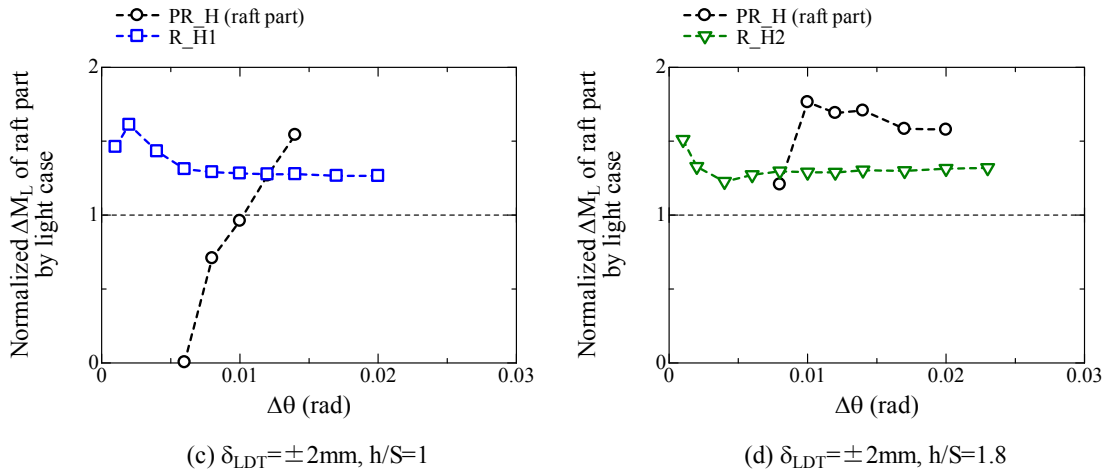
Figure 5.5.3.5 Relationship between \Delta\theta and normalized \Delta M of raft part normalized by light case for \delta_{LDT}=\pm 2\text{mm} , h/S=1 and 1.8 . (A. 5.5.3.6)
