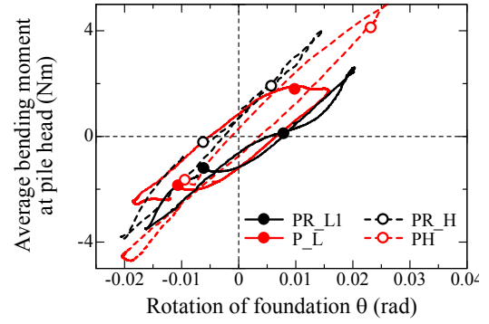
(j) \delta_{LDT} = \pm 2\text{mm} , h/S=1.8 (all piles)
