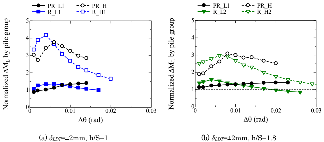
Figure 5.5.1.6 Relationship between \Delta\theta and normalized \Delta M_L by that of pile group. (A. 5.5.1.2)
