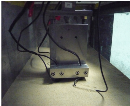
Figure 3.5.4 Model piled raft and pile group after penetration process.
