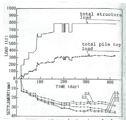
Figure 2.3.4 Time histories of load and settlement. (Kakurai et al. (1987))
