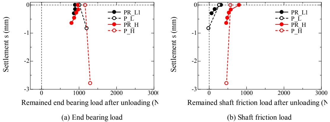
Figure 4.4.2.5 Variation of remained pile load after each unloading period with settlement s , (a) end bearing load, (b) shaft friction load.
