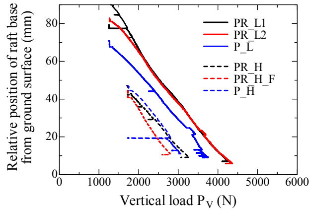
Figure 4.2.1.2 Variation of P_V with relative position of raft base from ground surface observed in the penetration process for all cases.
