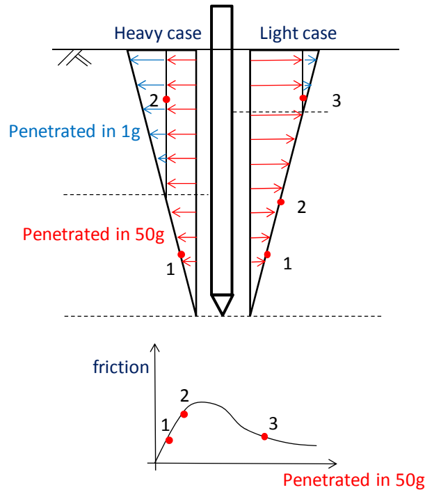
Figure 4.2.1.11 Pile penetration length along soil depth.
