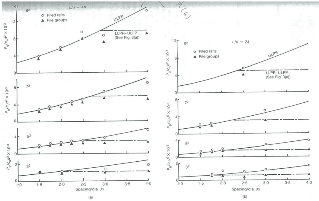
Figure 2.3.11 Comparisons of ultimate load capacities of piled rafts and free-standing pile groups. (Cooke (1986))
