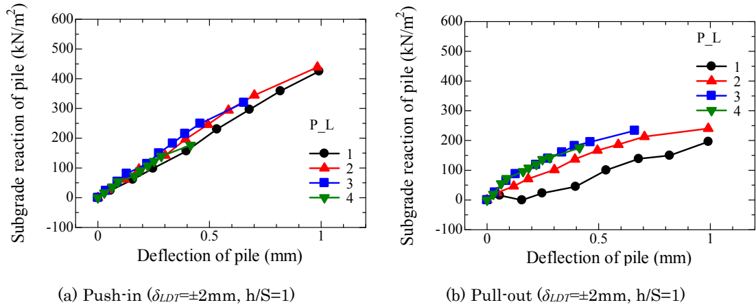
Figure 5.4.3.7 Relationship between pile deflection and subgrade reaction of pile for P_L. (A. 5.4.3.4)
