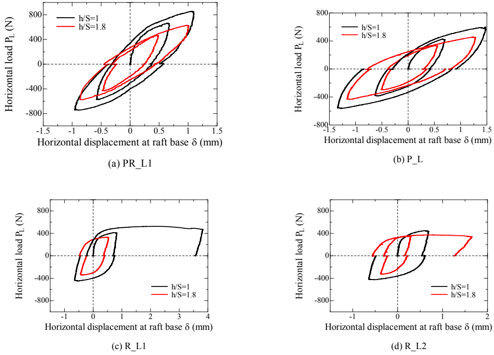
Figure 5.4.1.1 Relationship between horizontal displacement at raft base \delta and horizontal load P_L for light case.
