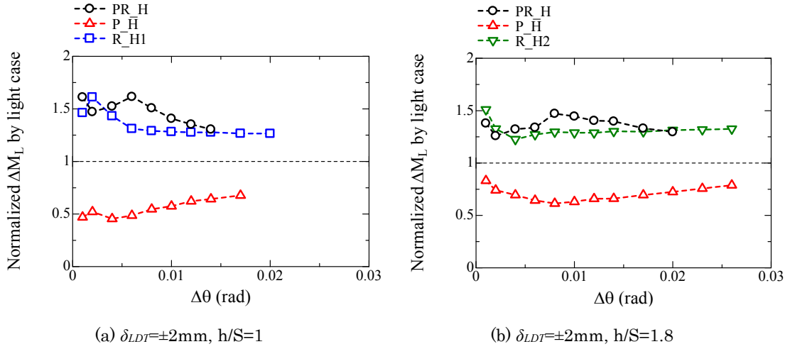
Figure 5.5.1.7 Relationship between \Delta\theta and normalized \Delta M_L of heavy case by that of light case. (A. 5.5.1.3)
