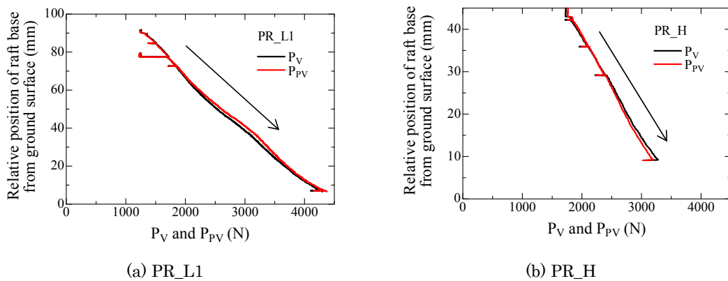
Figure 4.2.1.1 Variation of P_V , P_{PV} with relative position of raft base from ground surface during penetration process for (a) PR_L1 and (b) PR_H. (Other cases are shown in A. 4.2.1.1 and 4.2.1.2)
