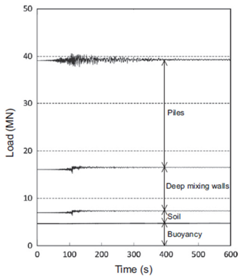
Figure 2.3.27 Load sharing among piles, deep mixing walls and soil during earthquake. (Yamashita et al. (2012))
