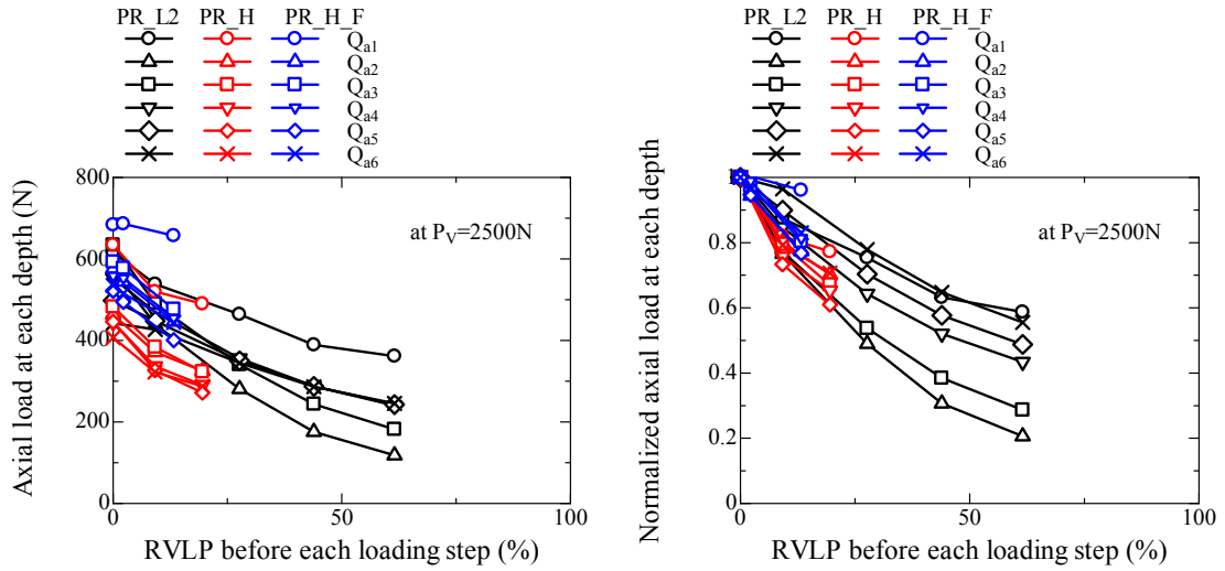
Figure 4.3.3.20 Variation of axial load at each depth and normalized axial load at each depth with RVLP before each loading step.
