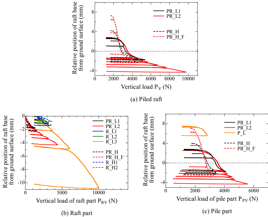
Figure 4.3.2.1 Relationship between vertical load and relative position of raft base from ground surface during vertical loading process.
