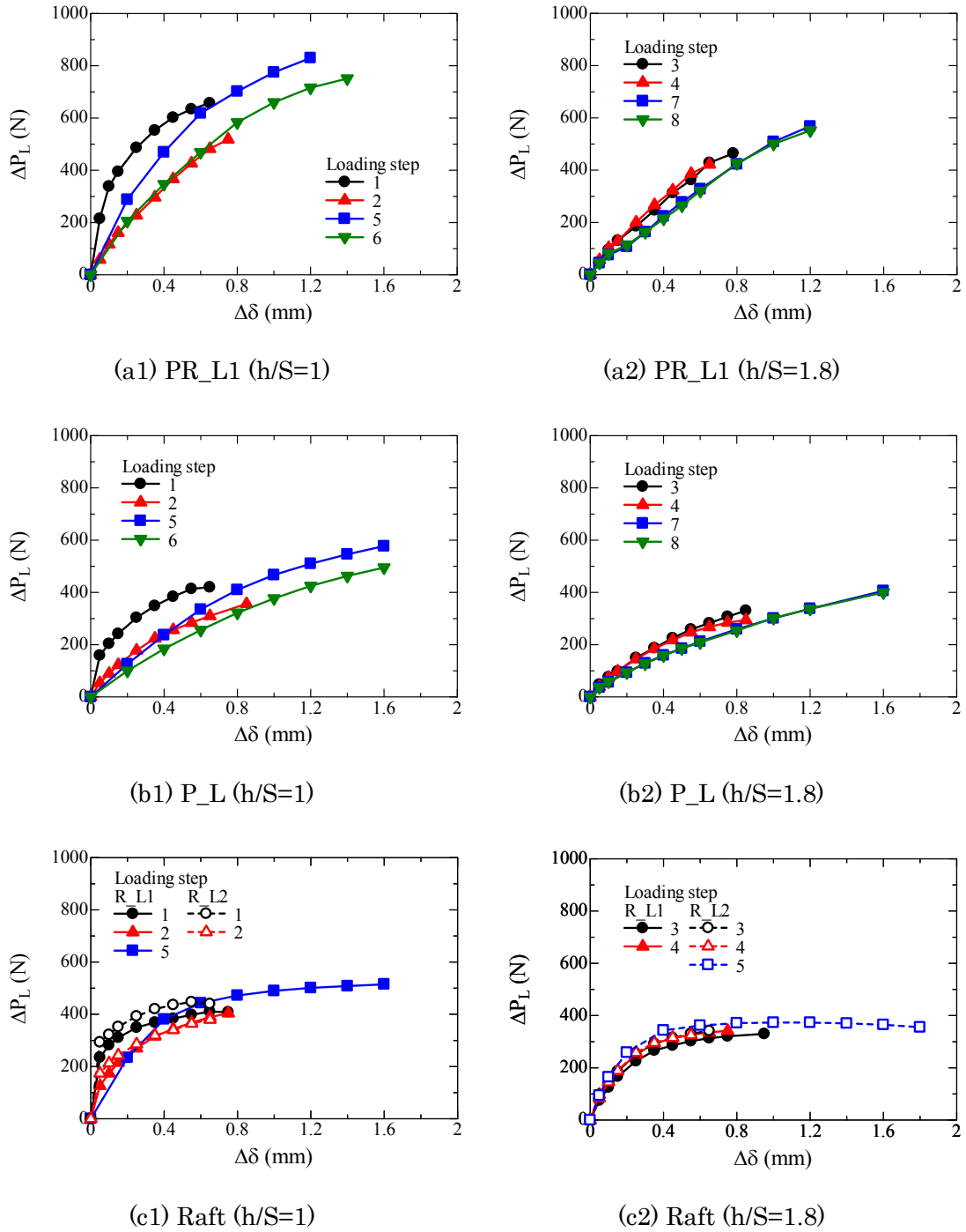
Figure 5.4.1.9 Relationship between \Delta\delta and \Delta P_L for light case observed in each loading step.
