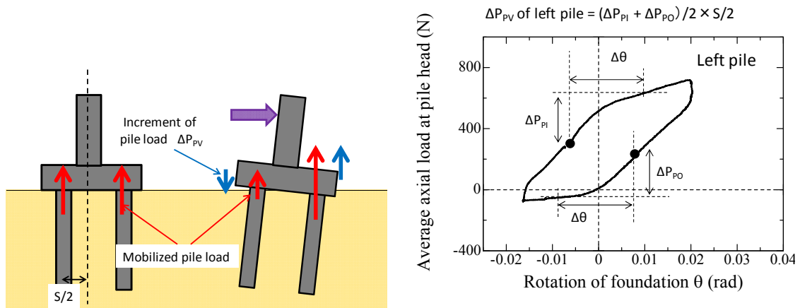
Figure 5.5.3.1 Calculation method to estimate moment resistance from pile load.
