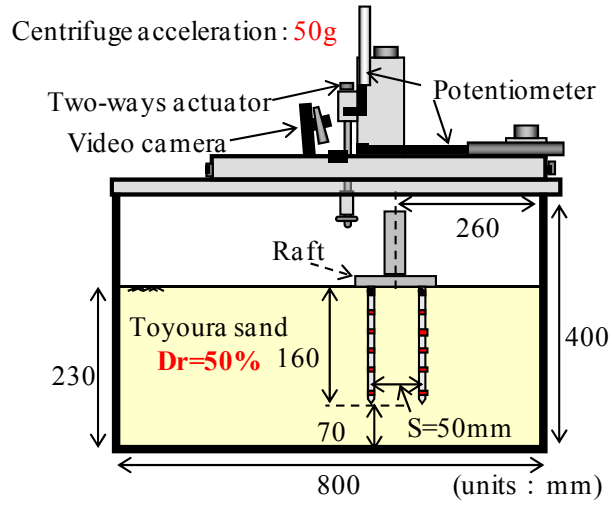
Figure 3.4.1 Schematic illustration of centrifuge package.
