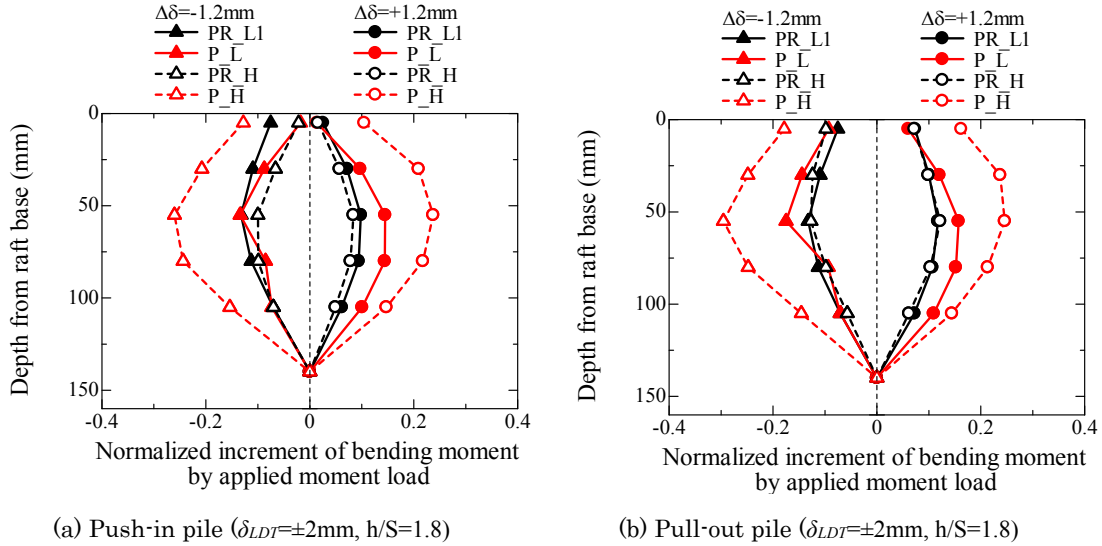
Figure 5.5.2.5 Profile of bending moment at \Delta\delta = \pm 1.2 \text{ mm} . (A. 5.5.2.1)
