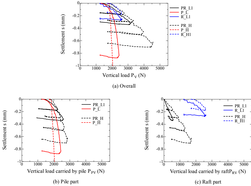
Figure 4.4.2.1 Relationship between vertical load carried by component and settlement.
