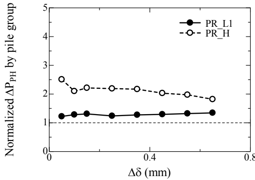
(c) All piles ( \delta_{LDT} = \pm 1\text{mm} , h/S = 1.8 )
