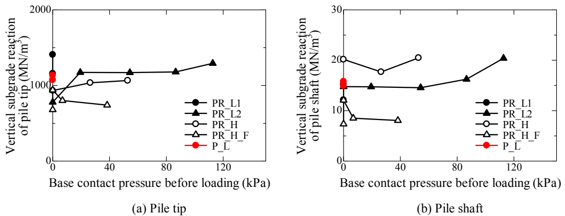
Figure 4.3.3.4 Variation of vertical subgrade reaction of pile with base contact pressure before loading.
