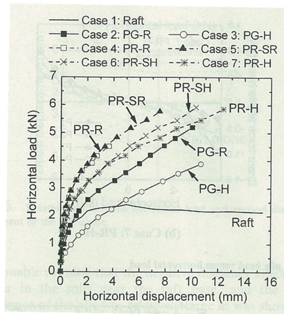
Figure 2.3.44 Horizontal load vs. Horizontal displacement at maximum load in each cycle. (Matsumoto et al. (2010))
