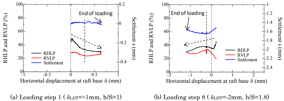
Figure 5.4.2.5 Variation of RHLP, RVLP and settlement s for heavy case. (A. 5.4.2.4)
