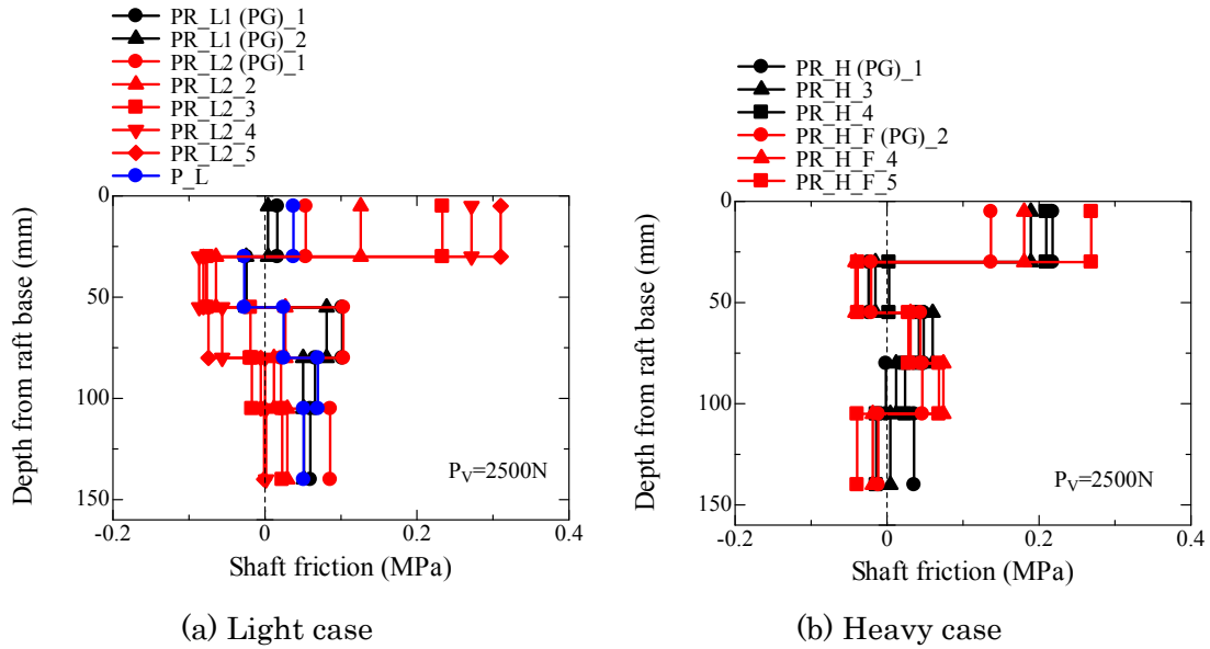
Figure 4.3.3.24 Profile of shaft friction at P_v of 2500N for (a) light case, (b) heavy case. (A. 4.3.3.23)
