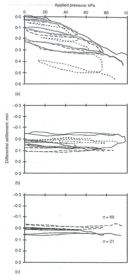
Figure 2.3.13 Differential settlement of raft during loading tests: (a) unpiled raft; (b) piled raft with 9 piles; (c) piled raft with 21 and 69 piles. (Horikoshi and Randolph (1996))
