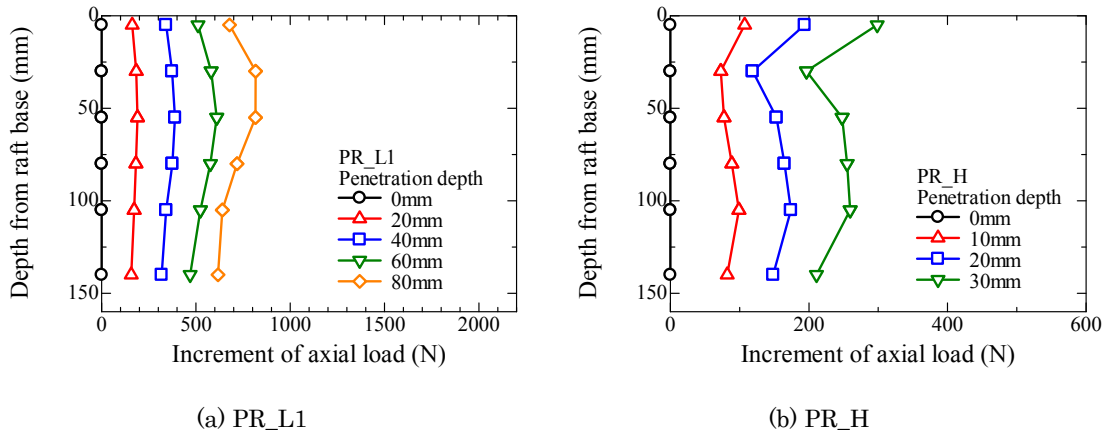
Figure 4.2.1.10 Profiles of axial load increment for PR_L1 and PR_H during penetration process.
