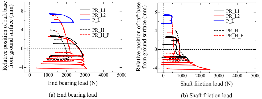
Figure 4.3.3.1 Variation of end bearing and shaft friction loads with relative position of raft base from ground surface for light and heavy cases observed in vertical loading process.
