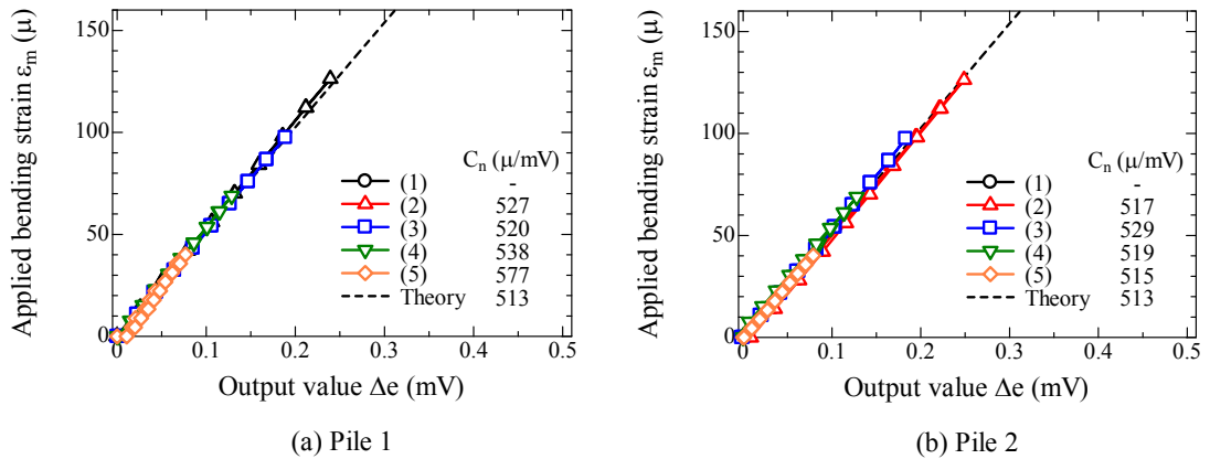
Figure 3.6.4 Relationship between output value and applied bending strain for heavy case pile.
