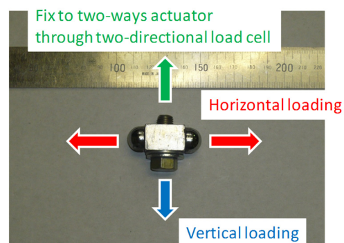
Figure 3.4.23 Horizontal loading device.
