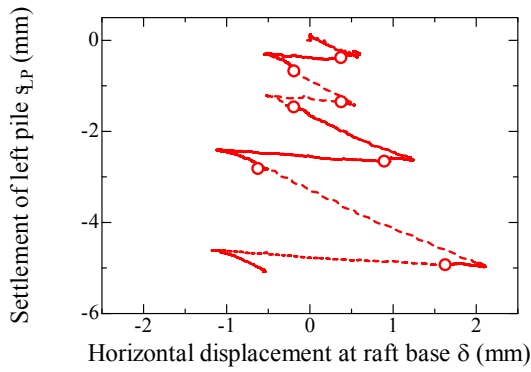
(c) P_H (left pile)
