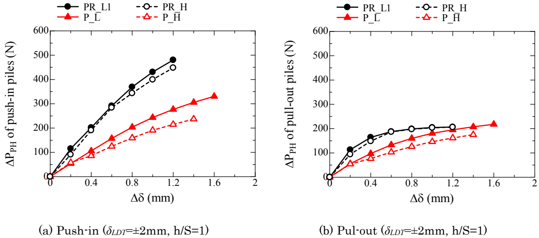
Figure 5.4.3.13 Relationship \Delta P_{PH} of push-in and pull-out piles with \Delta\delta for each loading step. (A. 5.4.3.10)
