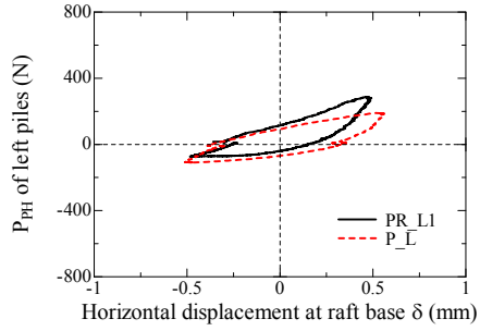
(c) Left piles ( \delta_{LDI} = \pm 1 \text{ mm} , h/S=1.8 )
