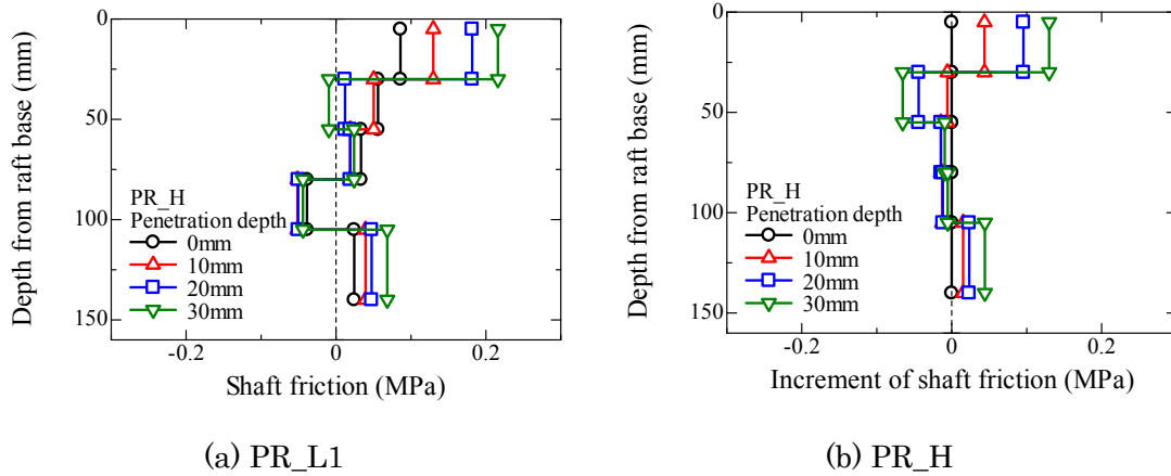
Figure 4.2.1.15 Profiles of shaft friction and shaft friction increment for PR_L1 and PR_H during penetration process. (A.4.2.1.21-4.2.1.26)
