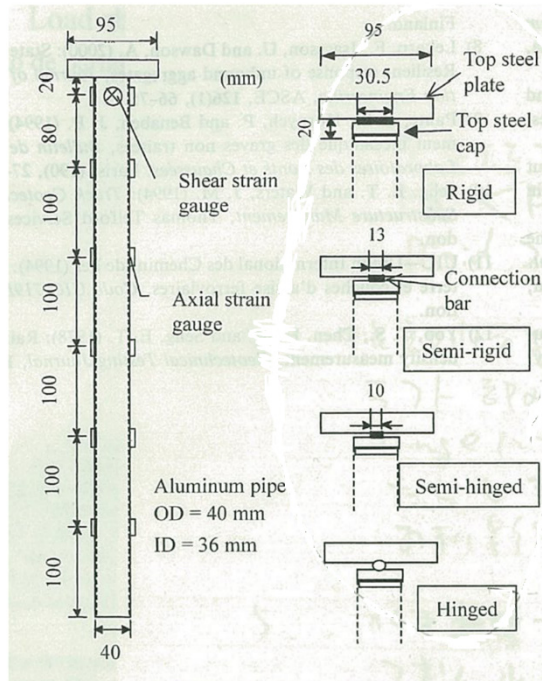
Figure 2.3.43 Model piles with different pile head connection conditions. (Matsumoto et al. (2010))
