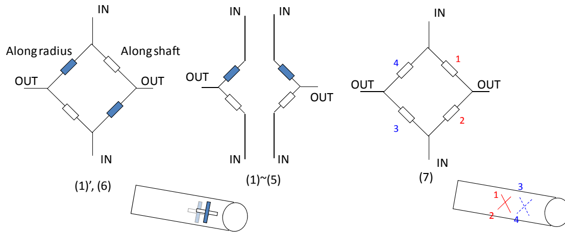
Figure 3.4.10 Bridge circuit for each strain gauge type.
