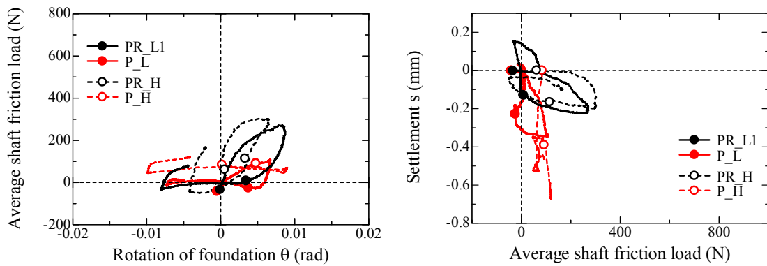
(c) Shaft friction load (Left pile)
