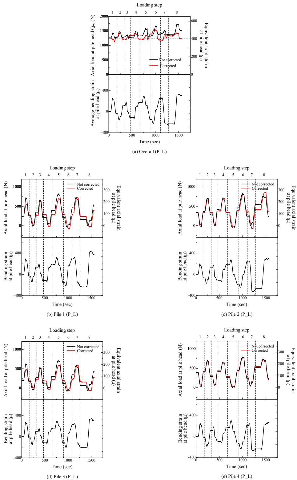
A. 3.6.10 Variation of axial load and bending strain at pile head with time for P_L during horizontal loading test.
