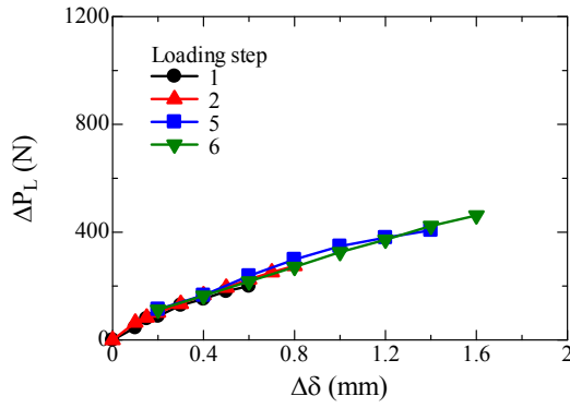
(b1) P_H (h/S=1)
