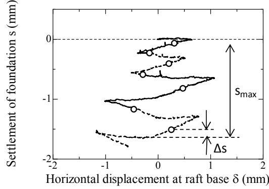
Figure 5.3.1.3 Definition of s_{max} and \Delta s .
