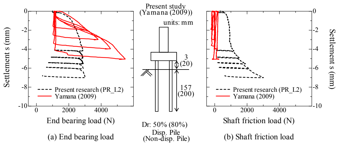
Figure 3.5.6 Variation of pile load with settlement during vertical loading test.
