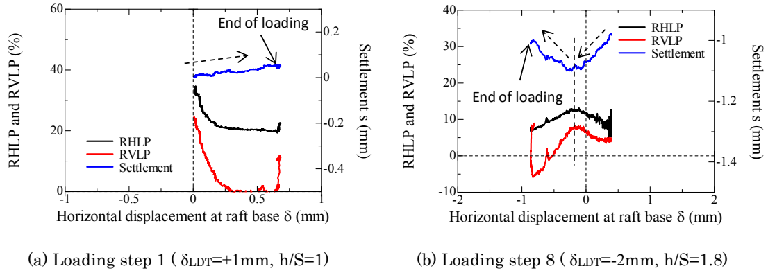
Figure 5.4.2.4 Variation of RHLP, RVLP and settlement s for light case. (A. 5.4.2.3)
