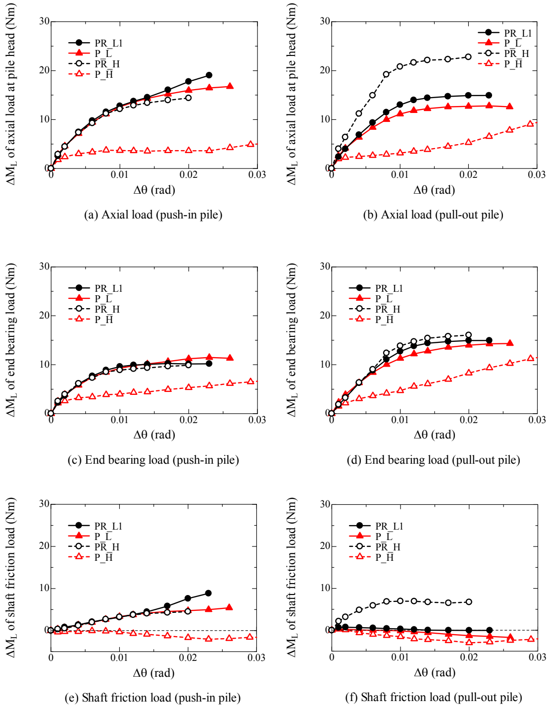
Figure 5.5.3.10 Relationship between \Delta\theta and \Delta M from pile load observed in \delta_{LDT}=\pm 2\text{mm} and h/S=1 (loading step 7 and 8). (A. 5.5.3.12-5.5.3.15)
