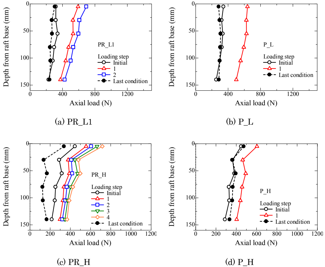
Figure 4.4.2.7 Profiles of axial load during pre-vertical loading process. (A. 4.4.2.6-4.4.2.9)
