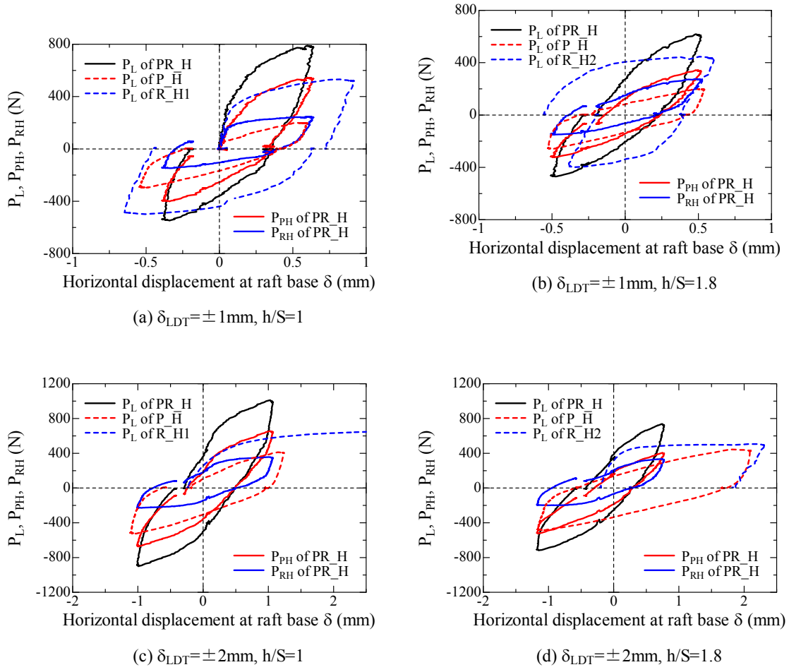
A. 5.4.2.2 Variation of horizontal load P_L and horizontal load carried by raft P_{RH} and piles P_{PH} with horizontal displacement at raft base \delta for heavy case.
