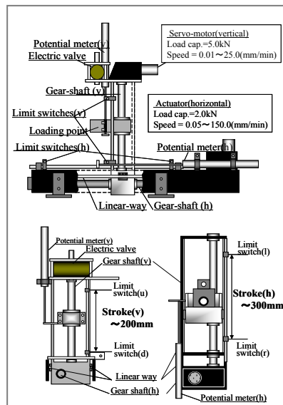
Figure 3.4.20 Details of two-ways actuator.
