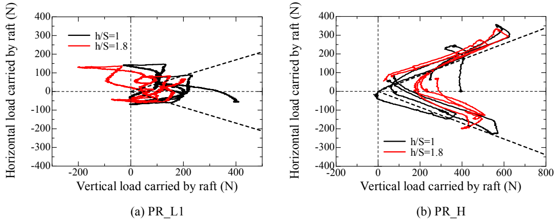
Figure 5.4.2.6 Relationship between vertical load carried by raft P_{RV} and horizontal load carried by raft P_{RH} .
