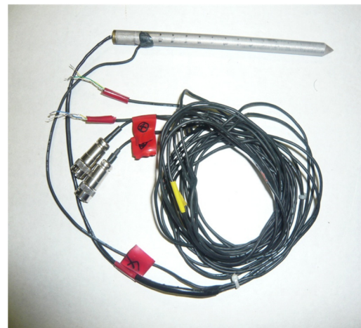
Figure 3.4.9 Picture of model pile.
