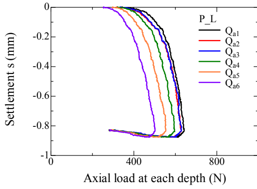
(a) Average of Pile 1 &amp; Pile 2
