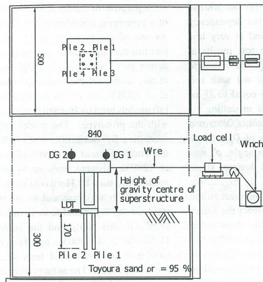
Figure 2.3.38 Schematic illustration of test setup. (Matsumoto et al. (2004a))
