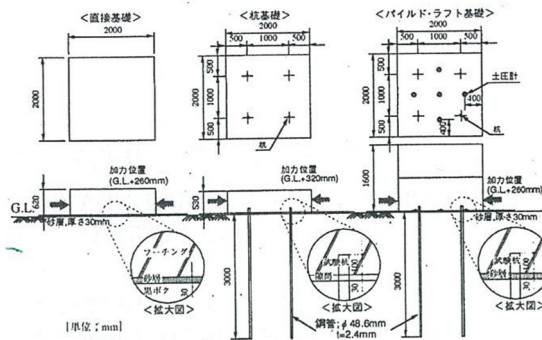
Figure 2.3.29 Schematic view of model foundations. (Nagano et al. (2002))
