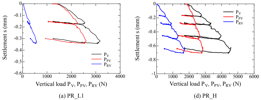
Figure 4.4.1.1 Variation of P_V , P_{PV} and P_{RV} with settlement during pre-vertical loading process.
