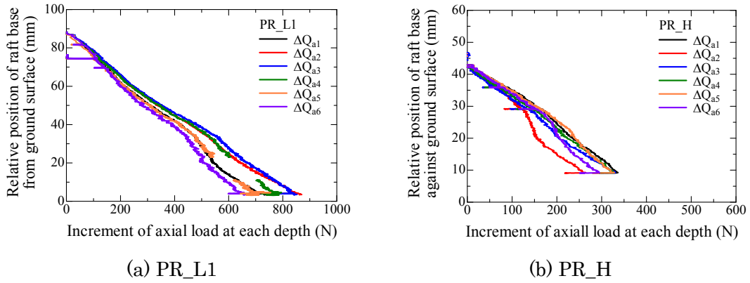
Figure 4.2.1.8 Variation of axial load increment at each depth with relative position of raft base from ground surface for PR_L1 and PR_H during penetration process. (A. 4.2.1.3-4.2.1.8)
