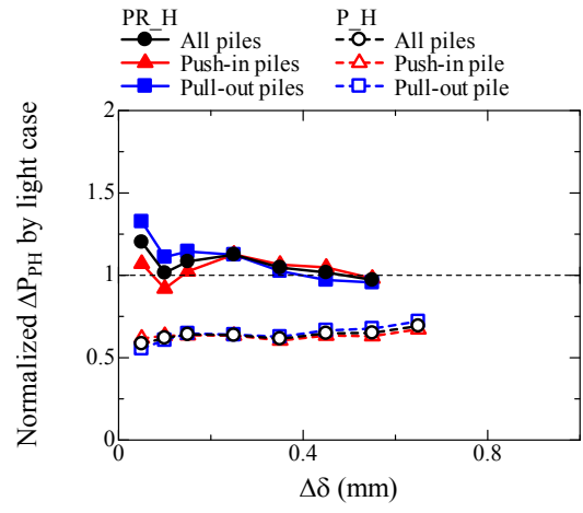
(b) \delta_{LDT} = \pm 1\text{mm} , h/S=1.8
