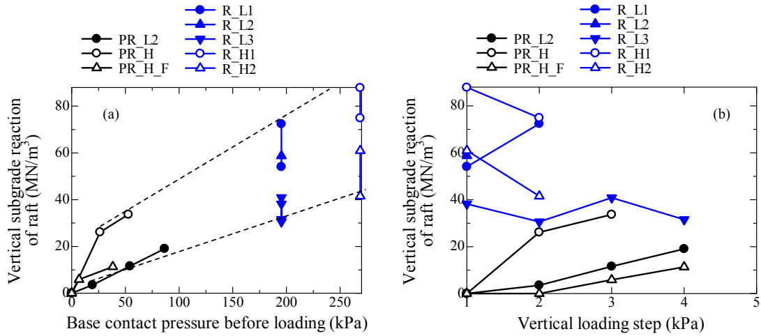
Figure 4.3.2.3 Variation of vertical subgrade reaction of raft with (a) base contact pressure before loading and (b) vertical loading step during vertical loading process.
