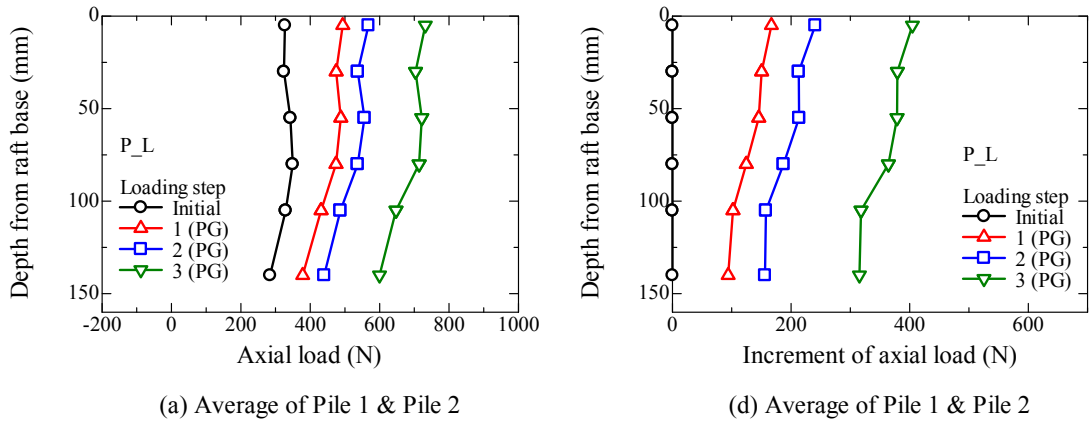
Figure 4.3.3.14 Profiles of axial load and axial load increment for P_L during vertical loading process.
