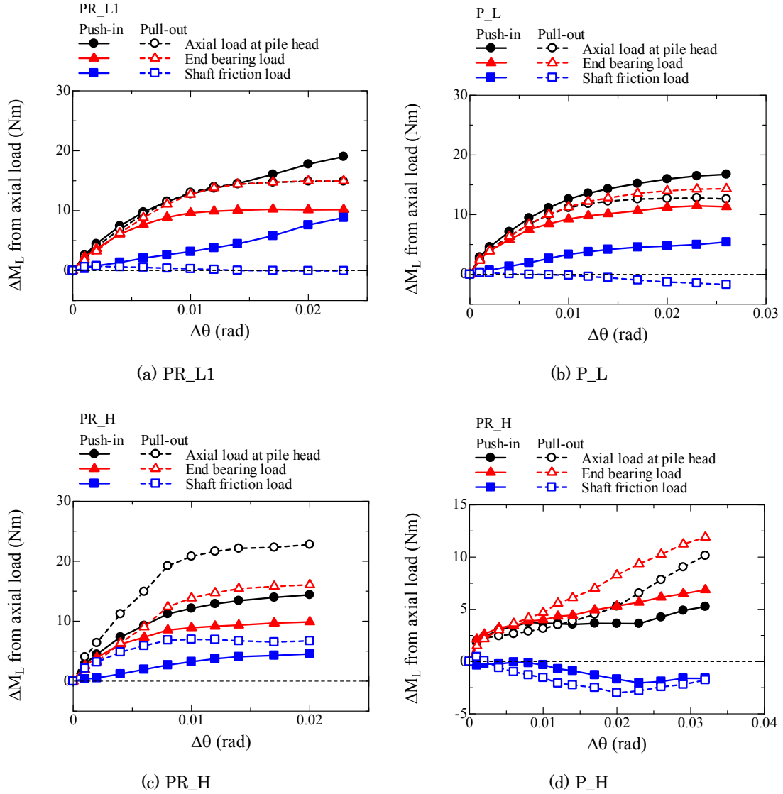
Figure 5.5.3.9 Relationship between \Delta\theta and \Delta M from axial load at pile head, end bearing load and shaft friction load for \delta_{LDT}=\pm 2\text{mm} and h/S=1.8 . (A. 5.5.3.8-5.5.3.11)
