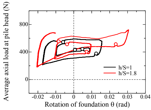
(a) Axial load at pile head (Left pile)
