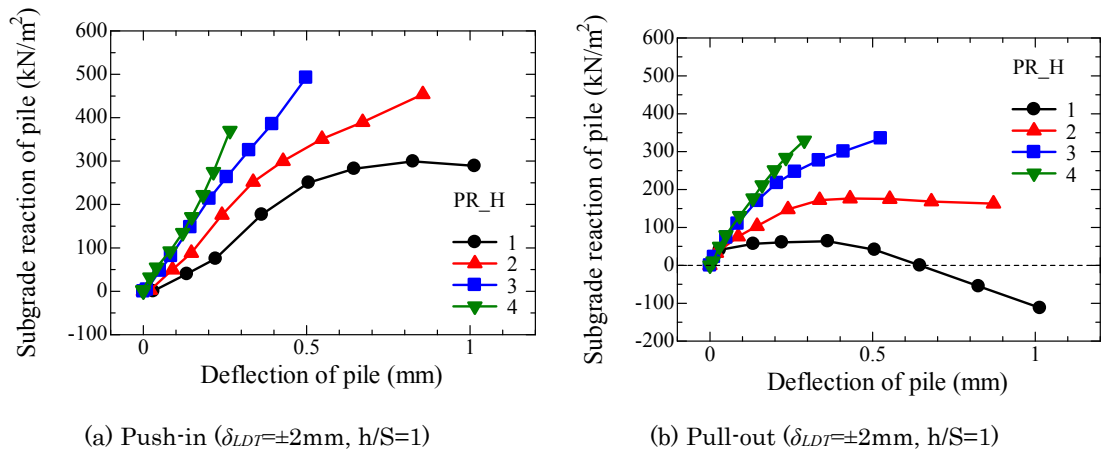
Figure 5.4.3.8 Relationship between pile deflection and subgrade reaction of pile for PR_H. (A. 5.4.3.5)
