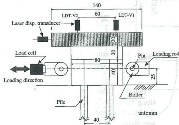
Figure 2.3.36 Illustration of horizontal loading system. (Horikoshi et al. (2003a))
