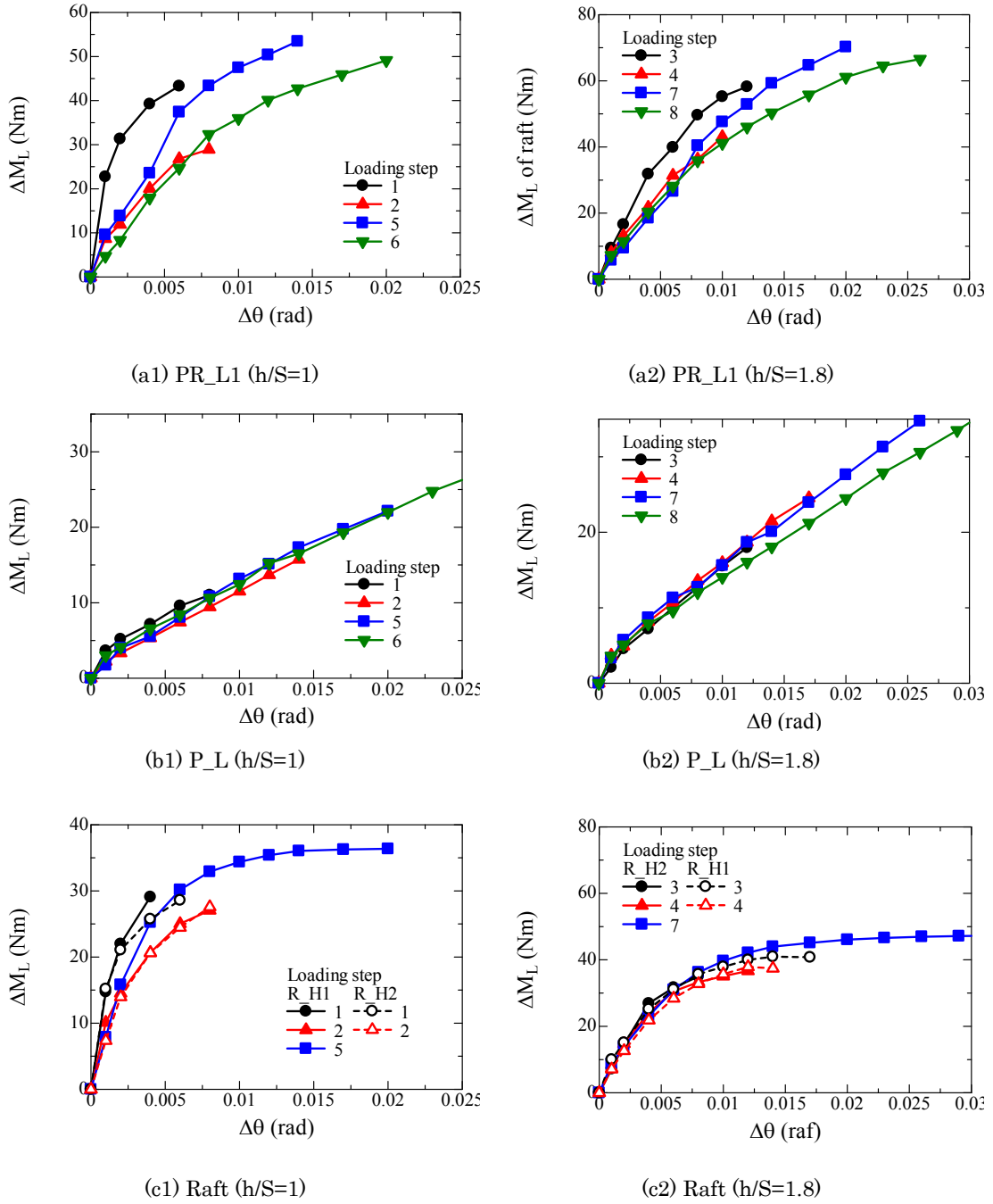
Figure 5.5.1.9 Relationship between \Delta \theta and \Delta M_L for heavy case observed in each loading step.
