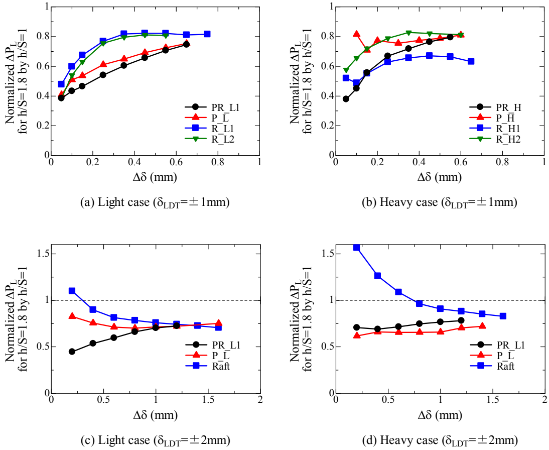
Figure 5.4.1.8 Relationship between \Delta\delta and normalized \Delta P_L for h/S=1.8 by that of h/S=1 .
