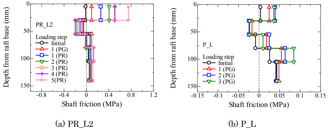
Figure 4.3.3.22 Profiles of shaft friction for PR_L2 and P_L during the vertical loading process. (A. 4.3.3.17-4.3.3.21)
