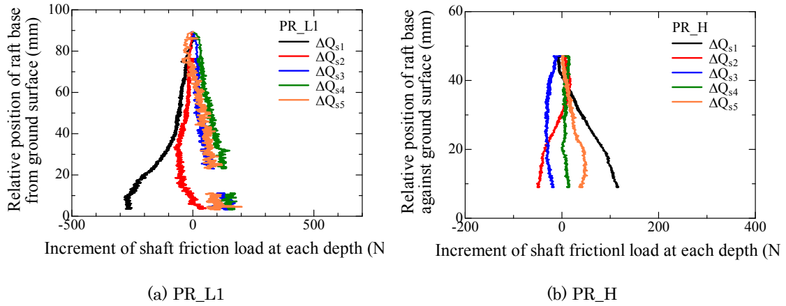
Figure 4.2.1.13 Variation of shaft friction at each depth with relative position of raft base from ground surface for PR_L1 and PR_H during penetration process. (A. 4.2.1.15-4.2.1.20)
