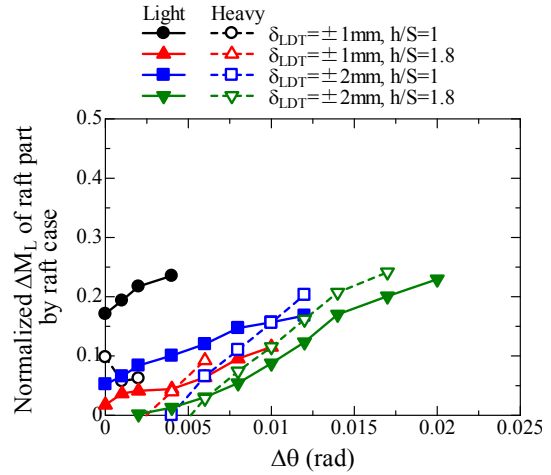
Figure 5.5.3.4 Relationship between \Delta\theta and normalized \Delta M of raft part by raft foundation.
