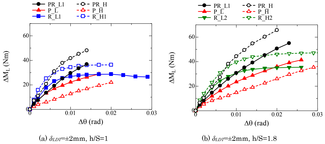
Figure 5.5.1.5 Relationship between \Delta\theta and \Delta M_L for each loading step.
