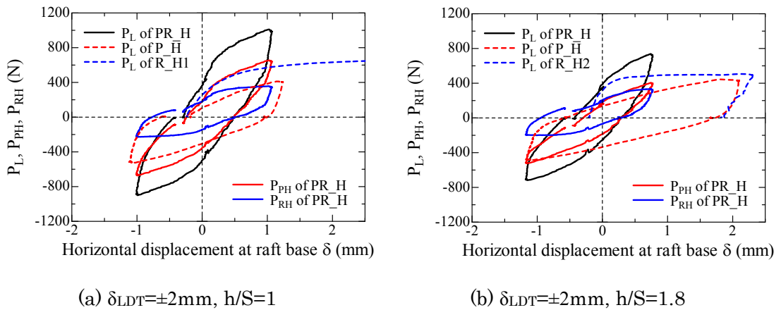
Figure 5.4.2.2 Variation of horizontal load P_L and horizontal load carried by raft P_{RH} and piles P_{PH} with horizontal displacement at raft base \delta for heavy case. (A. 5.4.2.2)
