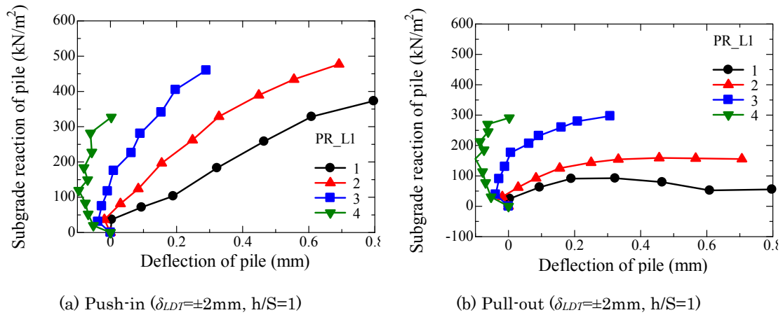
Figure 5.4.3.6 Relationship between pile deflection and subgrade reaction of pile for PR_L1. (A. 5.4.3.3)
