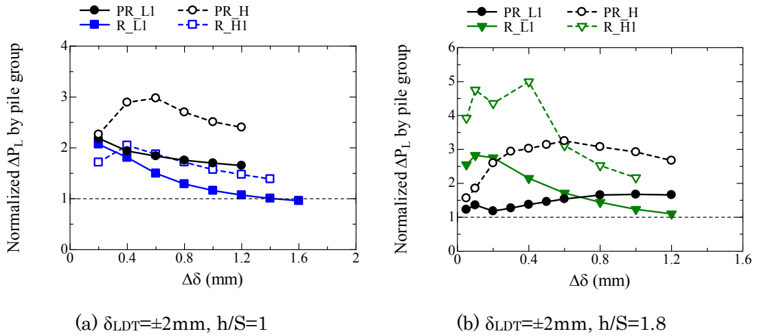
Figure 5.4.1.6 Relationship between \Delta\delta and normalized \Delta P_L by that of pile group for \delta_{LDT}=\pm 2\text{mm} , h/S=1, 1.8 . (A. 5.4.1.2)
