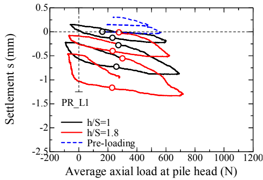
(a) Axial load at pile head (left pile)
