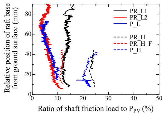
Figure 4.2.1.4 Ratio of shaft friction load to vertical load carried by piles P_{PV} during penetration process for all cases.
