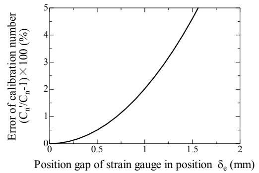
Figure 3.6.8 Error of calibration number caused by position gap \delta_e .
