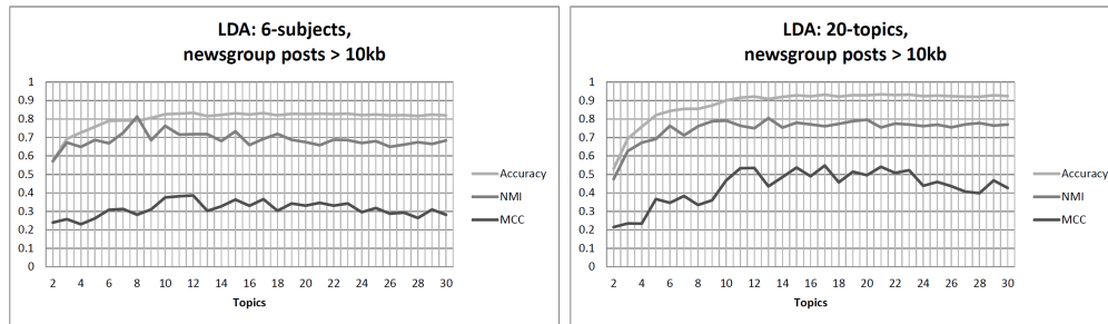
Figure 7.24: Results for LDA-based clustering on the newsgroup articles larger than 10.0 kb.
