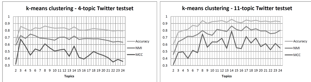
Figure 7.16: Results for k -means clustering on the Twitter ground truth.
