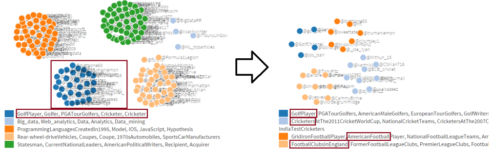
Figure 5.4: An example of cluster labeling and recursive clustering. For each cluster k , the top-5 cluster-based traits from \mathbf{t}_k are listed. A “Sports” cluster is isolated and further sub-divided into the individual sports that made up the cluster.
