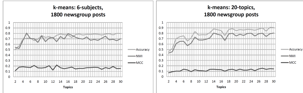
Figure 7.25: Results for k-means-based clustering on the newsgroup articles larger than 10.0 kb.
