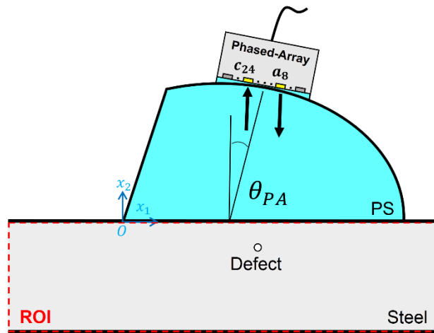
Figure 2.22 Test configuration for sub-section 2.4.2.
