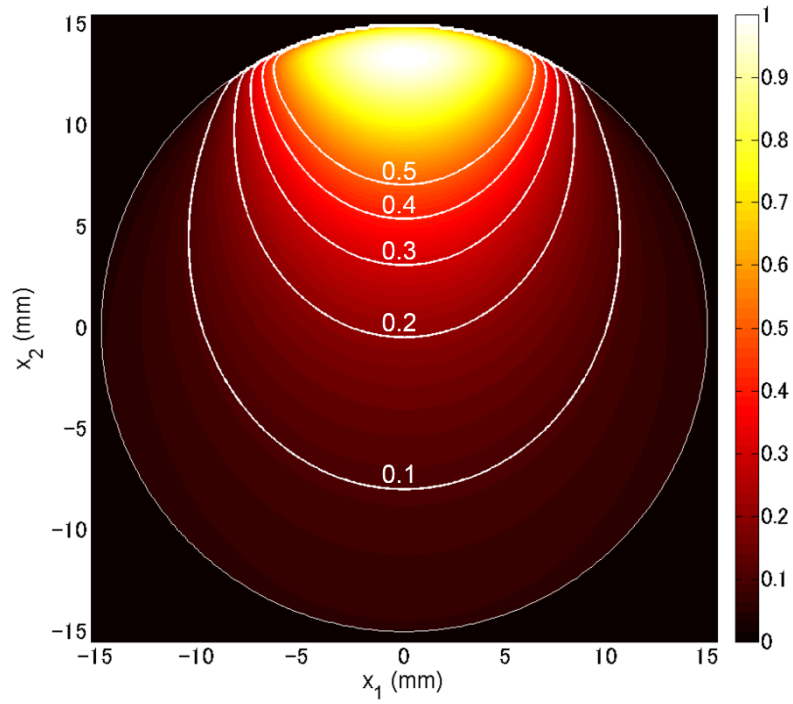
Figure 3.6 L-mode summed AWS beam radiations from all 64 transducers; \sum_i \sum_j |u_i^L u_j^L| .
