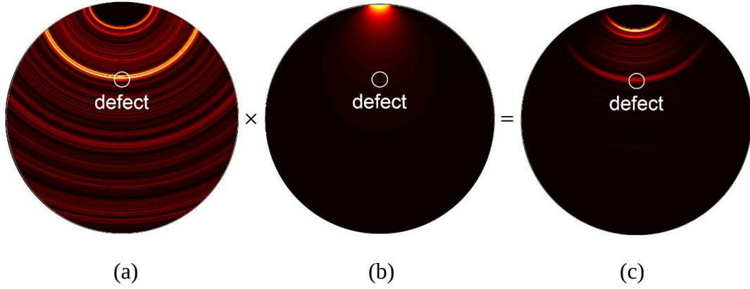
Figure 2.20 L-mode AWS-SAFT for transmitter i = 32 and receiver j = 32 ;
