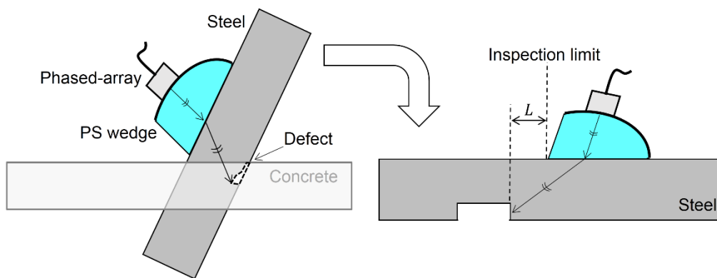
Figure 4.16 Simplified model used in this study.
