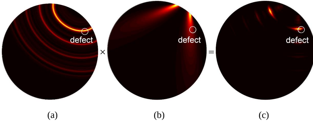
Figure 2.21 T-mode AWS-SAFT for transmitter i = 64 and receiver j = 64 ;
