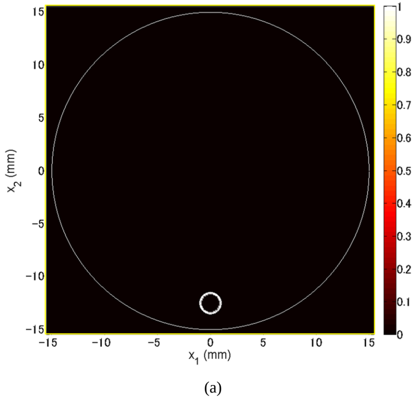
Figure 3.11 Case 1C results when SDH is outside the ER of L-mode. (a) Benchmark, MSSIM = 1; (b) SAFT, MSSIM = 0.2714 and (c) AWS-SAFT, MSSIM = 0.2792.
