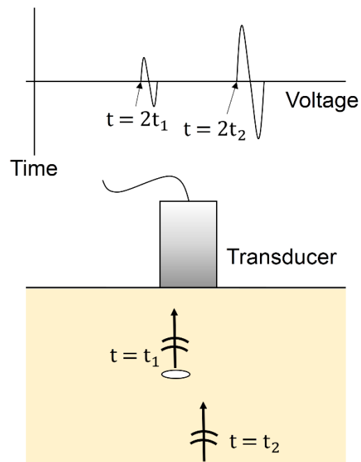
Figure 2.5 A-Scan presentation.
