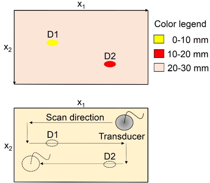
Figure 2.7 C-Scan presentation.
