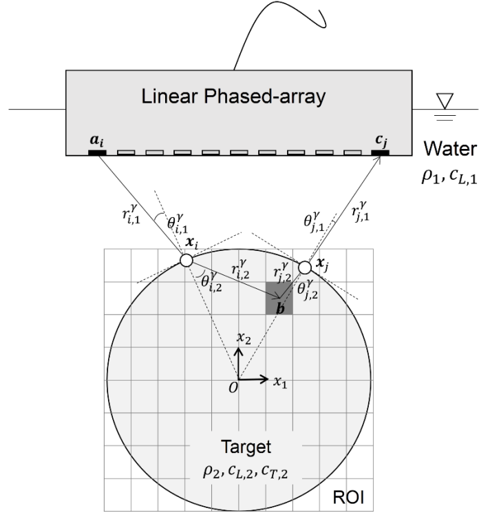
Figure 2.11 Outline of water immersion test.
