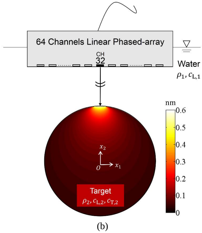
Figure 2.12 L-mode beam radiation; (a) Ch.16 and (b) Ch.32.
