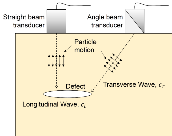
Figure 2.1 Longitudinal and transverse wave modes.
