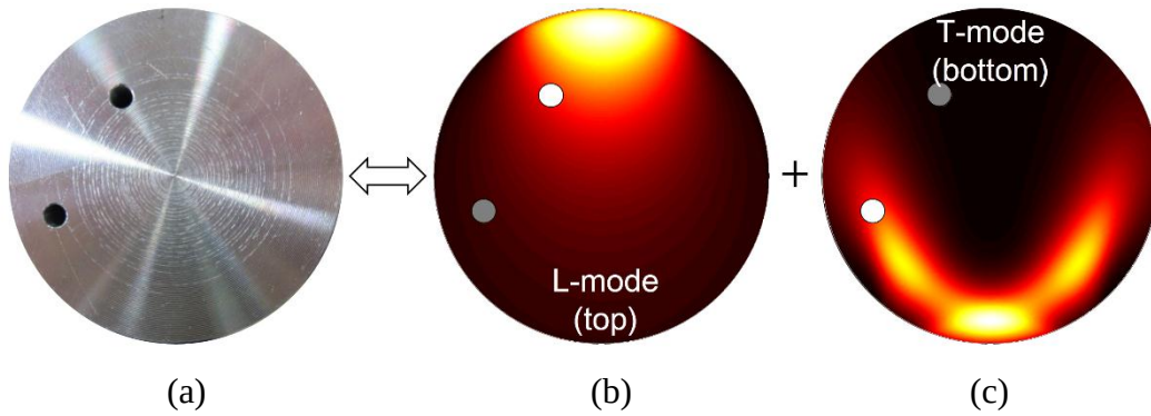
Figure 3.15 (a) Specimen for experiment case 2B and its ER in case of (b) L-mode with transducer on top and (c) T-mode with transducer at the bottom.
