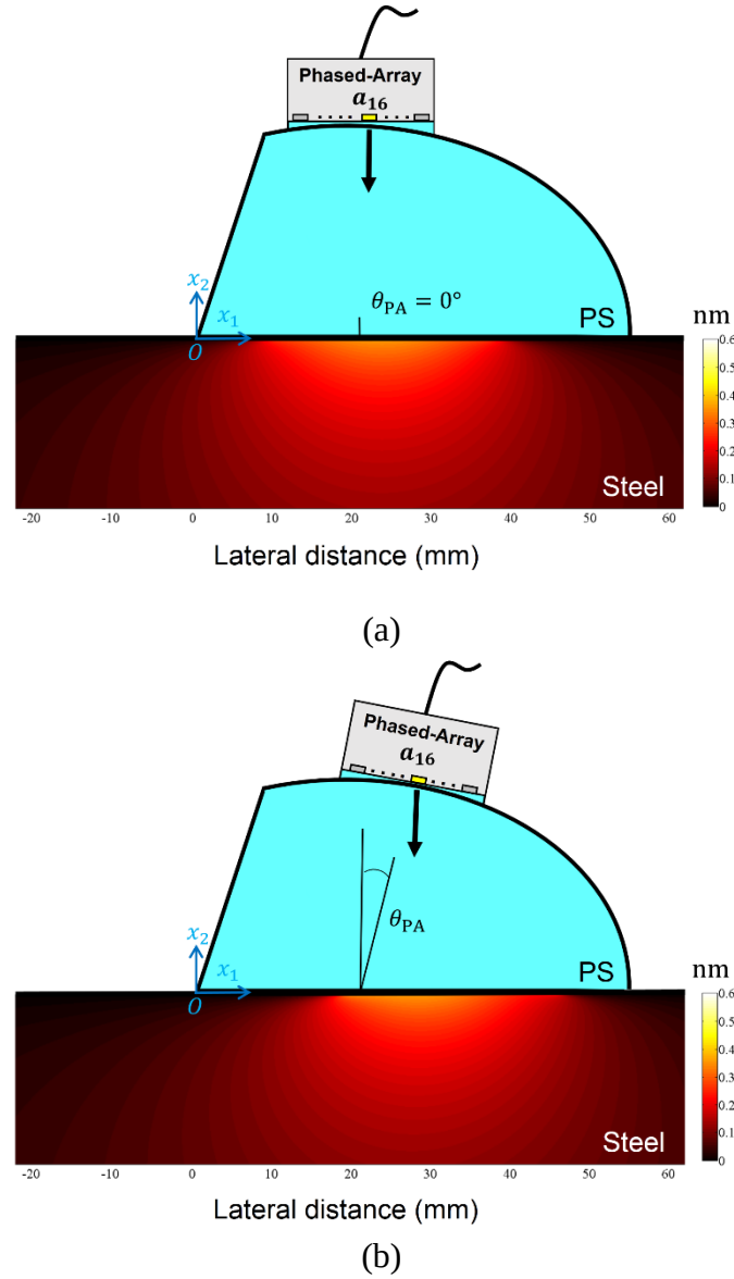
Figure 2.15 L-mode beam radiation models of transducer ch.16;
