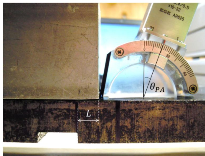
Figure 4.17 Typical setup of experiment in this section.
