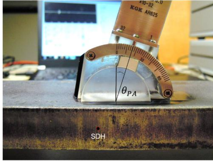
Figure 4.3 Typical setup for experiments in this Chapter.
