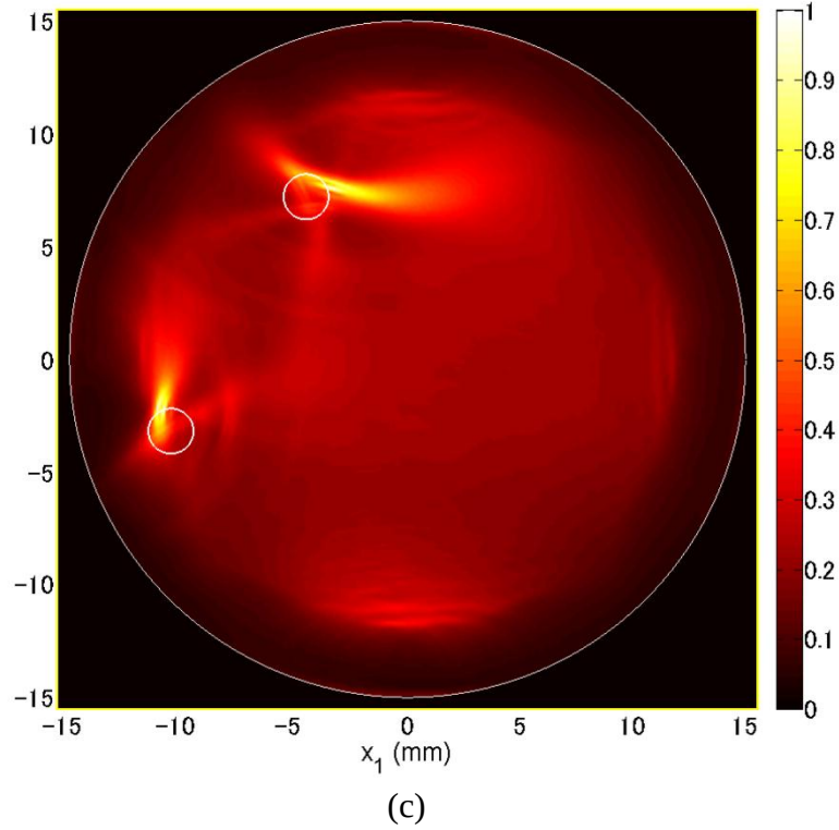
Figure 3.17 (Con't.) Case 2B results where d_1 is inside ER of L-mode and d_2 is inside ER of T-mode; (a) Benchmark, MSSIM = 1; (b) two tests with L- and T-modes, MSSIM = 0.2737 and (c) four tests with L-mode only, MSSIM = 0.2787.
