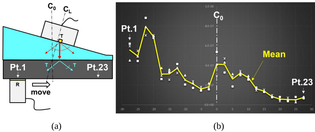
Figure 2.19 T-mode verification of actual beam radiation in two solids media.
