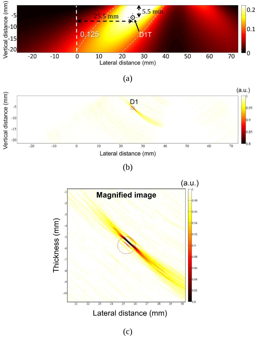
Figure 4.11 Case-T1 results testing \chi = 0.125 ; (a) Outline, (b) SSIM-MAP and (c) Magnified SSIM-MAP.
