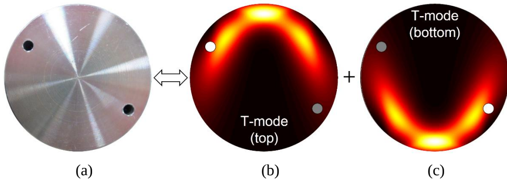
Figure 3.14 (a) Specimen for experiment case 2A and its ER in case of (b) T-mode with transducer on top and (c) T-mode with transducer at the bottom.
