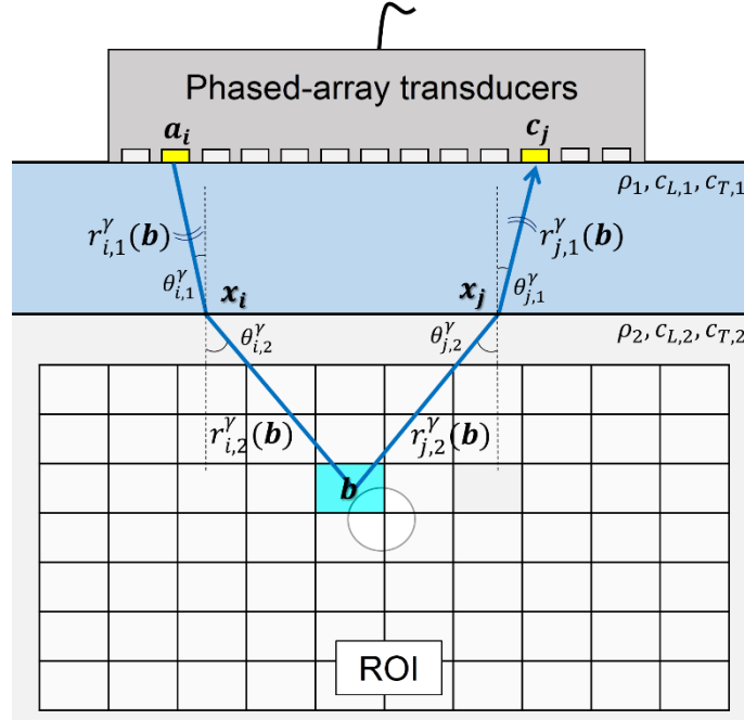
Figure 2.10 Outline for SAFT in a two media case.
