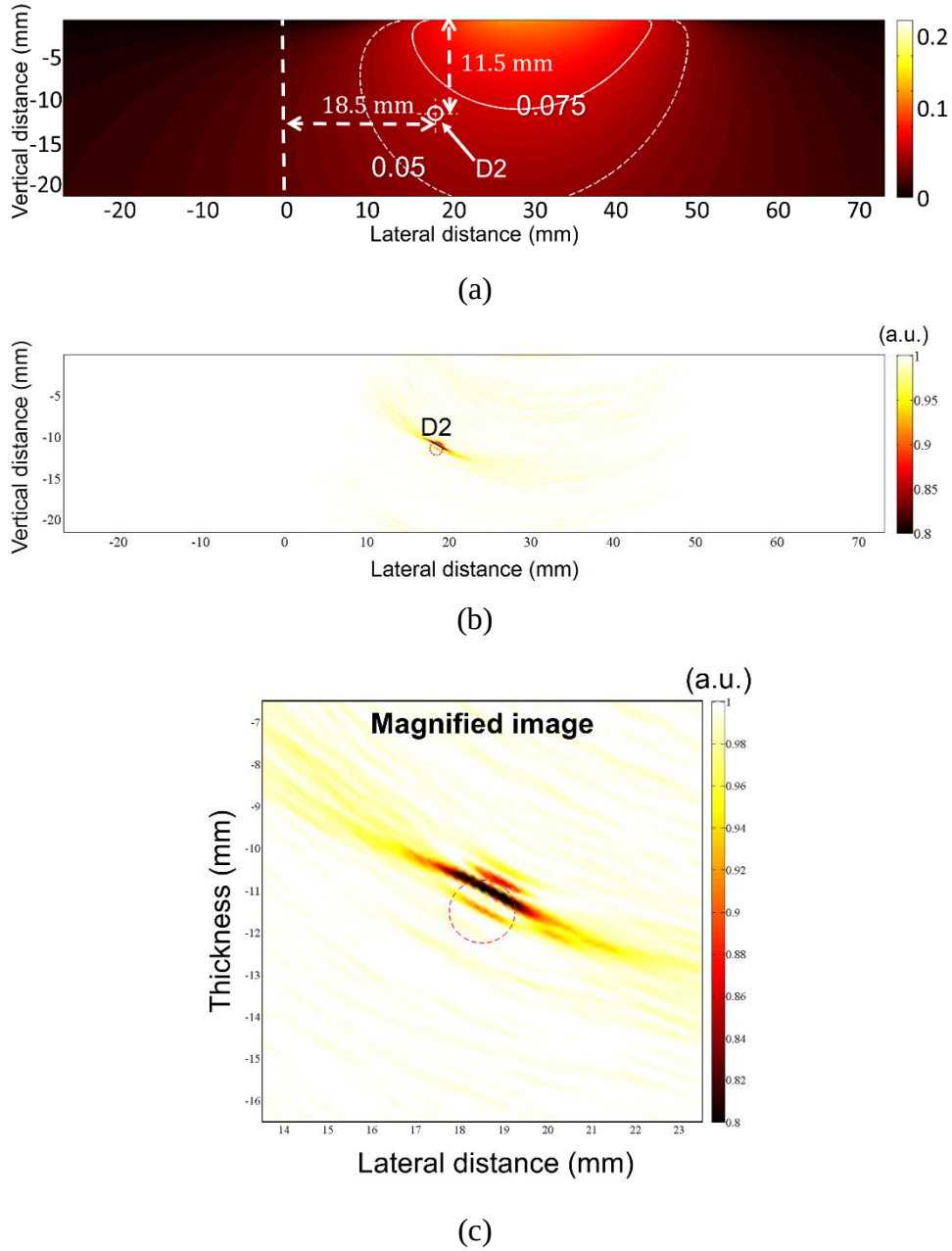
Figure 4.9 Case-L2 results testing \chi = 0.05 ; (a) Outline, (b) SSIM-MAP and (c) Magnified SSIM-MAP.
