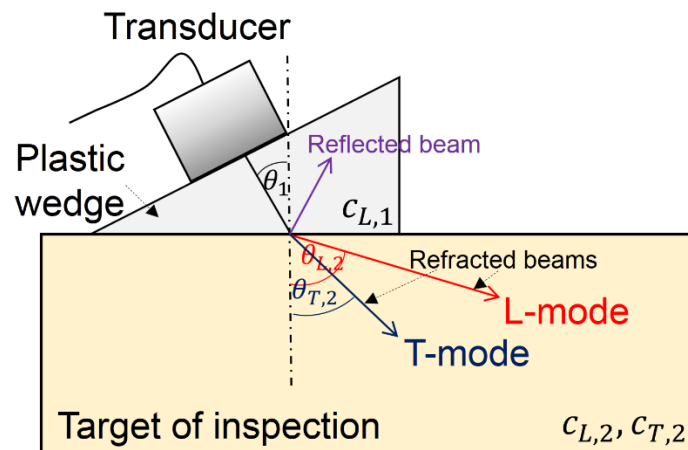
Figure 2.2 Wave refractions at the interface.
