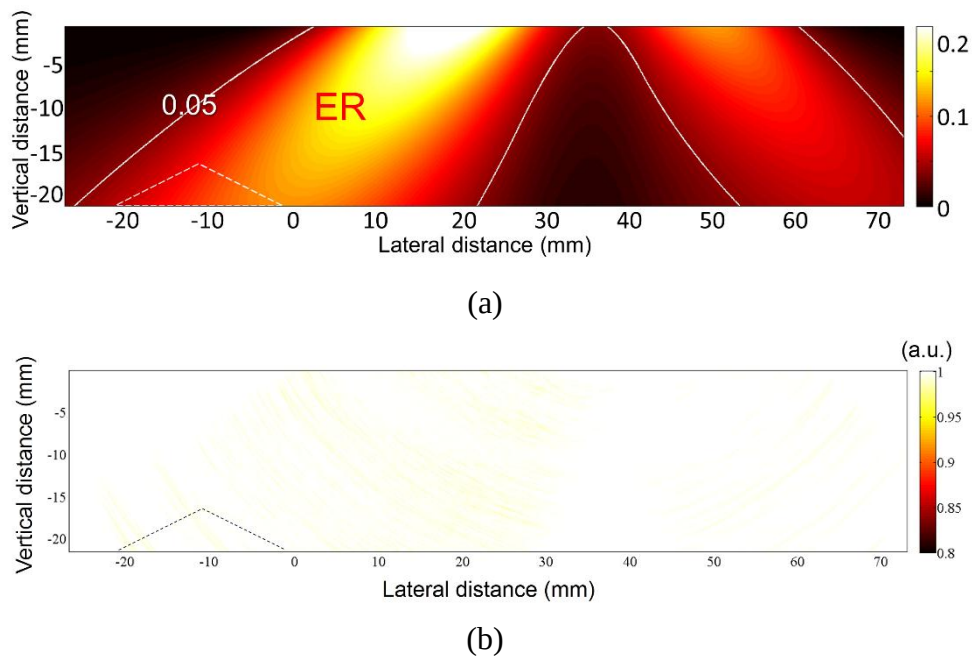
Figure 4.22 Triangular notch: L = 1 mm T-mode; (a) ER and (b) SSIM-MAP.
