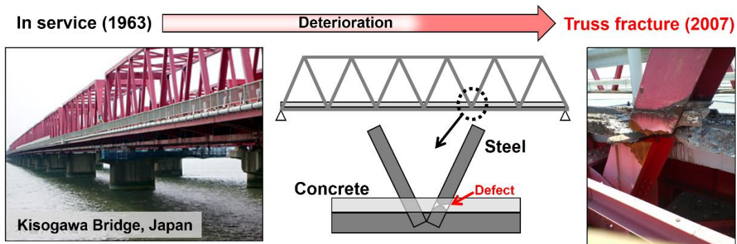
Figure 4.15 Photo and illustration of Kisogawa bridge case.
