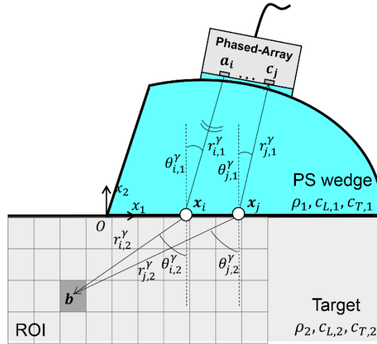
Figure 2.14 Outline of angle beam test.
