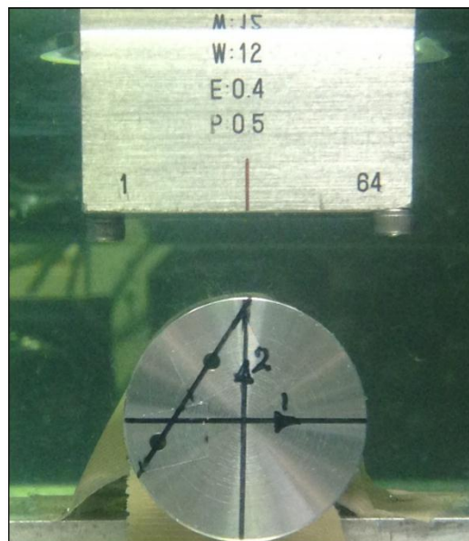
Figure 3.5 Photo of experimental setup.
