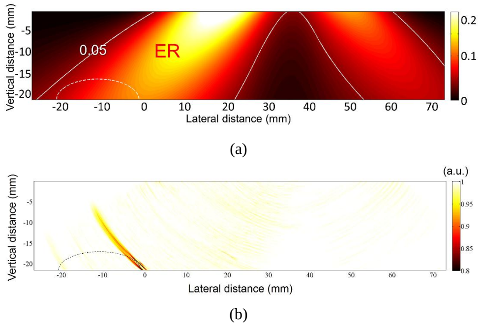
Figure 4.21 Circular notch: L = 1 mm T-mode; (a) ER and (b) SSIM-MAP.
