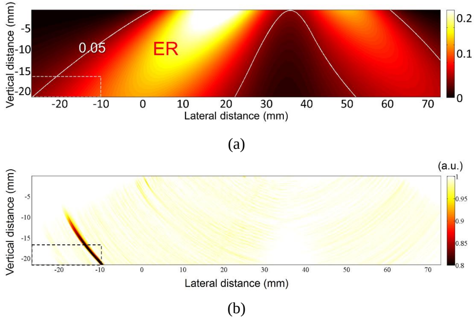
Figure 4.19 Case-2: L = 10 mm T-mode; (a) ER and (b) SSIM-MAP.
