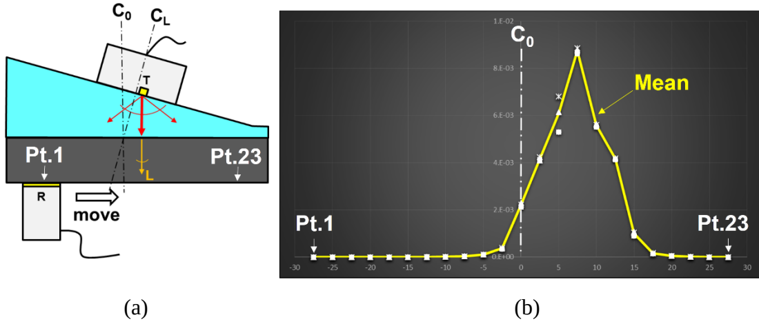
Figure 2.18 L-mode verification of actual beam radiation in two solids media.
