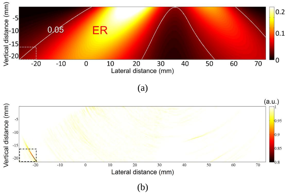
Figure 4.20 Case-3: L = 20 mm T-mode; (a) ER and (b) SSIM-MAP.
