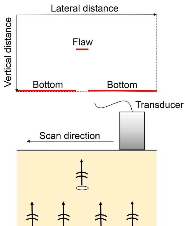
Figure 2.6 B-Scan presentation.
