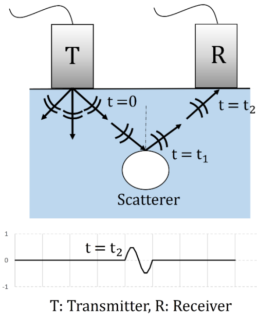
Figure 2.4 Pitch-catch test configuration.
