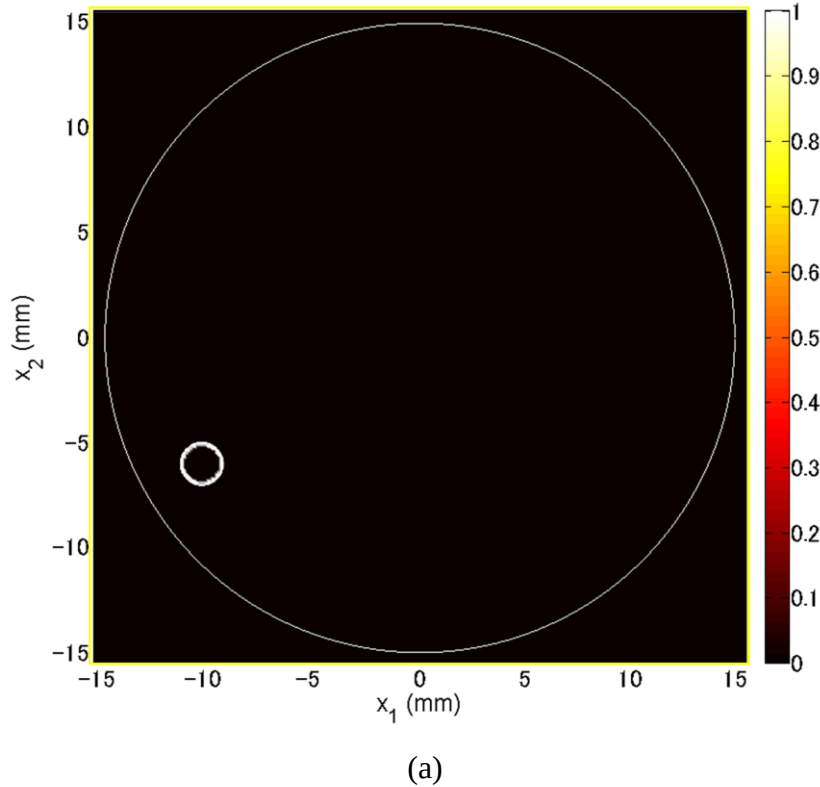
Figure 3.12 Case 1D results when SDH is outside the effective zone of T-mode. (a) Benchmark, MSSIM = 1; (b) SAFT, MSSIM = 0.2740 and (c) AWS-SAFT, MSSIM = 0.3956.
