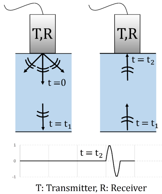
Figure 2.3 Pulse-echo test configuration.
