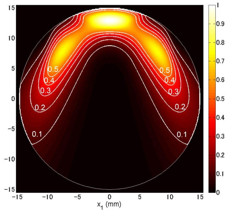
Figure 3.7 T-mode summed AWS beam radiations from all 64 transducers; \sum_i \sum_j |u_i^T u_j^T| .
