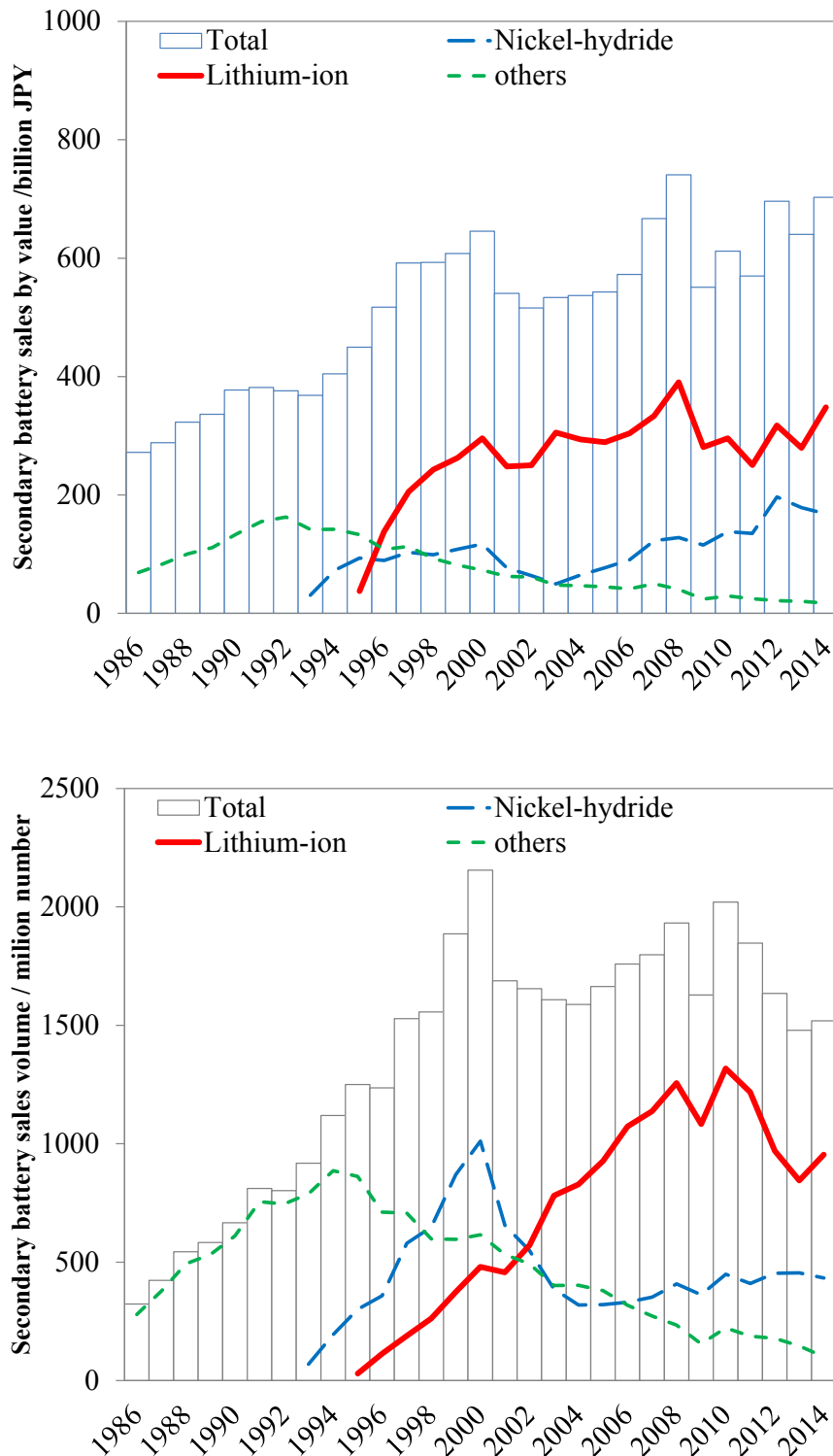
Figure 1-1 The secondary battery sales by (a) value and by (b) volume since the statistics for the secondary battery sales.
