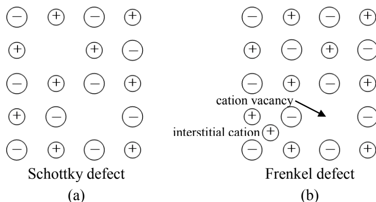
Figure 1-6 Types of point defect in ionic crystals.
