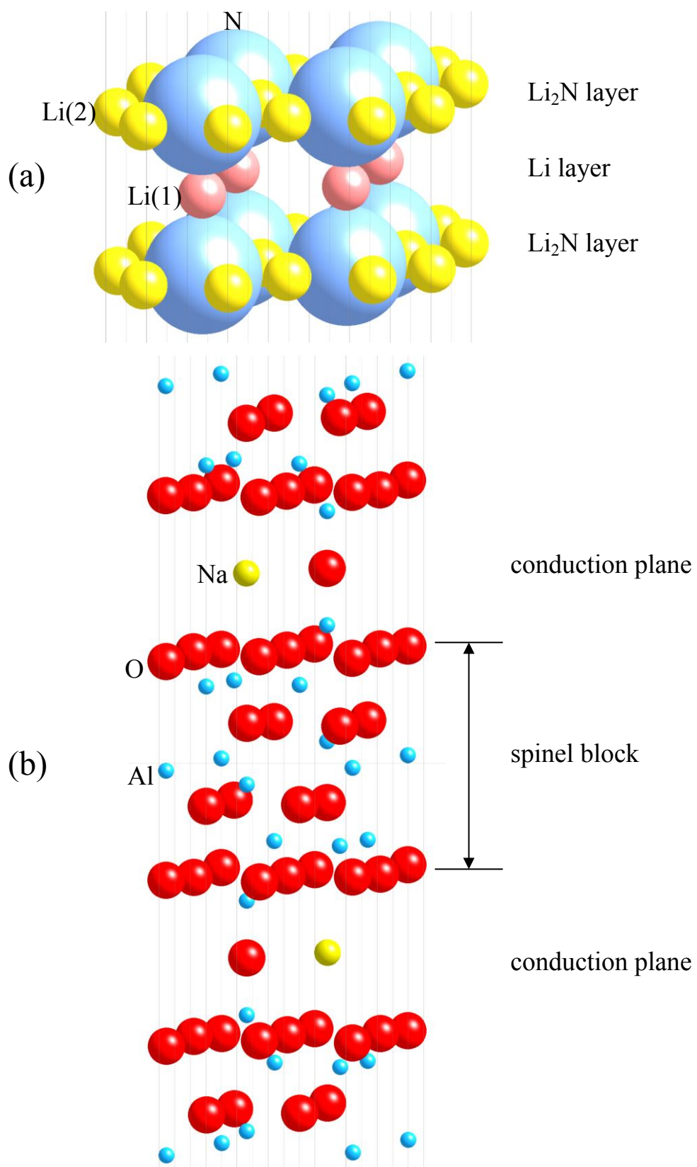
Figure 1-2 Structure of \text{Li}_3\text{N} (a), and \beta -Alumina (b).
