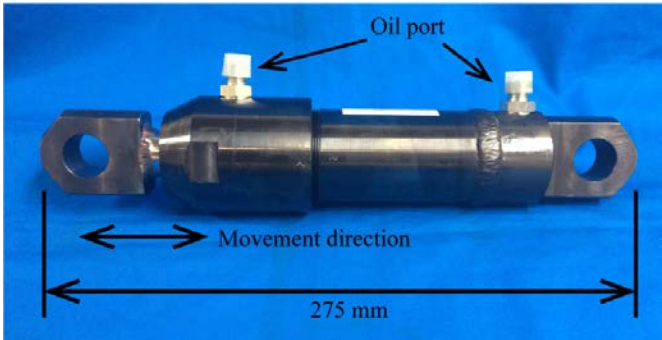
Fig.1: Developed hydraulic cylinder
